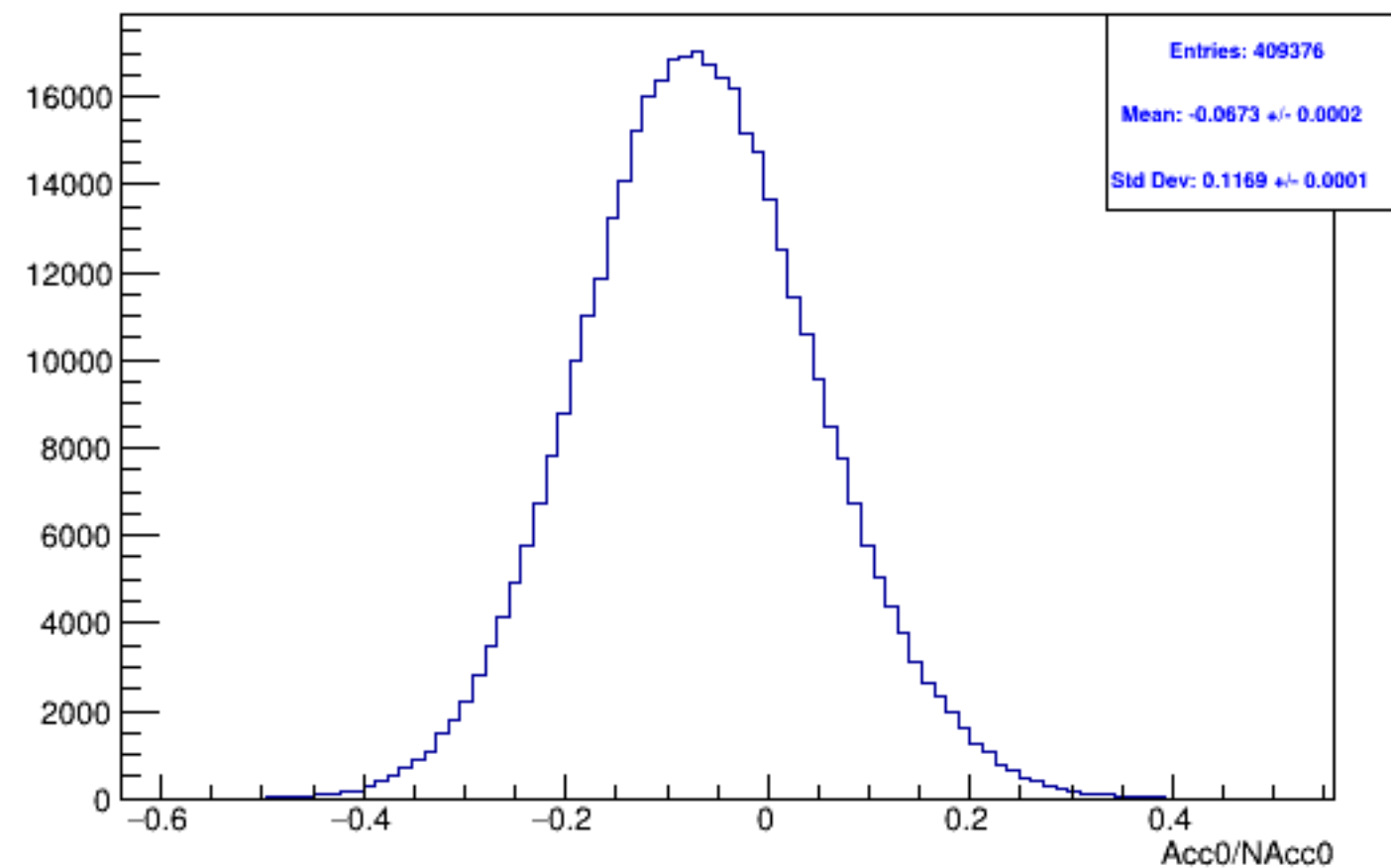
Run 5411 mpwise, acc0: Beam OFF
