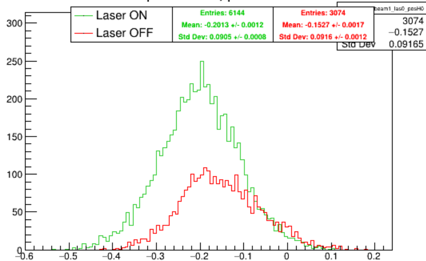
Run 5412 quartetwise, posH0: Beam ON
