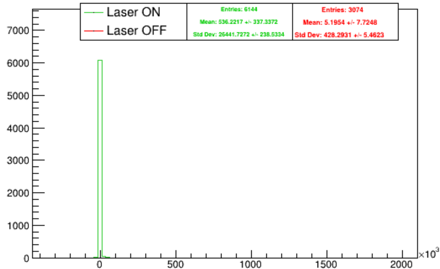
Run 5412 quartetwise, asym0sub: Beam ON
