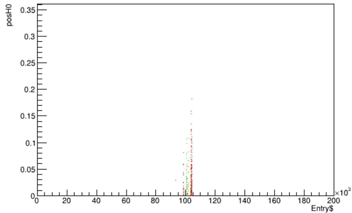
Run 5412 quartetwise, posH0 vs time
