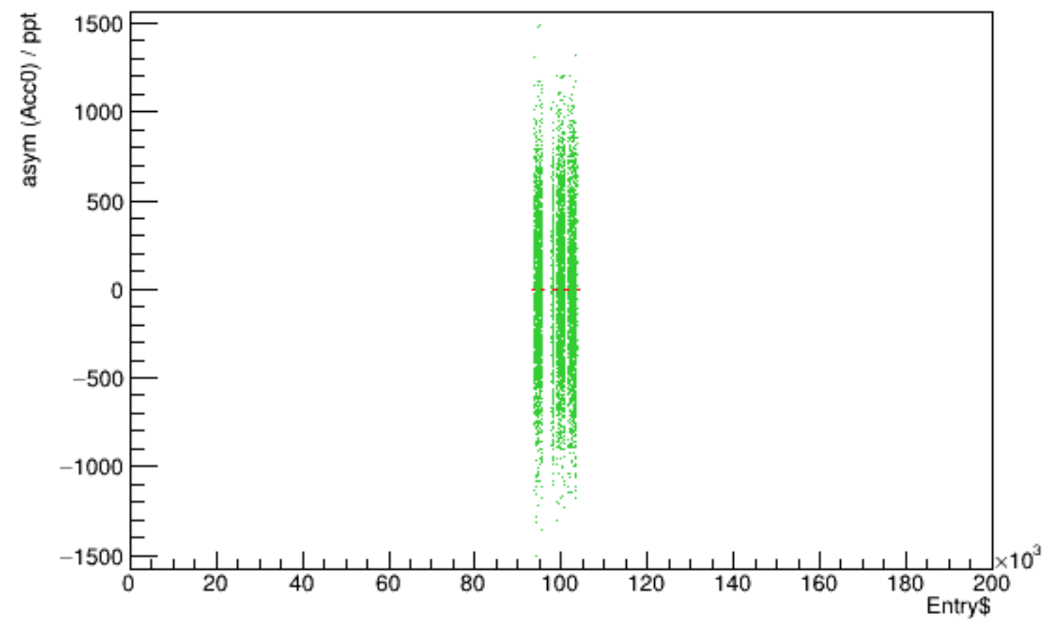
Run 5412 quartetwise, asym0sub vs time
