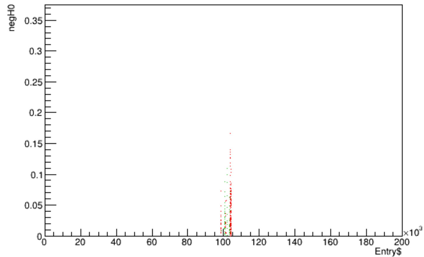
Run 5412 quartetwise, negH0 vs time
