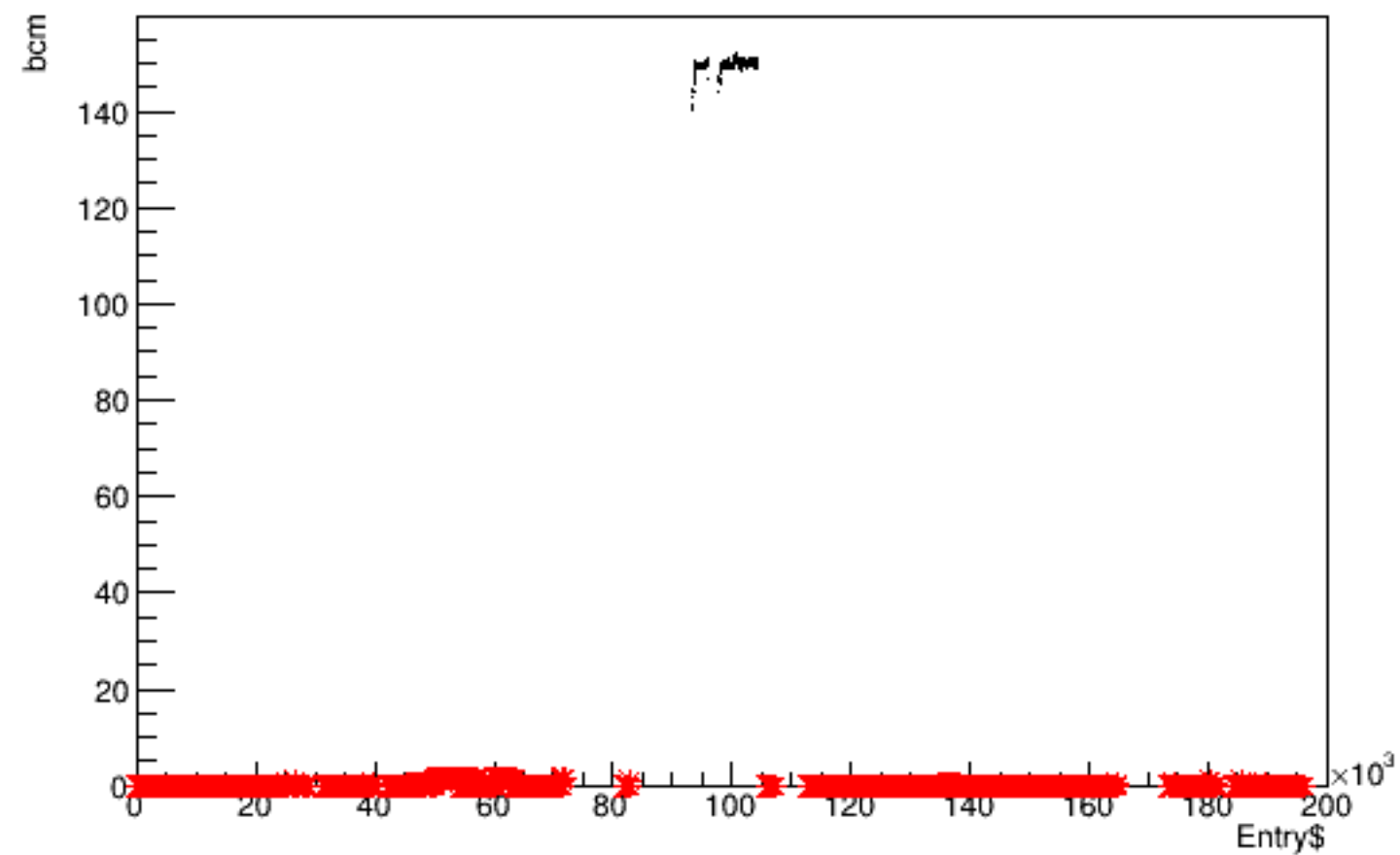
Run 5412 quartetwise, bcm vs time
