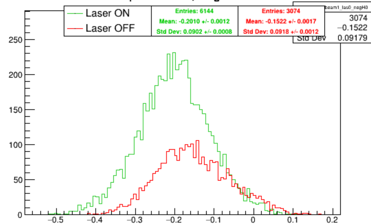
Run 5412 quartetwise, negH0: Beam ON
