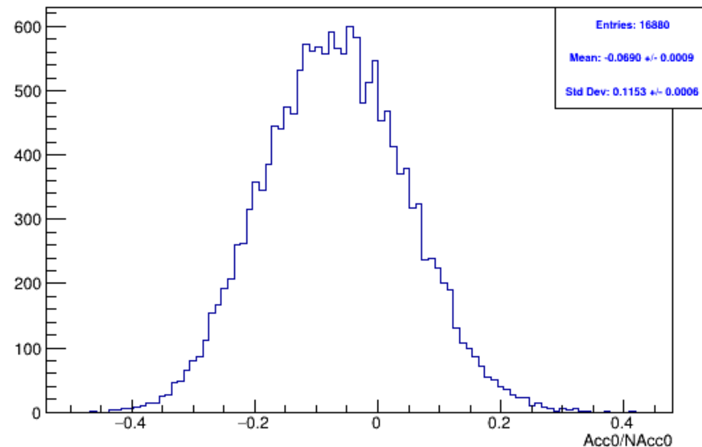
Run 5418 mpwise, acc0: Beam OFF
