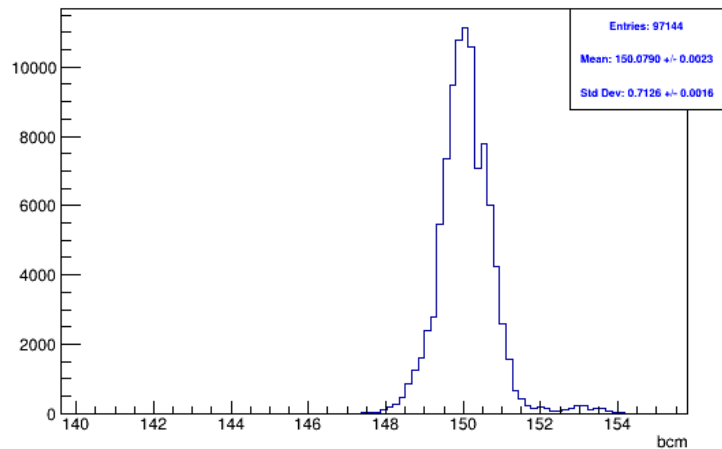
Run 5418, mpwise, BCM: Beam ON, Laser ON
