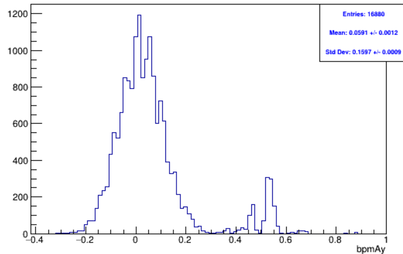
Run 5418 mpwise, bpmAy: Beam OFF
