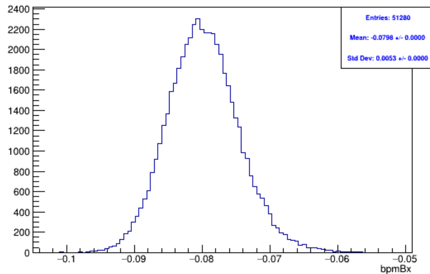
Run 5418, mpswise, bpmBx: Beam ON, Laser OFF
