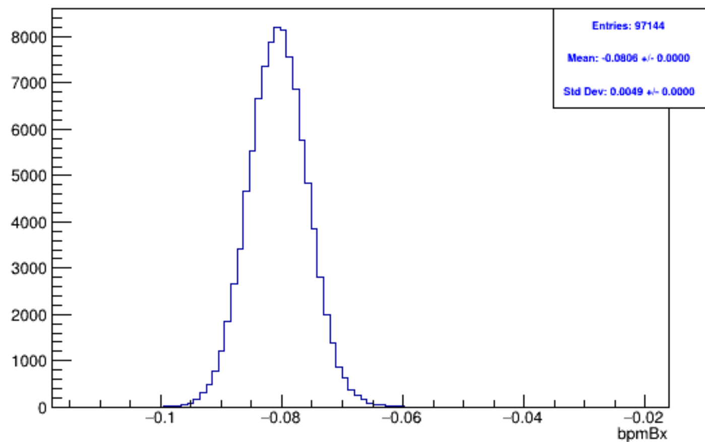
Run 5418, mpswise, bpmBx: Beam ON, Laser ON
