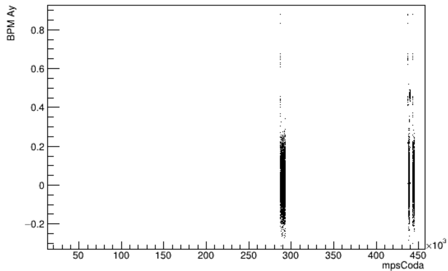
Run 5418 mpwise, beam OFF, laser ON
