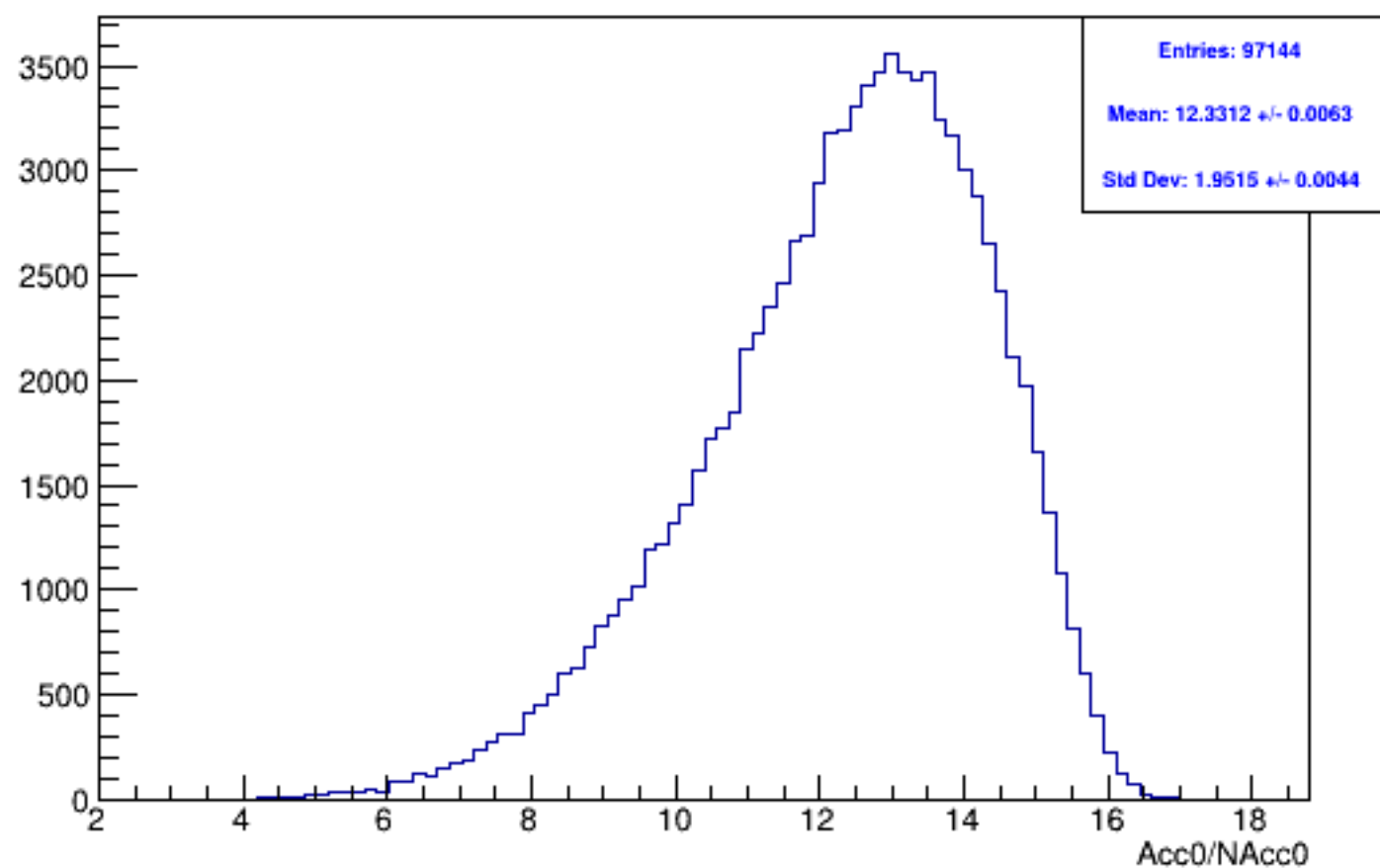
Run 5418, mpwise, acc0: Beam ON, Laser ON
