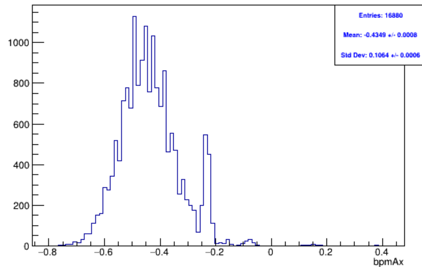
Run 5418 mpwise, bpmAx: Beam OFF
