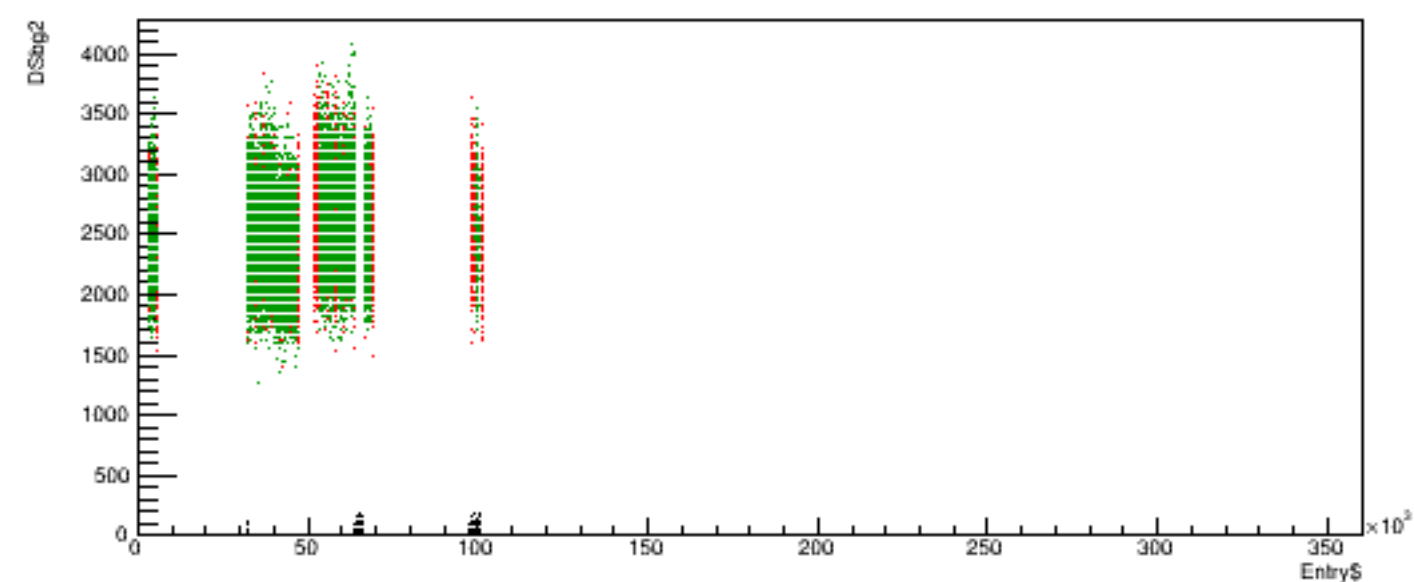
Run 5418 quartetwise, DSbg2 vs time
