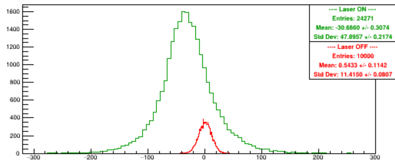
Run 5418 quartetwise, Asyms0
