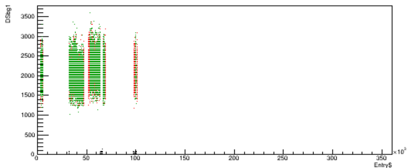
Run 5418 quartetwise, DSbg1 vs time
