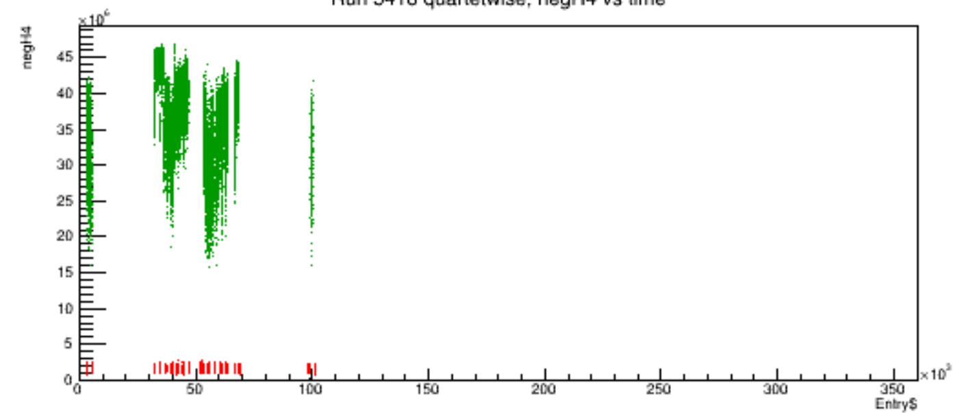
Run 5418 quartetwise, negH4 vs time
