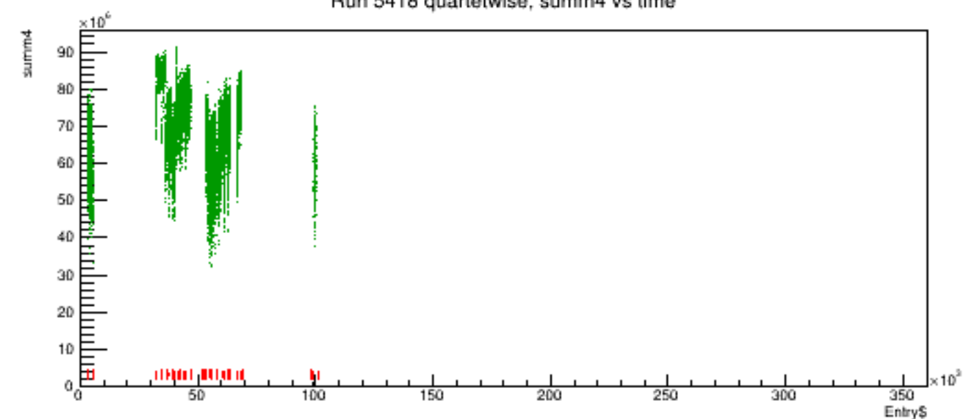
Run 5418 quartetwise, summ4 vs time
