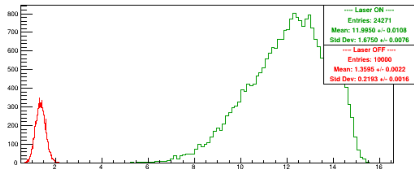
Run 5418 quartetwise, PosHelAcc0/NSamples0
