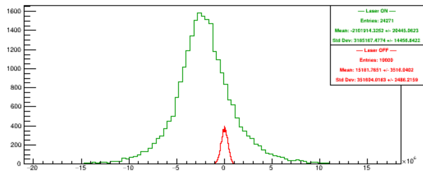
Run 5418 quartetwise, Diffs4
