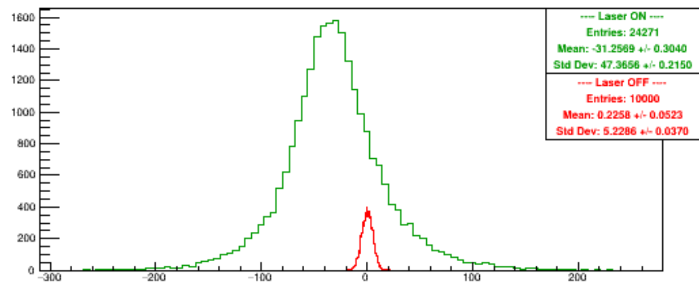
Run 5418 quartetwise, Asyms4
