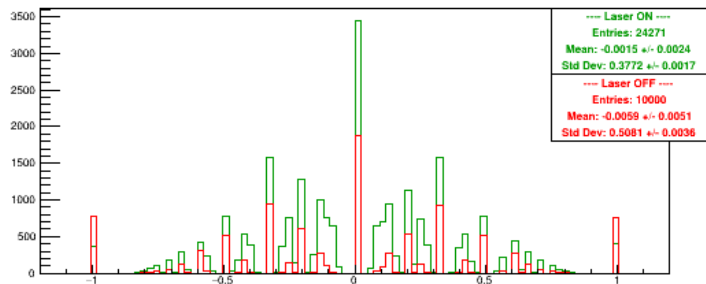
Run 5418 quartetwise, Asyms Horiz Finger
