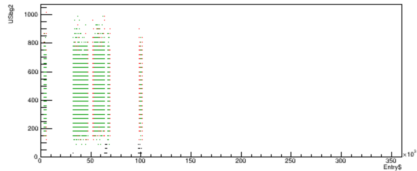
Run 5418 quartetwise, USbg2 vs time
