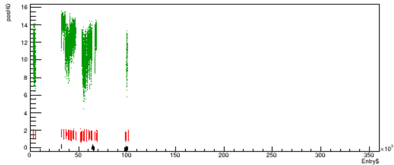
Run 5418 quartetwise, posH0 vs time
