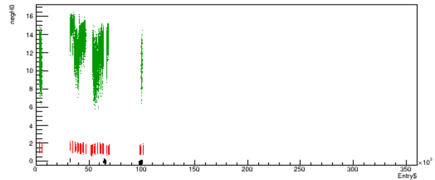
Run 5418 quartetwise, negH0 vs time
