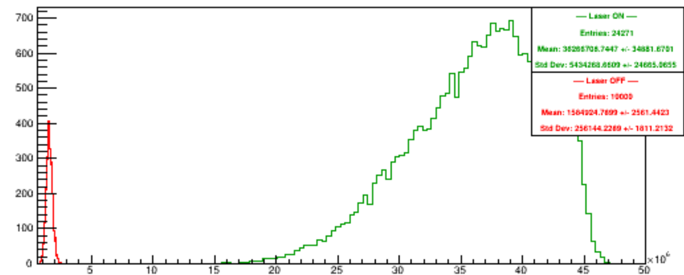
Run 5418 quartetwise, NegHelAcc4
