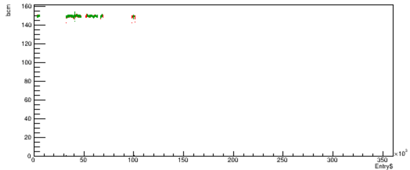
Run 5418 quartetwise, posH4 vs time
