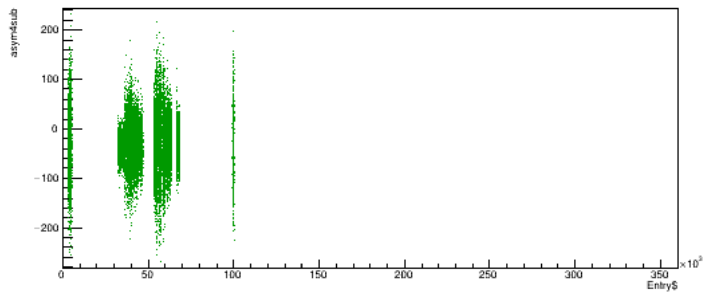
Run 5418 quartetwise, asym4sub vs time
