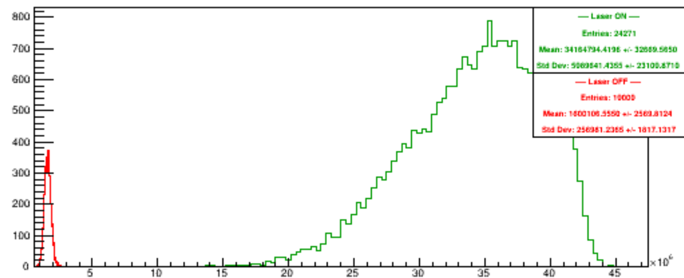
Run 5418 quartetwise, PosHelAcc4
