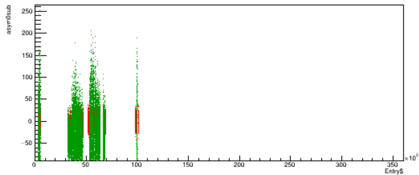
Run 5418 quartetwise, asym0sub vs time
