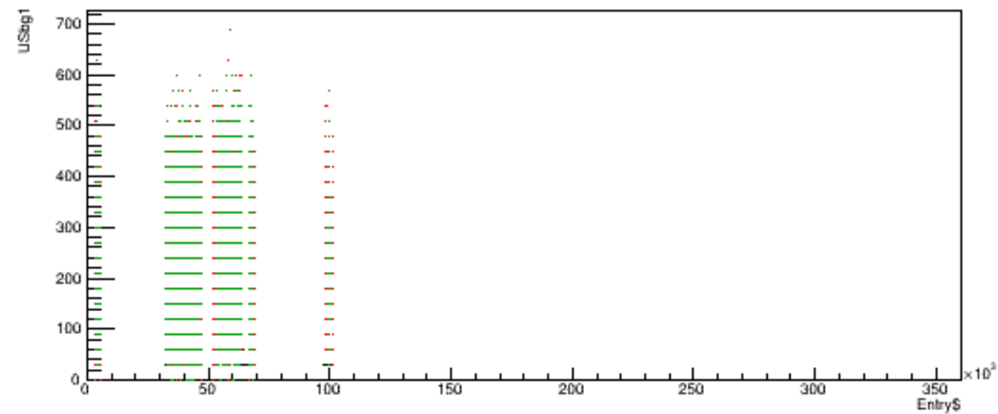
Run 5418 quartetwise, USbg1 vs time
