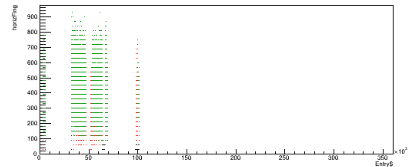
Run 5418 quartetwise, horizFing vs time
