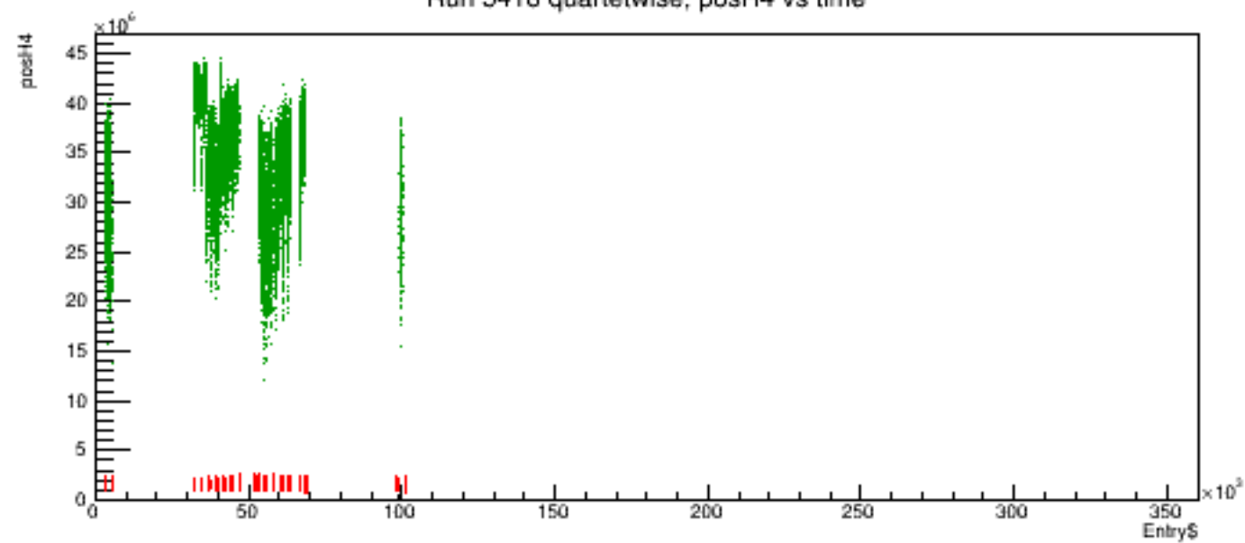
Run 5418 quartetwise, posH4 vs time
