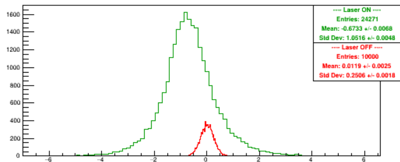
Run 5418 quartetwise, Diffs0
