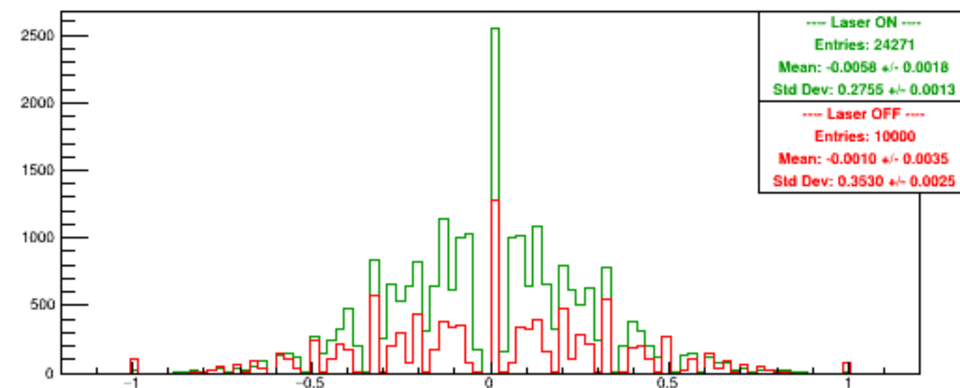
Run 5418 quartetwise, Asyms Vert Finger
