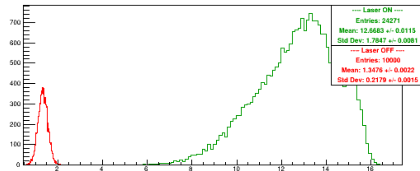
Run 5418 quartetwise, NegHelAcc0/NSamples0
