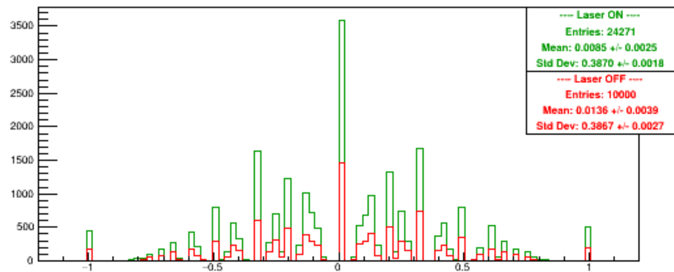
Run 5418 quartetwise, Asyms USbg1
