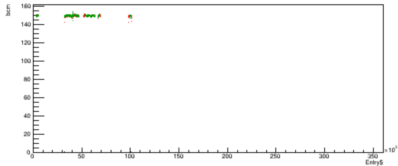
Run 5418 quartetwise, posH4 vs time
