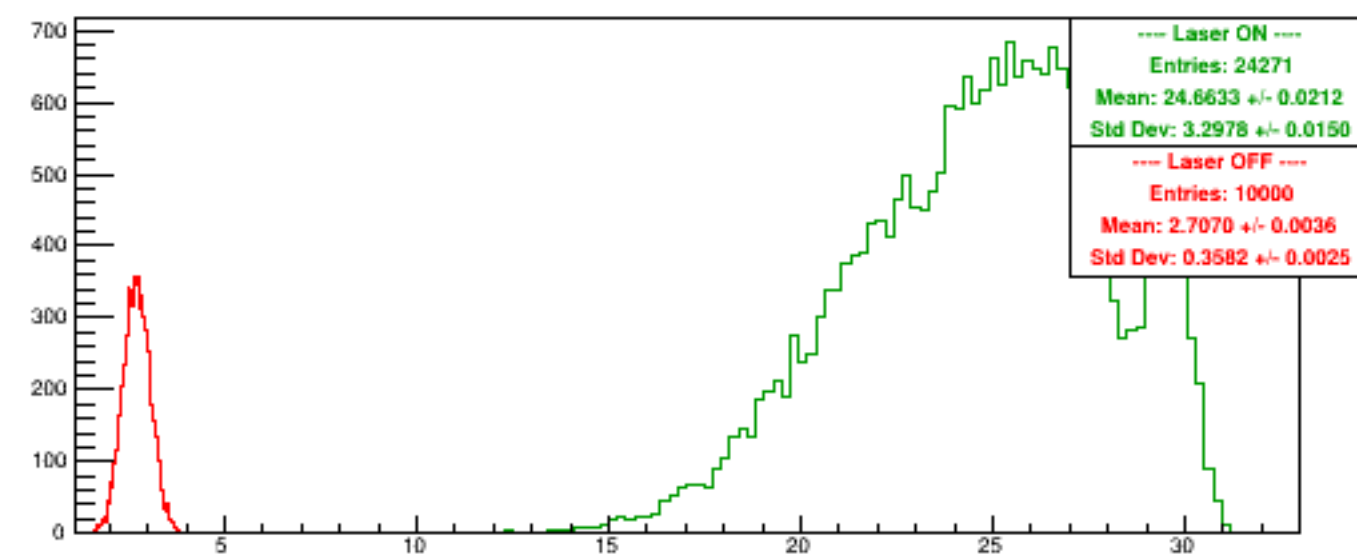
Run 5418 quartetwise, Sums0
