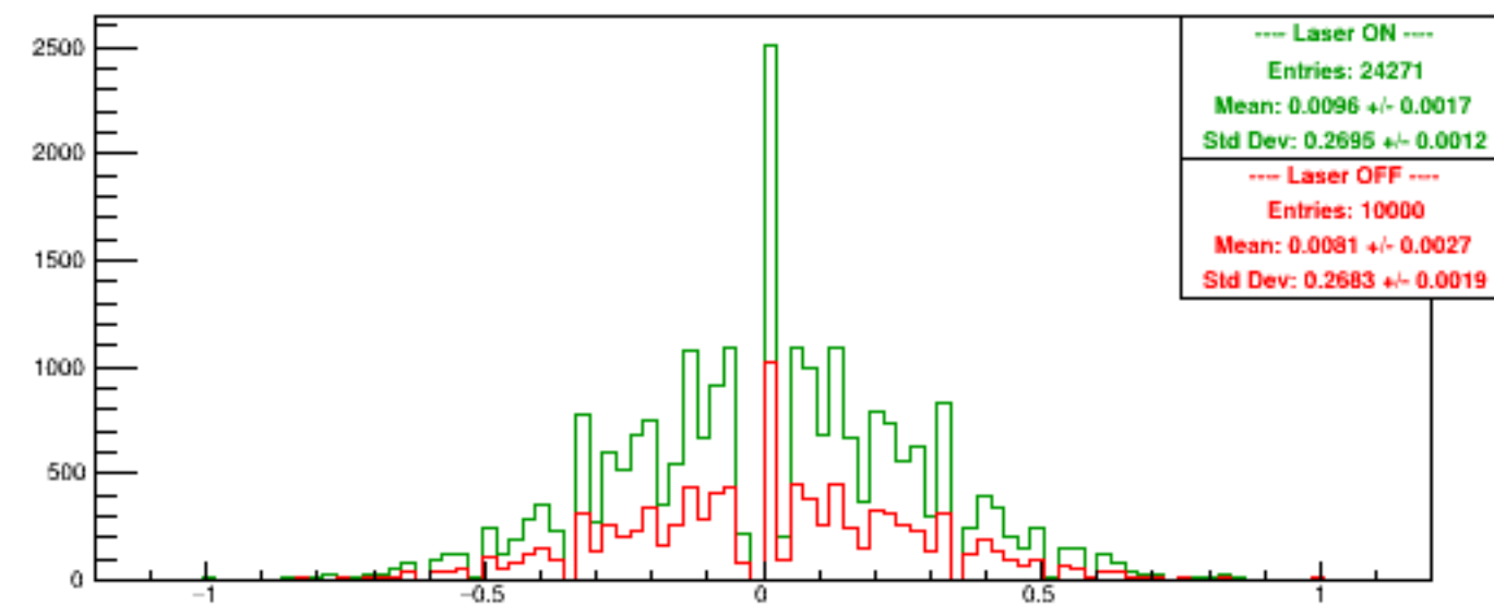
Run 5418 quartetwise, Asyms USbg2
