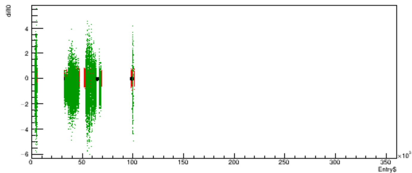
Run 5418 quartetwise, diff0 vs time
