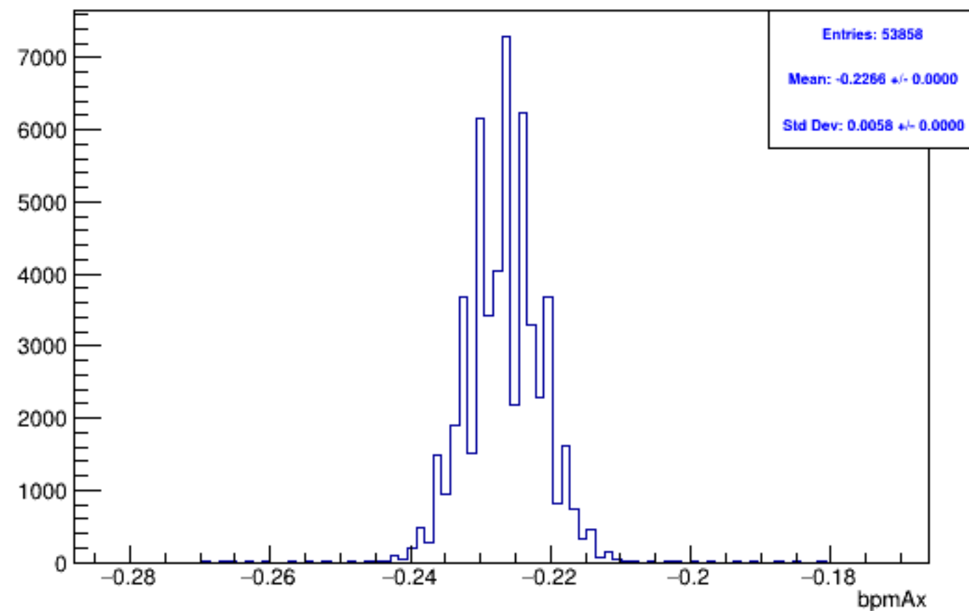
Run 5419, mpwise, bpmAx: Beam ON, Laser OFF
