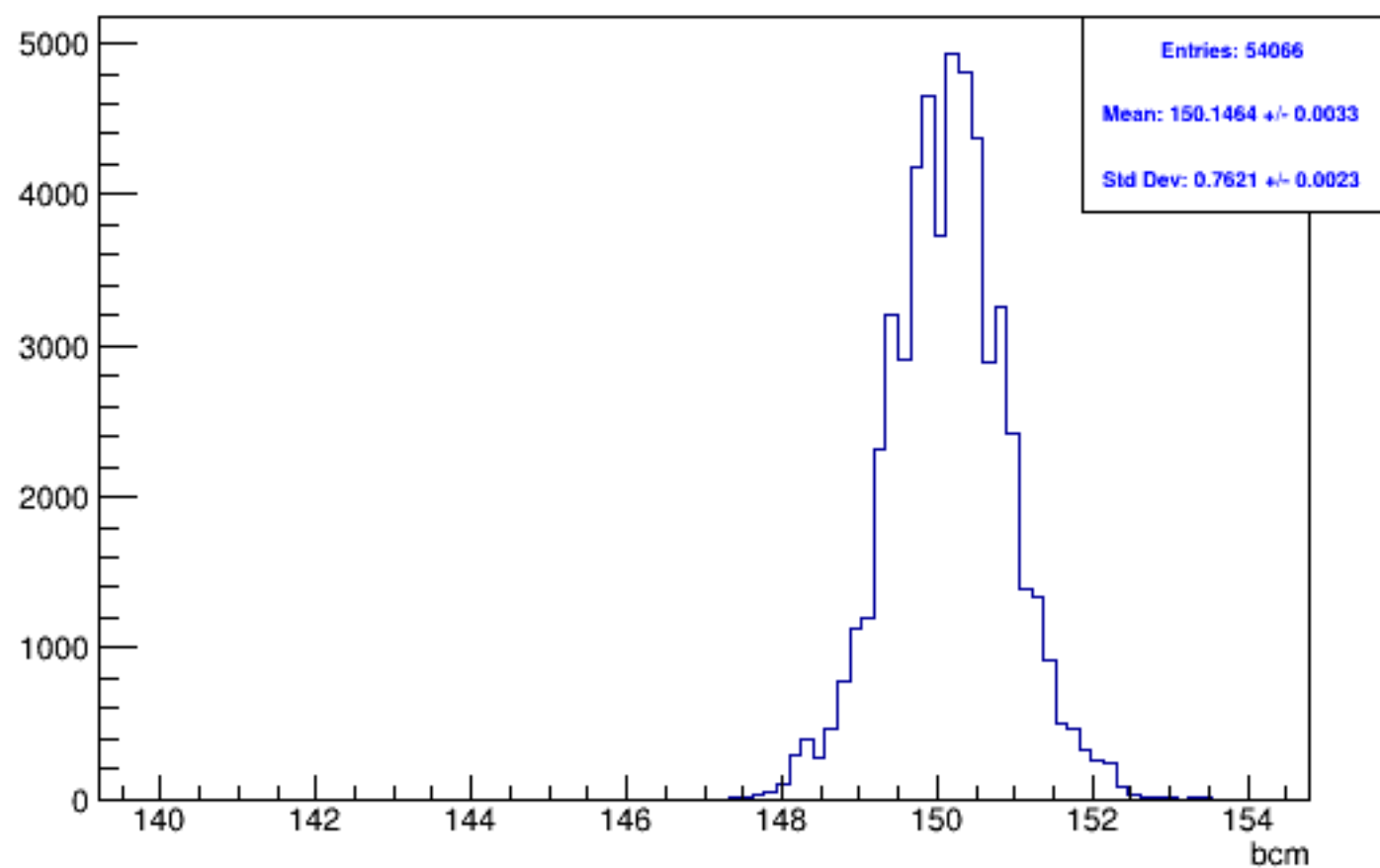
Run 5419, mpwise, BCM: Beam ON, Laser ON
