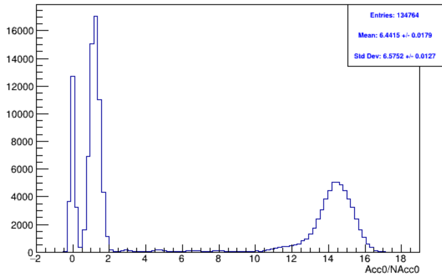
Run 5419 mpwise, acc0: All
