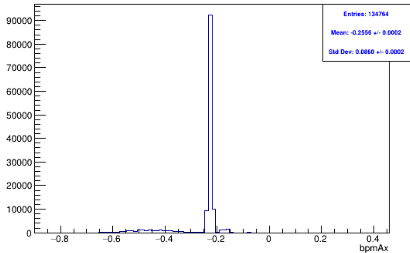
Run 5419 mpwise, bpmAx: All
