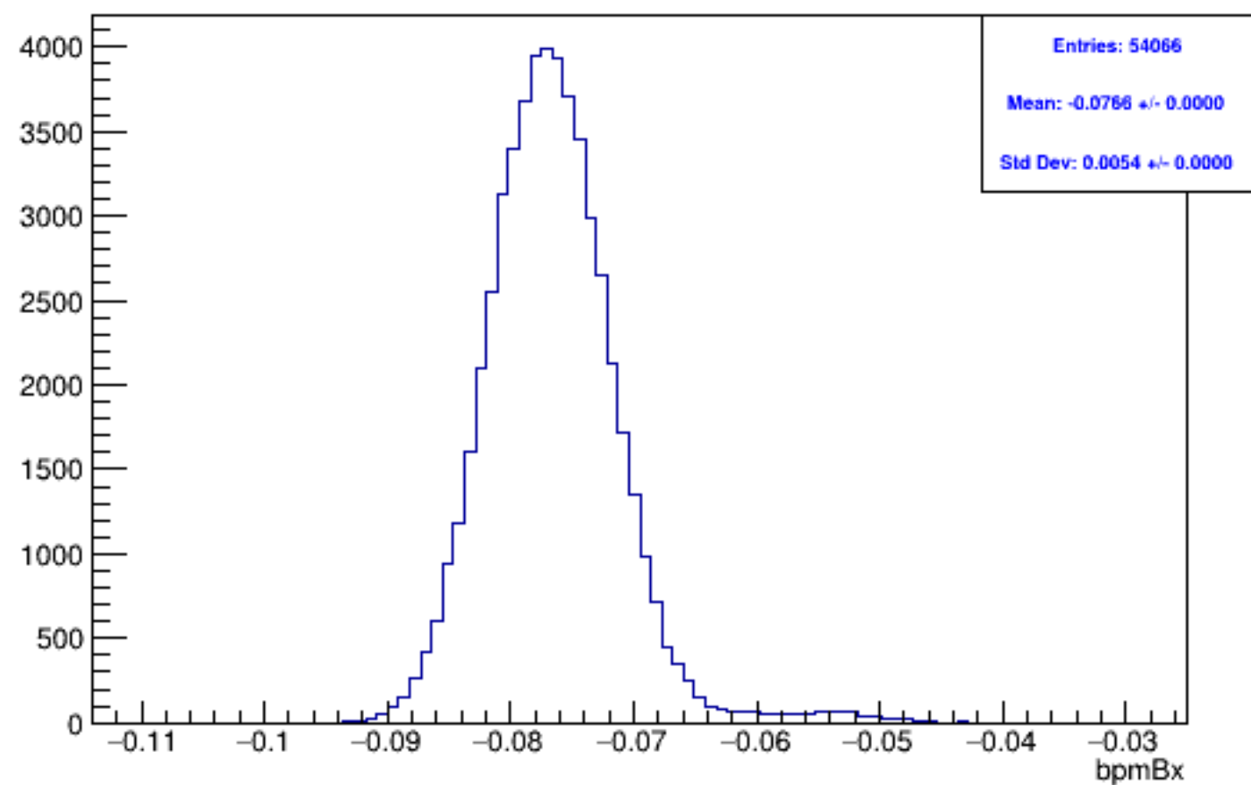
Run 5419, mpswise, bpmBx: Beam ON, Laser ON
