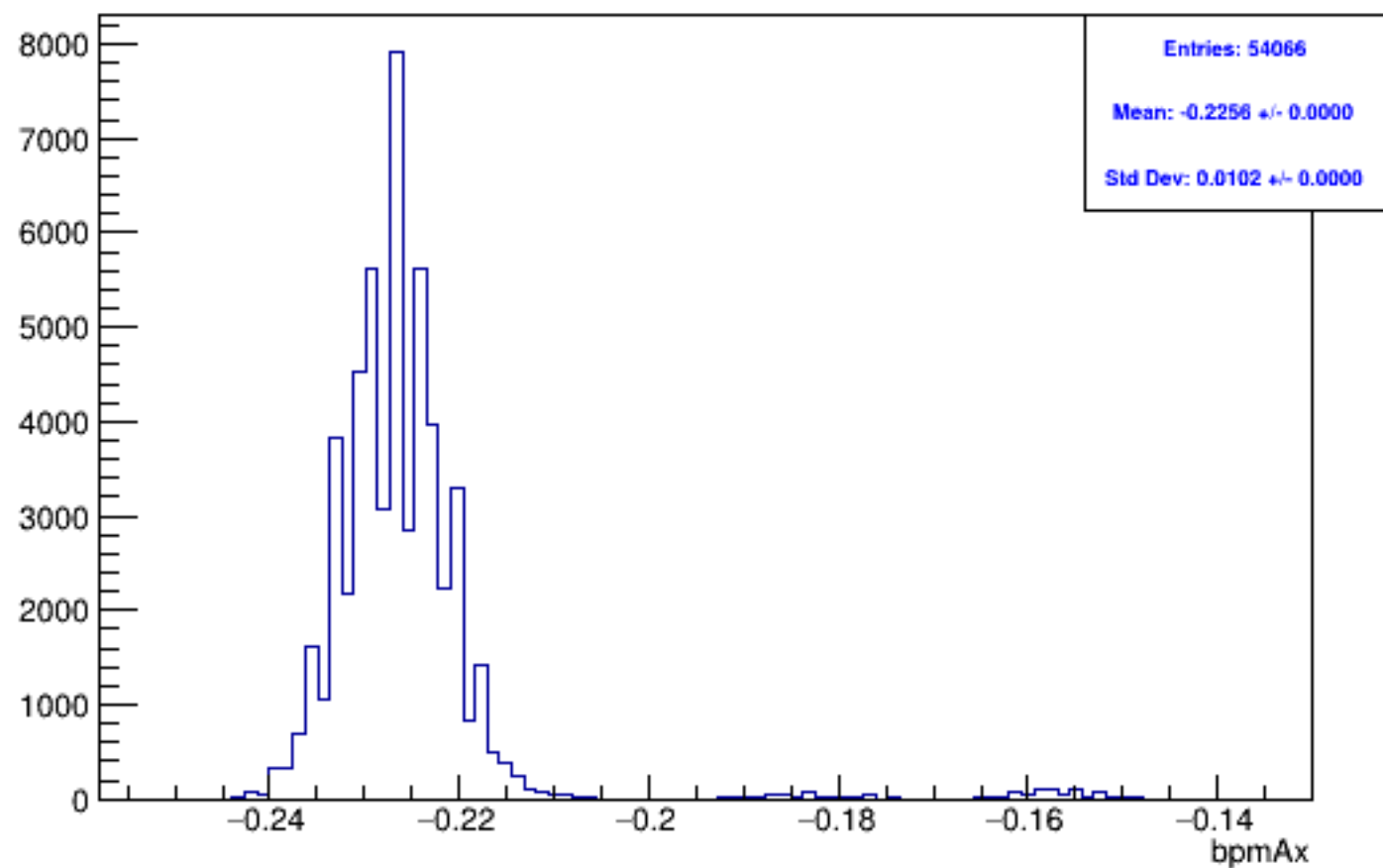
Run 5419, mpwise, bpmAx: Beam ON, Laser ON
