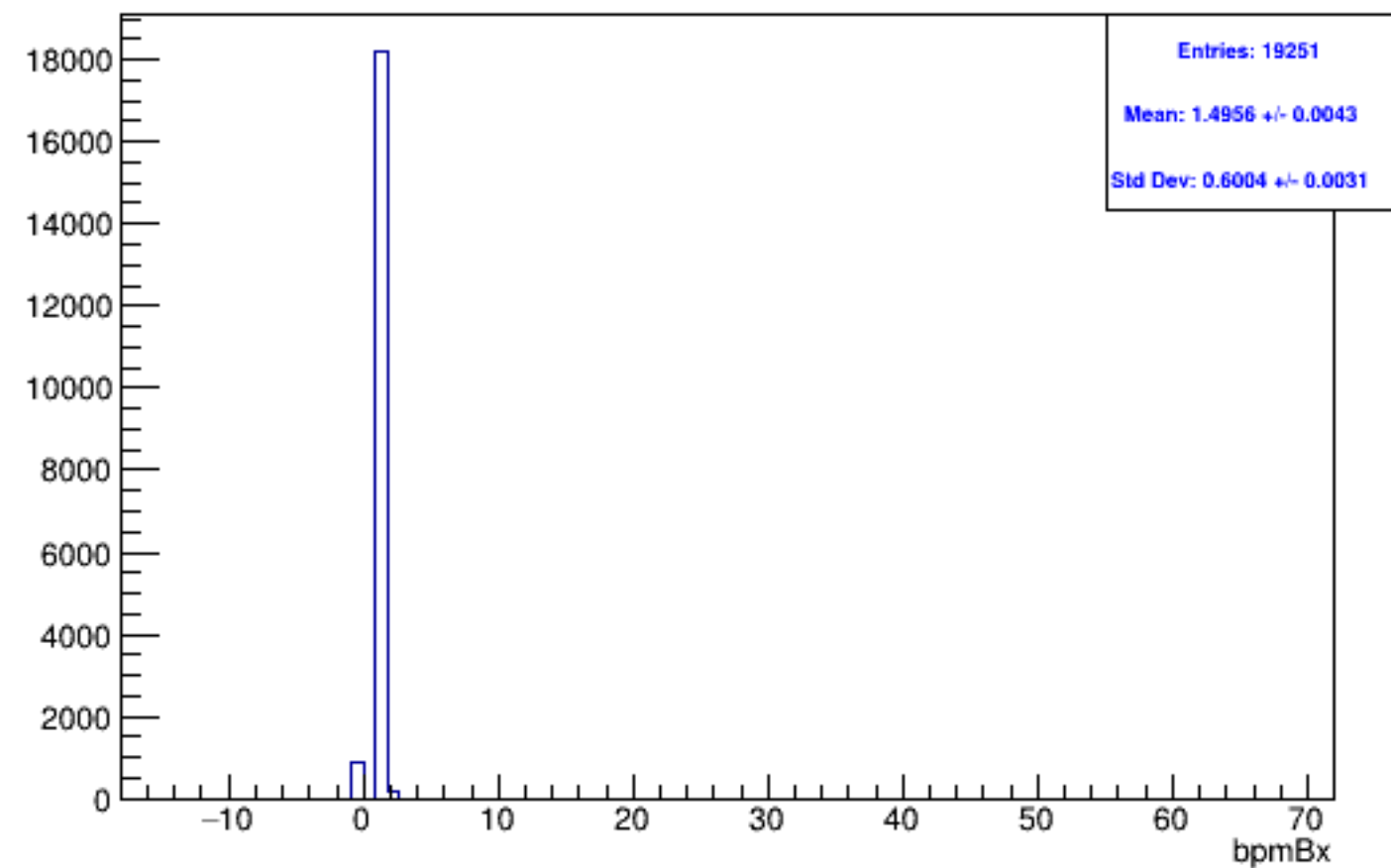
Run 5419 mpswise, bpmBx: Beam OFF
