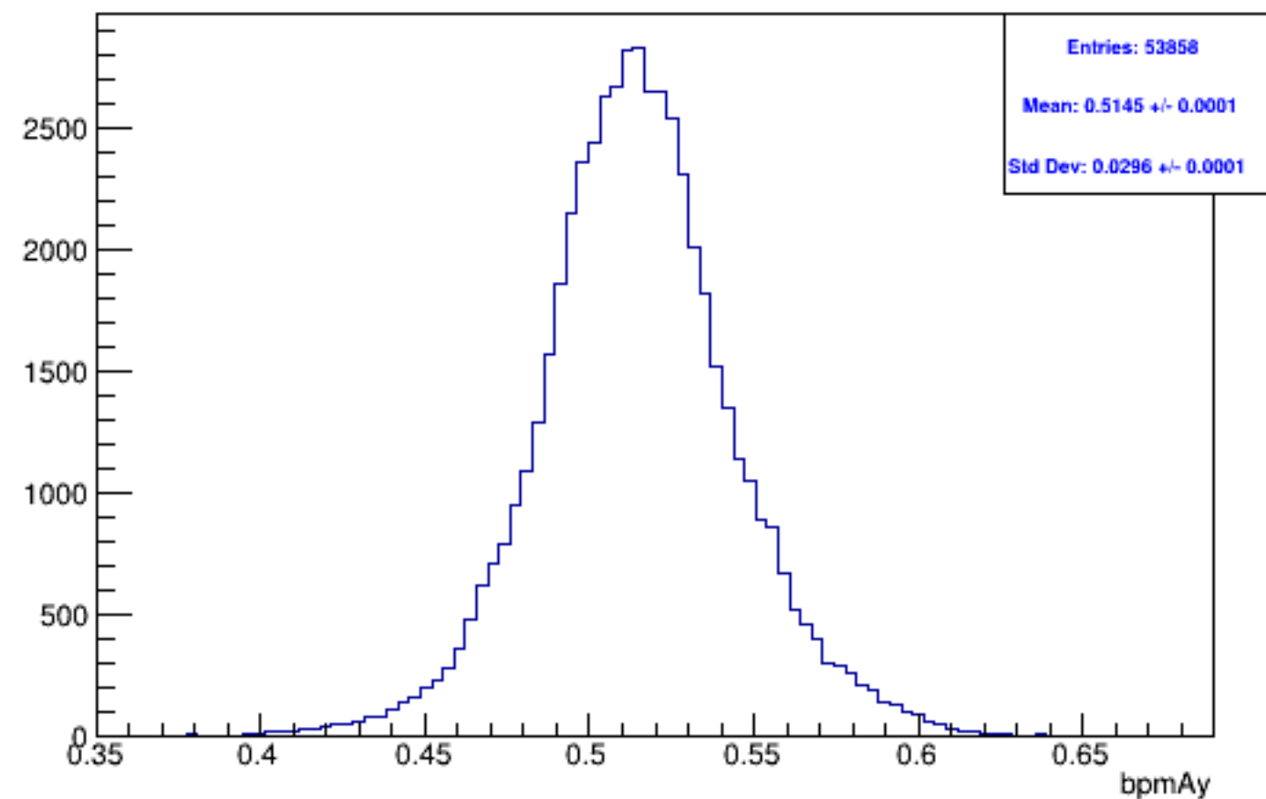
Run 5419, mpwise, bpmAy: Beam ON, Laser OFF
