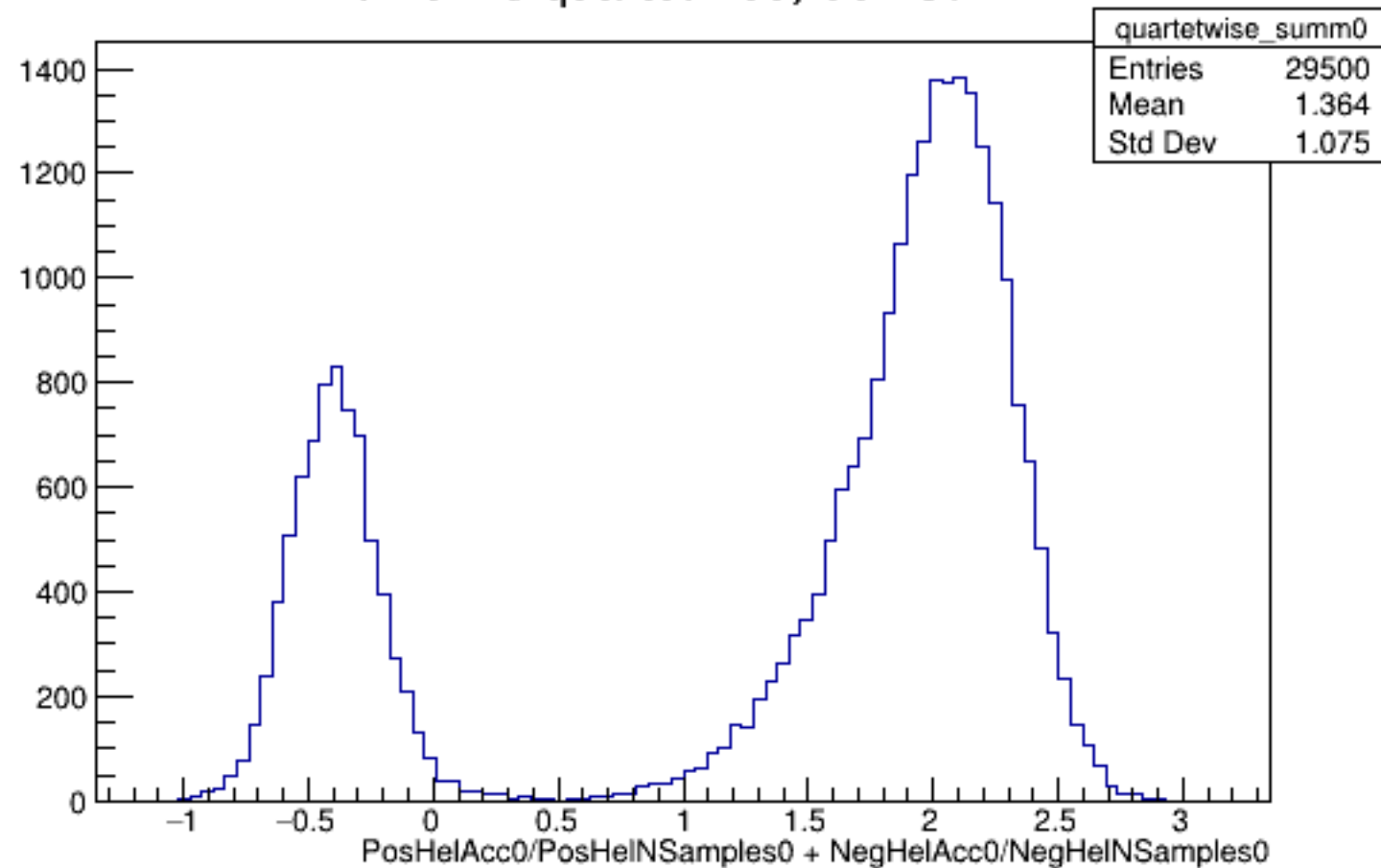
Run 5423 quartetwise, Sums0: All
