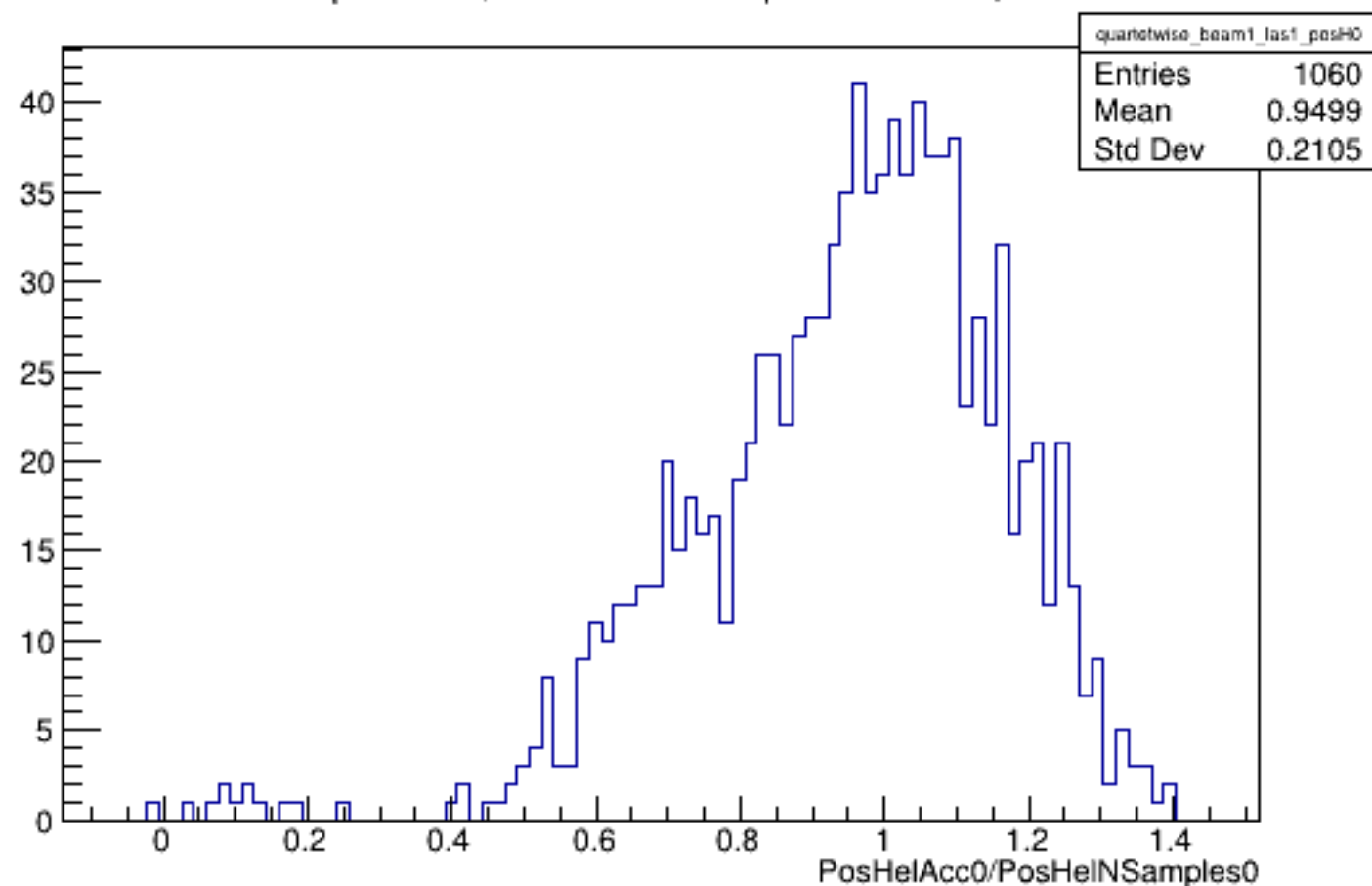
Run 5423 quartetwise, PosHelAcc0/NSamples0: Beam ON, Laser ON
