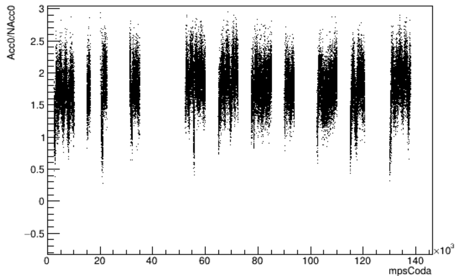
Run 5425 mpwise, Acc0 vs Time: Beam ON, Laser ON
