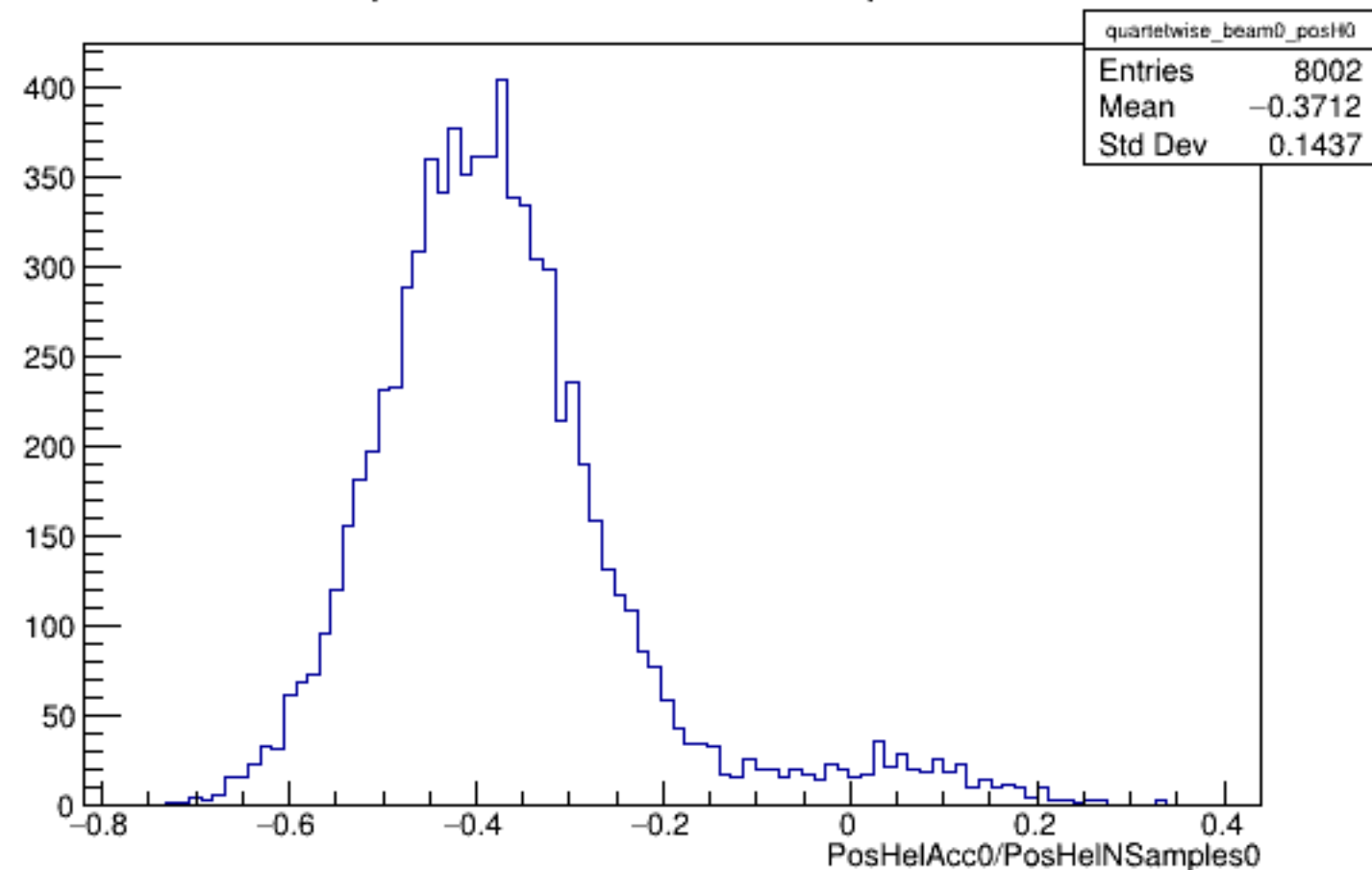
Run 5425 quartetwise, PosHelAcc0/NSamples0: Beam OFF
