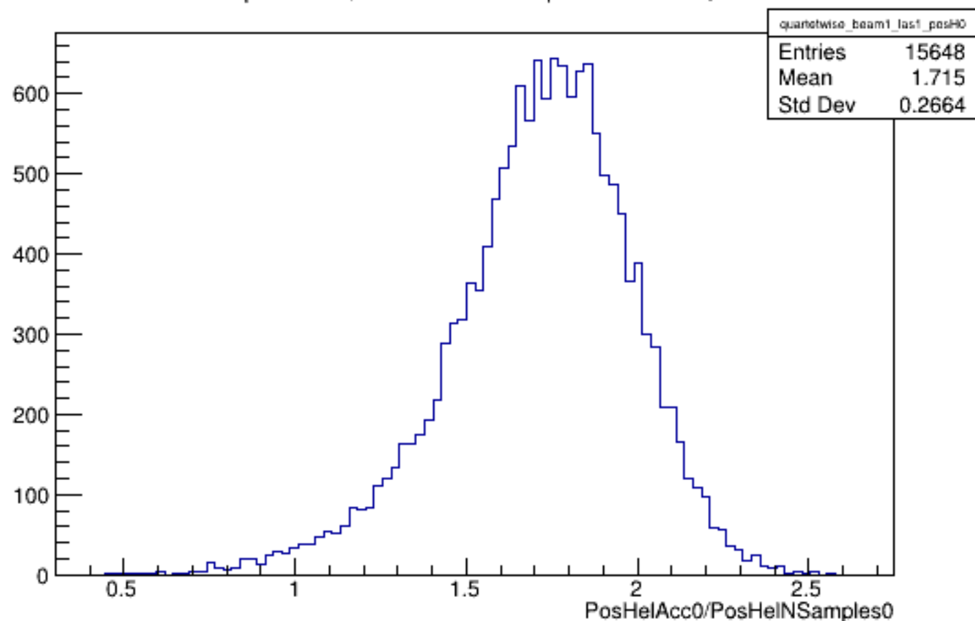
Run 5425 quartetwise, PosHelAcc0/NSamples0: Beam ON, Laser ON
