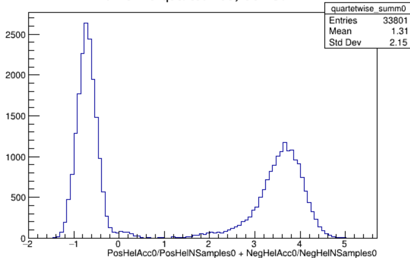
Run 5425 quartetwise, Sums0: All
