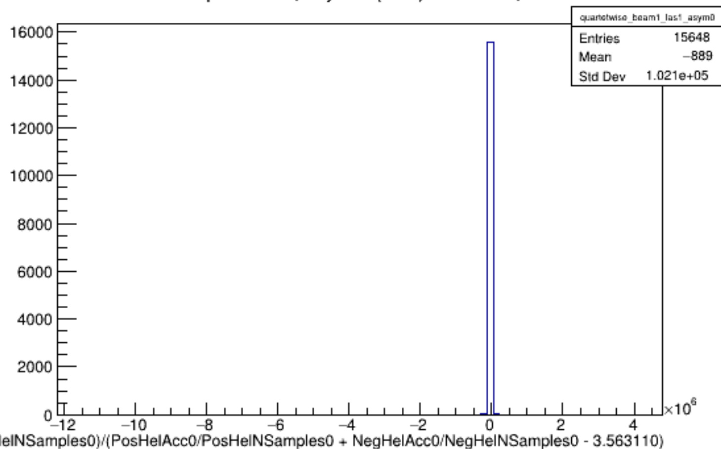
Run 5425 quartetwise, Asyms0 (Raw): Beam ON, Laser ON
