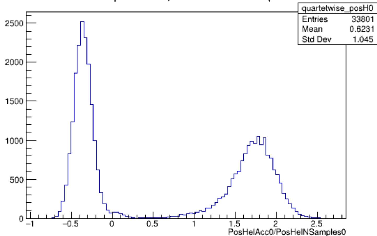
Run 5425 quartetwise, PosHelAcc0/NSamples0: All
