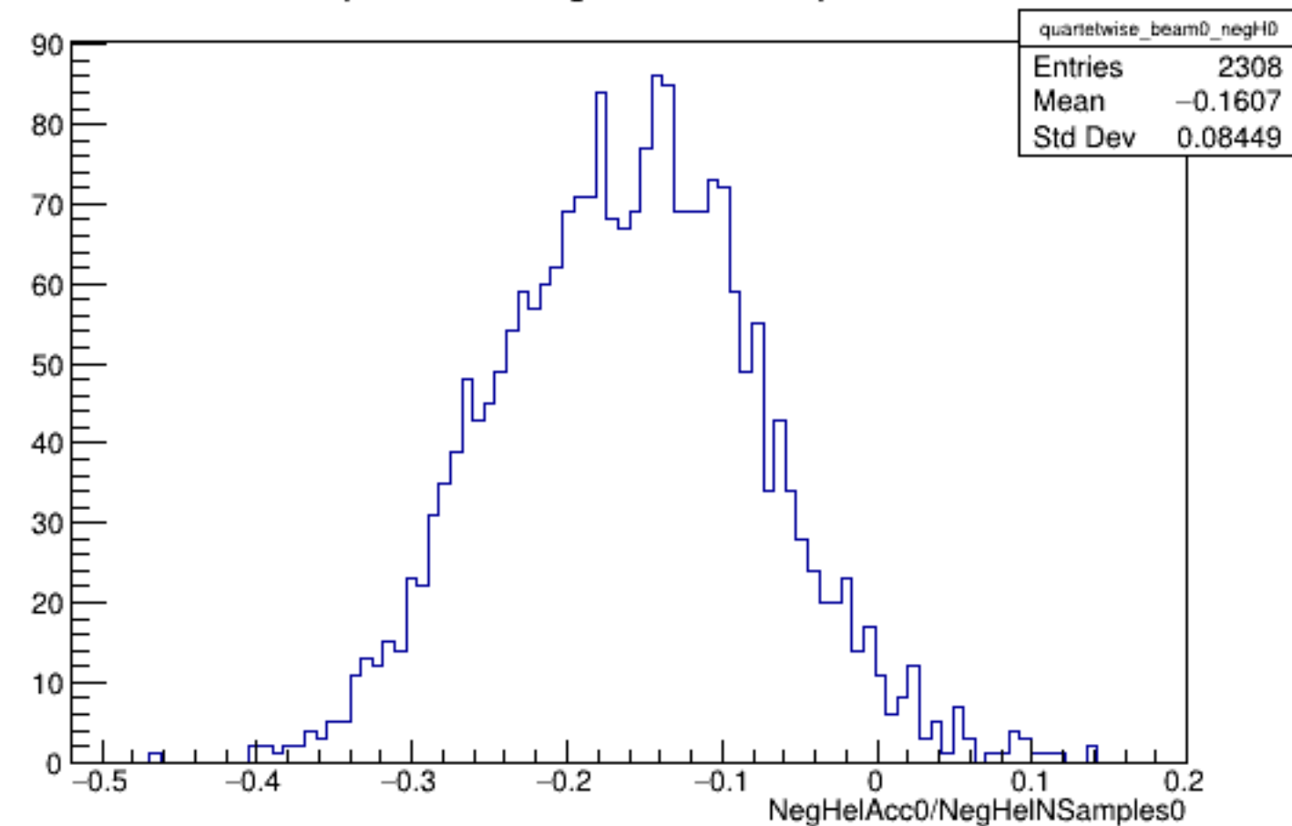
Run 5429 quartetwise, NegHelAcc0/NSamples0: Beam OFF
