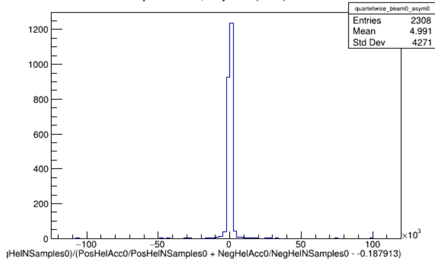
Run 5429 quartetwise, Asyms0 (Raw): Beam OFF
