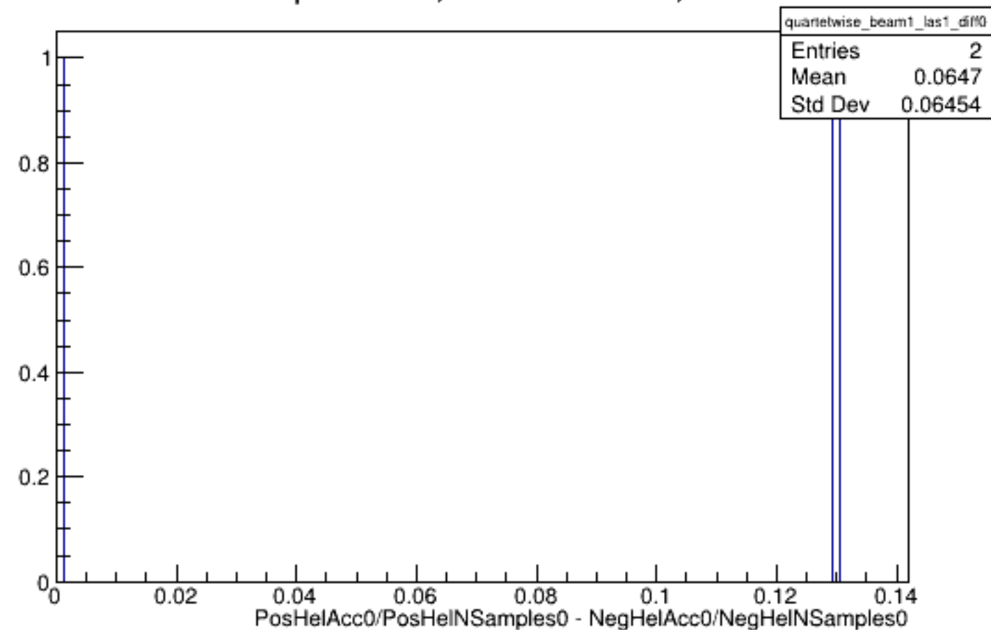
Run 5429 quartetwise, Diffs0: Beam ON, Laser ON
