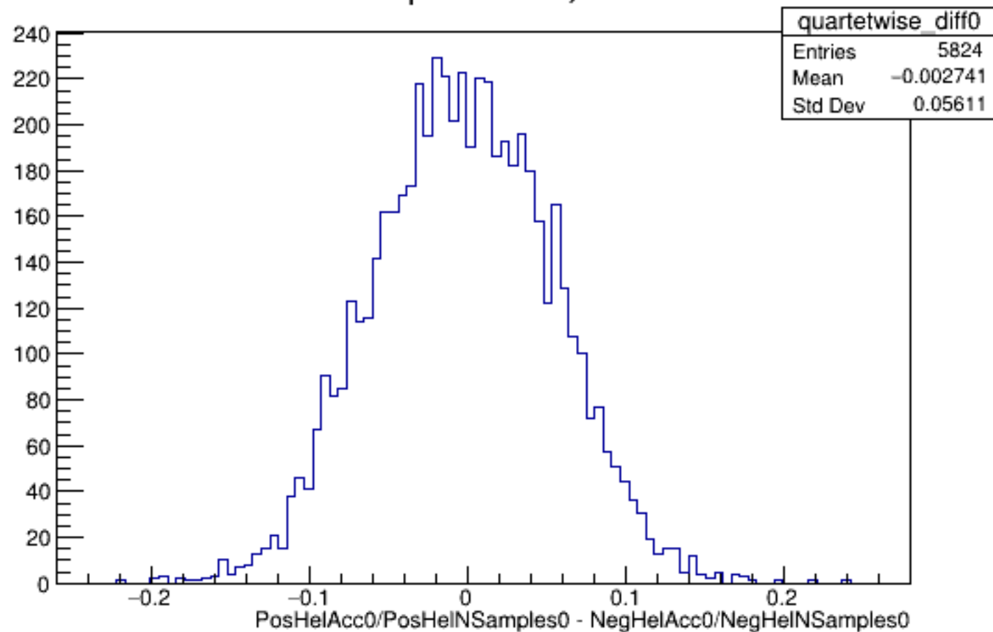
Run 5429 quartetwise, Diffs0: All
