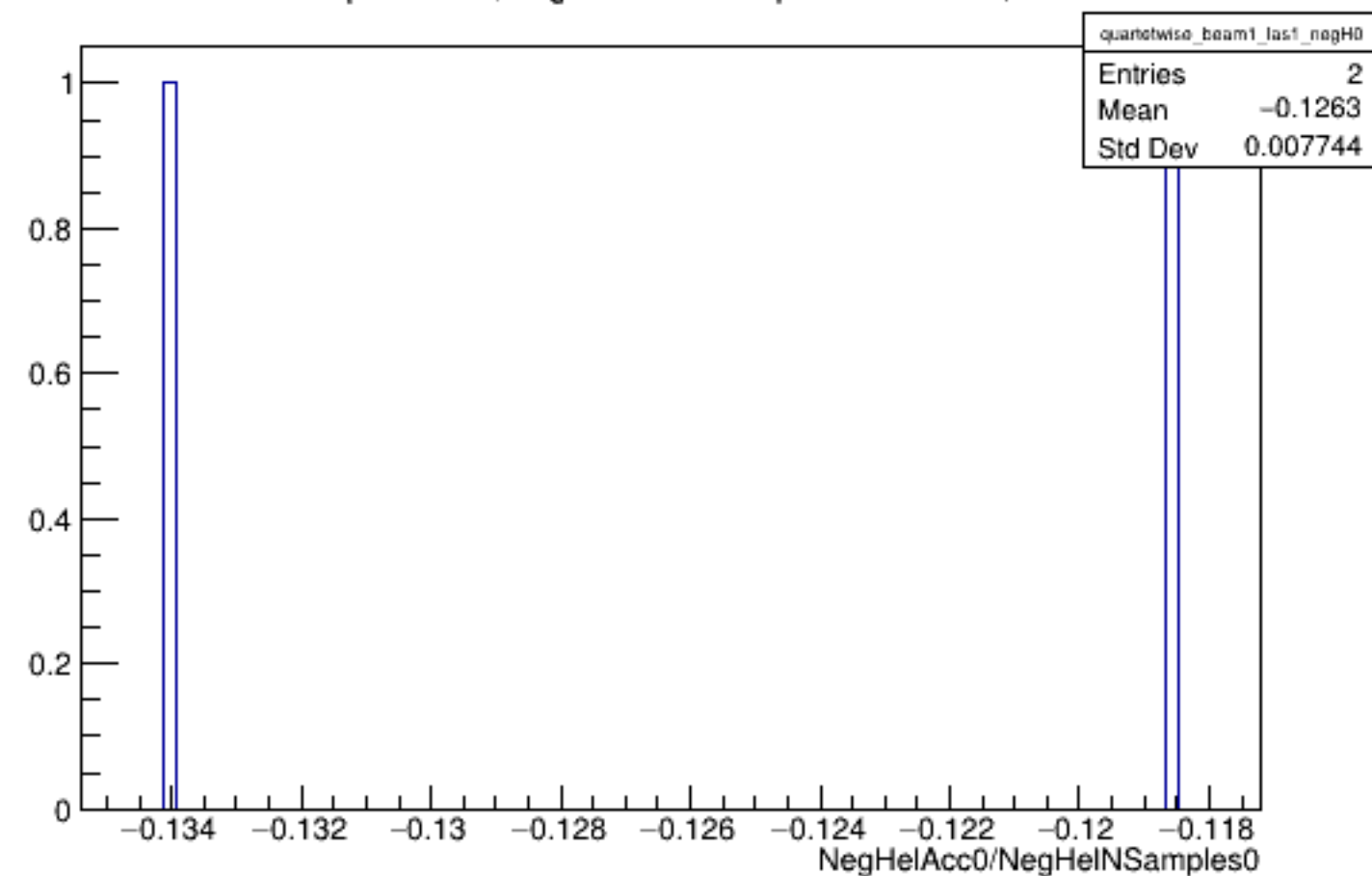
Run 5429 quartetwise, NegHelAcc0/NSamples0: Beam ON, Laser ON
