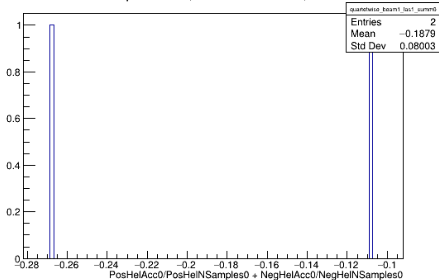
Run 5429 quartetwise, Sums0: Beam ON, Laser ON
