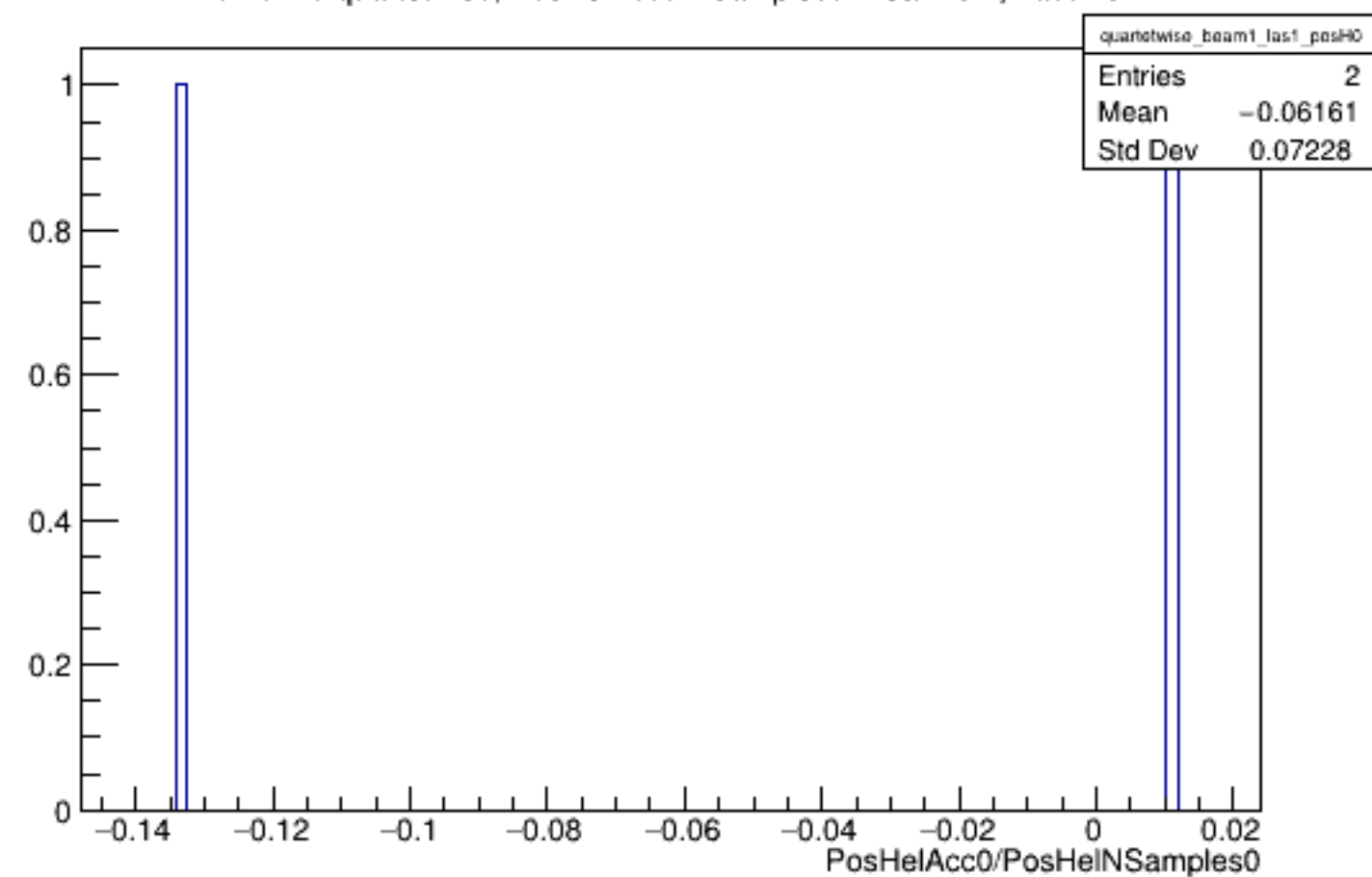
Run 5429 quartetwise, PosHelAcc0/NSamples0: Beam ON, Laser ON
