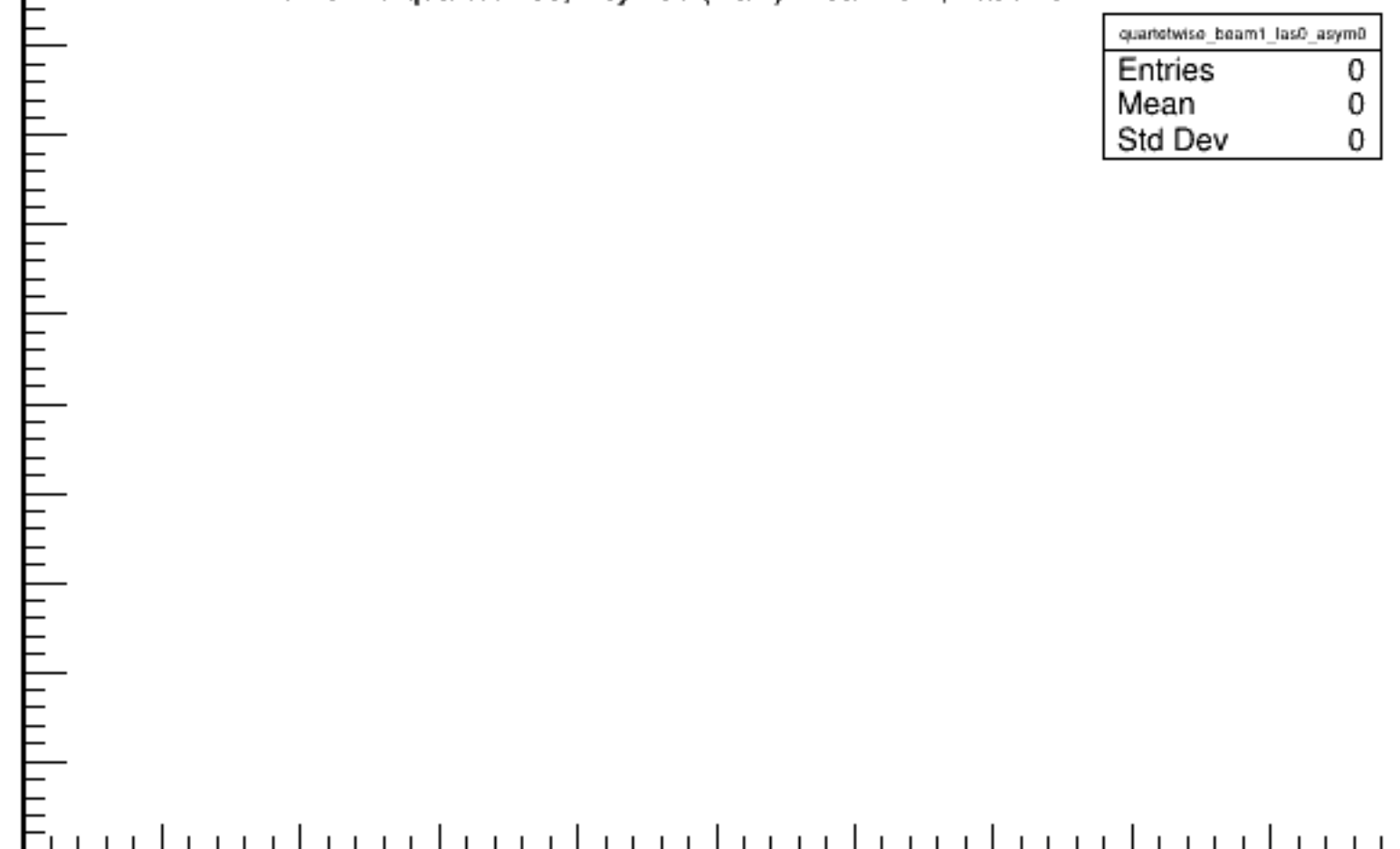
Run 5429 quartetwise, Asyms0 (Raw): Beam ON, Laser OFF
