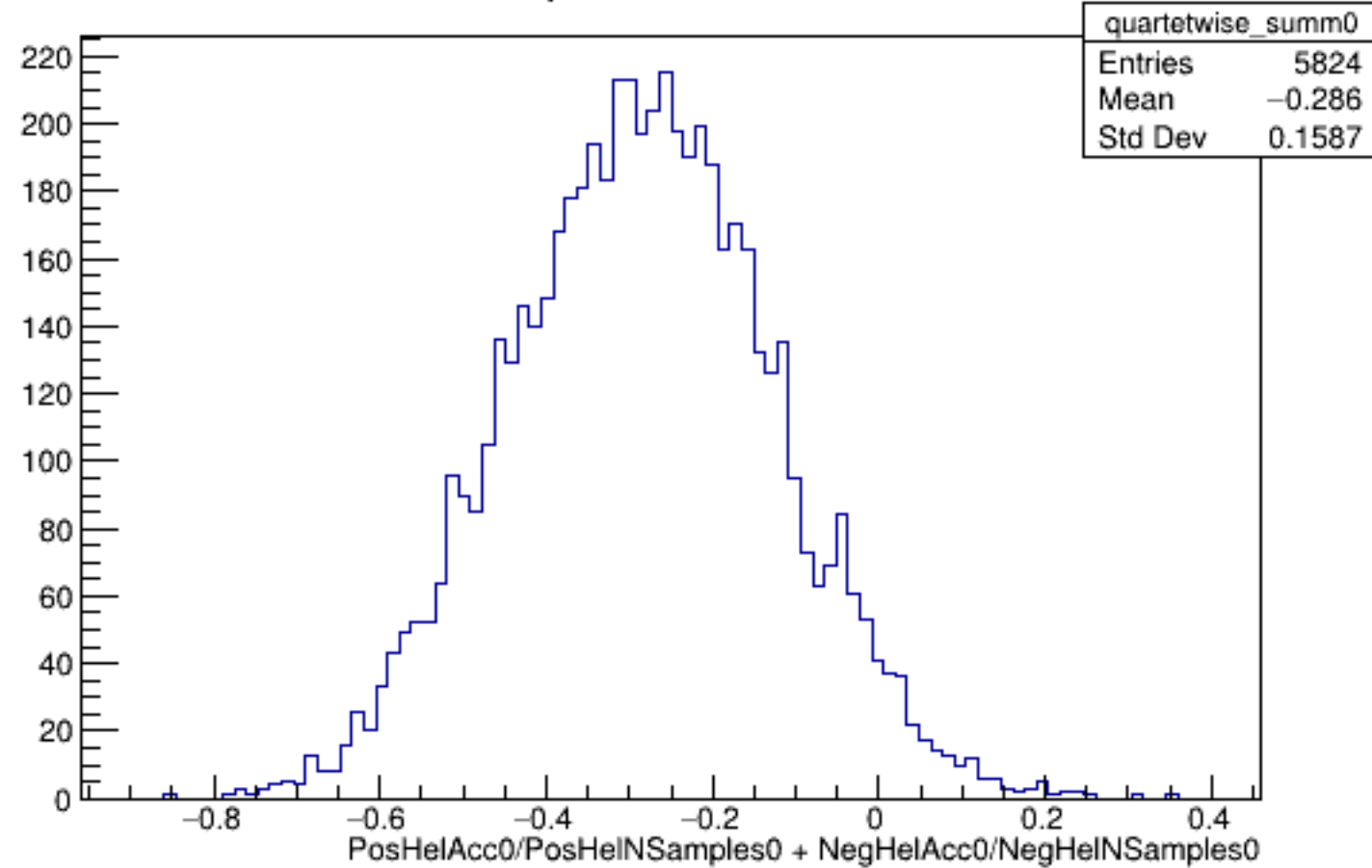
Run 5429 quartetwise, Sums0: All
