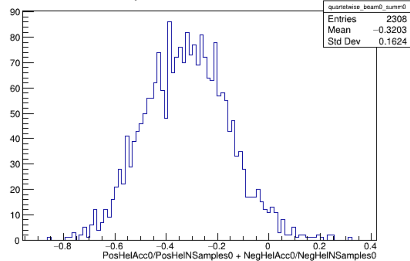
Run 5429 quartetwise, Sums0: Beam OFF
