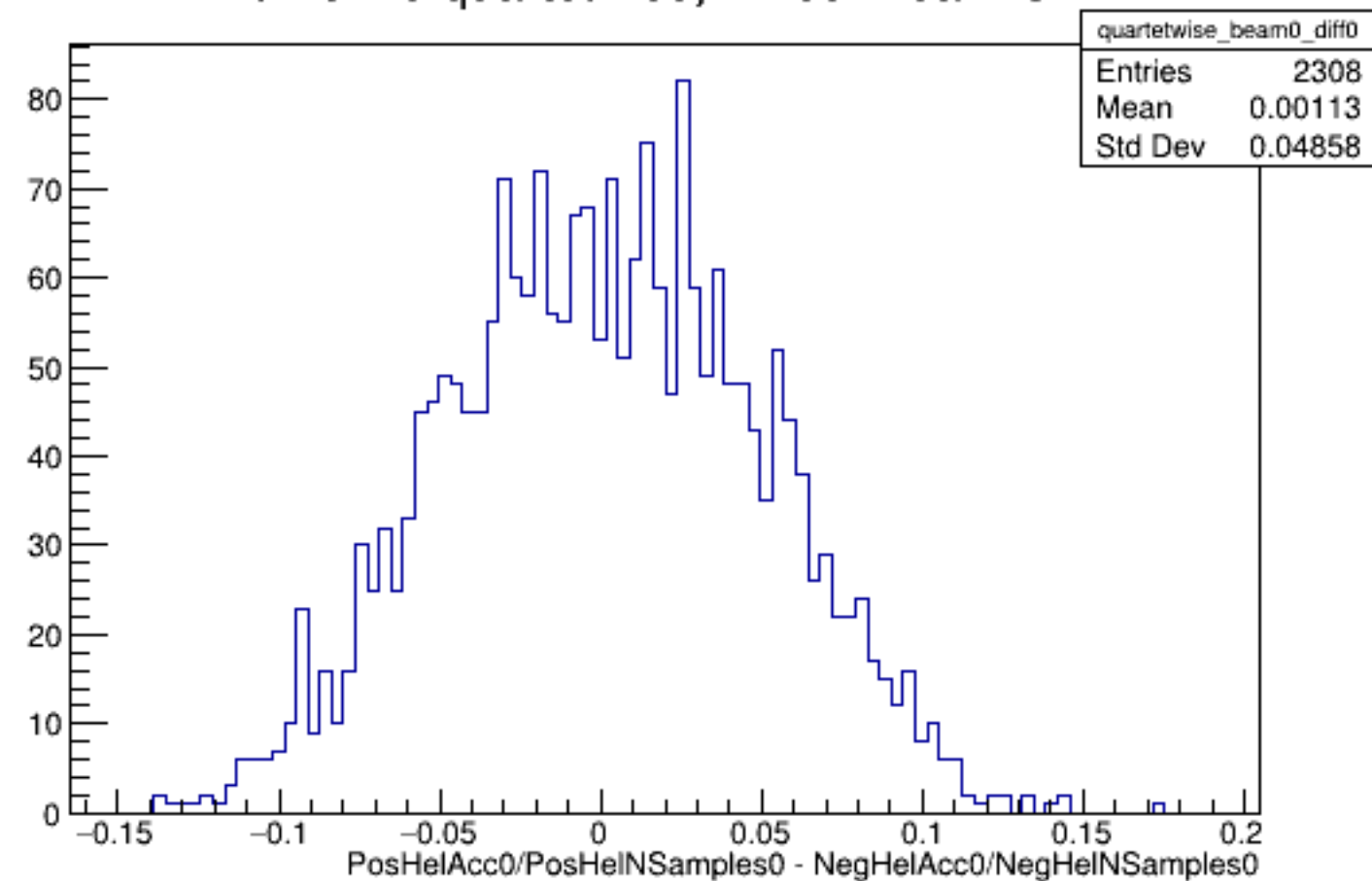
Run 5429 quartetwise, Diffs0: Beam OFF
