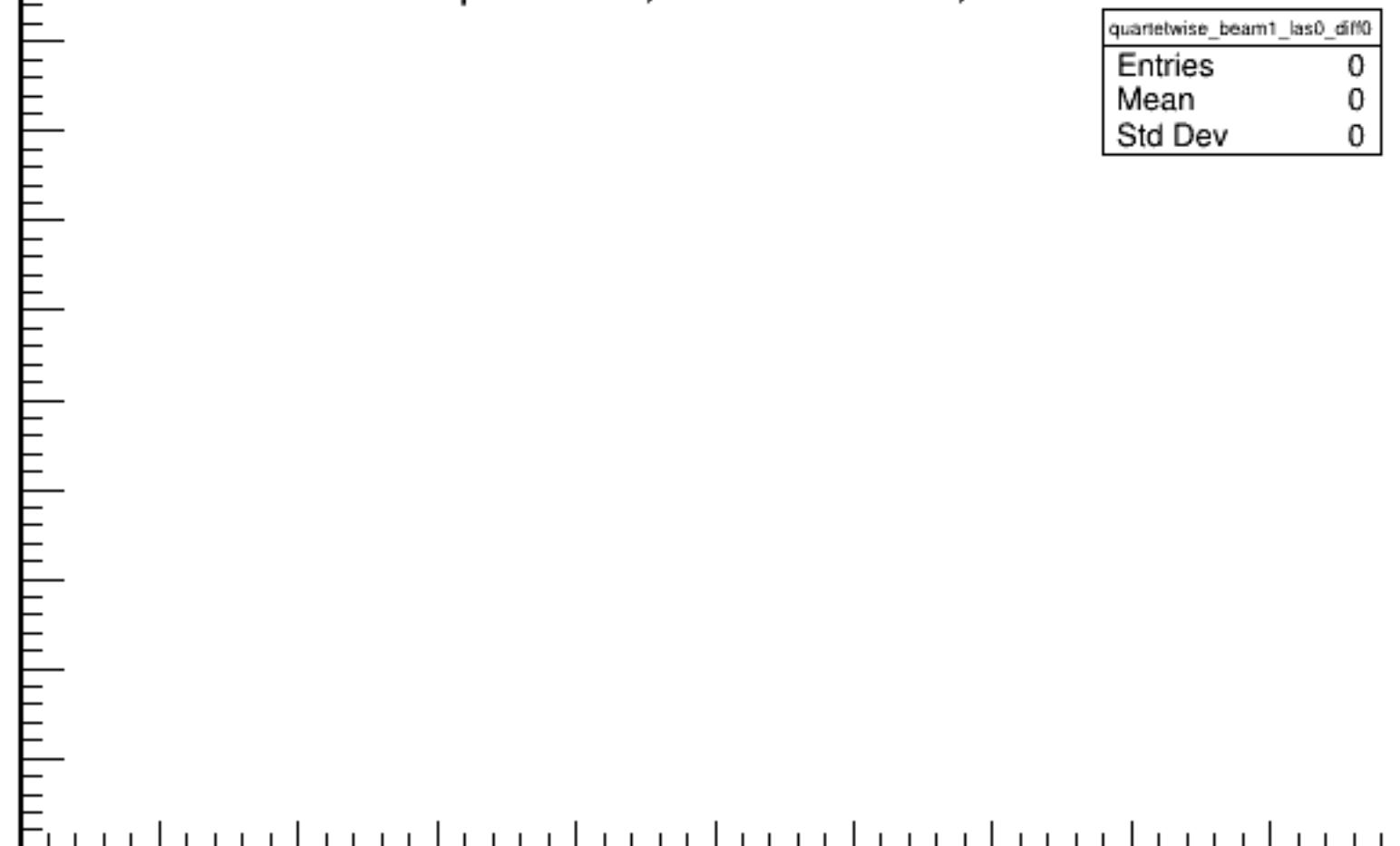
Run 5429 quartetwise, Diffs0: Beam ON, Laser OFF
