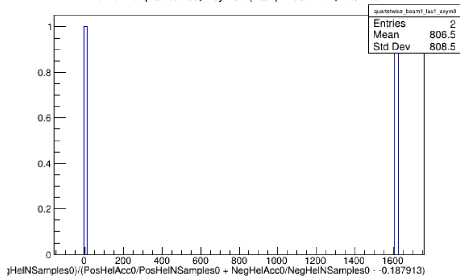
Run 5429 quartetwise, Asyms0 (Raw): Beam ON, Laser ON
