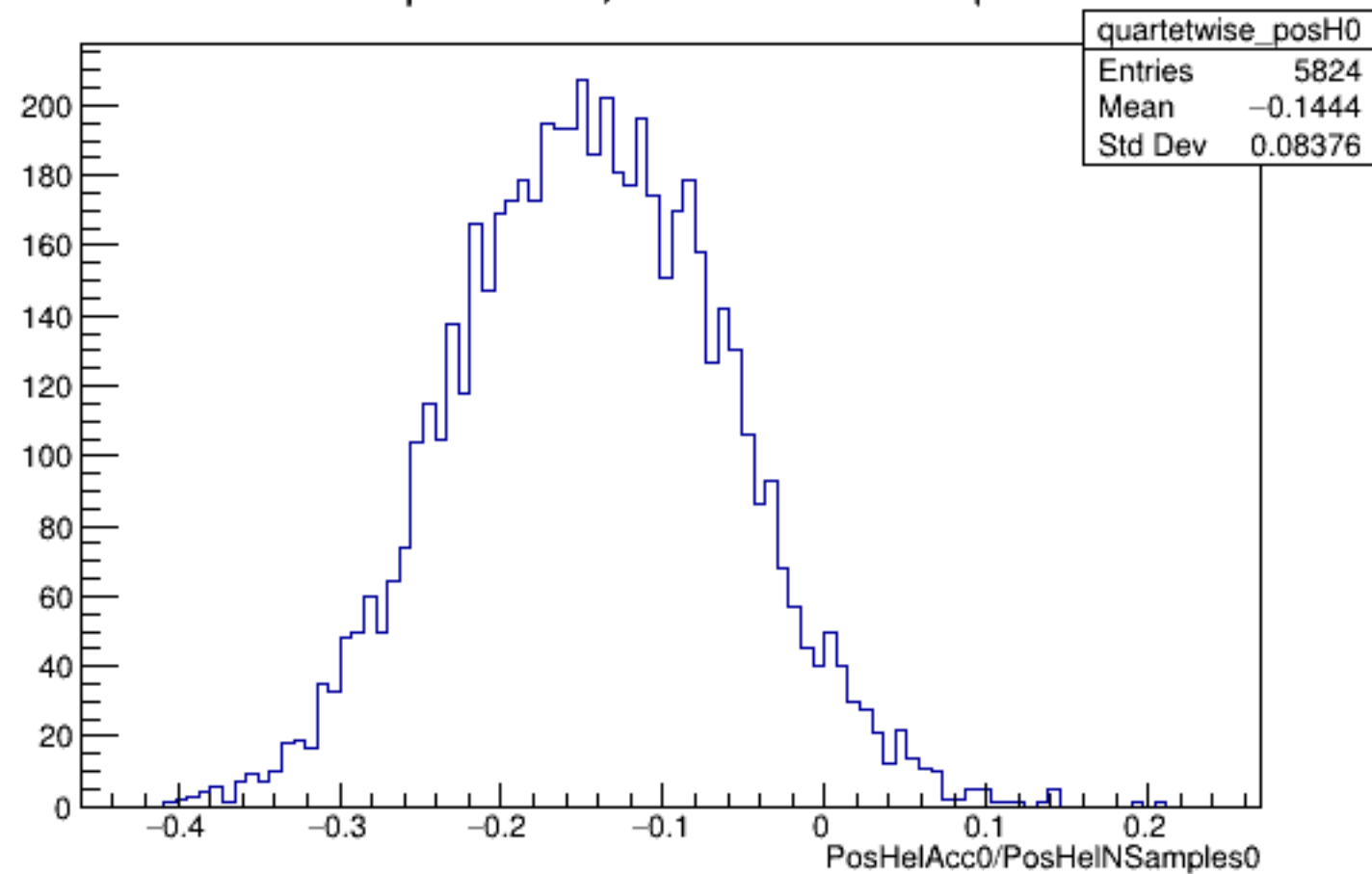
Run 5429 quartetwise, PosHelAcc0/NSamples0: All
