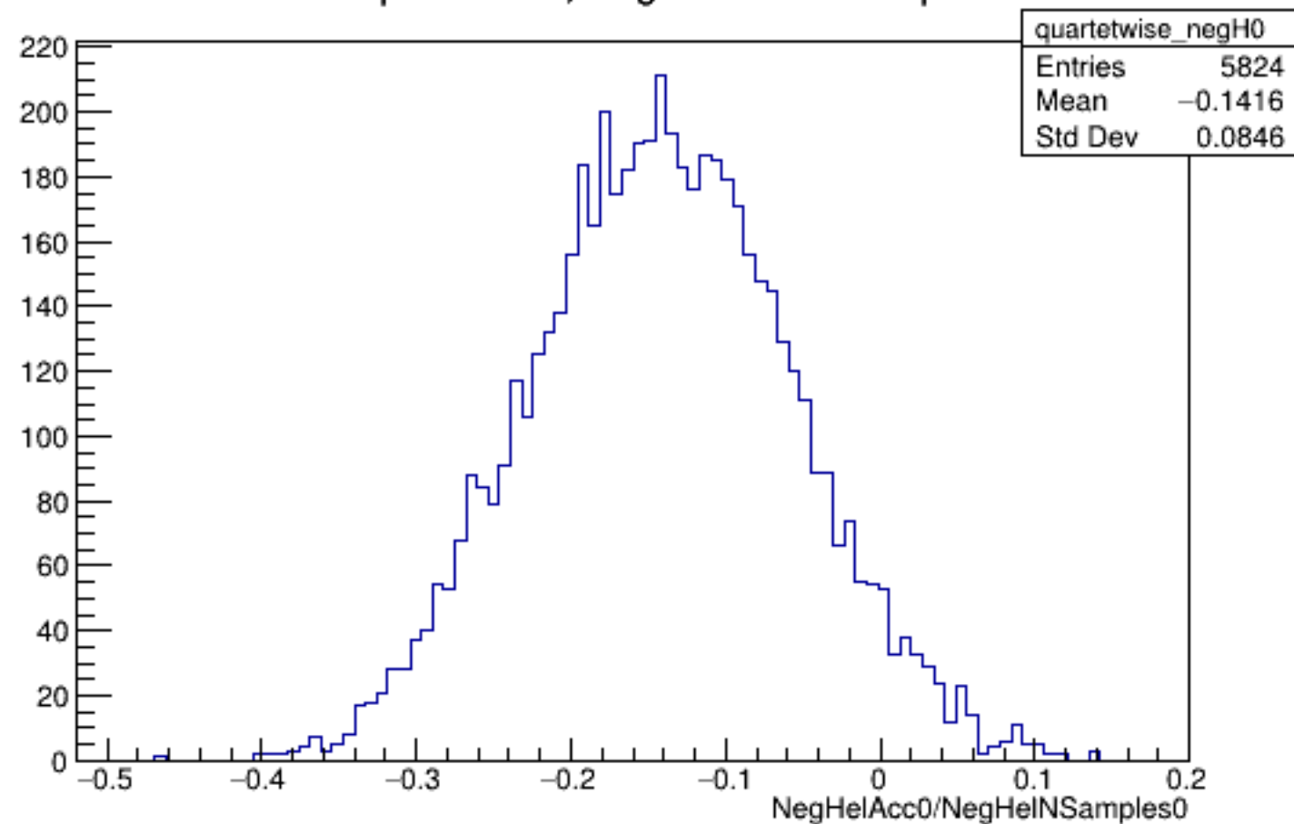
Run 5429 quartetwise, NegHelAcc0/NSamples0: All
