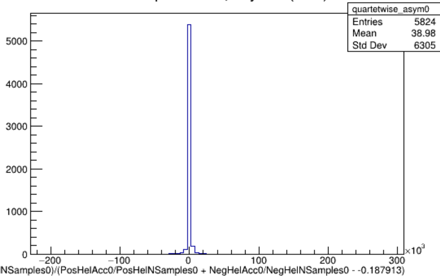
Run 5429 quartetwise, Asyms0 (Raw): All
