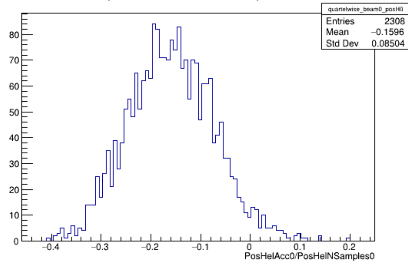
Run 5429 quartetwise, PosHelAcc0/NSamples0: Beam OFF
