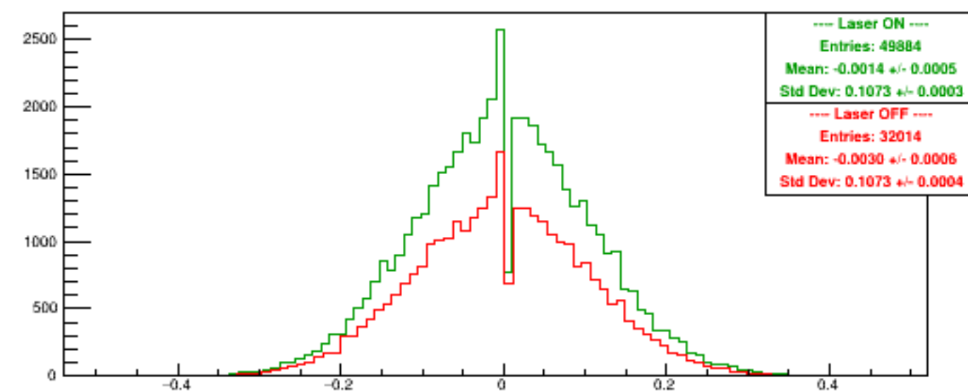
Run 5436 quartetwise, Asyms DSbg2
