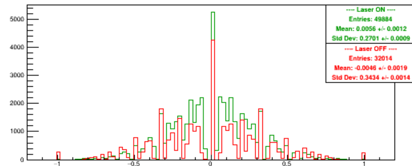
Run 5436 quartetwise, Asyms Vert Finger
