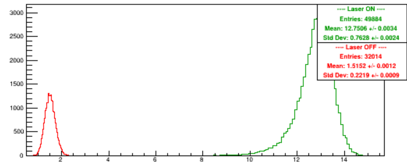
Run 5436 quartetwise, NegHelAcc0/NSamples0
