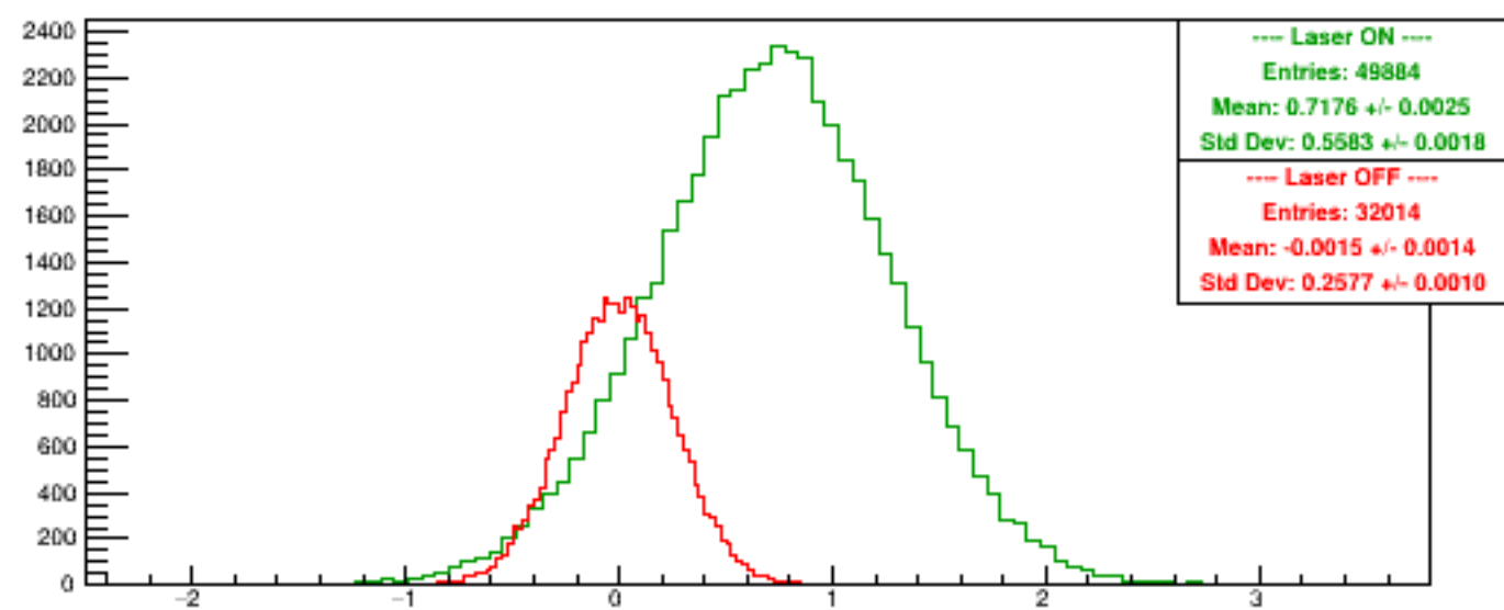
Run 5436 quartetwise, Diffs0
