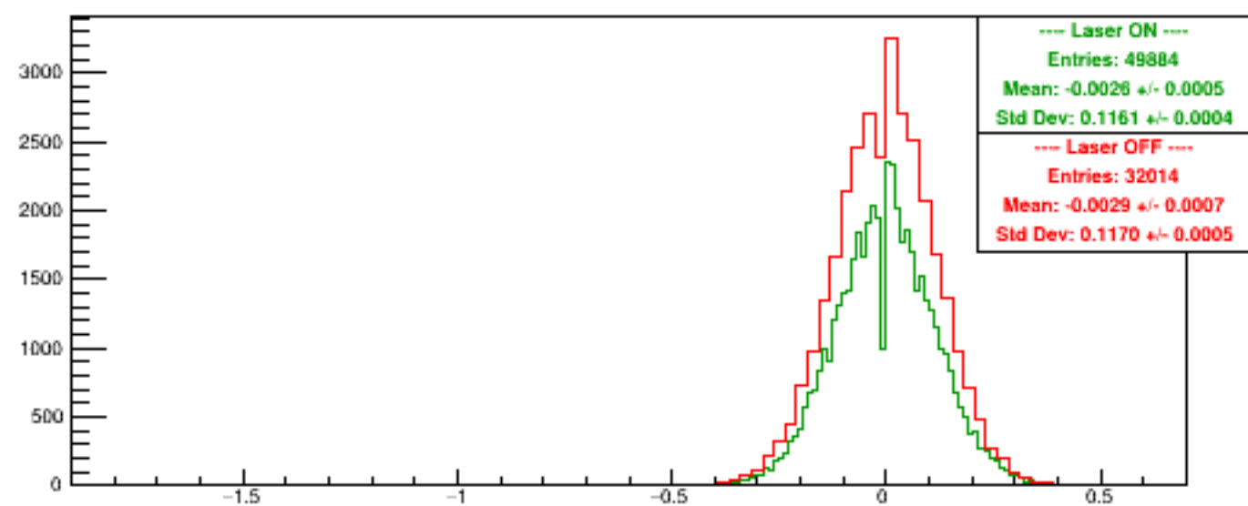
Run 5436 quartetwise, Asyms DSbg1
