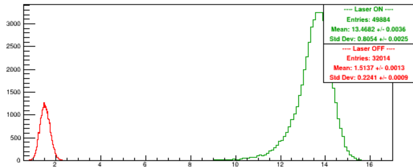
Run 5436 quartetwise, PosHelAcc0/NSamples0
