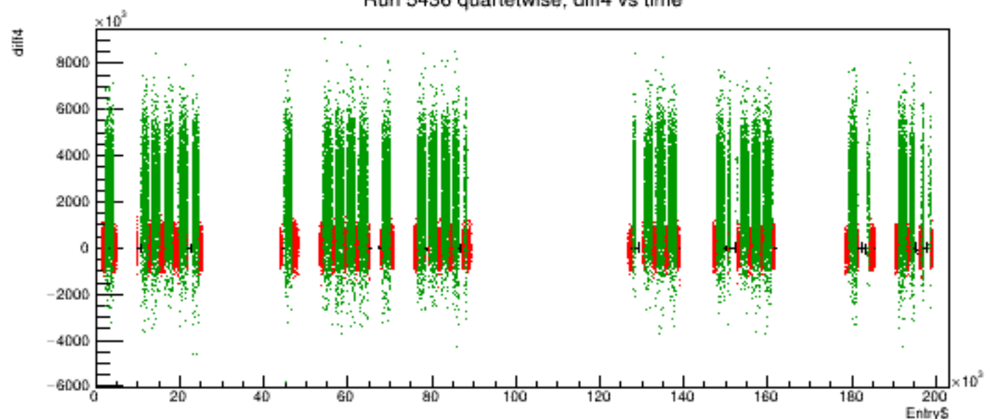
Run 5436 quartetwise, diff4 vs time
