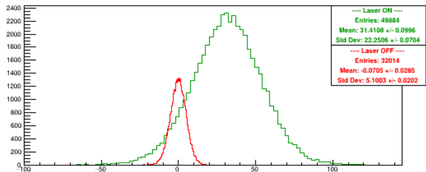
Run 5436 quartetwise, Asyms4
