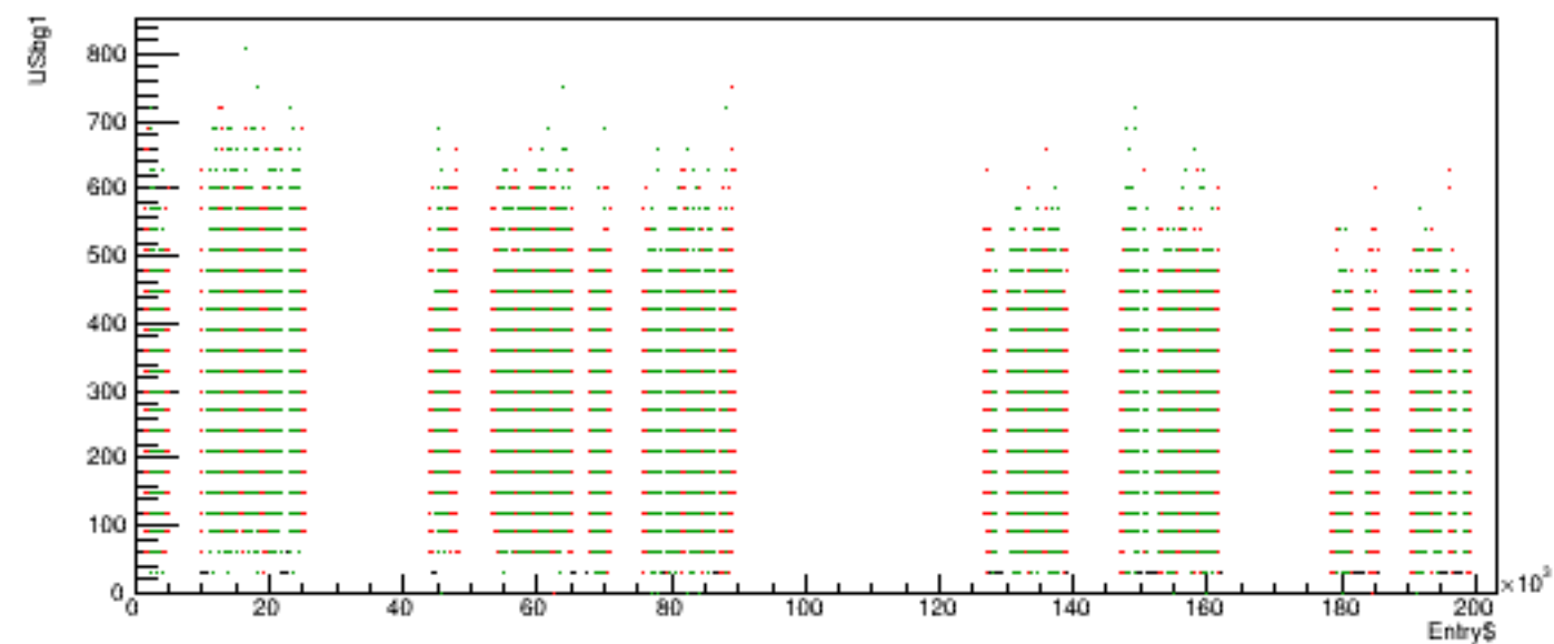
Run 5436 quartetwise, USbg1 vs time
