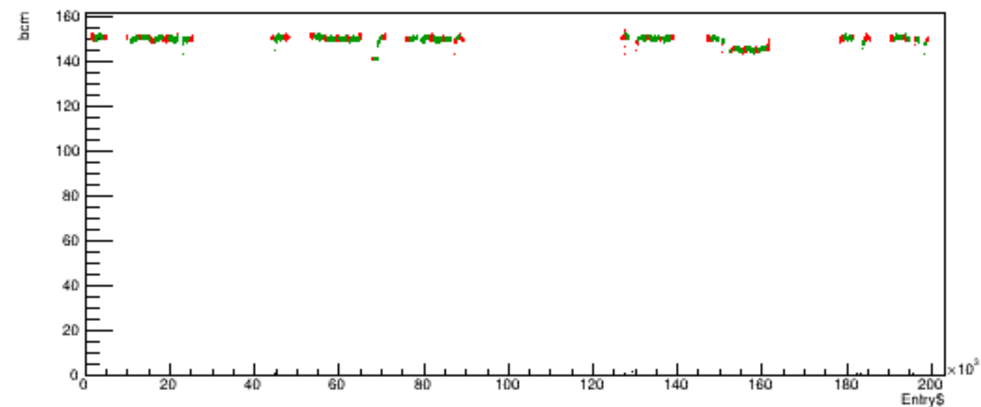
Run 5436 quartetwise, posH4 vs time
