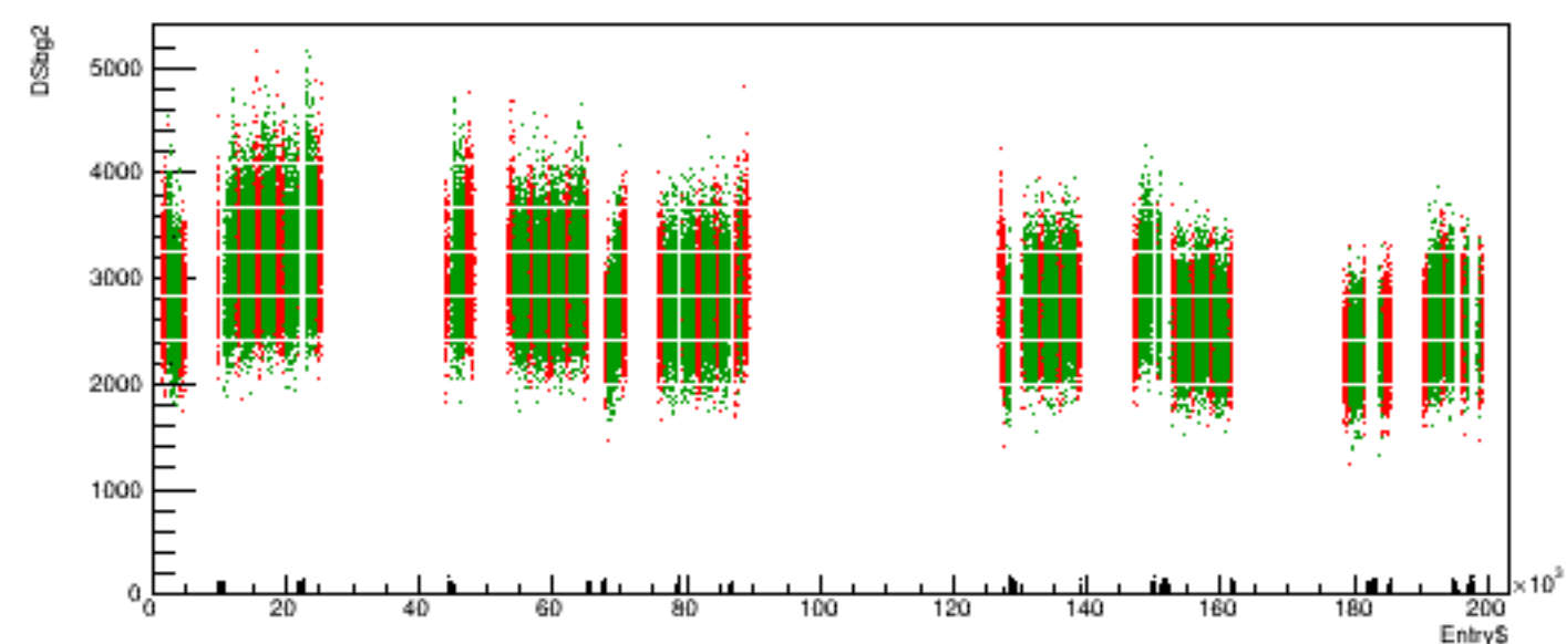
Run 5436 quartetwise, DSbg2 vs time
