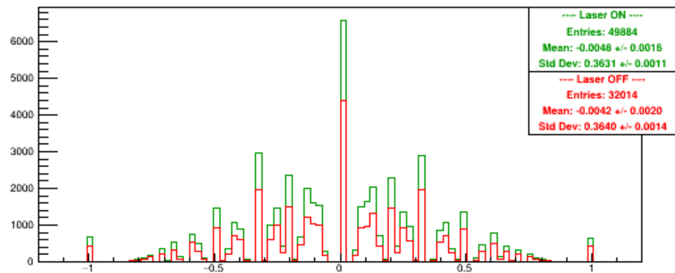
Run 5436 quartetwise, Asyms USbg1
