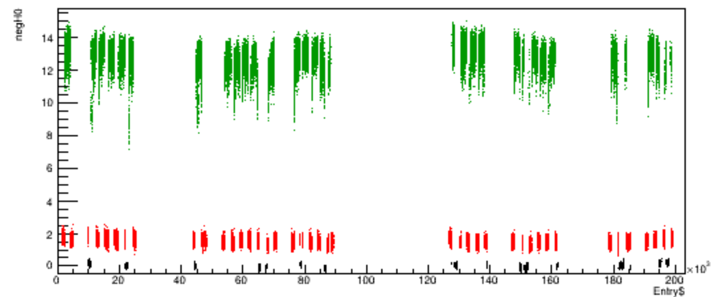
Run 5436 quartetwise, negH0 vs time
