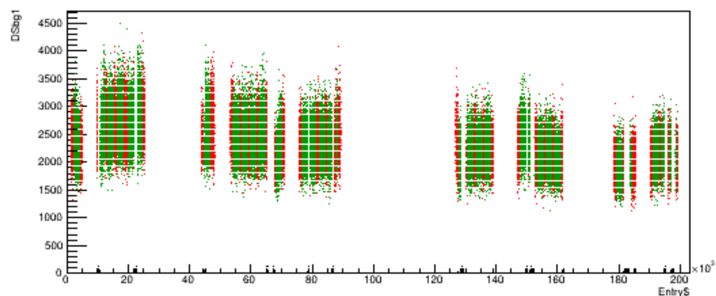
Run 5436 quartetwise, DSbg1 vs time
