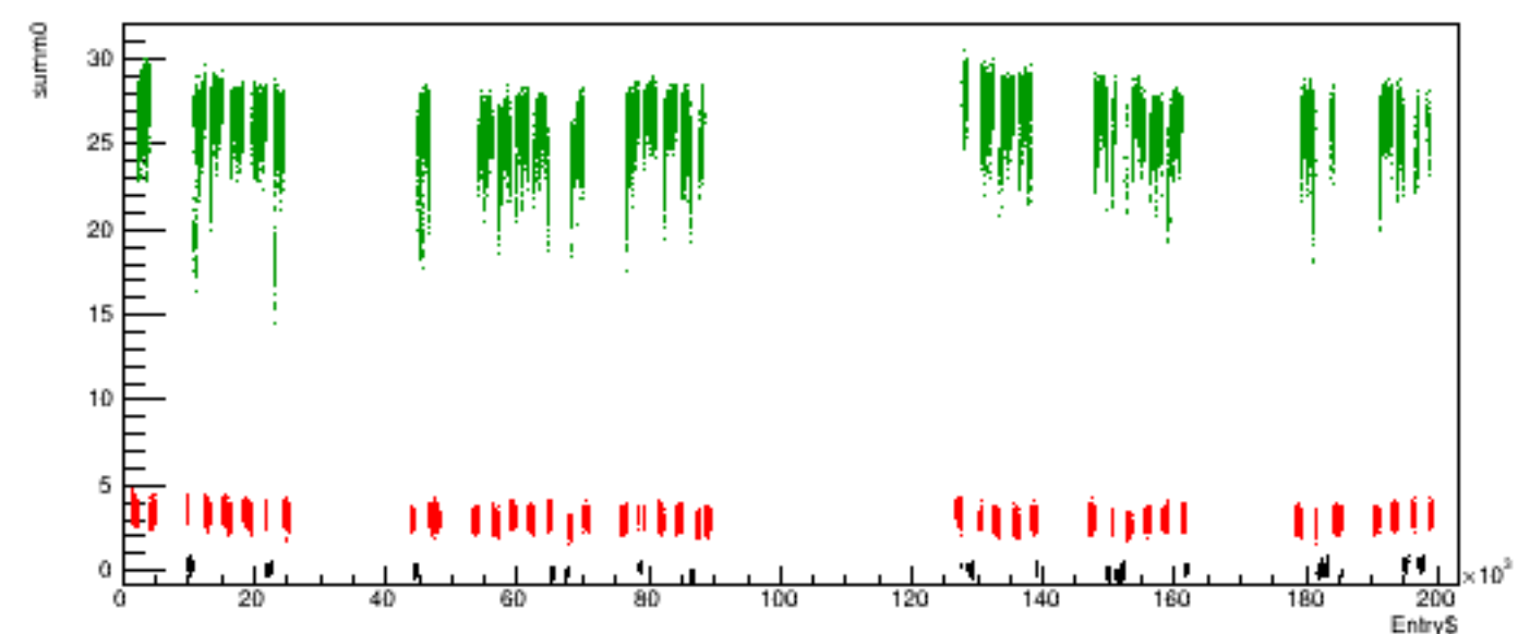
Run 5436 quartetwise, summ0 vs time
