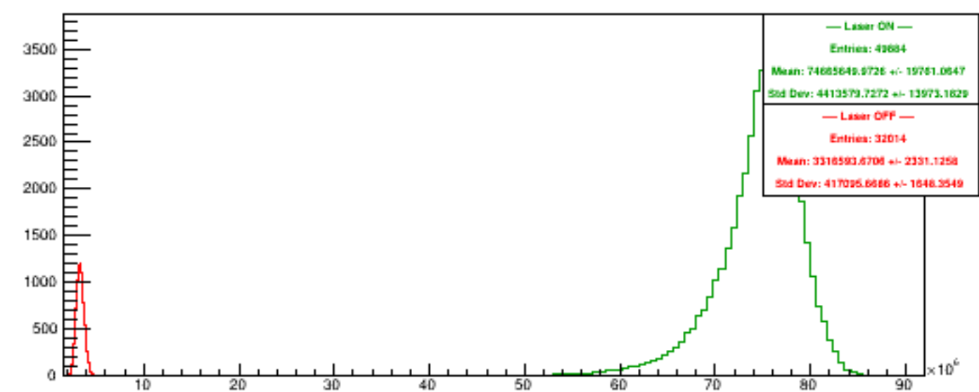
Run 5436 quartetwise, Sums4
