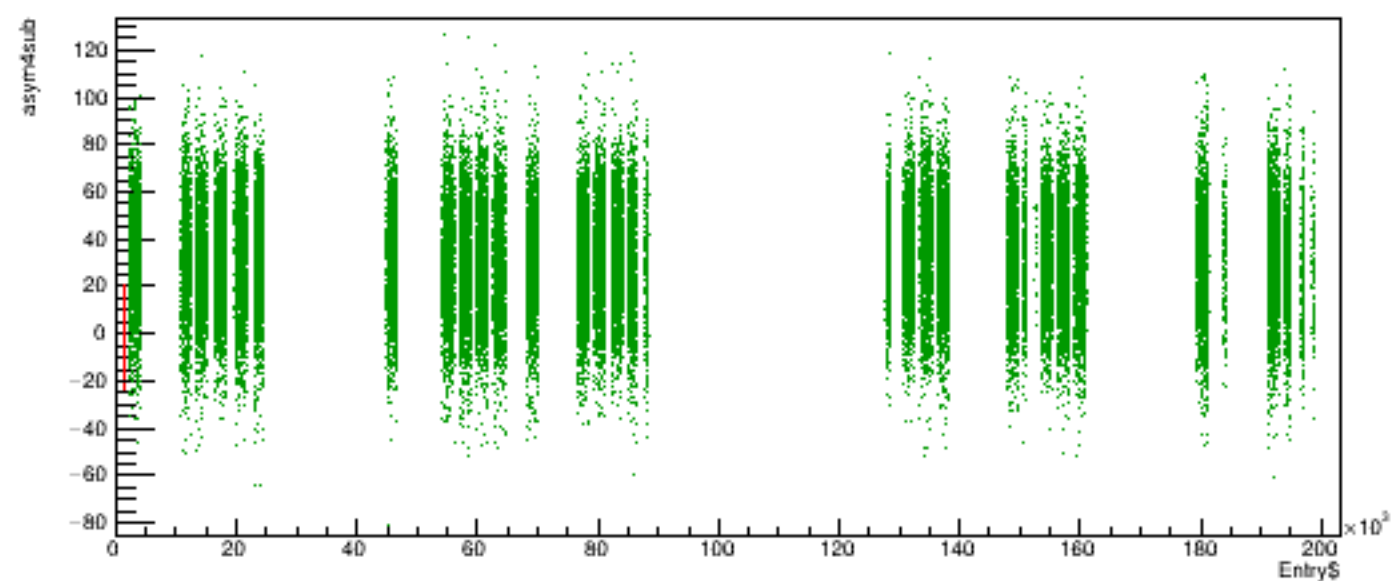
Run 5436 quartetwise, asym4sub vs time
