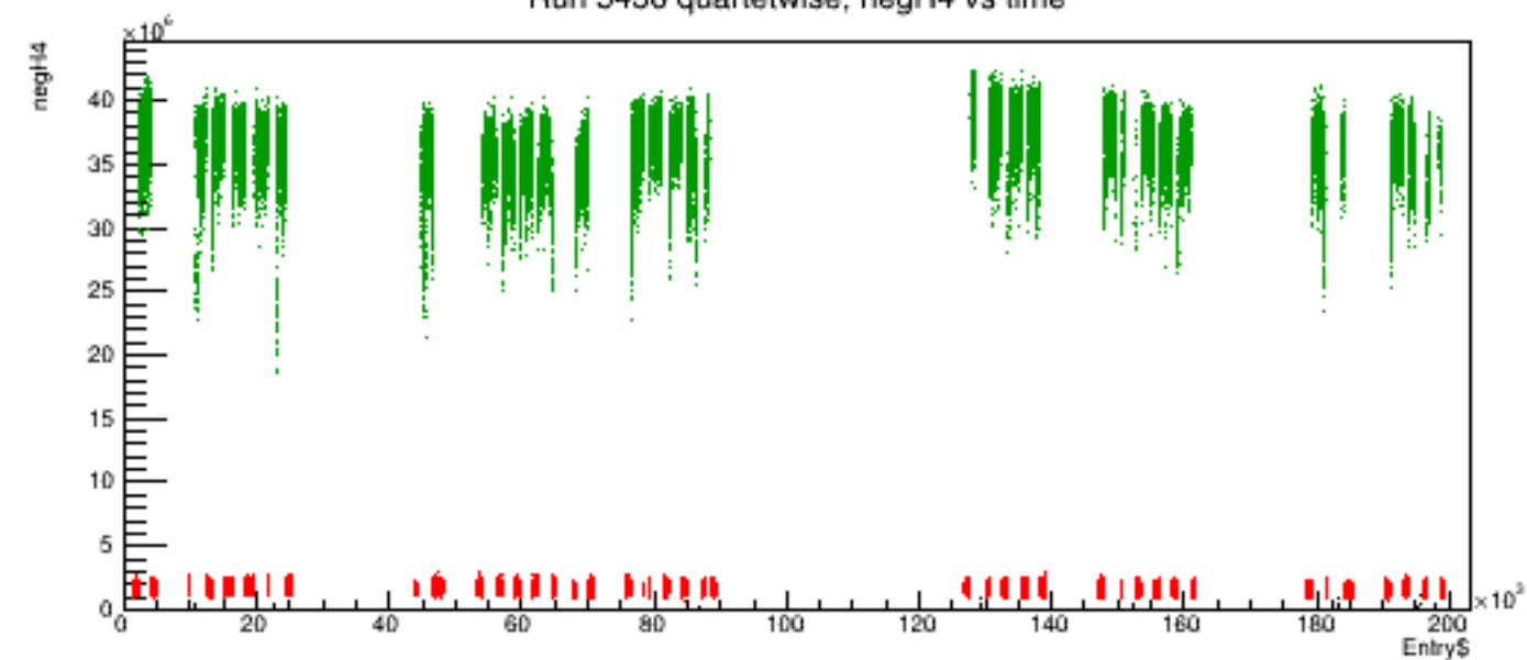
Run 5436 quartetwise, negH4 vs time
