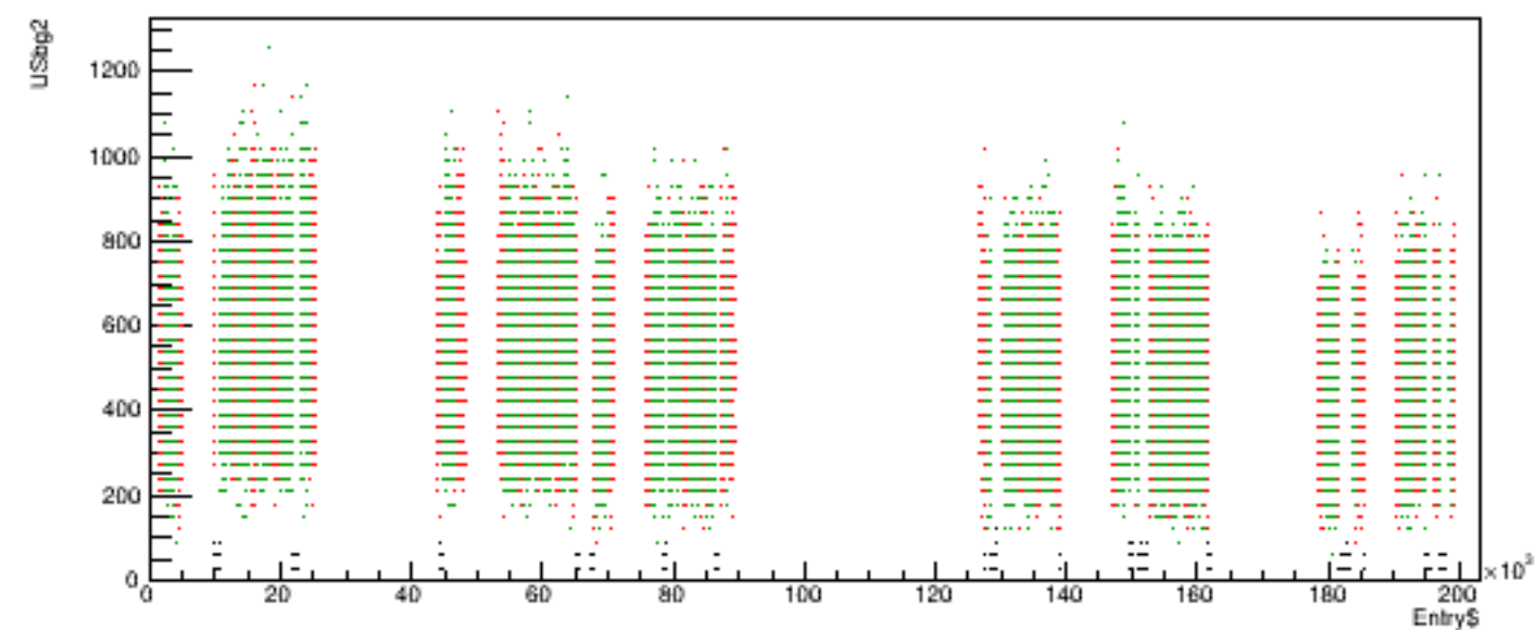
Run 5436 quartetwise, USbg2 vs time
