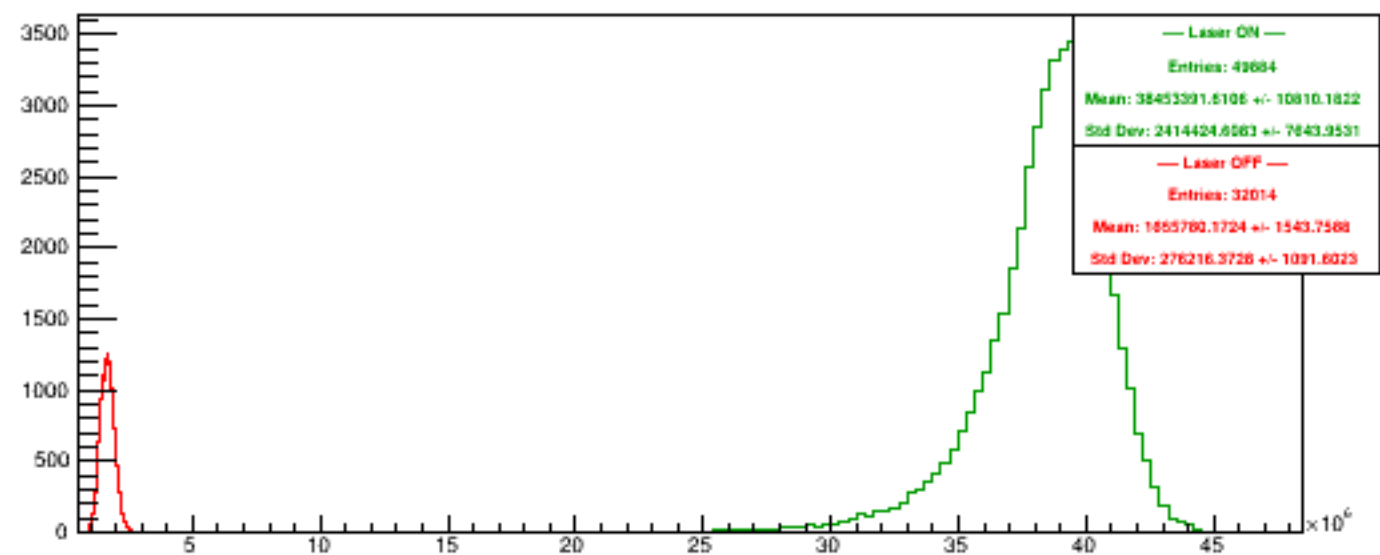
Run 5436 quartetwise, PosHelAcc4
