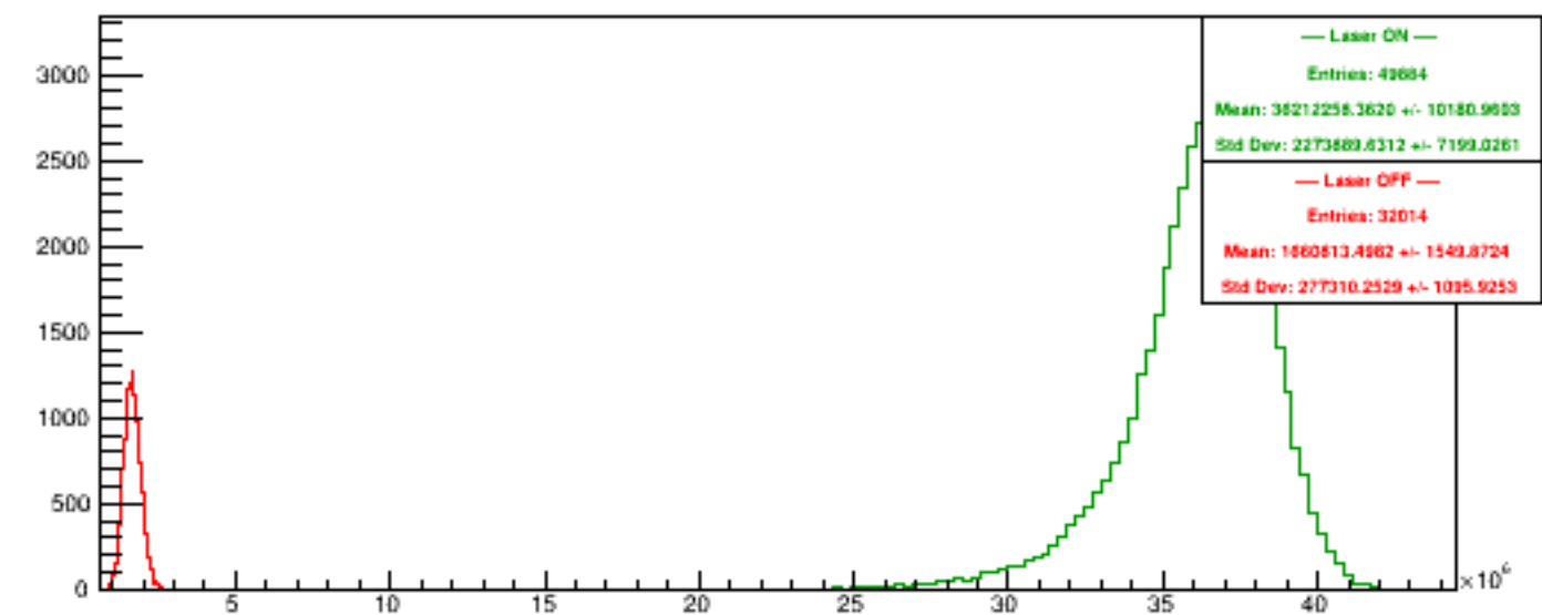
Run 5436 quartetwise, NegHelAcc4
