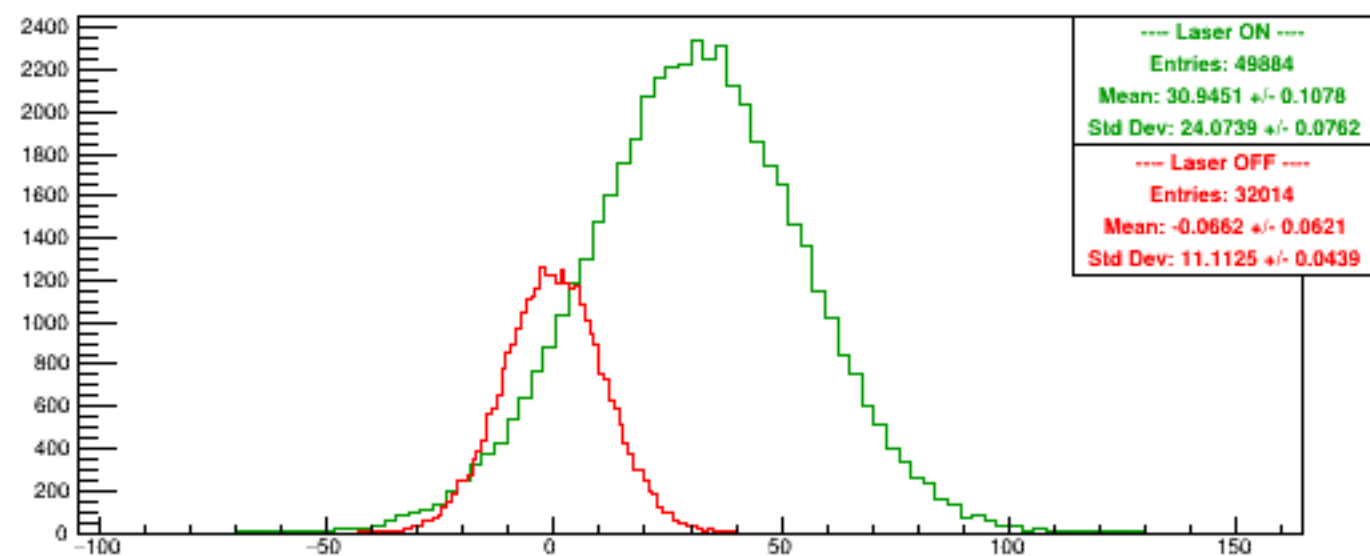
Run 5436 quartetwise, Asyms0
