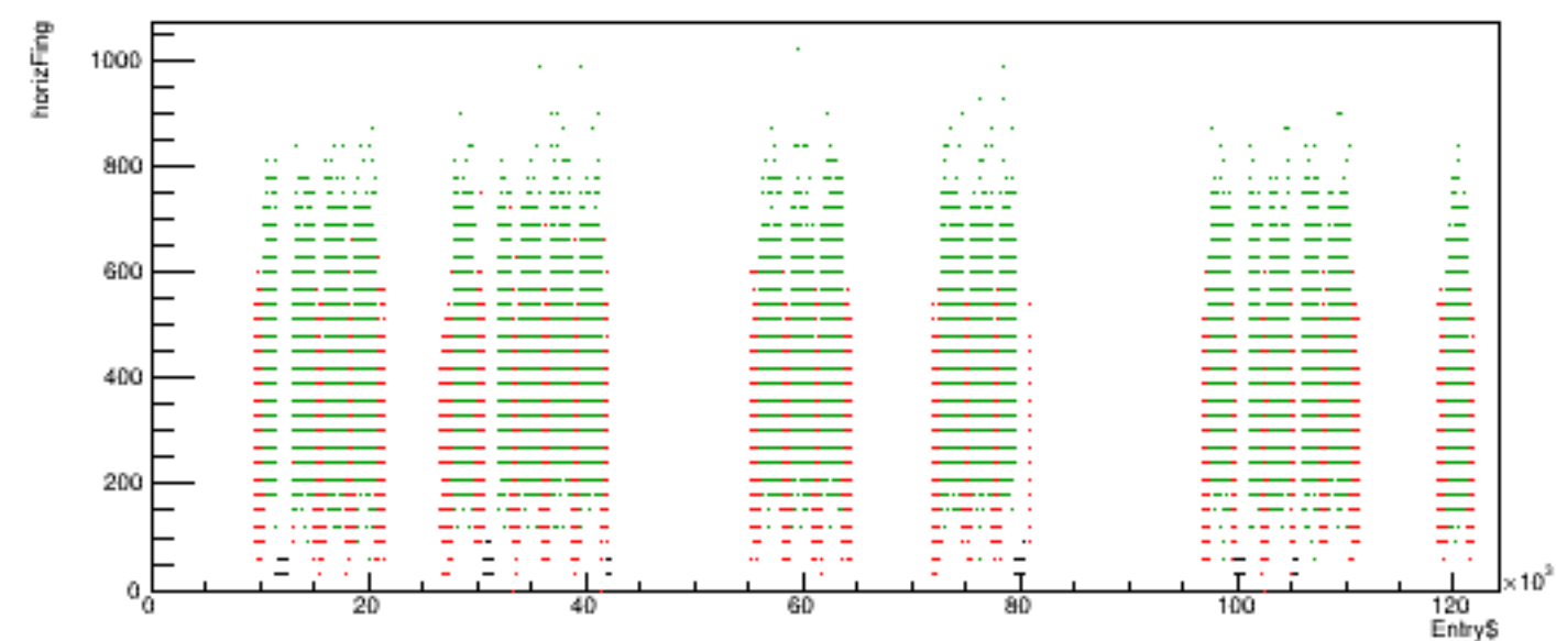
Run 5441 quartetwise, horizFing vs time
