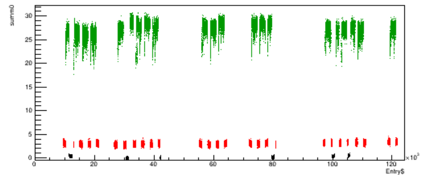
Run 5441 quartetwise, summ0 vs time
