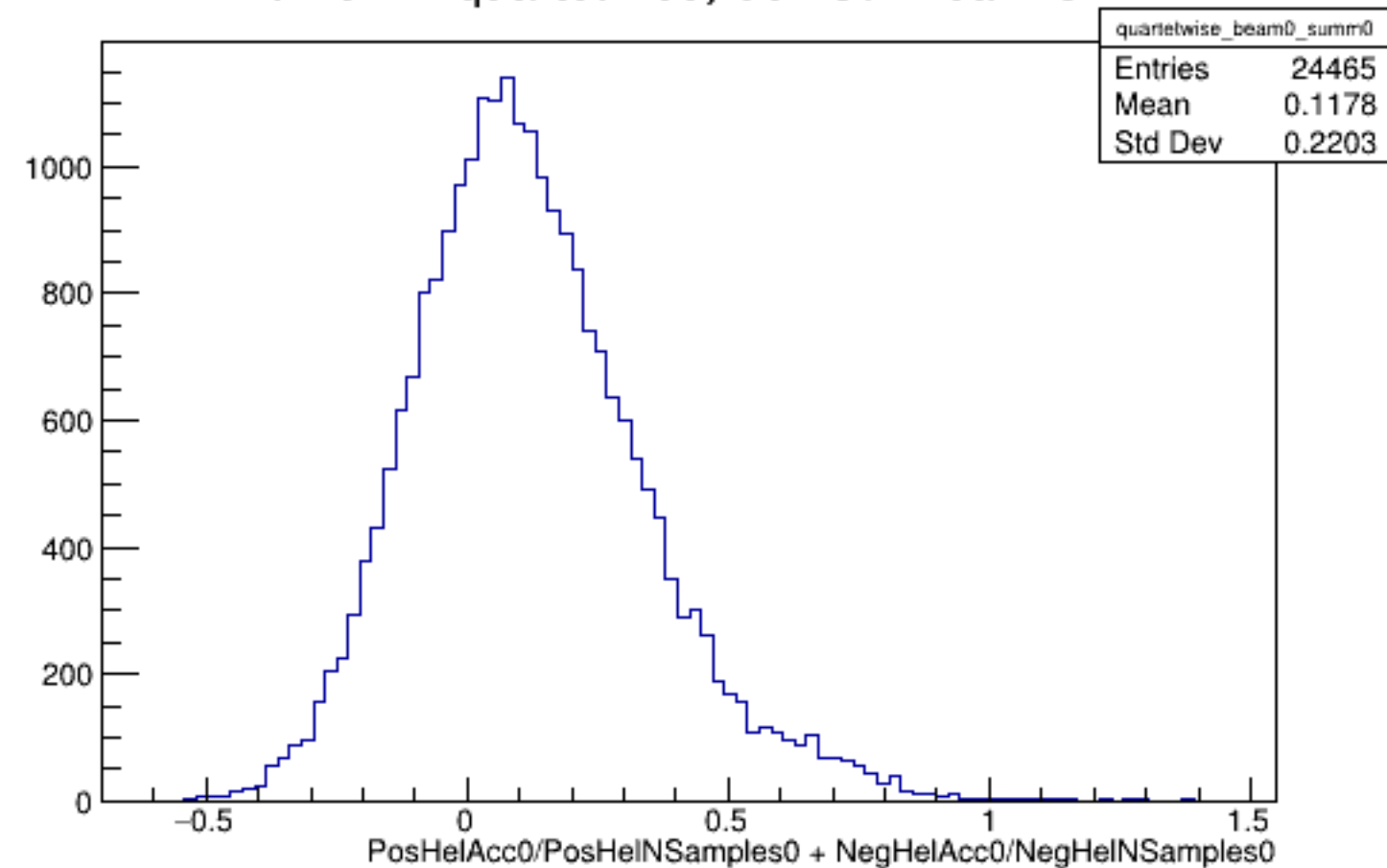
Run 5441 quartetwise, Sums0: Beam OFF
