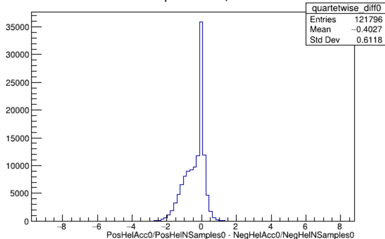
Run 5441 quartetwise, Diffs0: All
