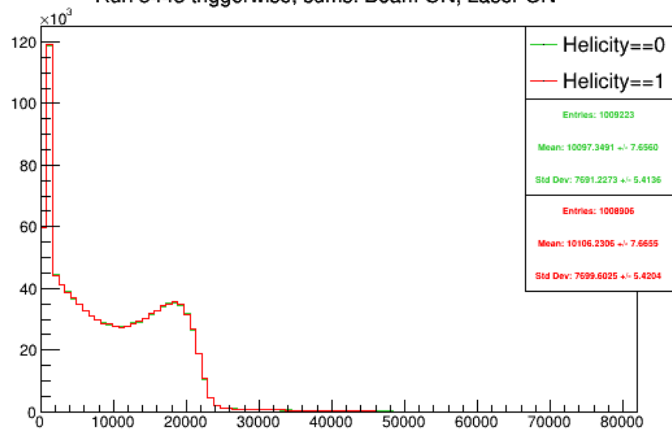
Run 5443 triggerwise, sums: Beam ON, Laser ON
