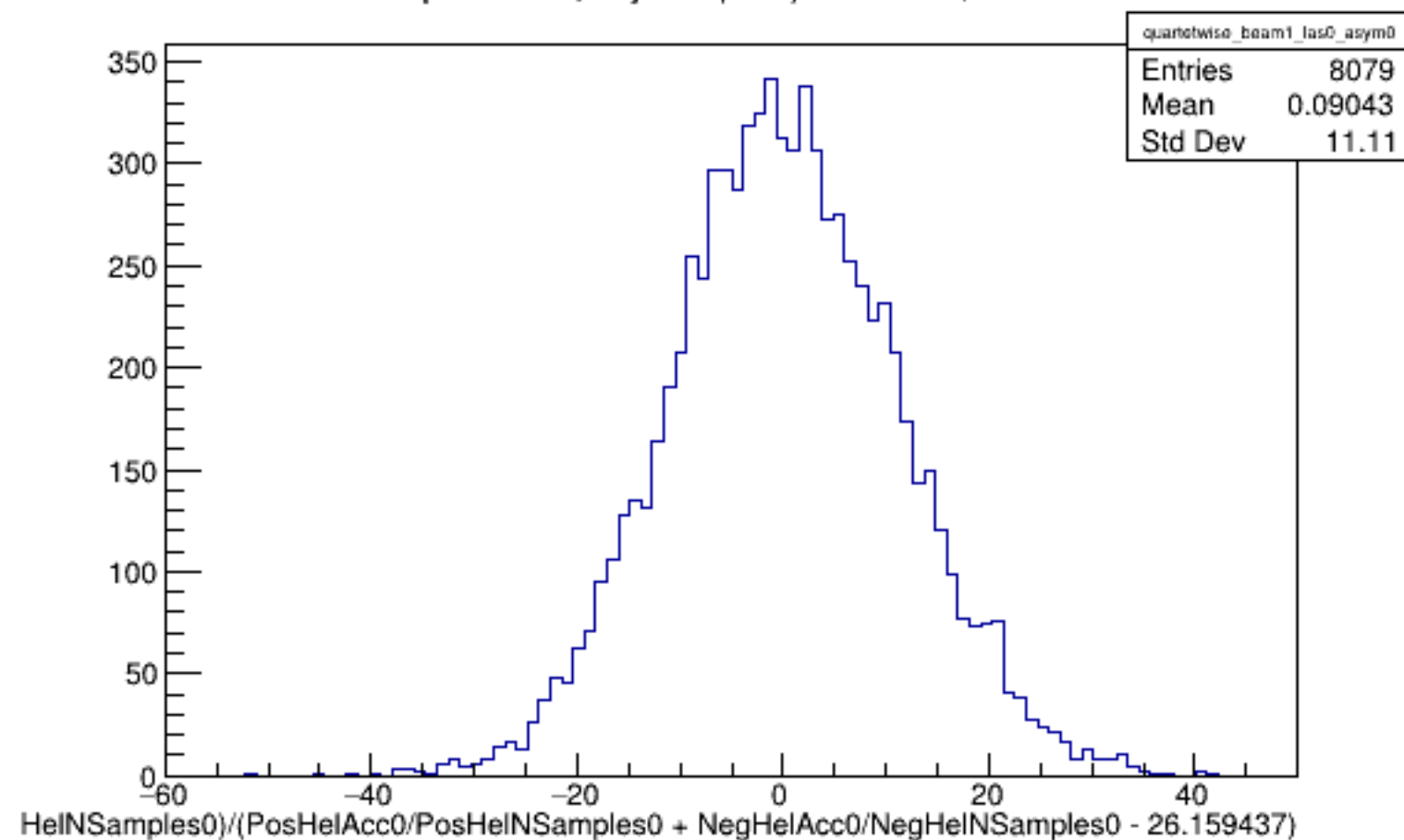
Run 5446 quartetwise, Asyms0 (Raw): Beam ON, Laser OFF
