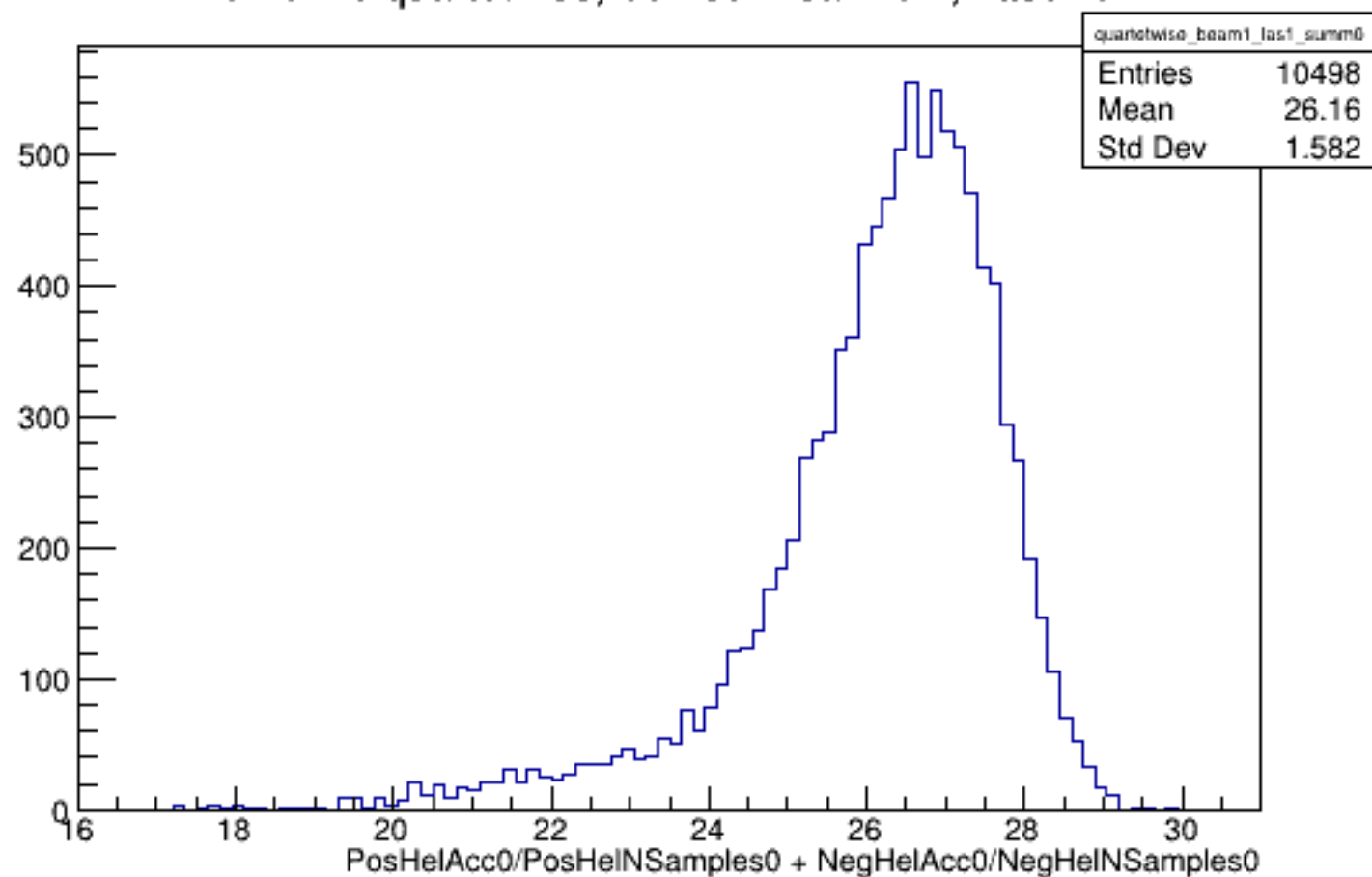
Run 5446 quartetwise, Sums0: Beam ON, Laser ON
