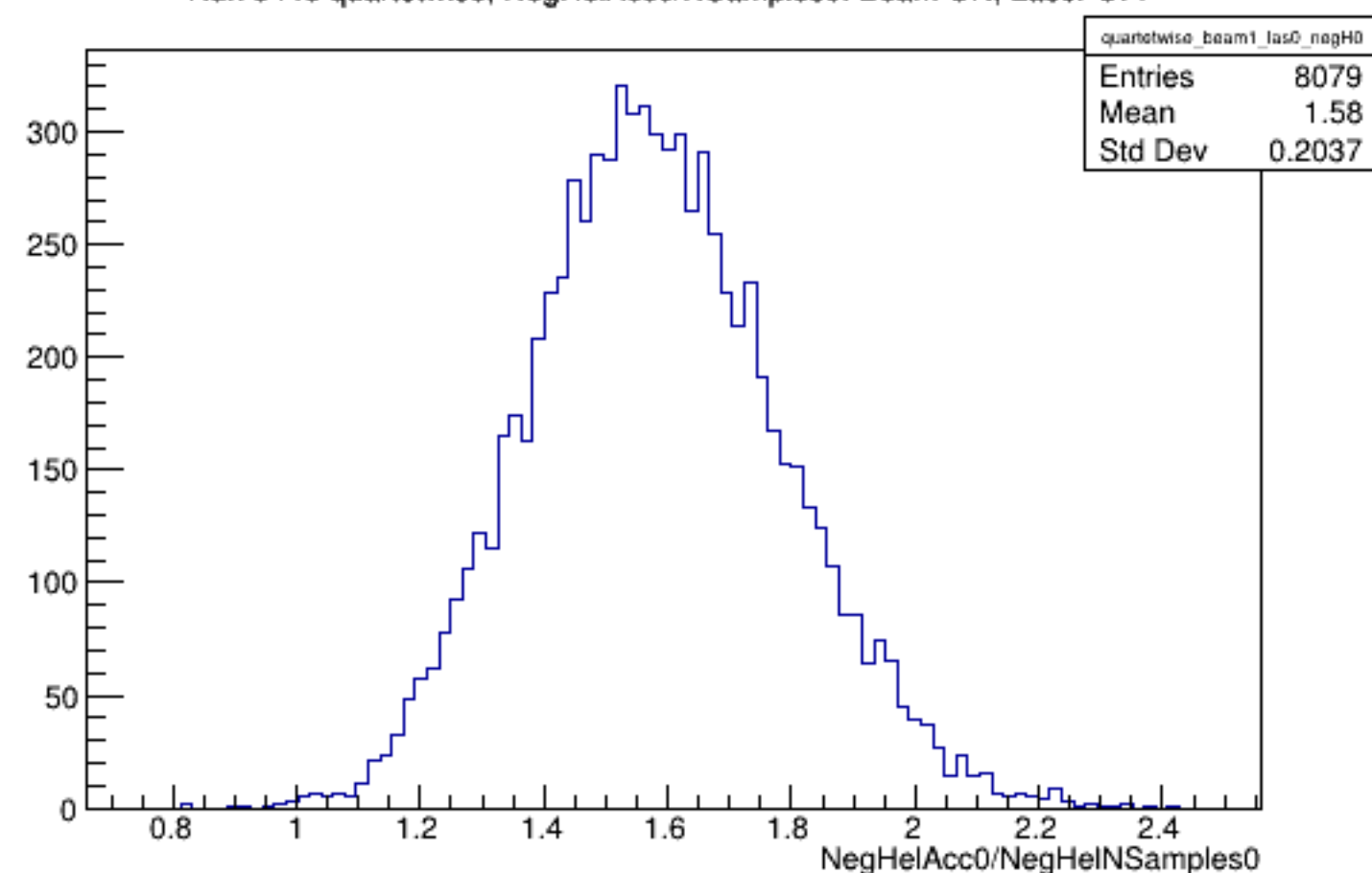
Run 5446 quartetwise, NegHelAcc0/NSamples0: Beam ON, Laser OFF
