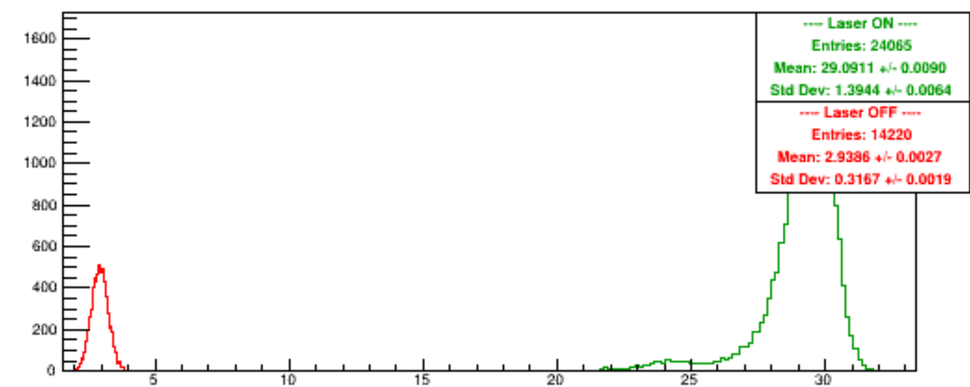
Run 5448 quartetwise, Sums0
