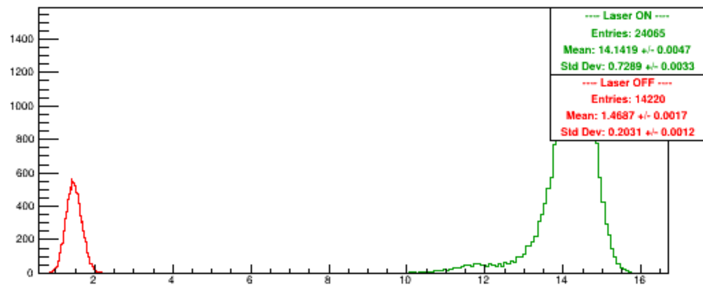
Run 5448 quartetwise, PosHelAcc0/NSamples0
