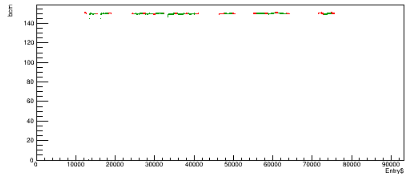
Run 5448 quartetwise, posH4 vs time
