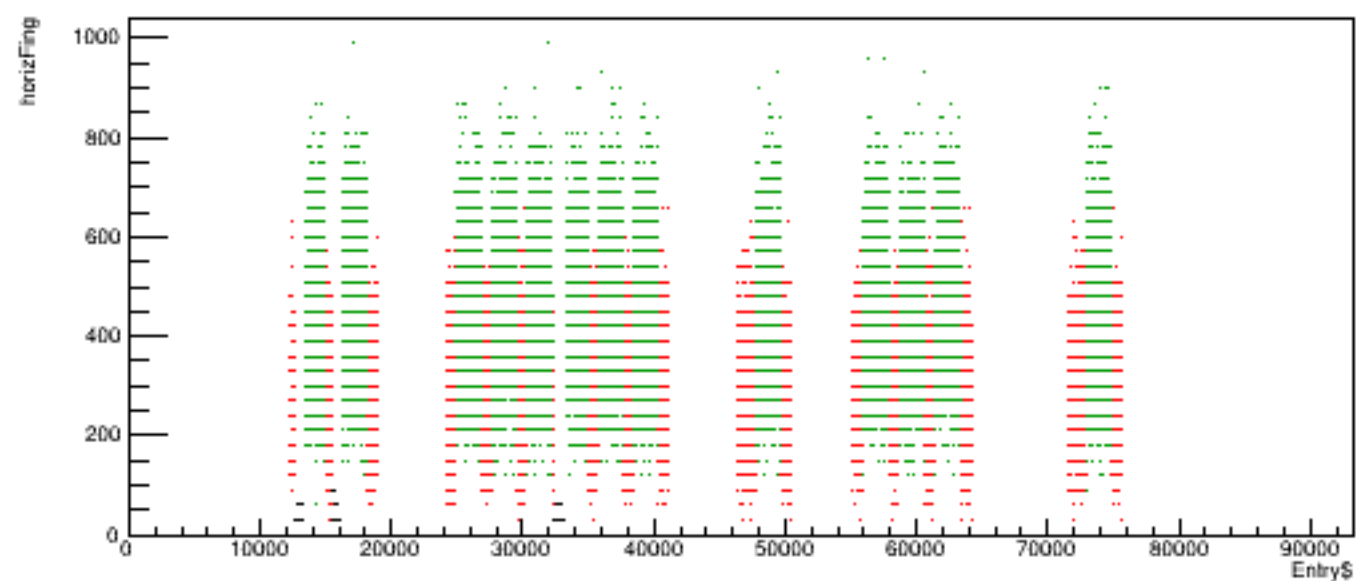
Run 5448 quartetwise, horizFing vs time
