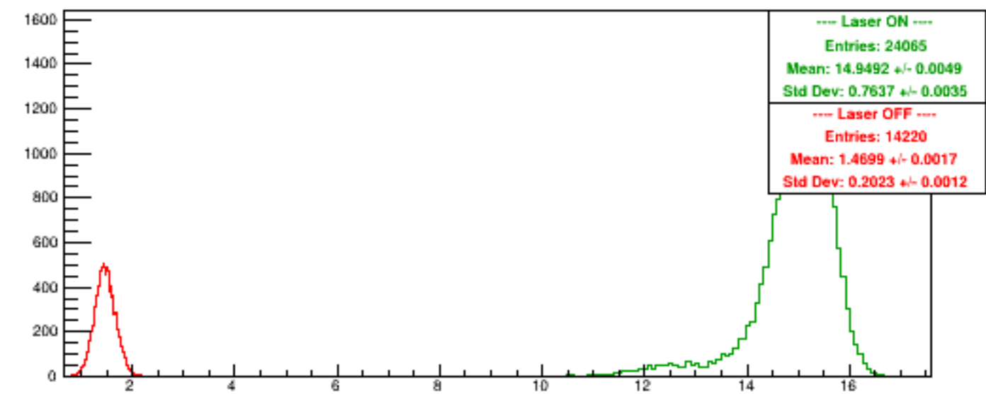
Run 5448 quartetwise, NegHelAcc0/NSamples0
