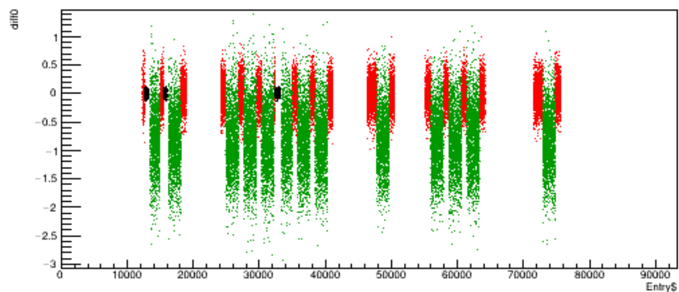
Run 5448 quartetwise, diff0 vs time
