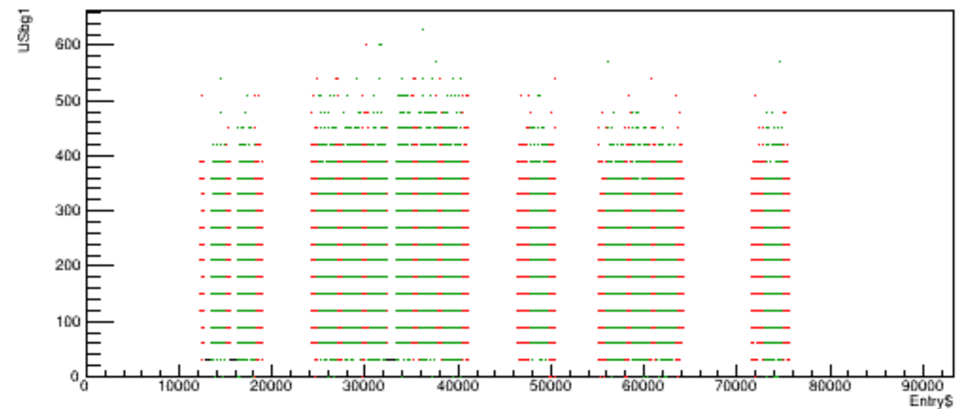
Run 5448 quartetwise, USbg1 vs time
