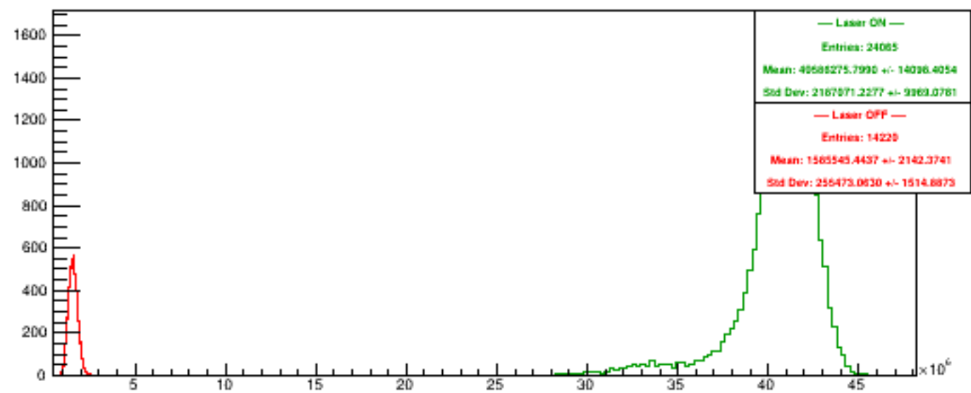
Run 5448 quartetwise, PosHelAcc4
