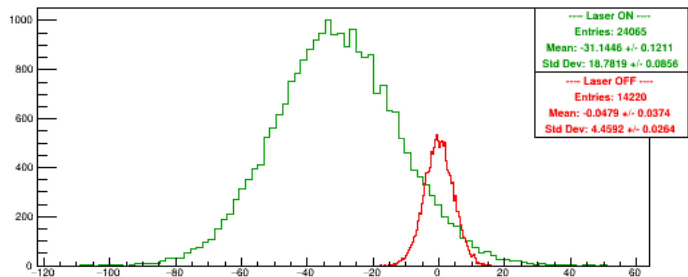
Run 5448 quartetwise, Asyms4
