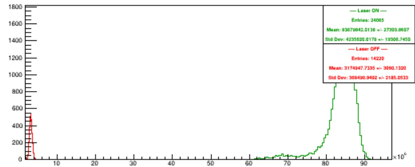
Run 5448 quartetwise, Sums4
