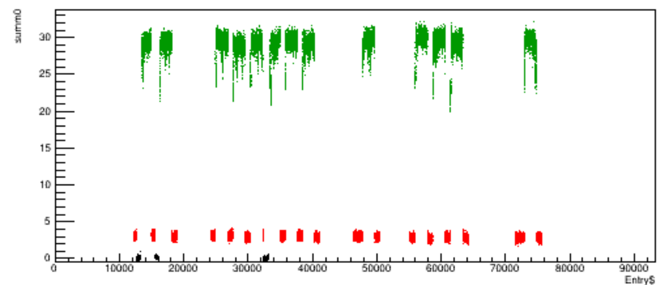
Run 5448 quartetwise, summ0 vs time
