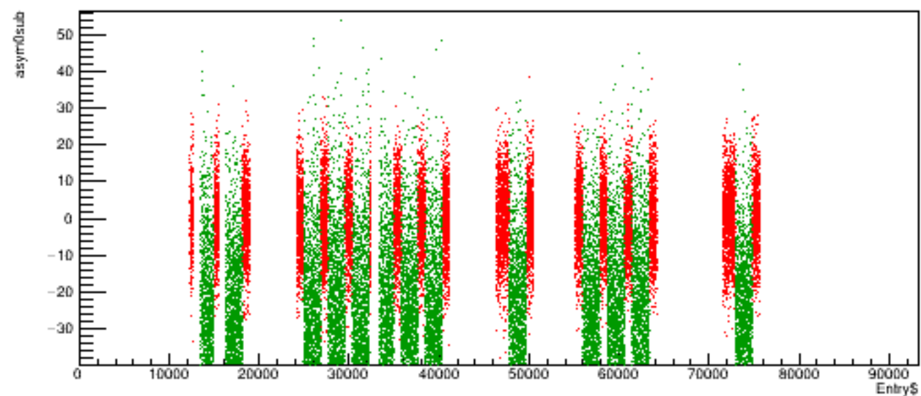
Run 5448 quartetwise, asym0sub vs time
