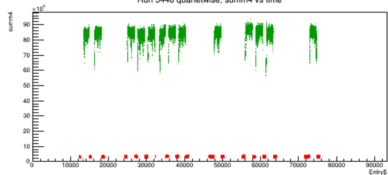
Run 5448 quartetwise, summ4 vs time
