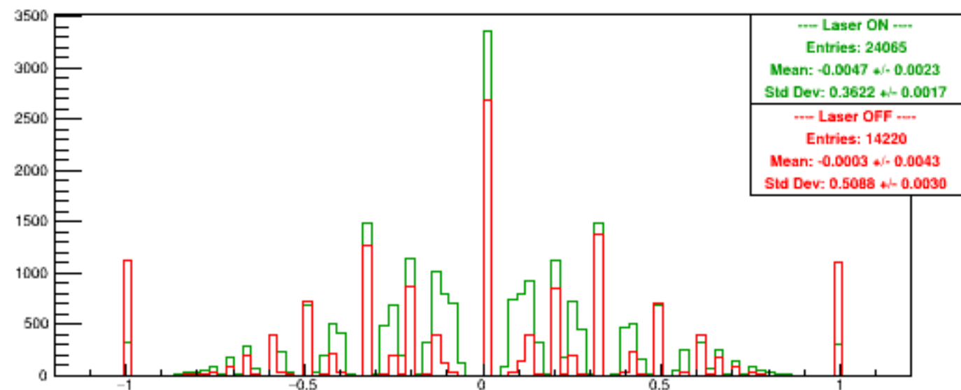
Run 5448 quartetwise, Asyms Horiz Finger
