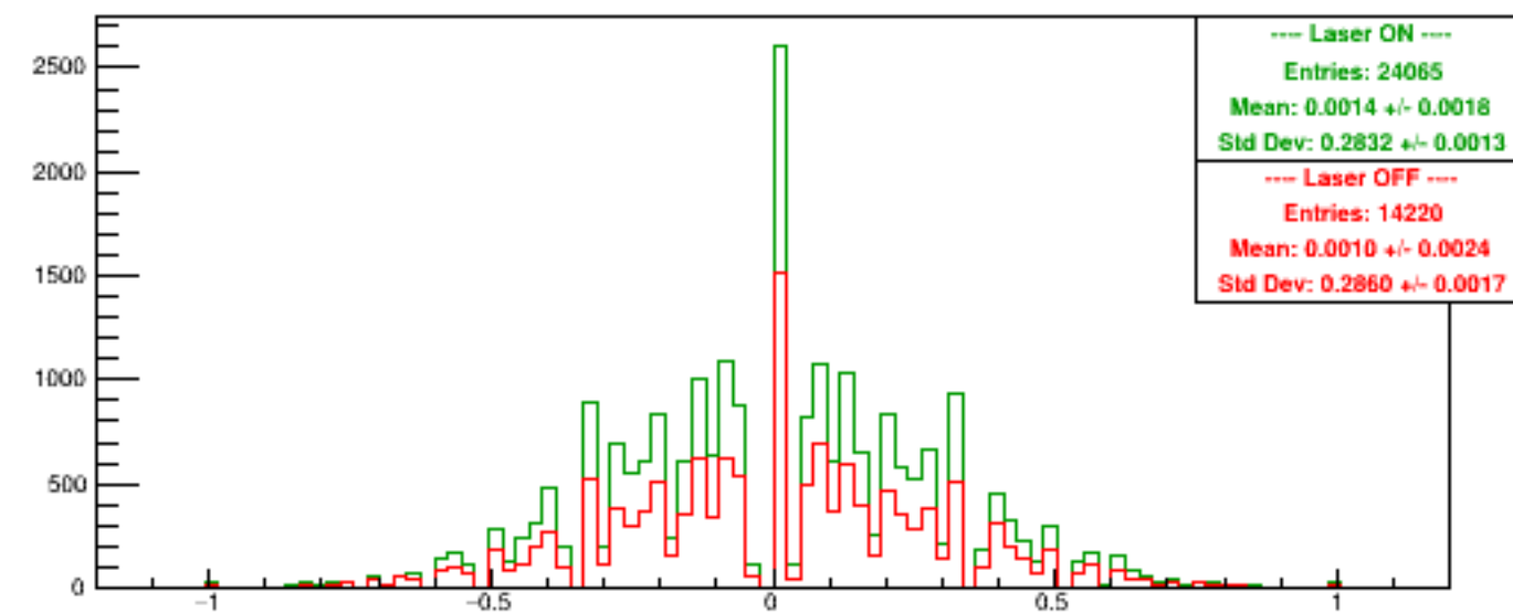
Run 5448 quartetwise, Asyms USbg2
