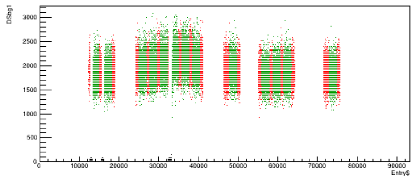
Run 5448 quartetwise, DSbg1 vs time
