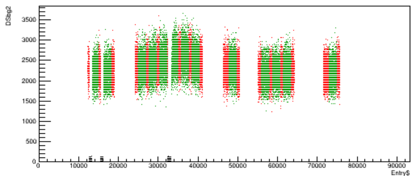
Run 5448 quartetwise, DSbg2 vs time
