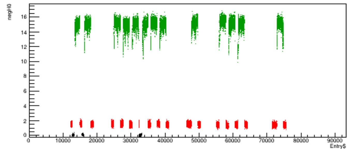
Run 5448 quartetwise, negH0 vs time
