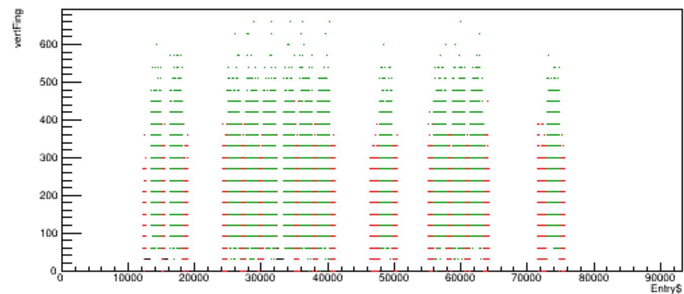
Run 5448 quartetwise, vertFing vs time
