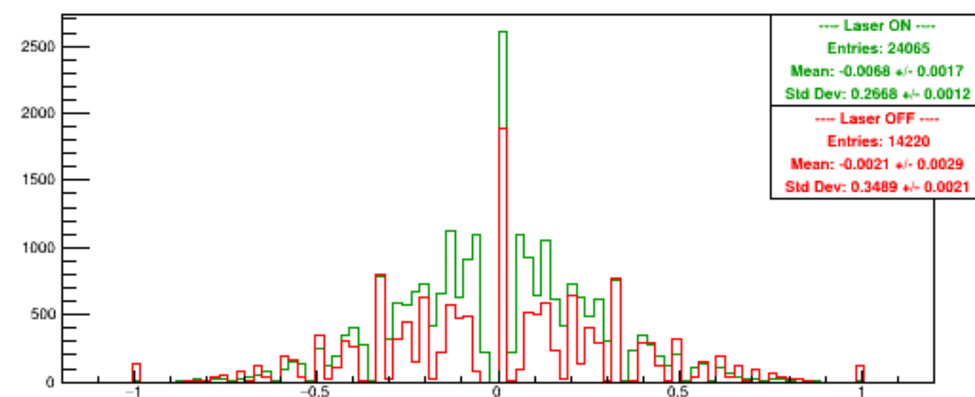
Run 5448 quartetwise, Asyms Vert Finger
