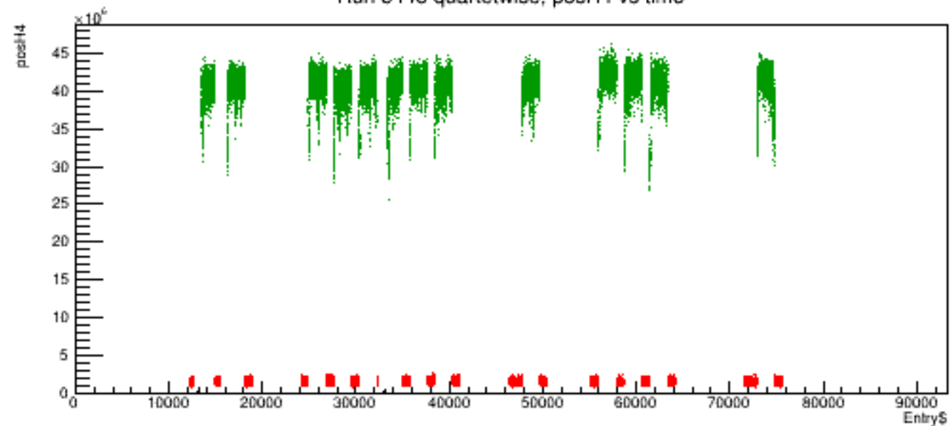
Run 5448 quartetwise, posH4 vs time
