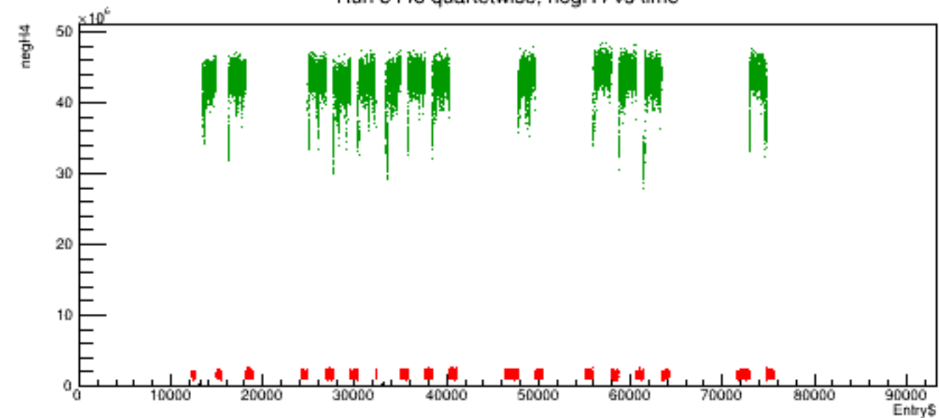
Run 5448 quartetwise, negH4 vs time
