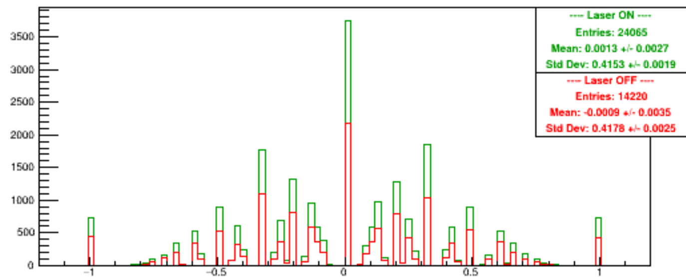
Run 5448 quartetwise, Asyms USbg1
