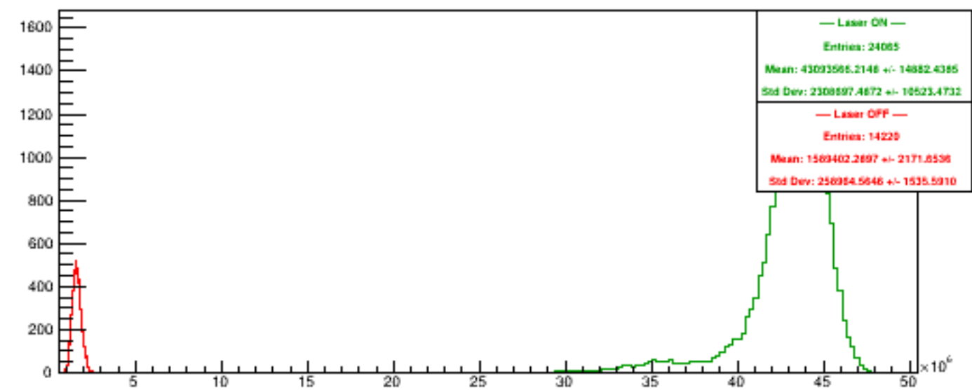
Run 5448 quartetwise, NegHelAcc4
