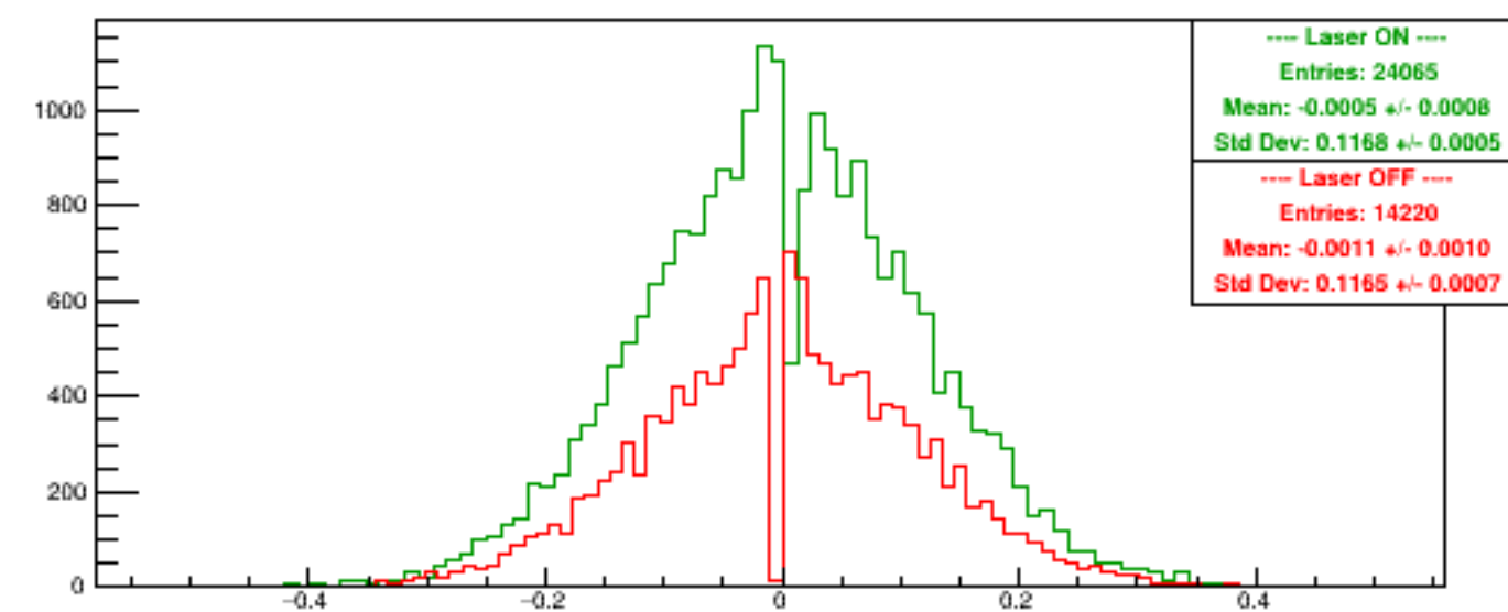
Run 5448 quartetwise, Asyms DSbg2
