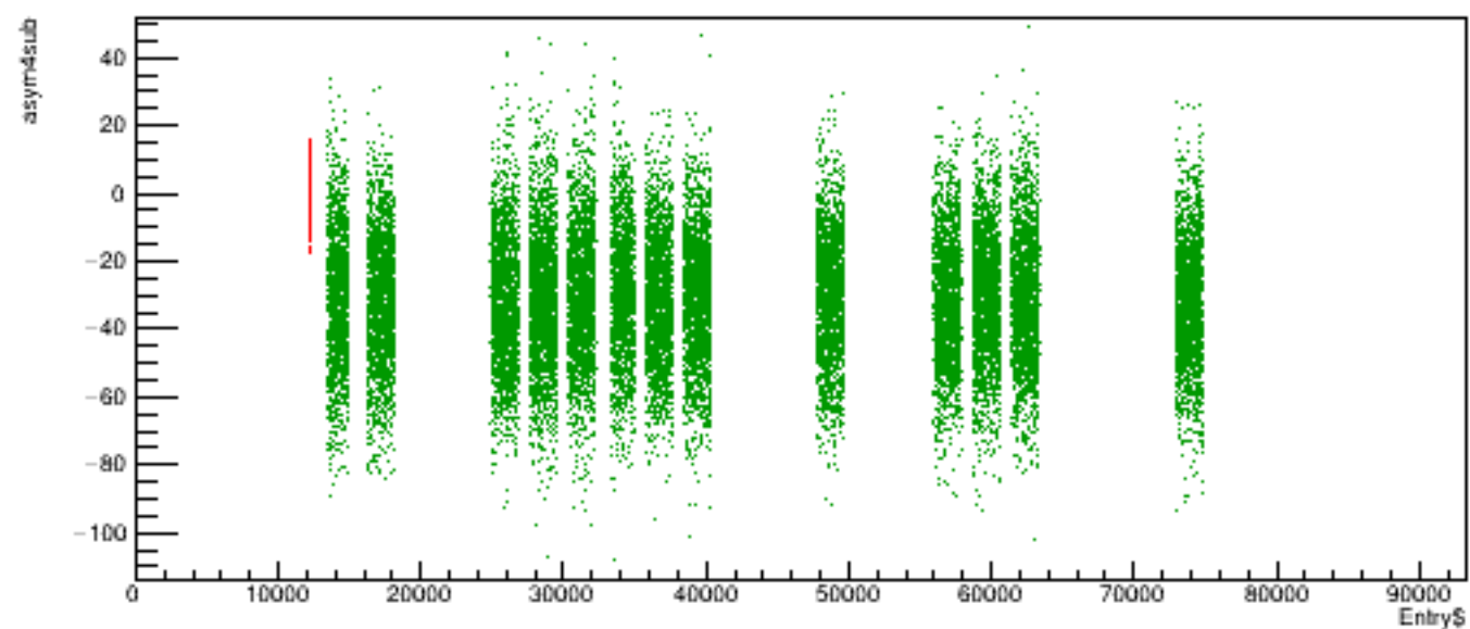
Run 5448 quartetwise, asym4sub vs time
