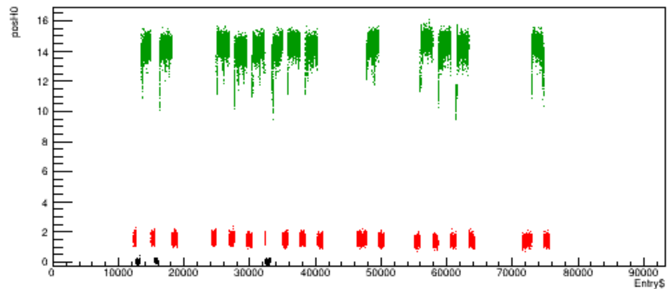
Run 5448 quartetwise, posH0 vs time
