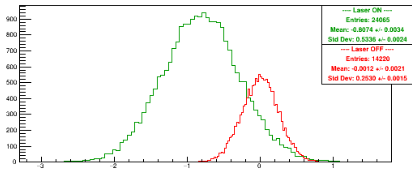
Run 5448 quartetwise, Diffs0
