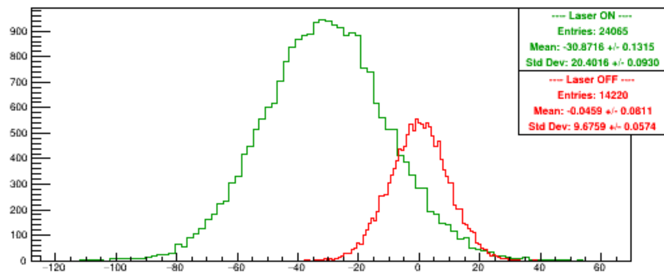
Run 5448 quartetwise, Asyms0
