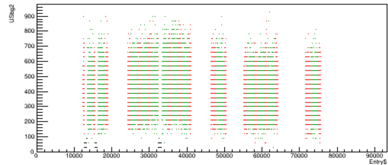
Run 5448 quartetwise, USbg2 vs time
