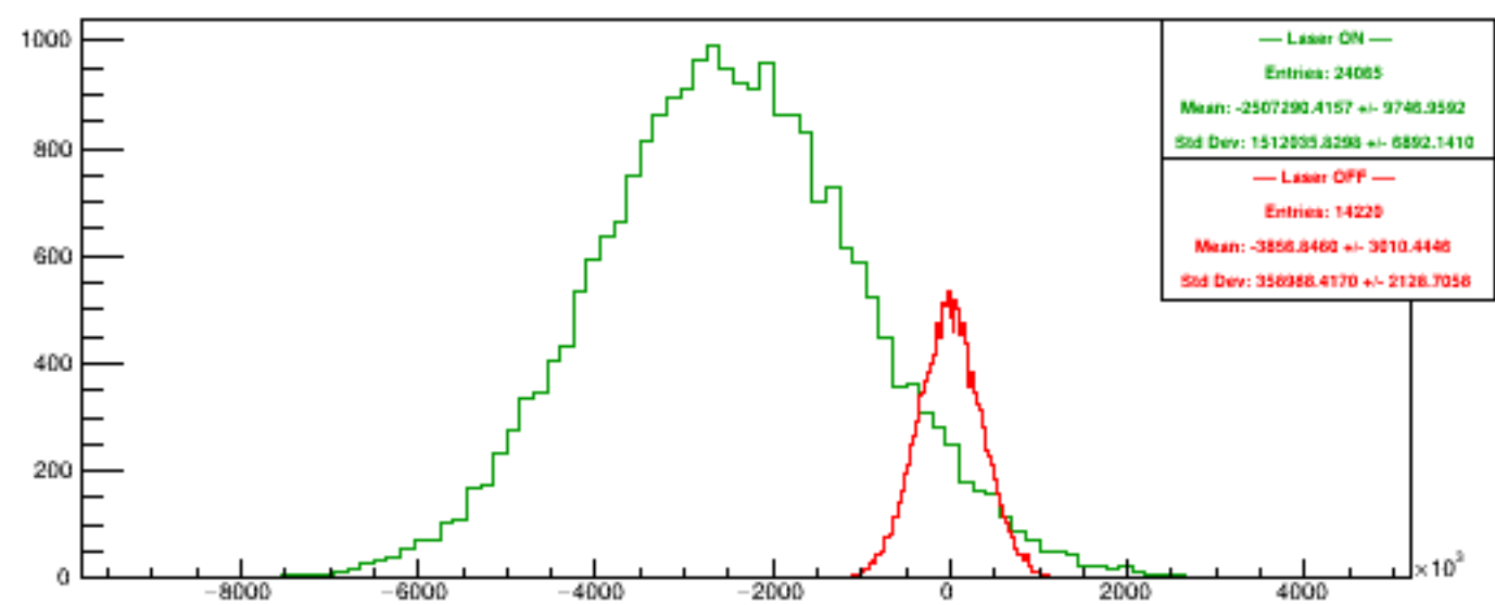
Run 5448 quartetwise, Diffs4
