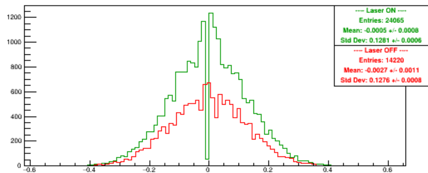
Run 5448 quartetwise, Asyms DSbg1
