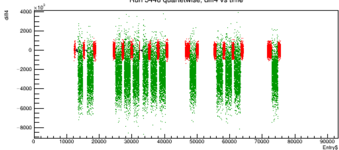
Run 5448 quartetwise, diff4 vs time
