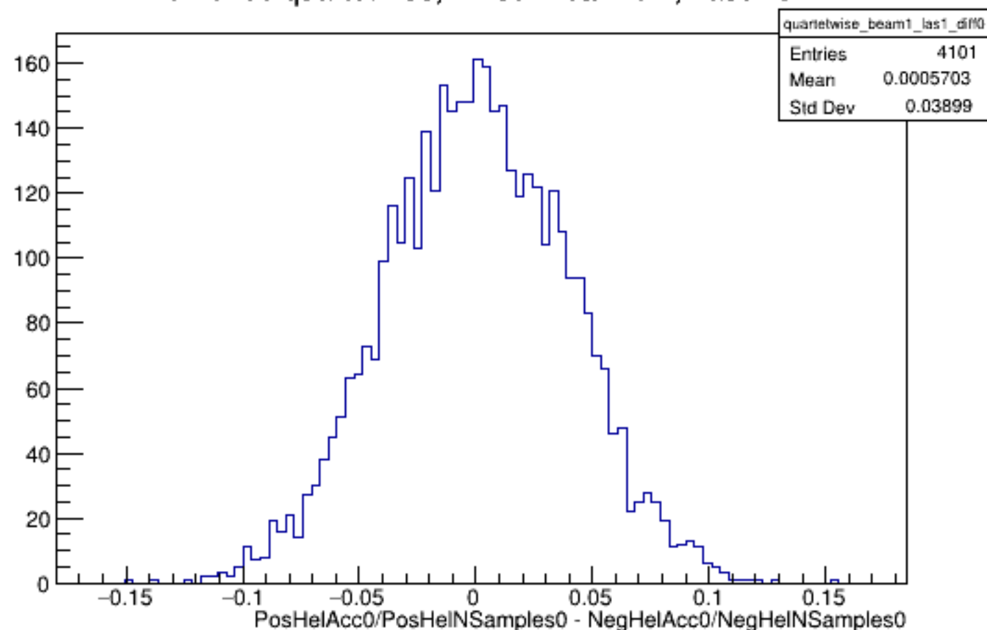
Run 5465 quartetwise, Diffs0: Beam ON, Laser ON
