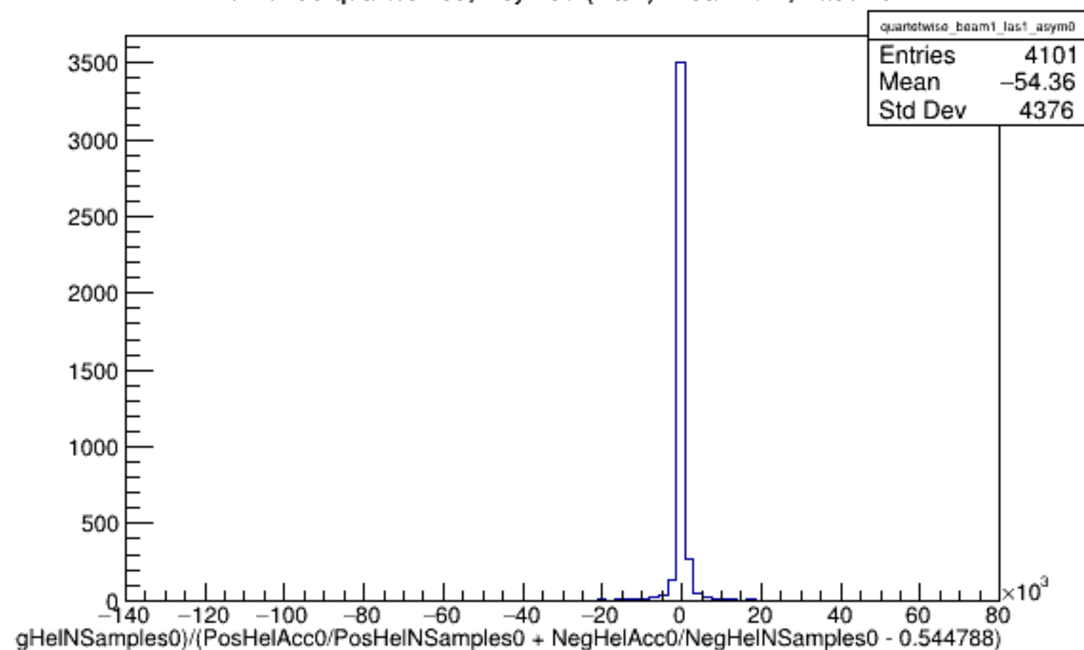
Run 5465 quartetwise, Asyms0 (Raw): Beam ON, Laser ON
