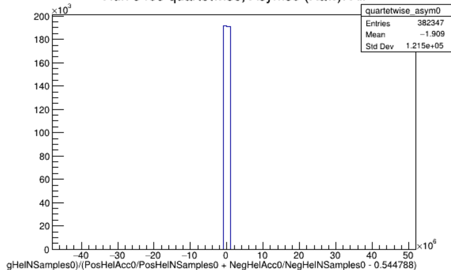
Run 5465 quartetwise, Asyms0 (Raw): All
