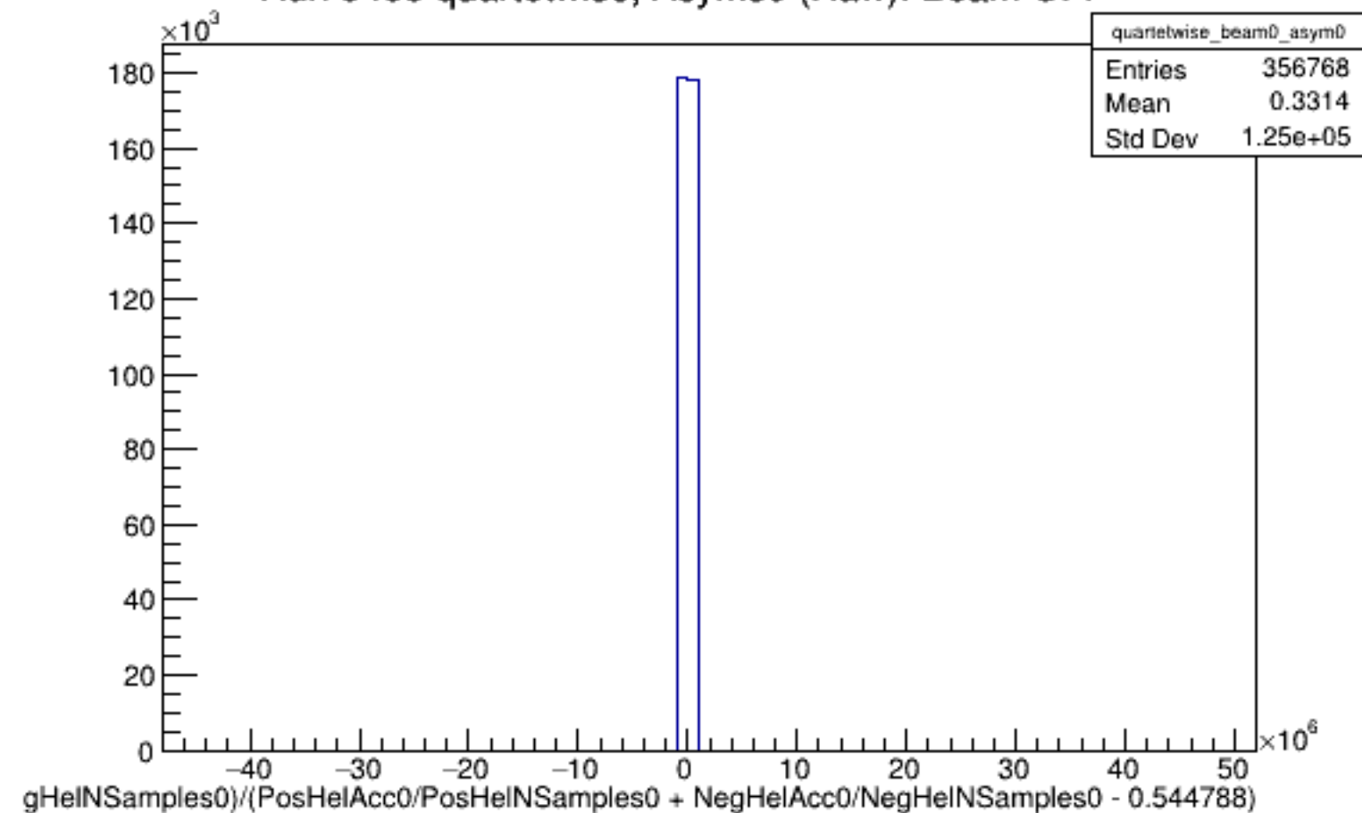
Run 5465 quartetwise, Asyms0 (Raw): Beam OFF
