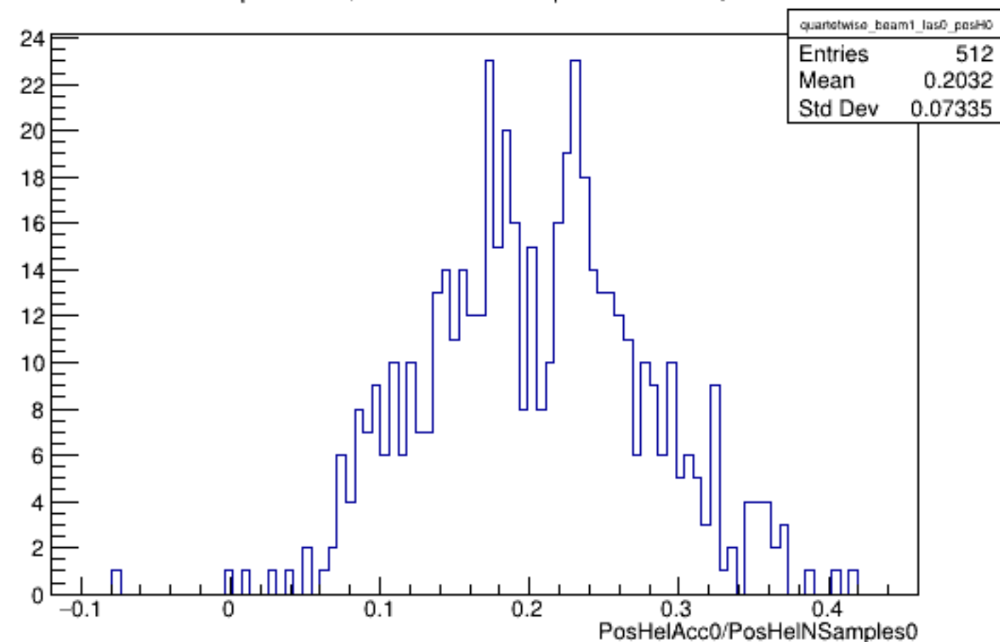
Run 5465 quartetwise, PosHelAcc0/NSamples0: Beam ON, Laser OFF
