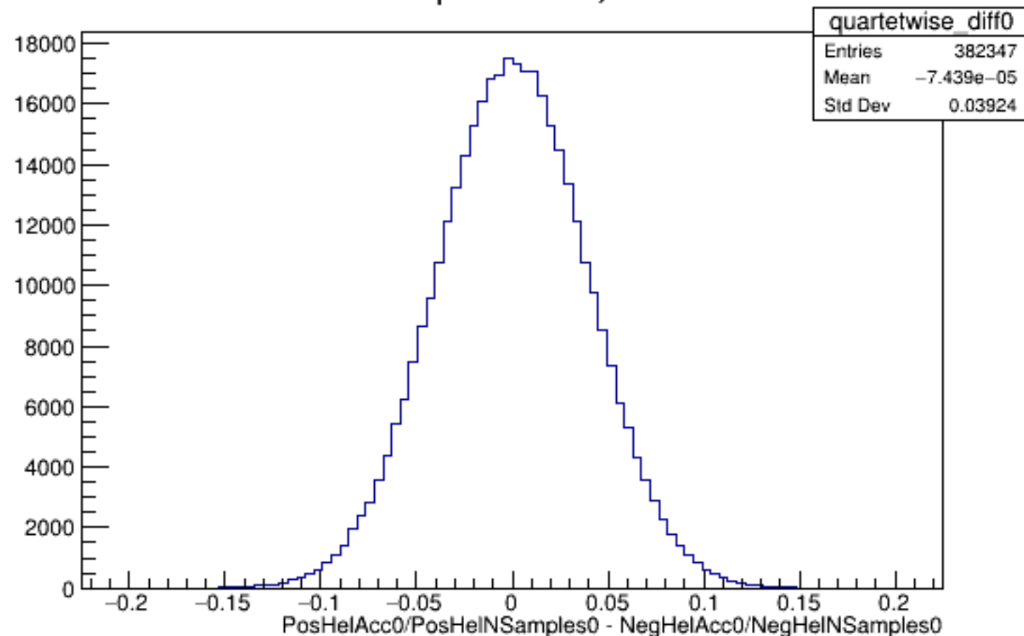
Run 5465 quartetwise, Diffs0: All
