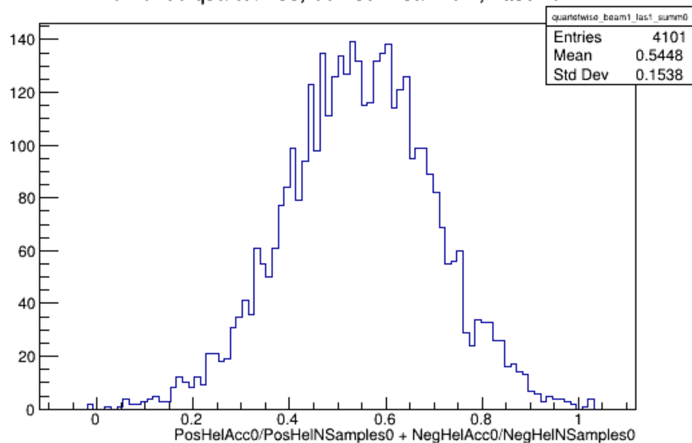
Run 5465 quartetwise, Sums0: Beam ON, Laser ON
