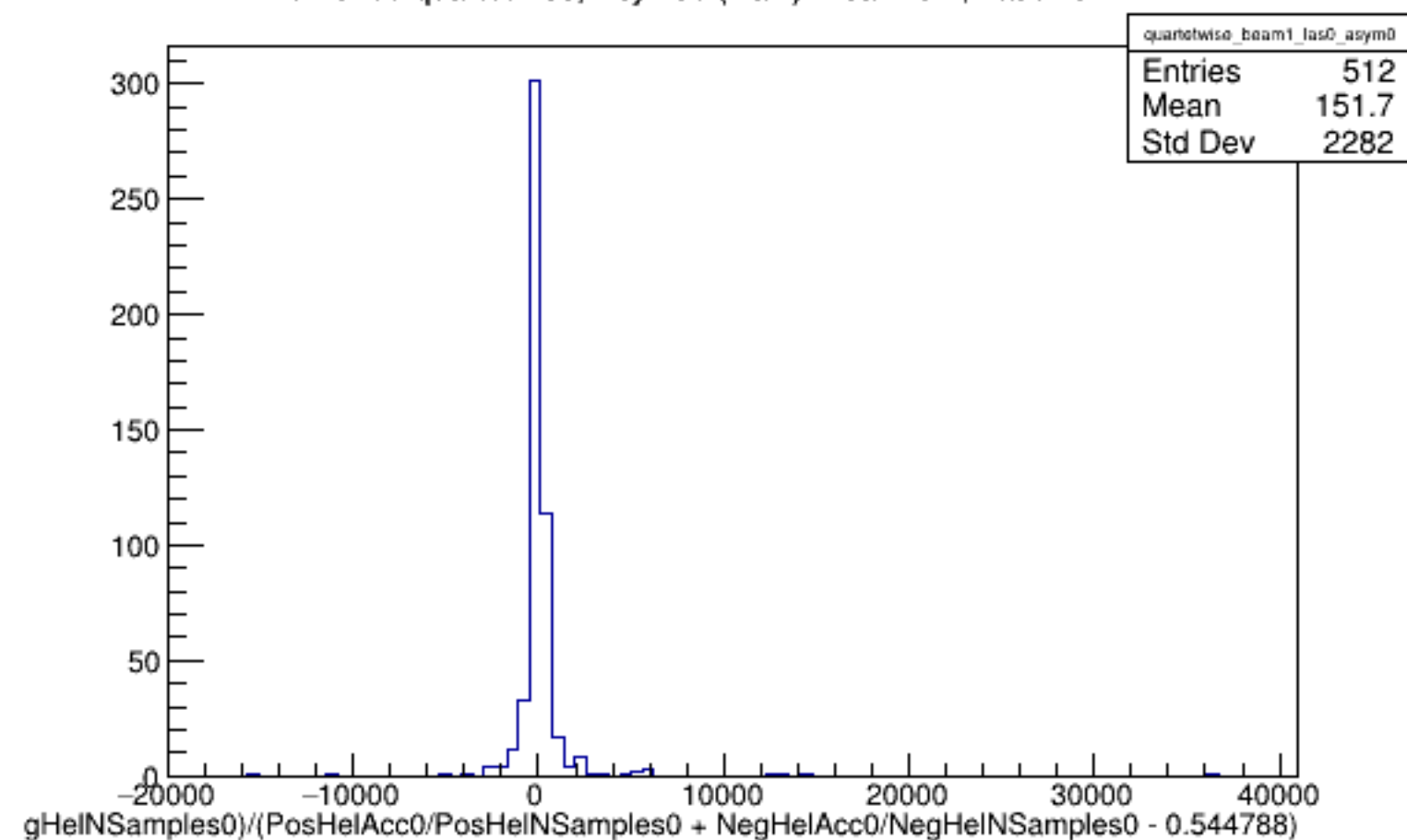
Run 5465 quartetwise, Asyms0 (Raw): Beam ON, Laser OFF
