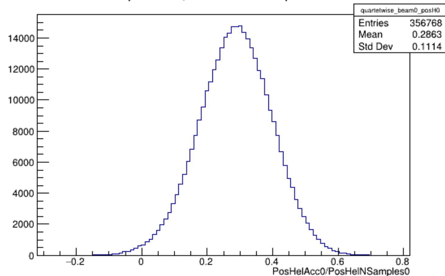
Run 5465 quartetwise, PosHelAcc0/NSamples0: Beam OFF
