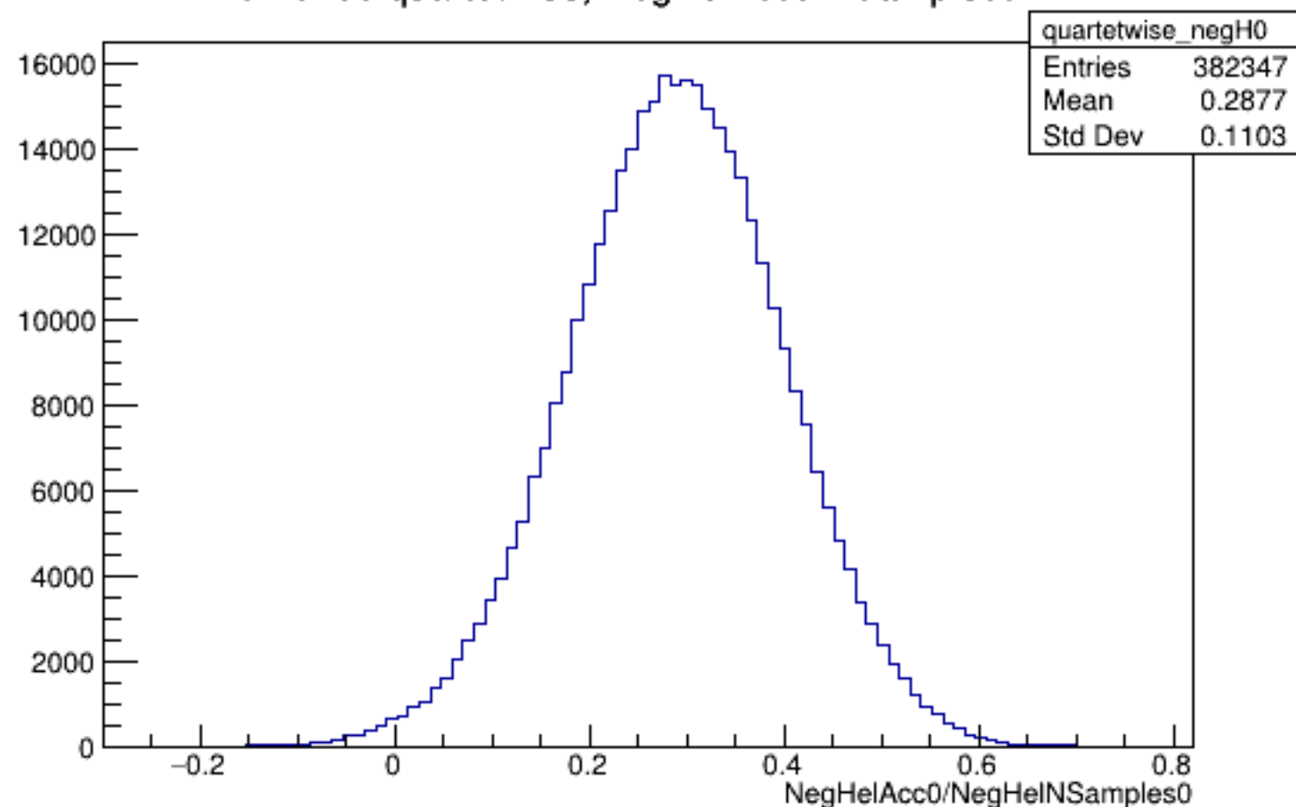
Run 5465 quartetwise, NegHelAcc0/NSamples0: All
