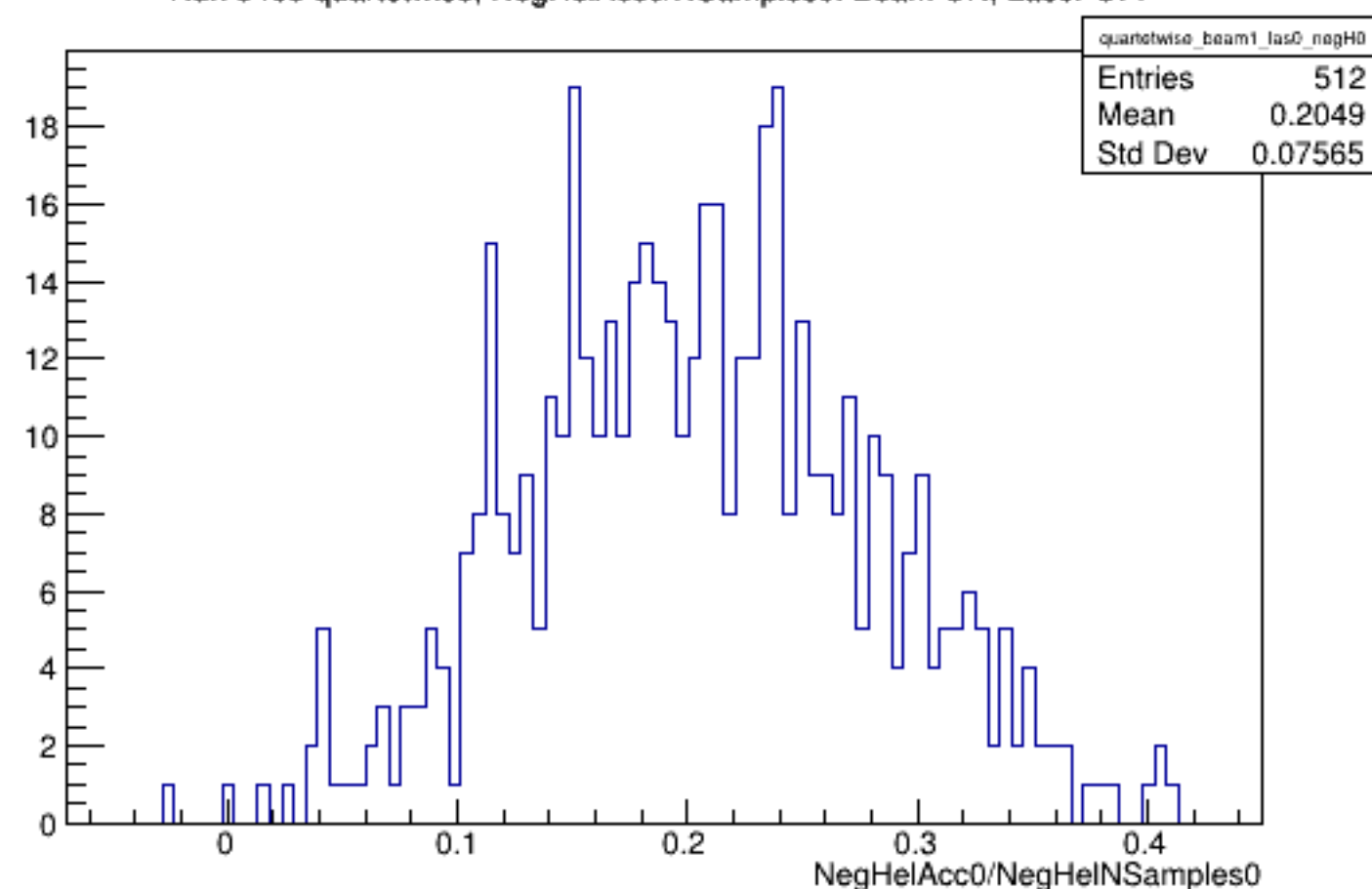
Run 5465 quartetwise, NegHelAcc0/NSamples0: Beam ON, Laser OFF
