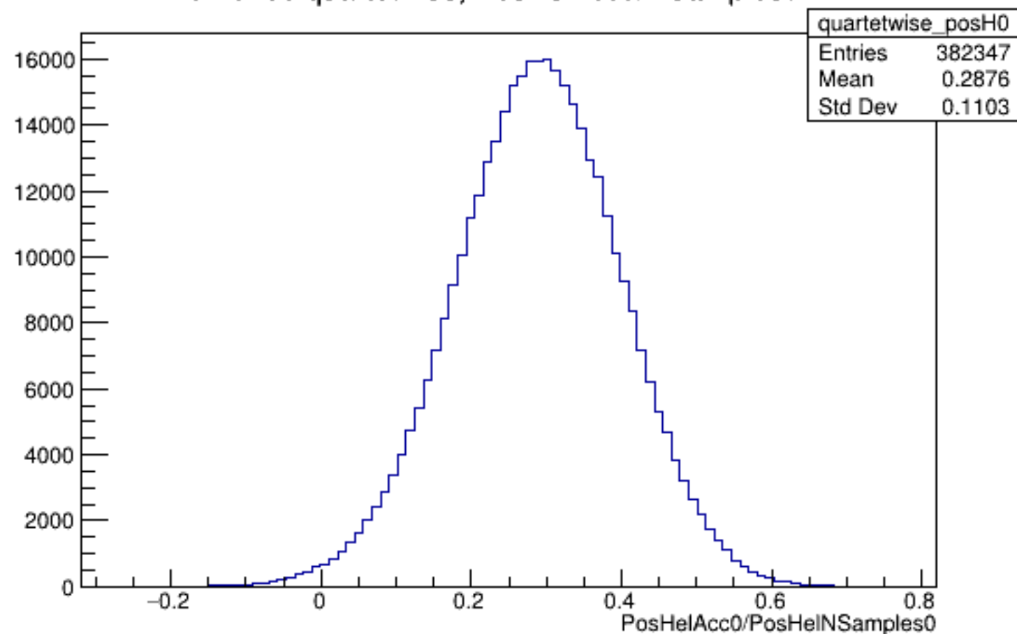
Run 5465 quartetwise, PosHelAcc0/NSamples0: All
