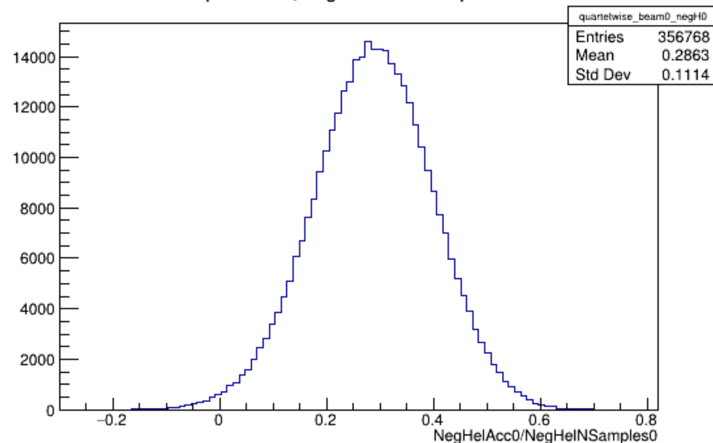
Run 5465 quartetwise, NegHelAcc0/NSamples0: Beam OFF
