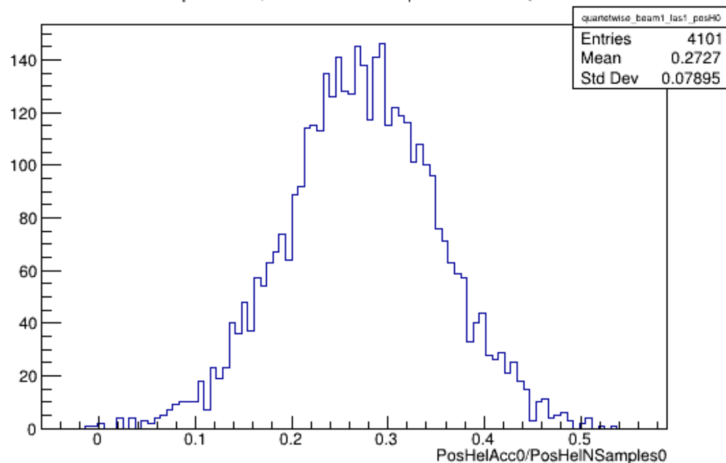
Run 5465 quartetwise, PosHelAcc0/NSamples0: Beam ON, Laser ON
