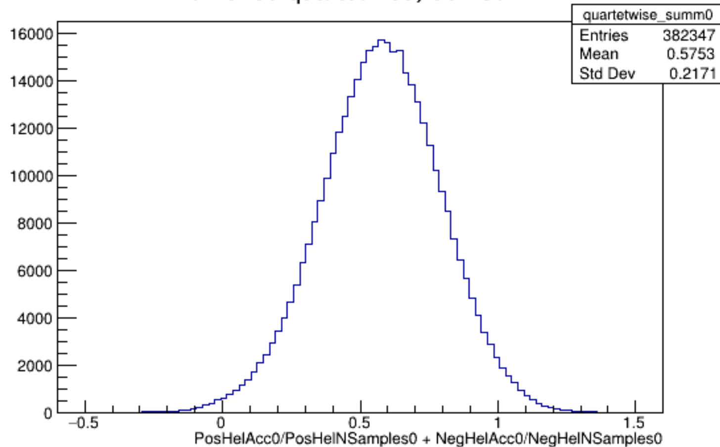
Run 5465 quartetwise, Sums0: All
