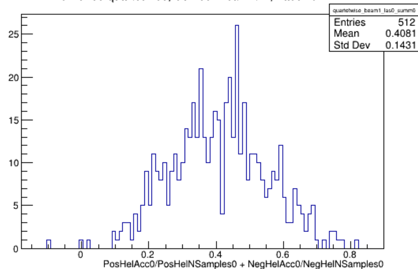
Run 5465 quartetwise, Sums0: Beam ON, Laser OFF
