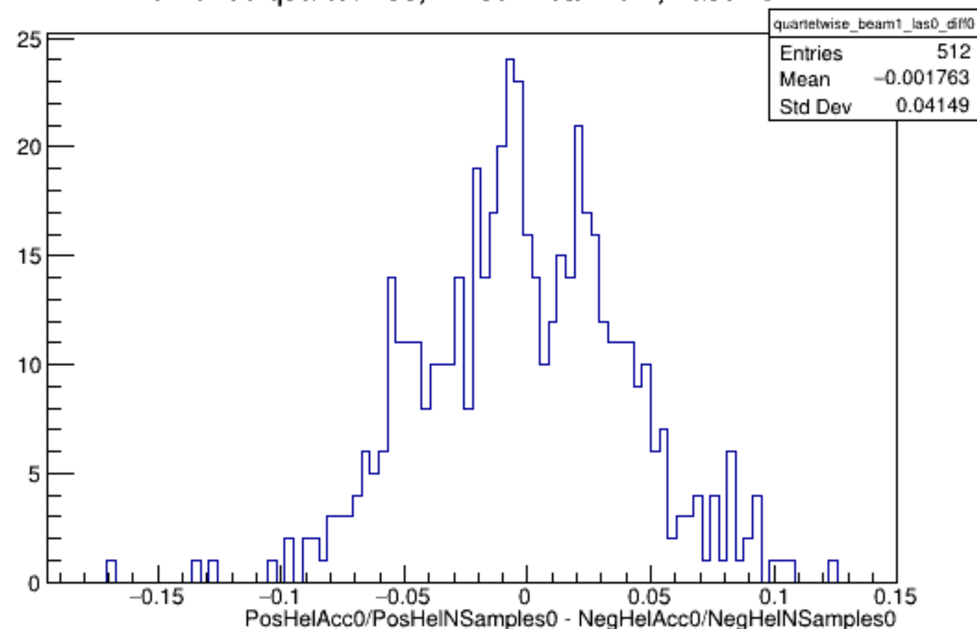
Run 5465 quartetwise, Diffs0: Beam ON, Laser OFF
