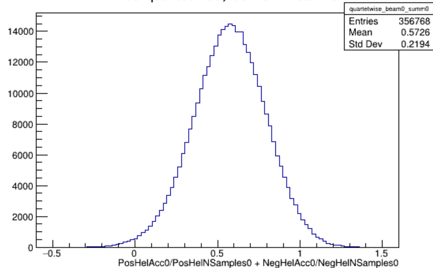
Run 5465 quartetwise, Sums0: Beam OFF
