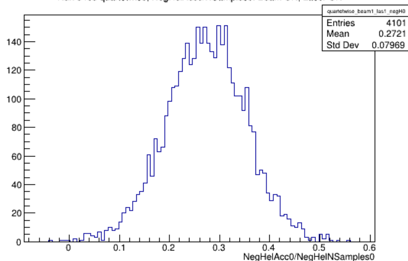
Run 5465 quartetwise, NegHelAcc0/NSamples0: Beam ON, Laser ON
