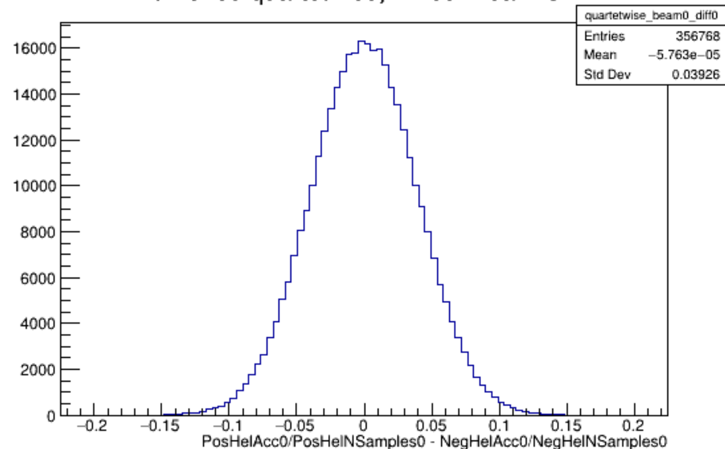
Run 5465 quartetwise, Diffs0: Beam OFF
