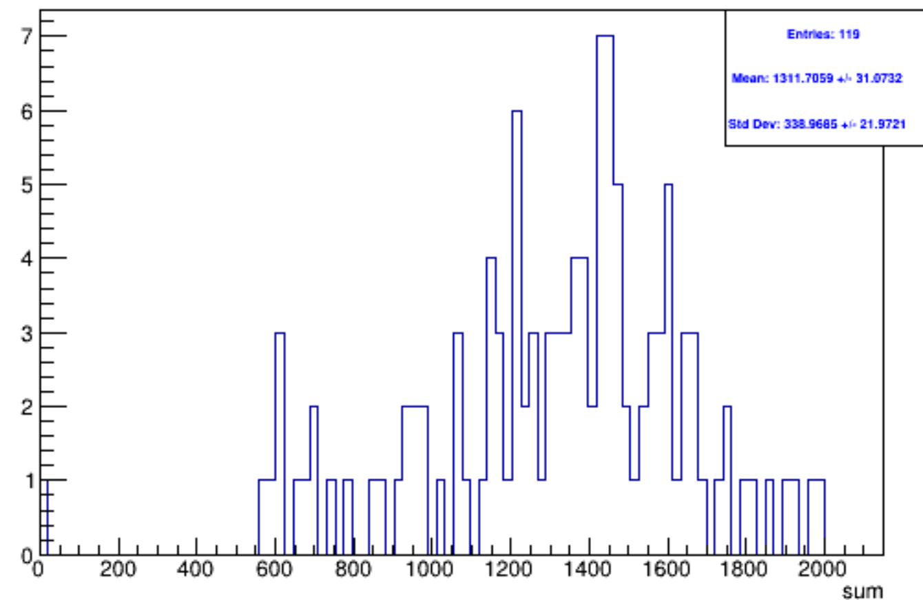
Run 5465 triggerwise, sums: Beam OFF
