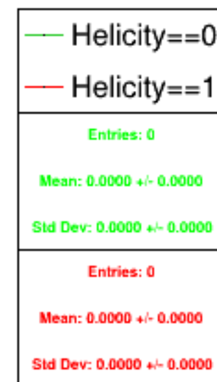
Run 5465 triggerwise, sums: Beam ON, Laser OFF
