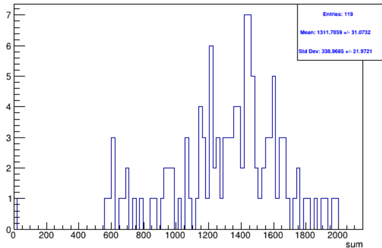
Run 5465 triggerwise, sums: All
