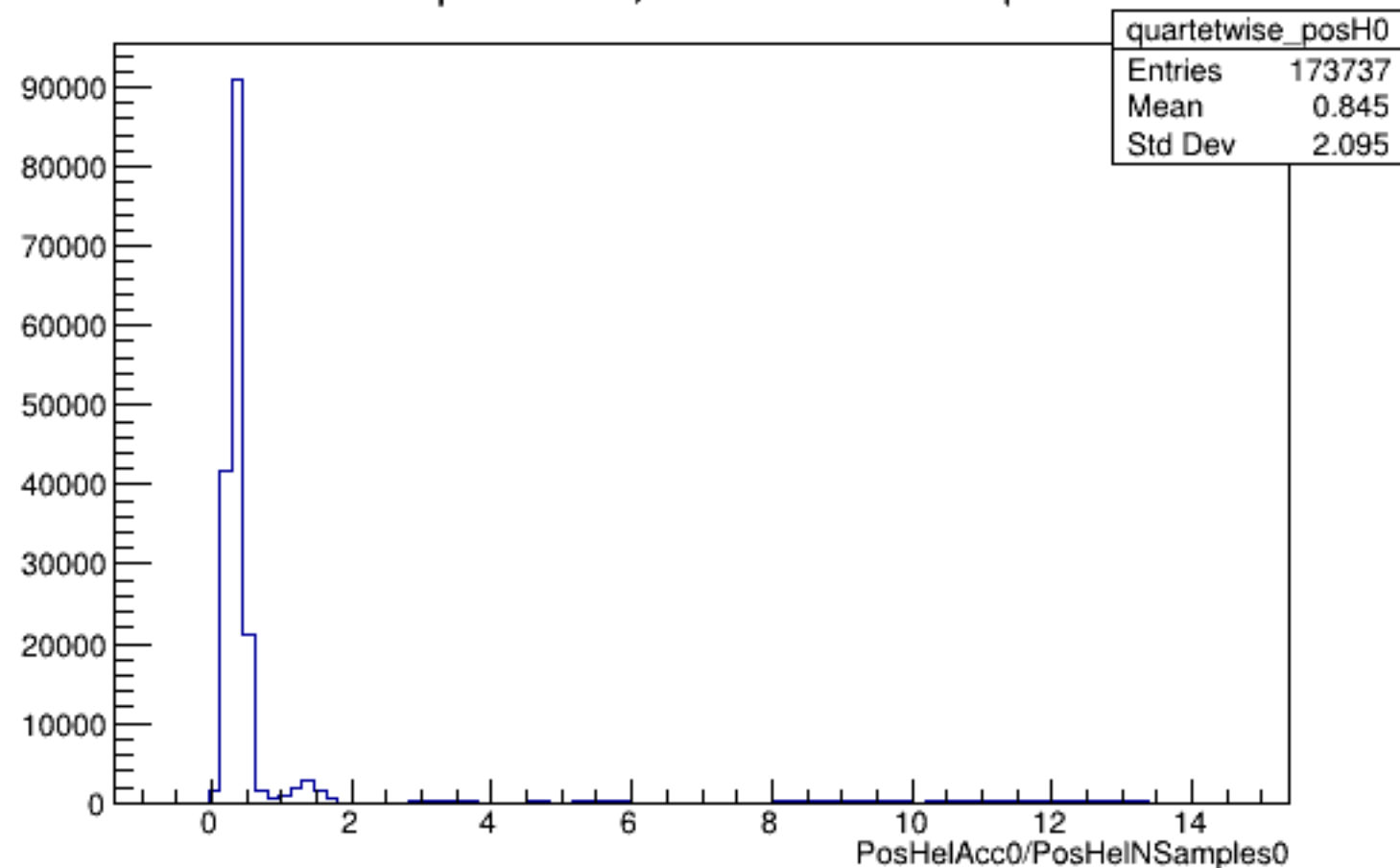
Run 5469 quartetwise, PosHelAcc0/NSamples0: All
