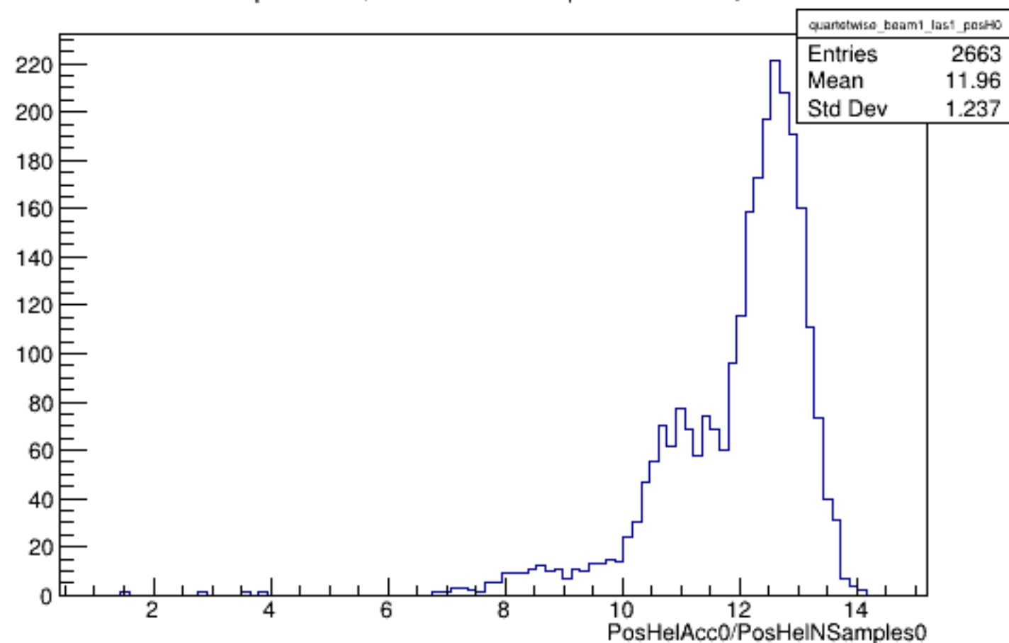
Run 5469 quartetwise, PosHelAcc0/NSamples0: Beam ON, Laser ON
