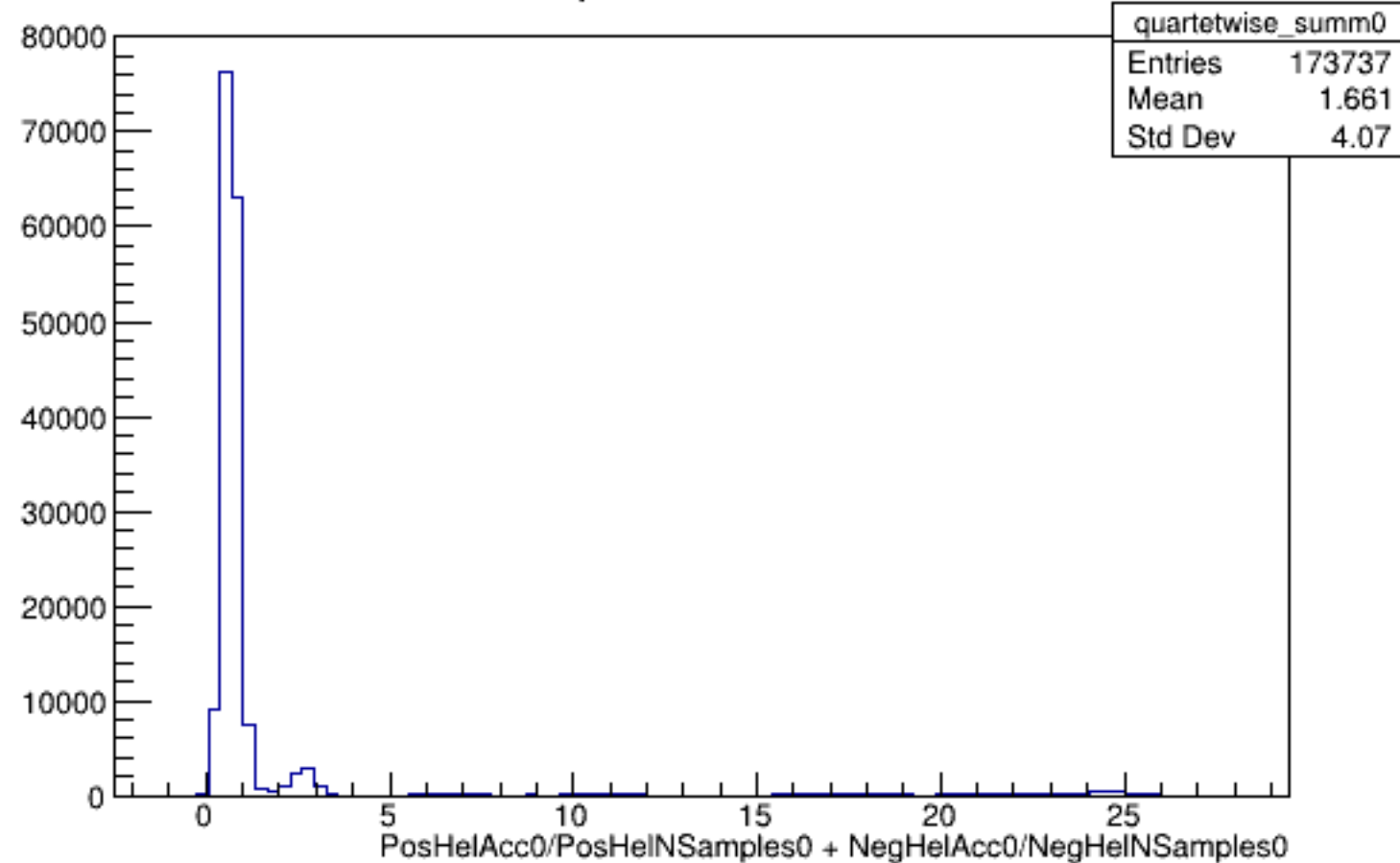
Run 5469 quartetwise, Sums0: All
