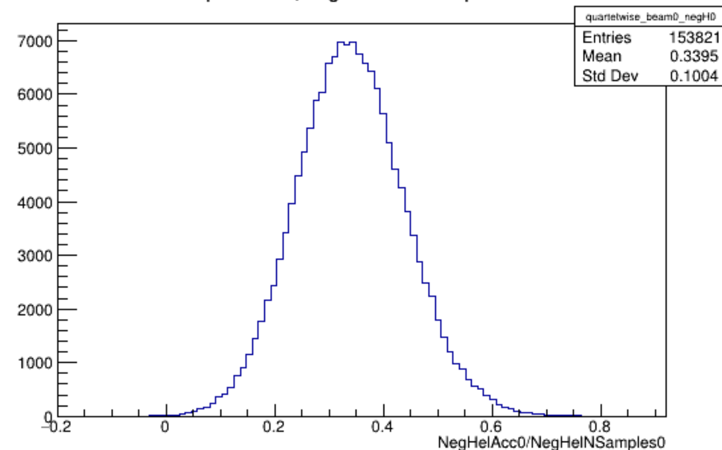
Run 5469 quartetwise, NegHelAcc0/NSamples0: Beam OFF
