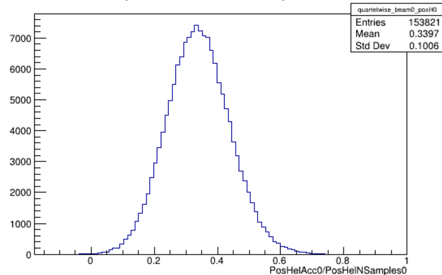
Run 5469 quartetwise, PosHelAcc0/NSamples0: Beam OFF
