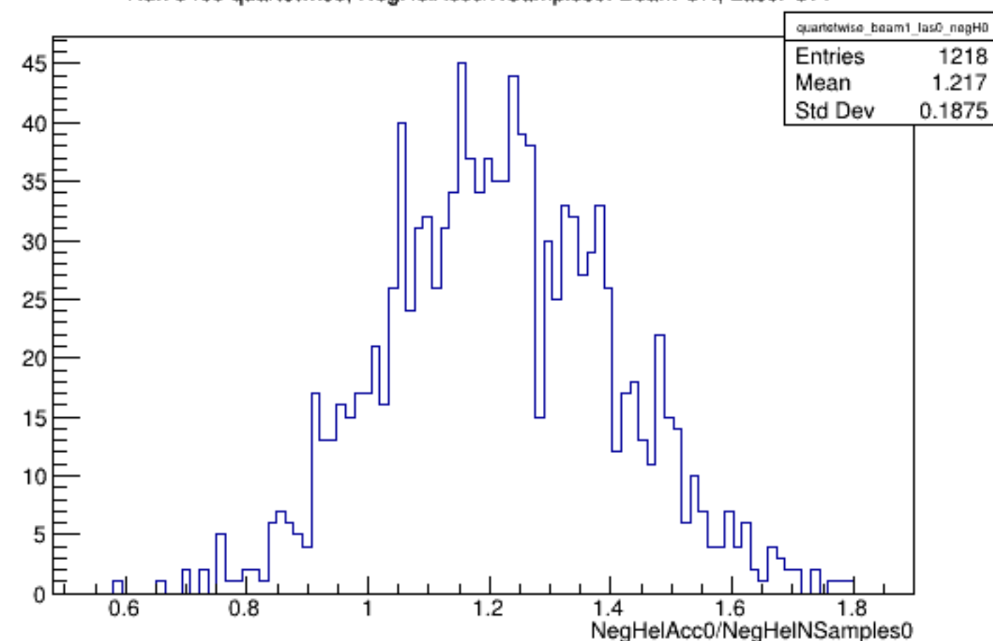
Run 5469 quartetwise, NegHelAcc0/NSamples0: Beam ON, Laser OFF
