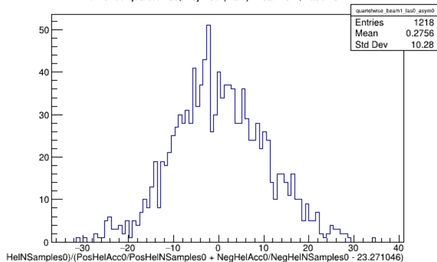
Run 5469 quartetwise, Asyms0 (Raw): Beam ON, Laser OFF
