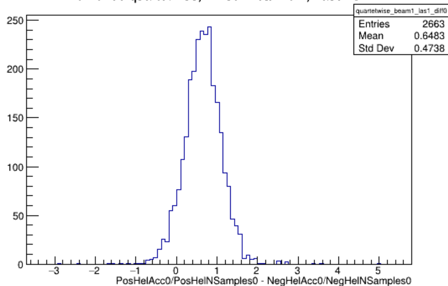
Run 5469 quartetwise, Diffs0: Beam ON, Laser ON
