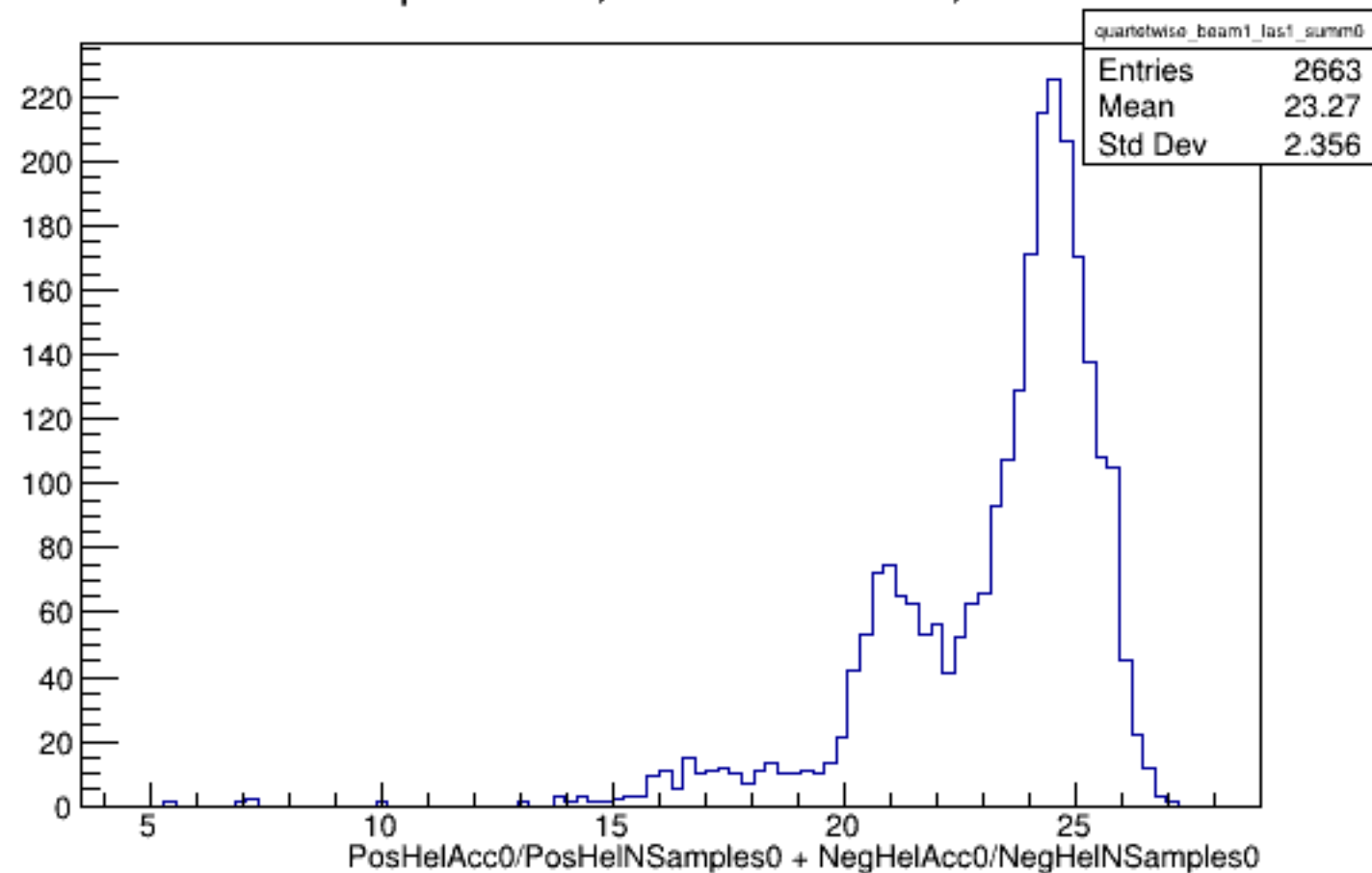
Run 5469 quartetwise, Sums0: Beam ON, Laser ON
