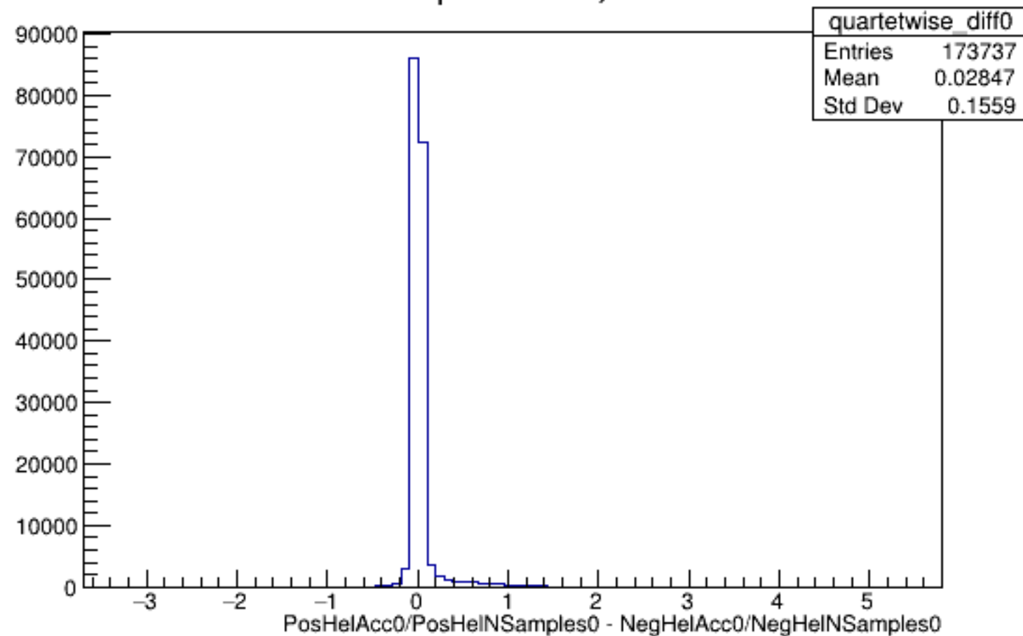
Run 5469 quartetwise, Diffs0: All
