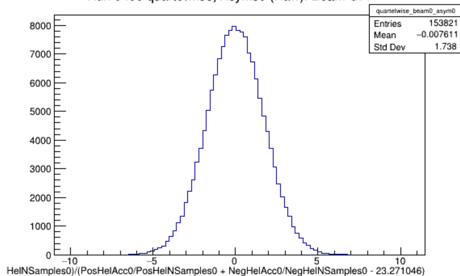
Run 5469 quartetwise, Asyms0 (Raw): Beam OFF
