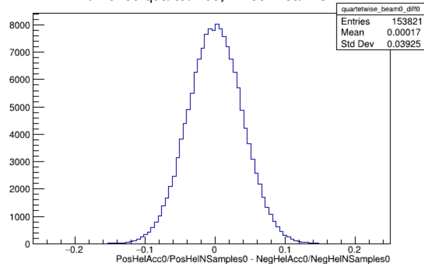
Run 5469 quartetwise, Diffs0: Beam OFF
