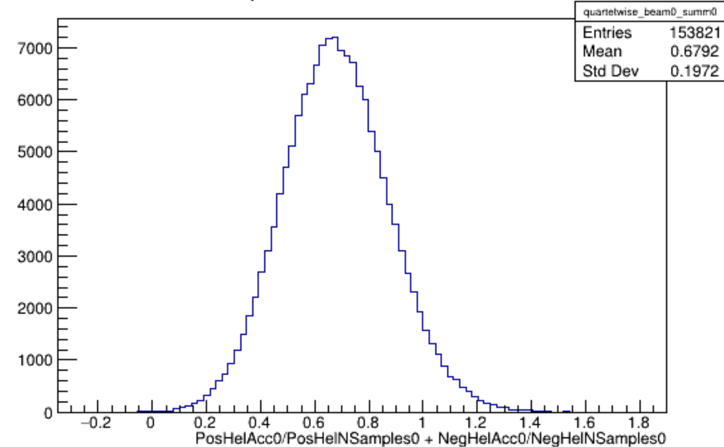
Run 5469 quartetwise, Sums0: Beam OFF
