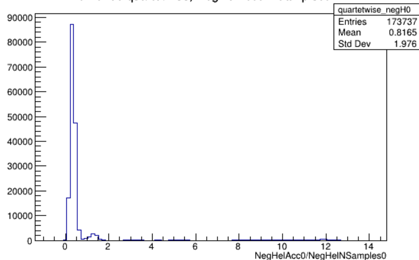
Run 5469 quartetwise, NegHelAcc0/NSamples0: All
