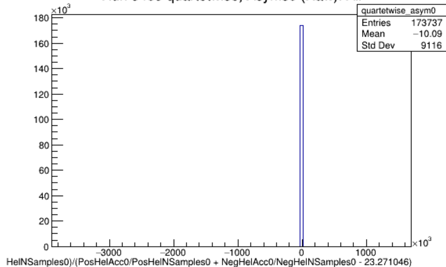
Run 5469 quartetwise, Asyms0 (Raw): All
