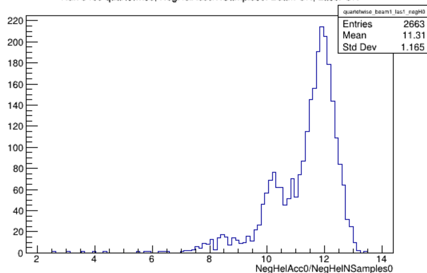
Run 5469 quartetwise, NegHelAcc0/NSamples0: Beam ON, Laser ON
