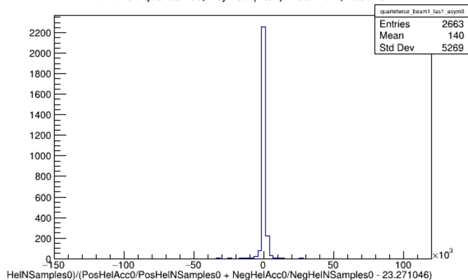
Run 5469 quartetwise, Asyms0 (Raw): Beam ON, Laser ON
