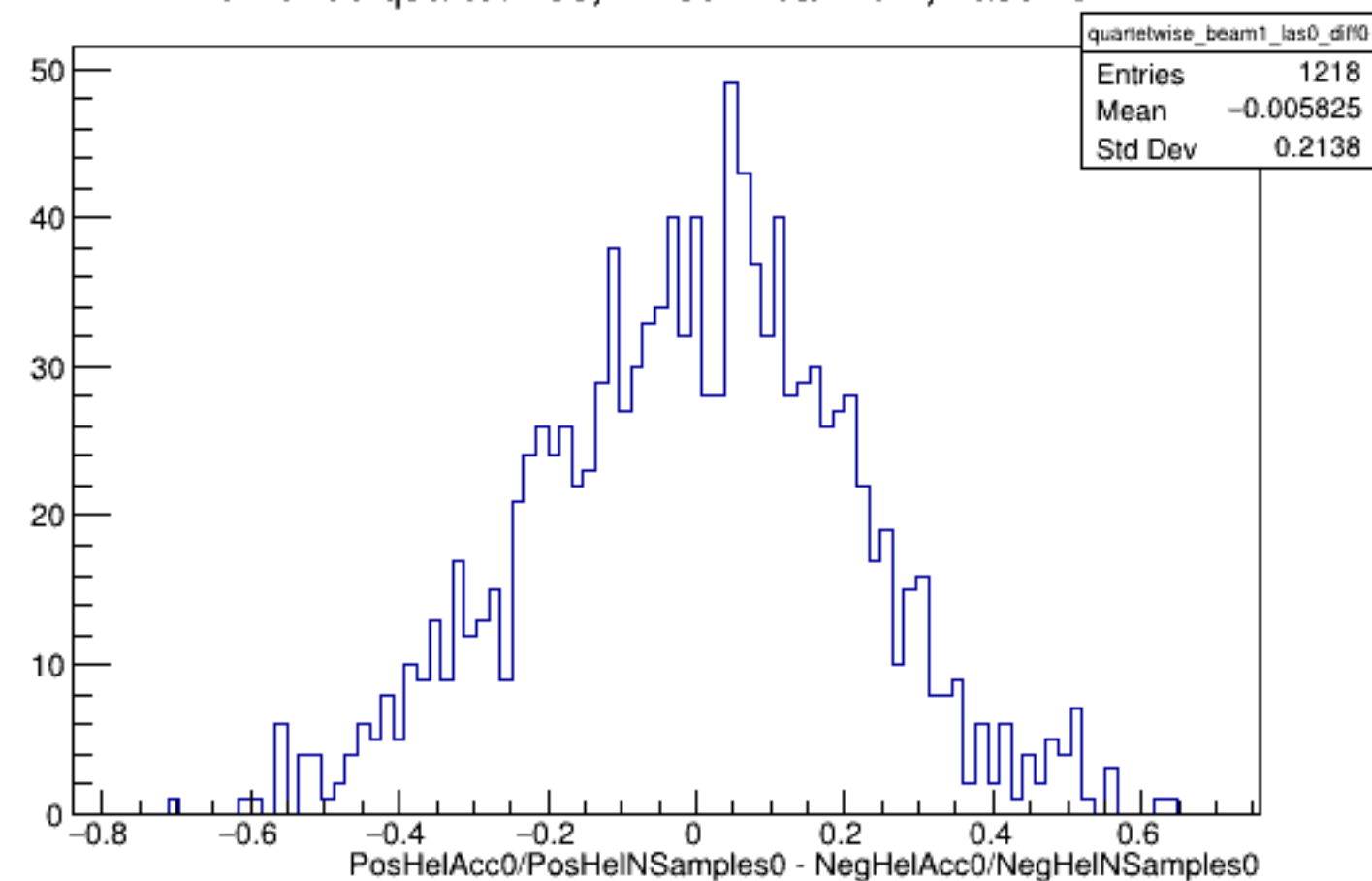
Run 5469 quartetwise, Diffs0: Beam ON, Laser OFF
