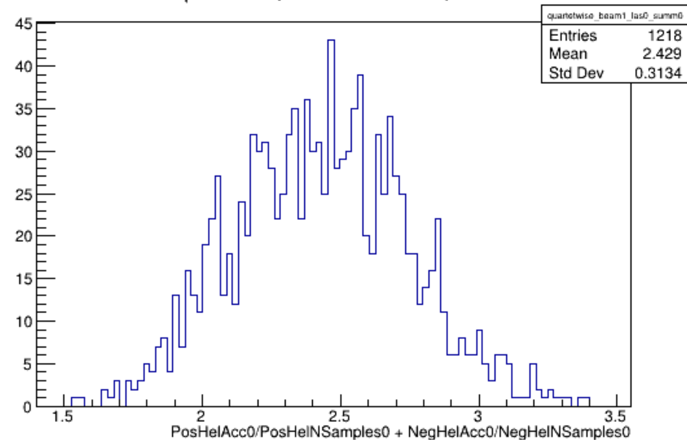
Run 5469 quartetwise, Sums0: Beam ON, Laser OFF
