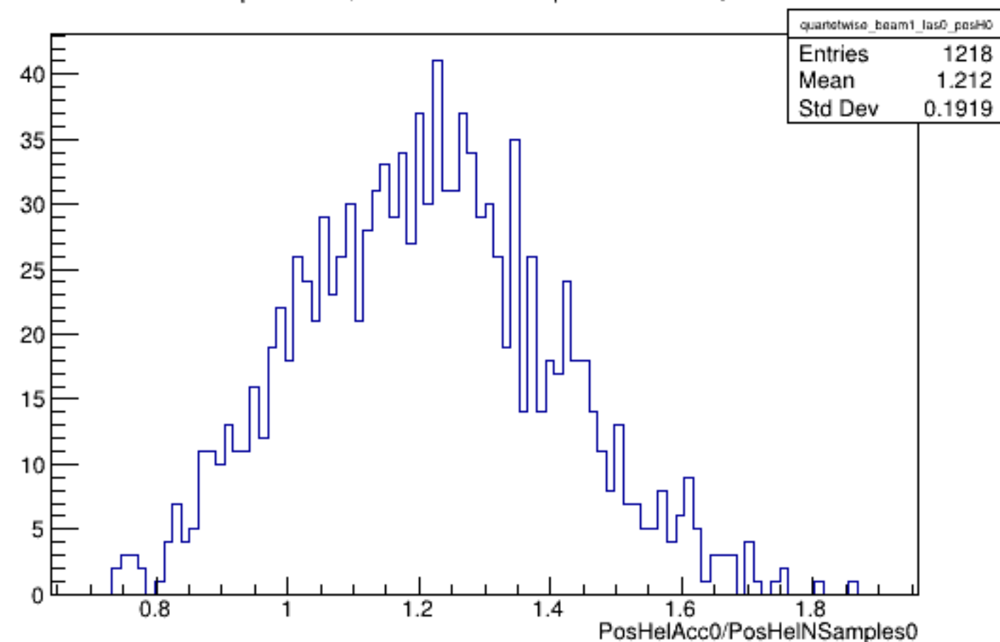
Run 5469 quartetwise, PosHelAcc0/NSamples0: Beam ON, Laser OFF
