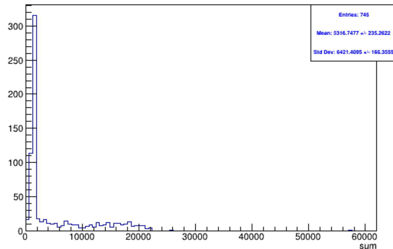
Run 5469 triggerwise, sums: Beam OFF
