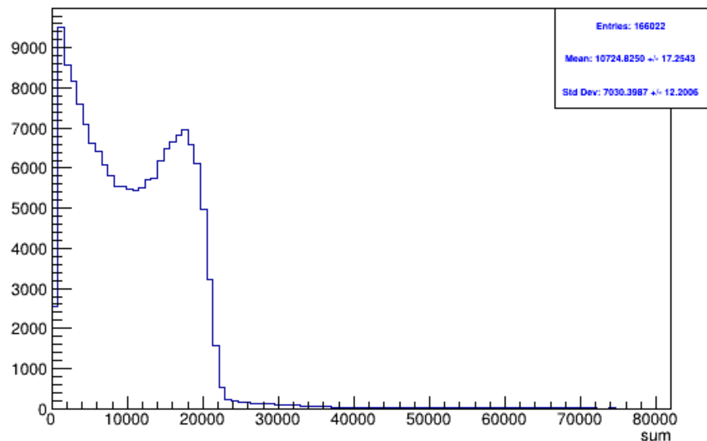
Run 5469 triggerwise, sums: All
