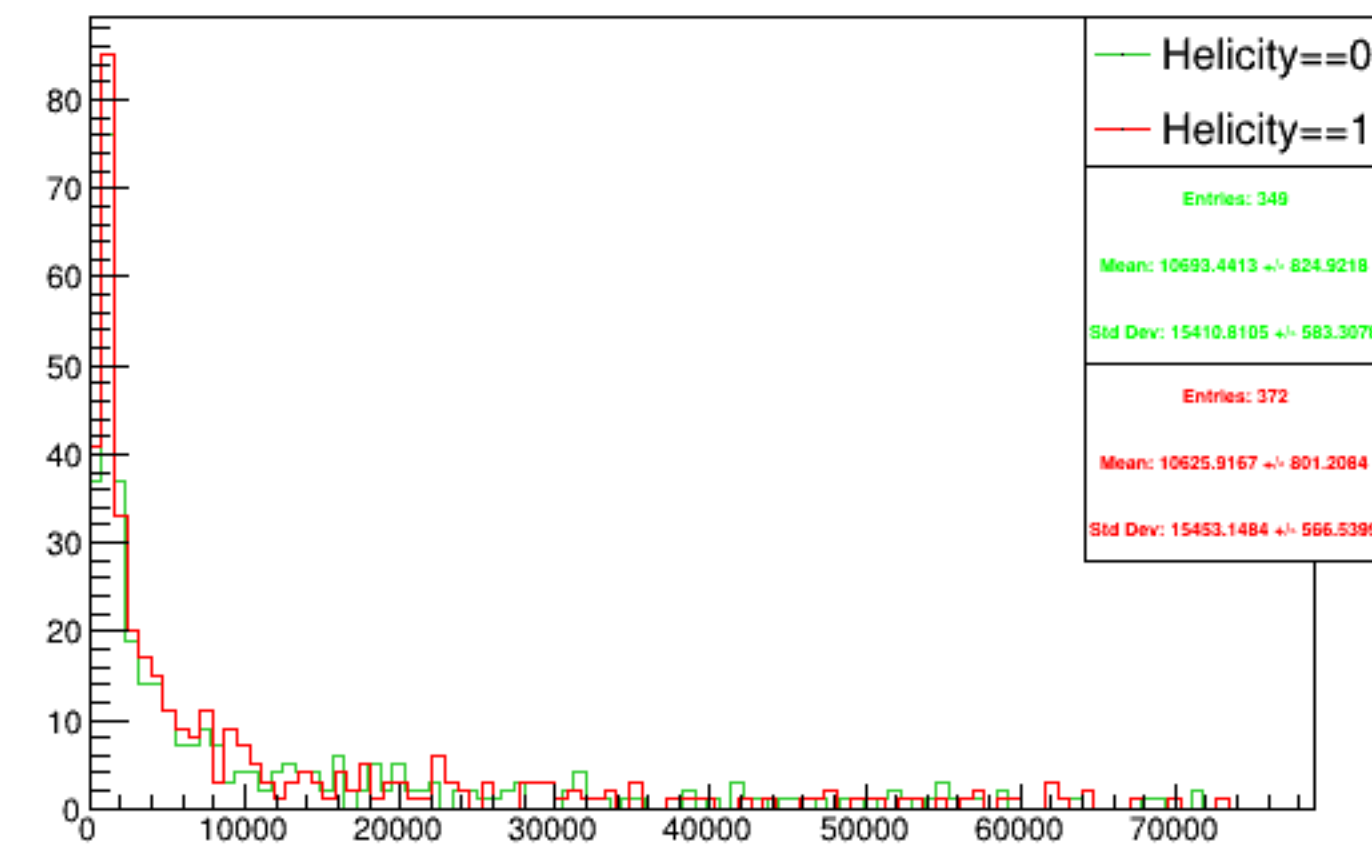
Run 5469 triggerwise, sums: Beam ON, Laser OFF
