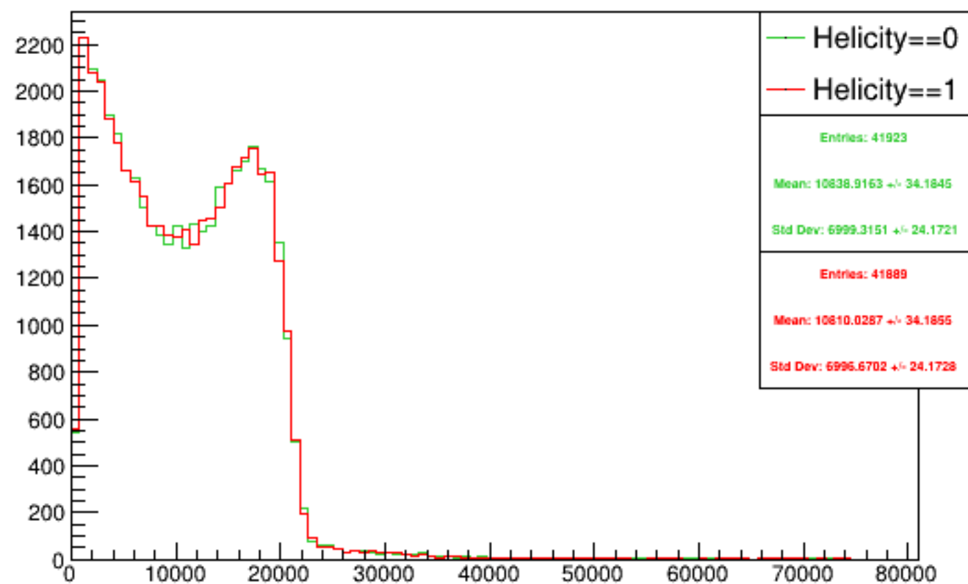
Run 5469 triggerwise, sums: Beam ON, Laser ON
