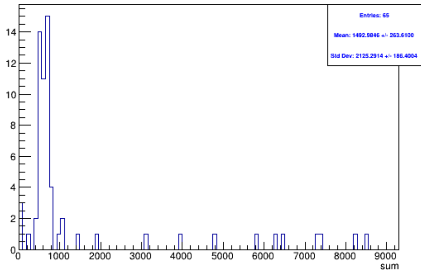
Run 5482 triggerwise, sums: All
