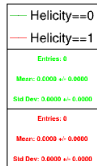
Run 5482 triggerwise, sums: Beam ON, Laser OFF
