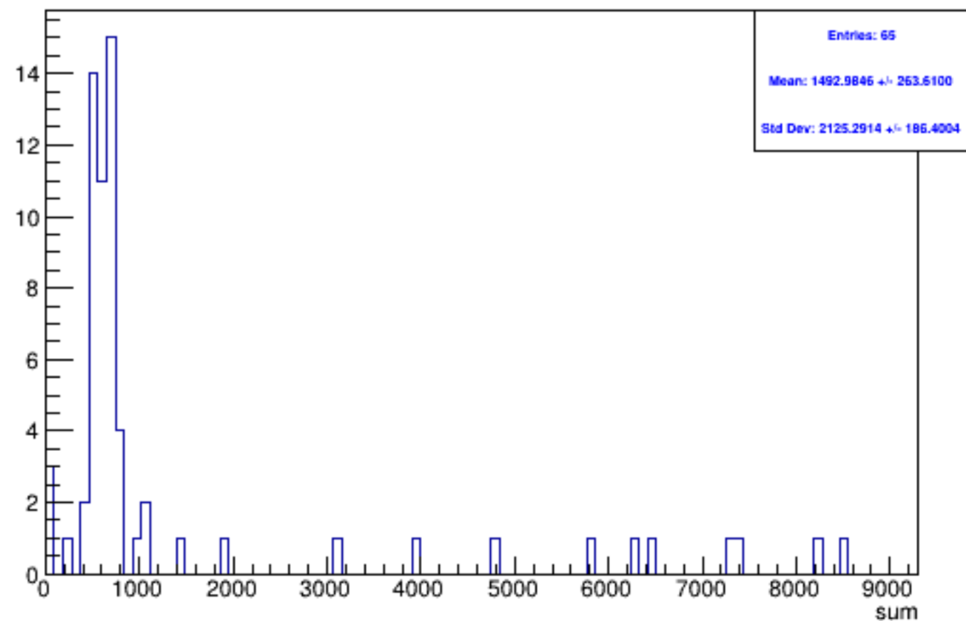
Run 5482 triggerwise, sums: Beam OFF
