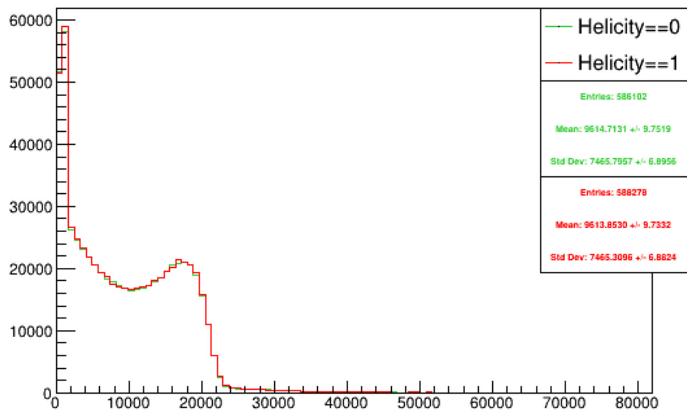
Run 5497 triggerwise, sums: Beam ON, Laser ON
