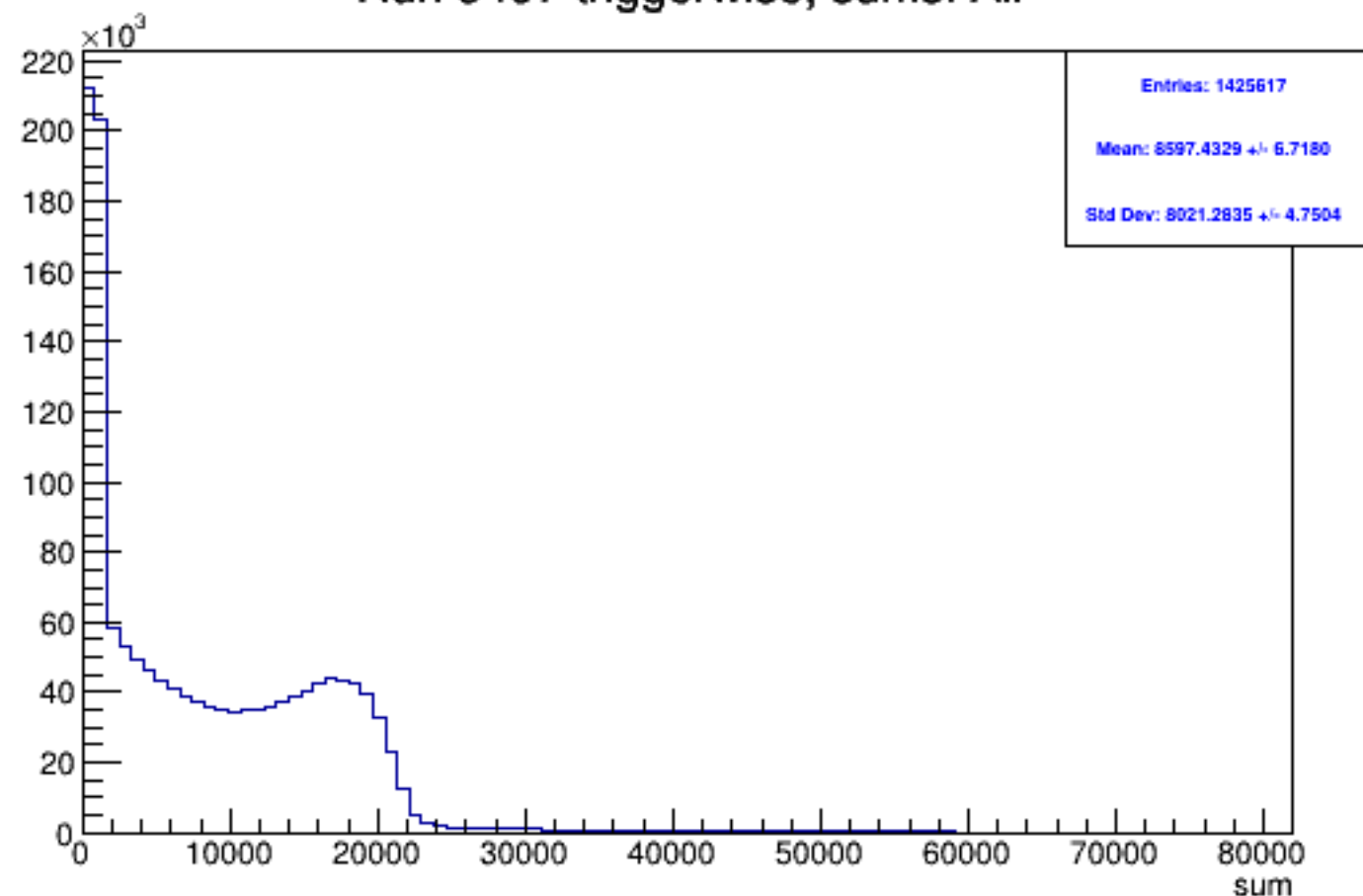
Run 5497 triggerwise, sums: All
