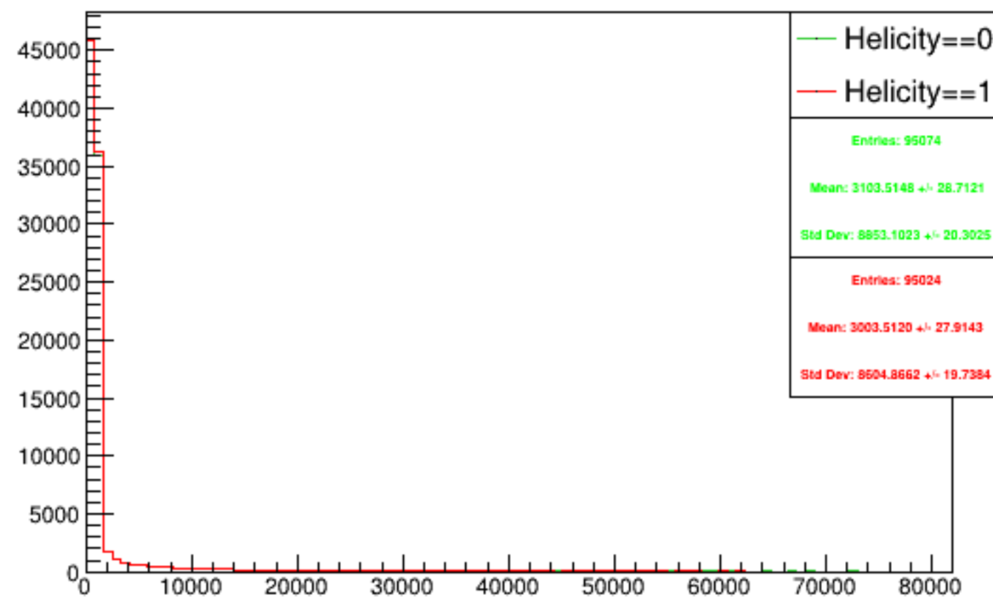
Run 5497 triggerwise, sums: Beam ON, Laser OFF
