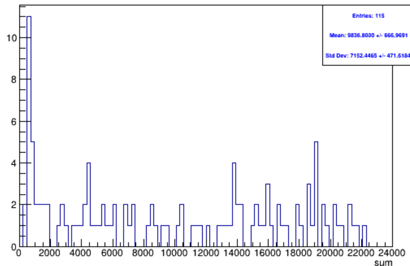
Run 5497 triggerwise, sums: Beam OFF
