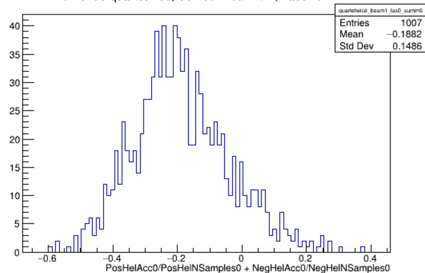
Run 5498 quartetwise, Sums0: Beam ON, Laser OFF
