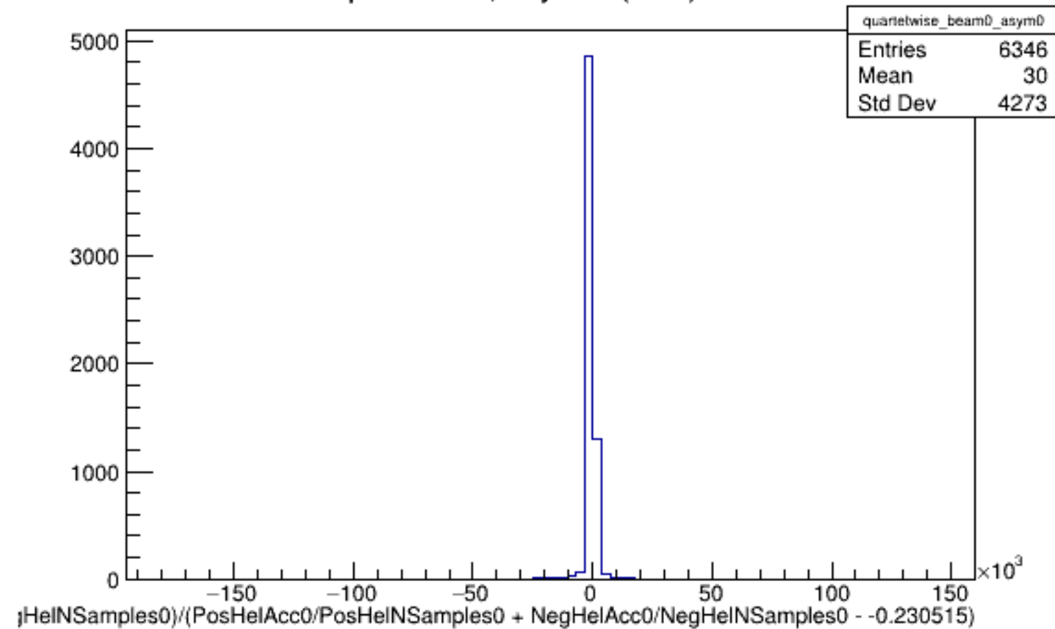
Run 5498 quartetwise, Asyms0 (Raw): Beam OFF
