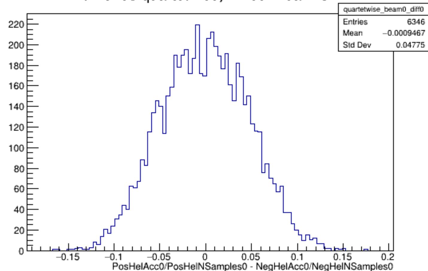
Run 5498 quartetwise, Diffs0: Beam OFF
