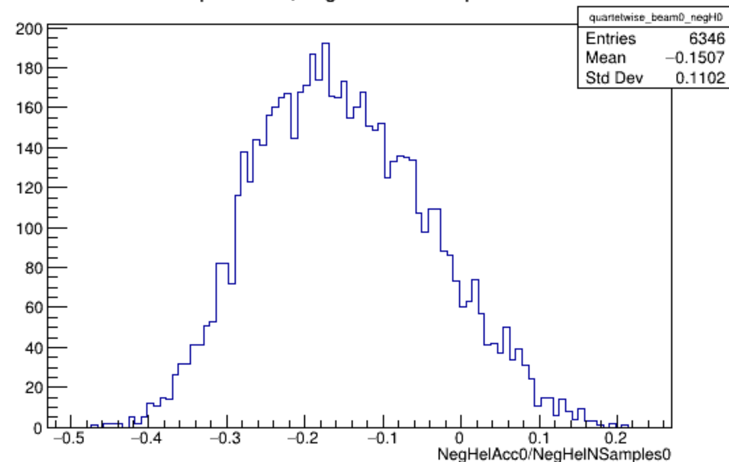
Run 5498 quartetwise, NegHelAcc0/NSamples0: Beam OFF
