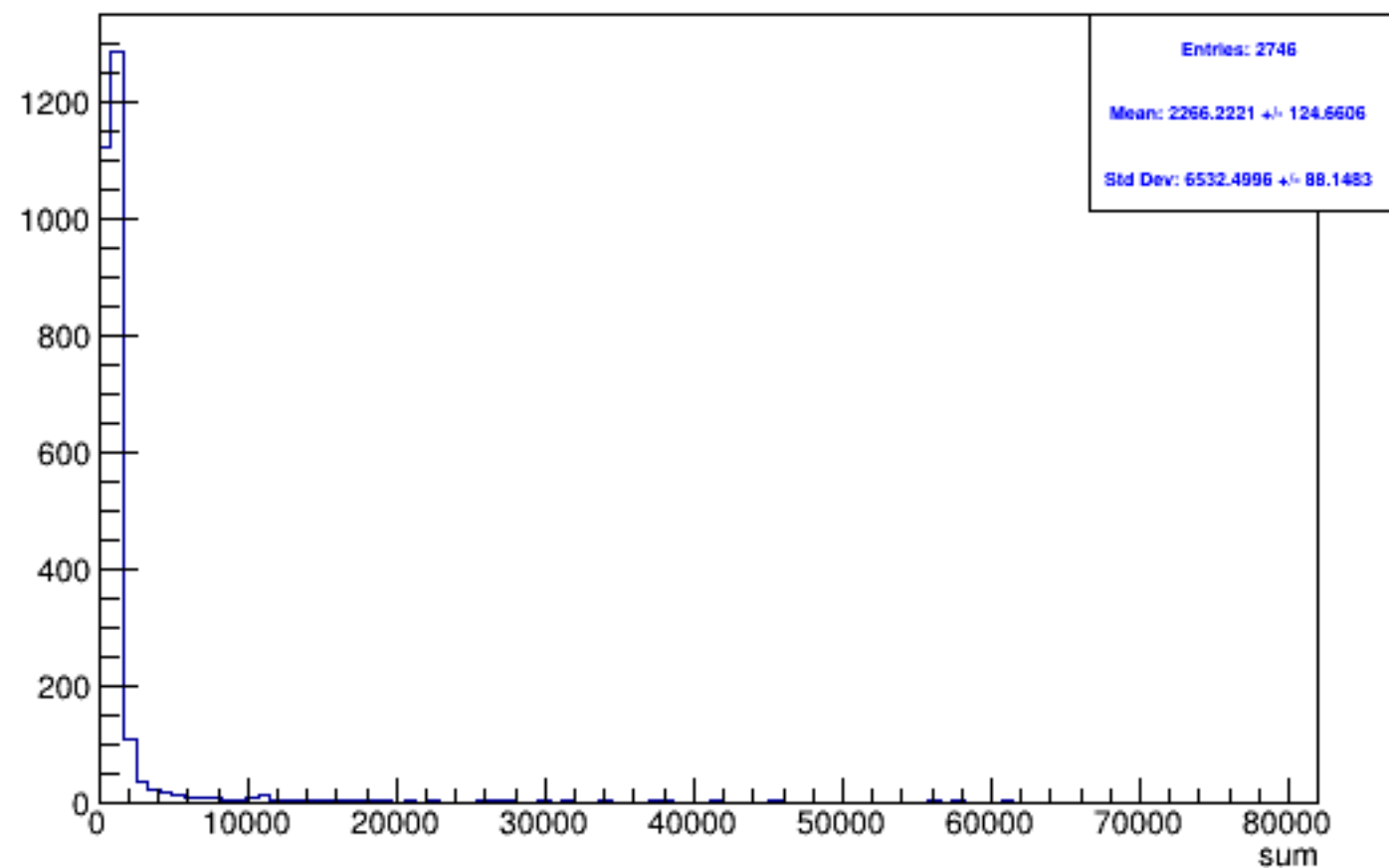
Run 5498 triggerwise, sums: All
