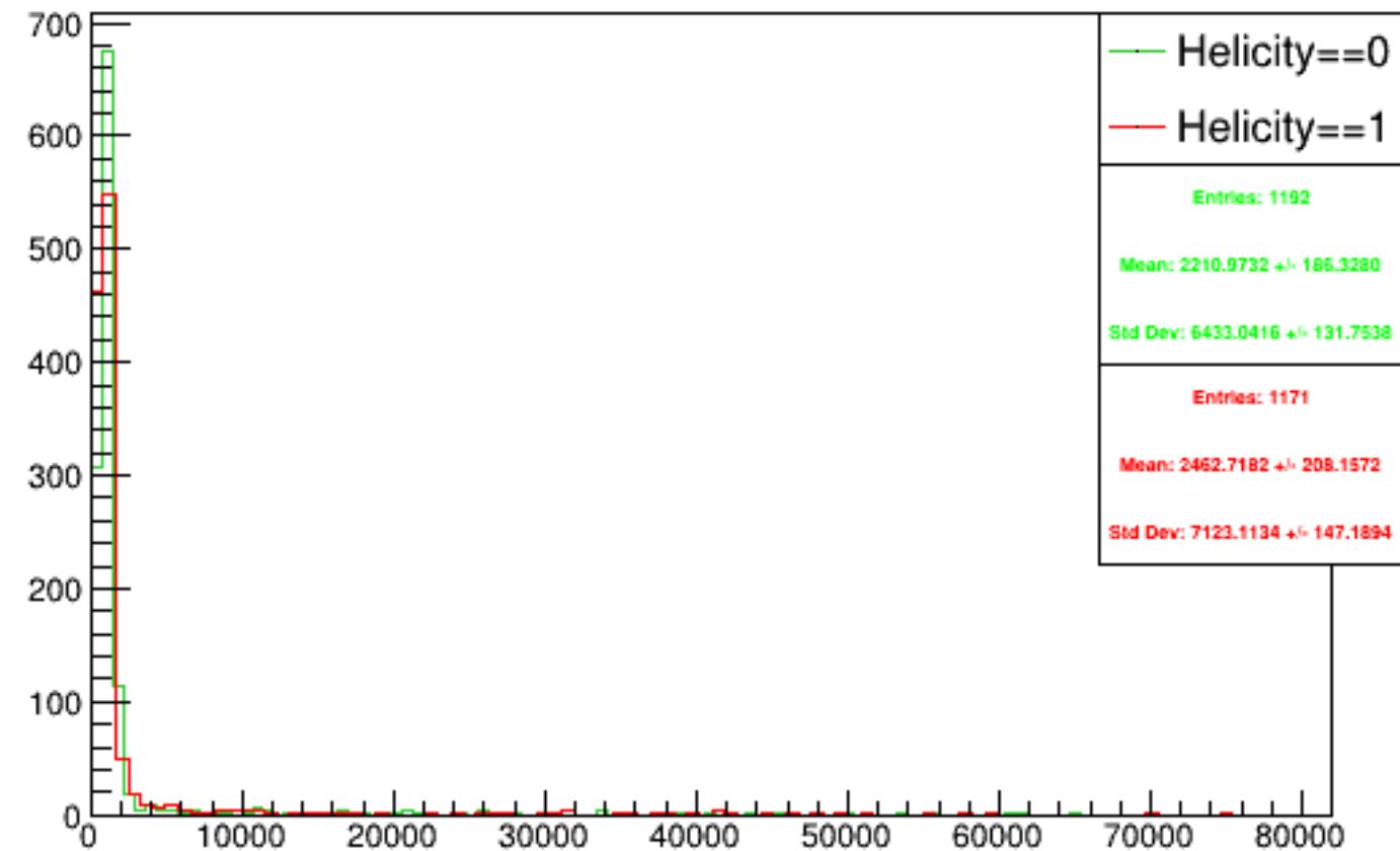
Run 5498 triggerwise, sums: Beam ON, Laser OFF
