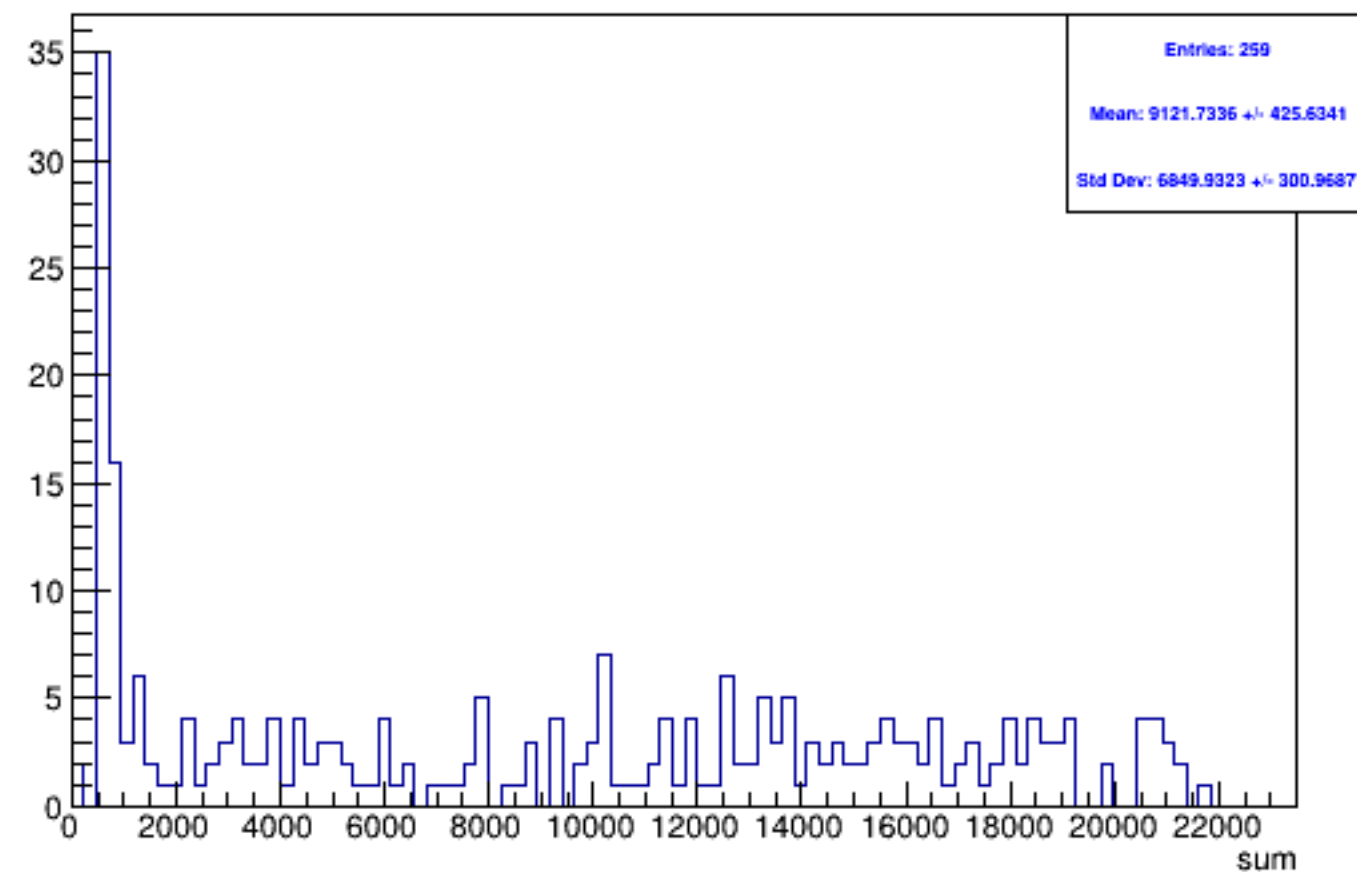
Run 5500 triggerwise, sums: Beam OFF
