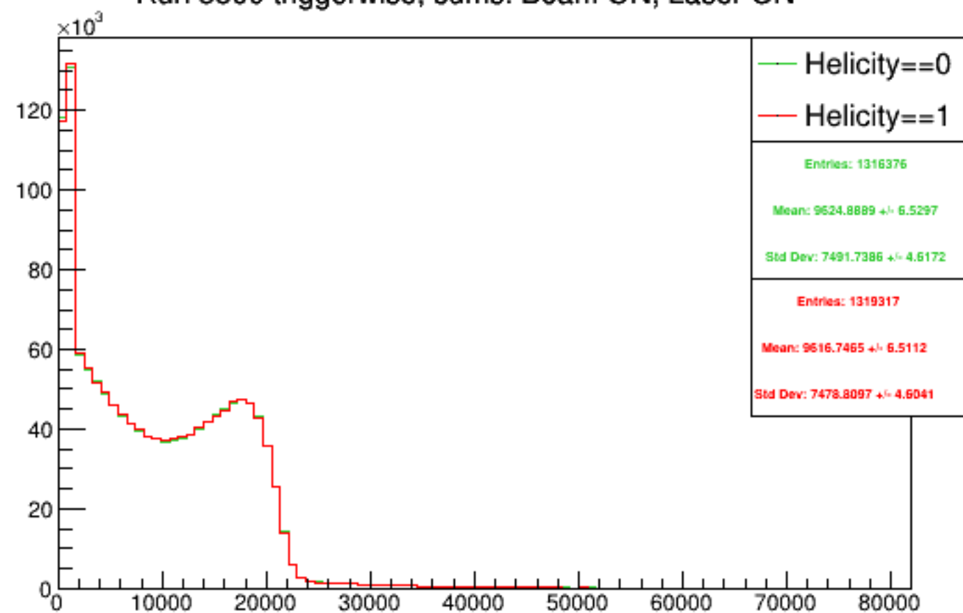
Run 5500 triggerwise, sums: Beam ON, Laser ON
