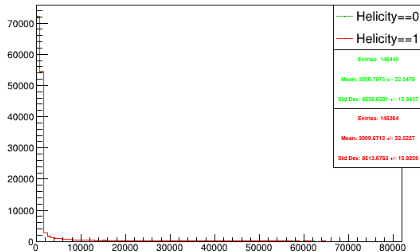
Run 5500 triggerwise, sums: Beam ON, Laser OFF
