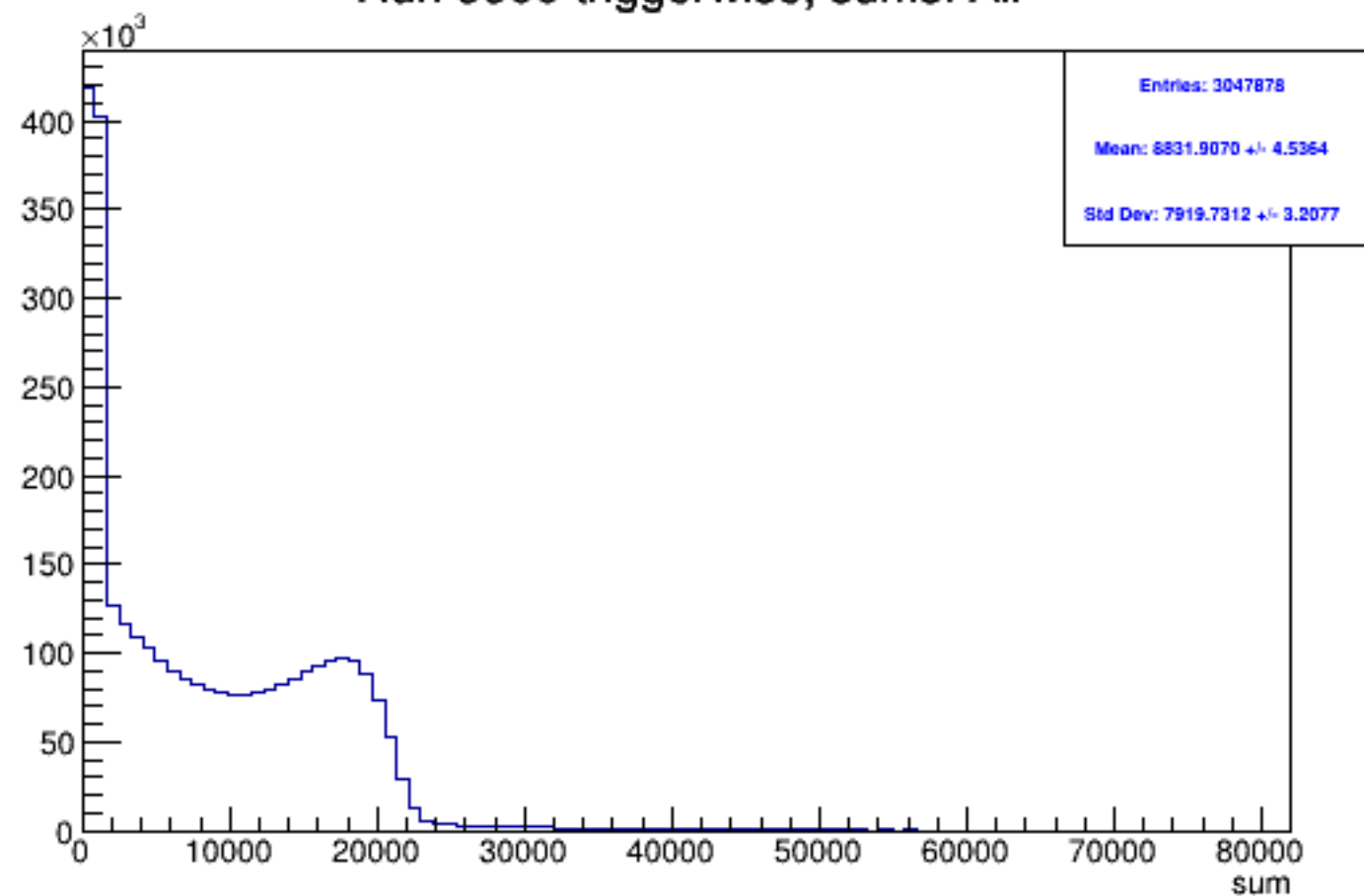
Run 5500 triggerwise, sums: All
