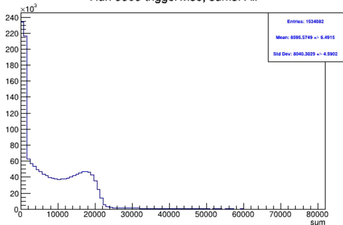
Run 5505 triggerwise, sums: All
