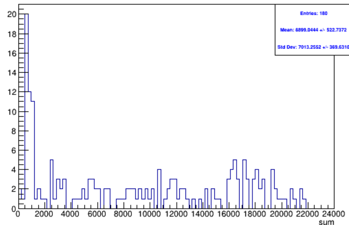
Run 5505 triggerwise, sums: Beam OFF
