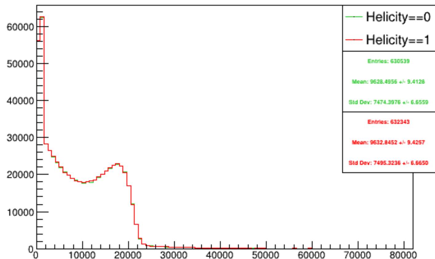
Run 5505 triggerwise, sums: Beam ON, Laser ON
