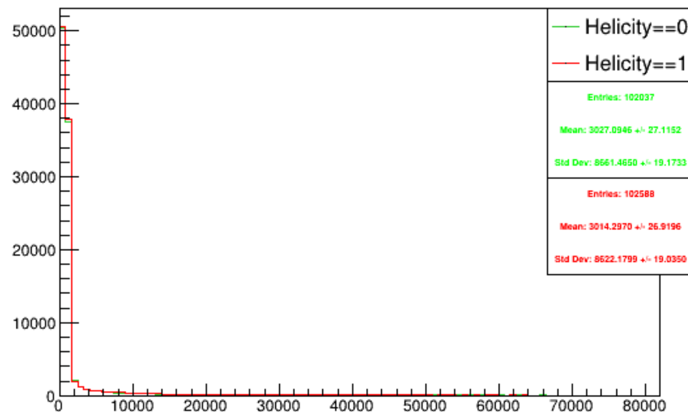
Run 5505 triggerwise, sums: Beam ON, Laser OFF
