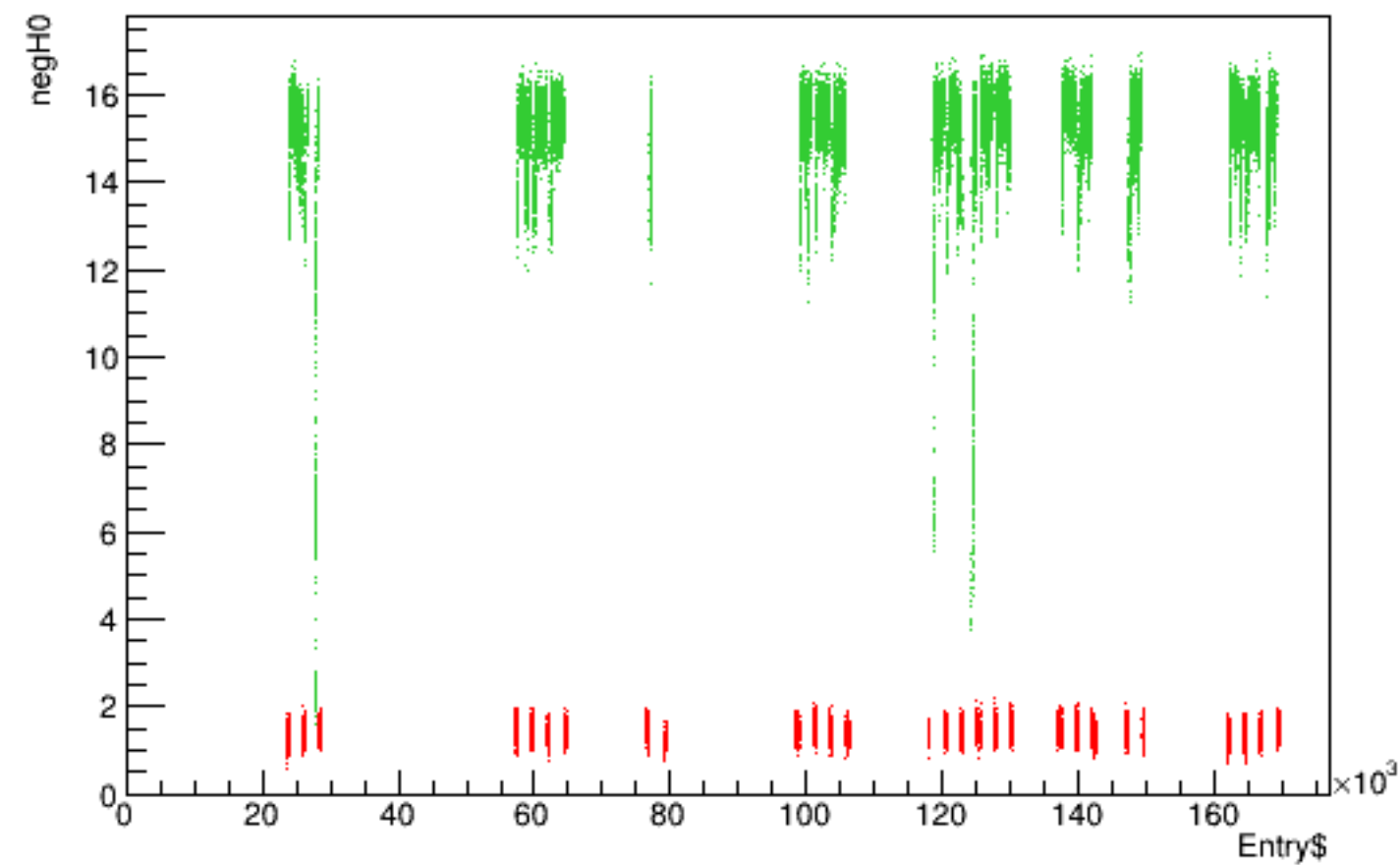
Run 5511 quartetwise, negH0 vs time
