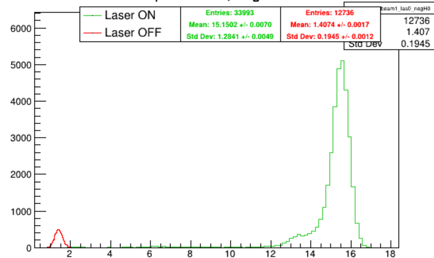
Run 5511 quartetwise, negH0: Beam ON
