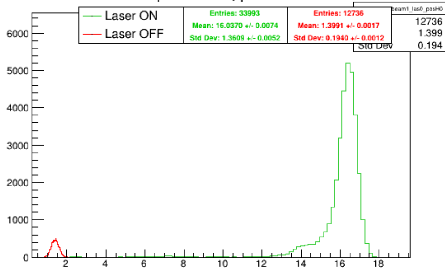
Run 5511 quartetwise, posH0: Beam ON
