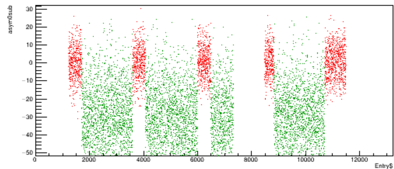
Run 5518 quartetwise, asym0sub vs time
