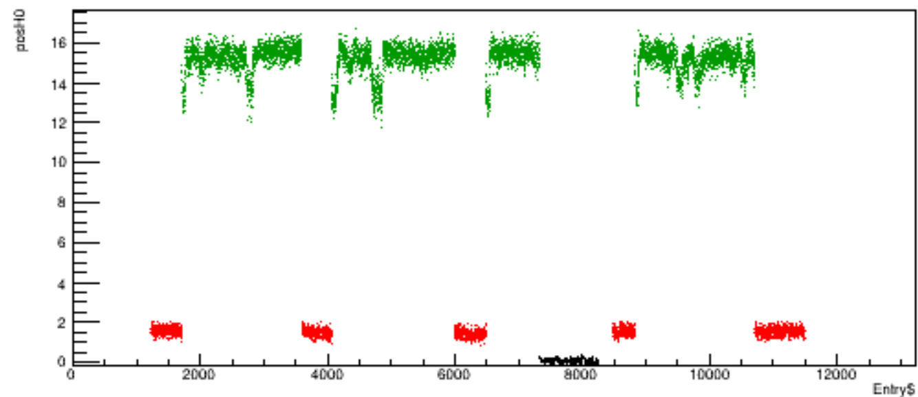
Run 5518 quartetwise, posH0 vs time
