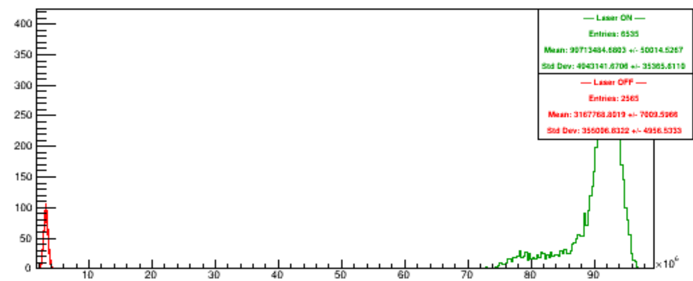
Run 5518 quartetwise, Sums4
