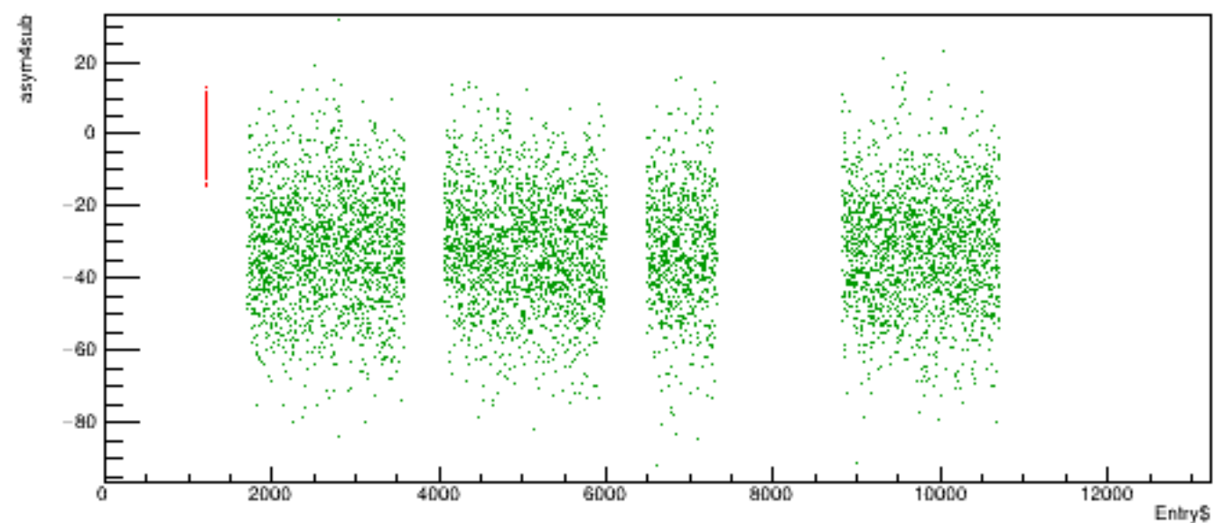
Run 5518 quartetwise, asym4sub vs time
