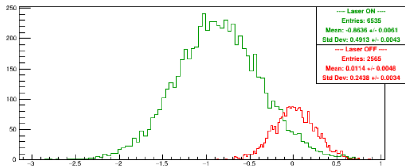
Run 5518 quartetwise, Diffs0
