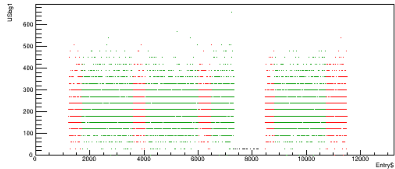
Run 5518 quartetwise, USbg1 vs time
