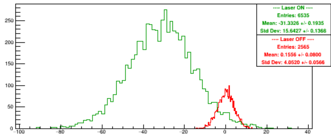
Run 5518 quartetwise, Asyms4
