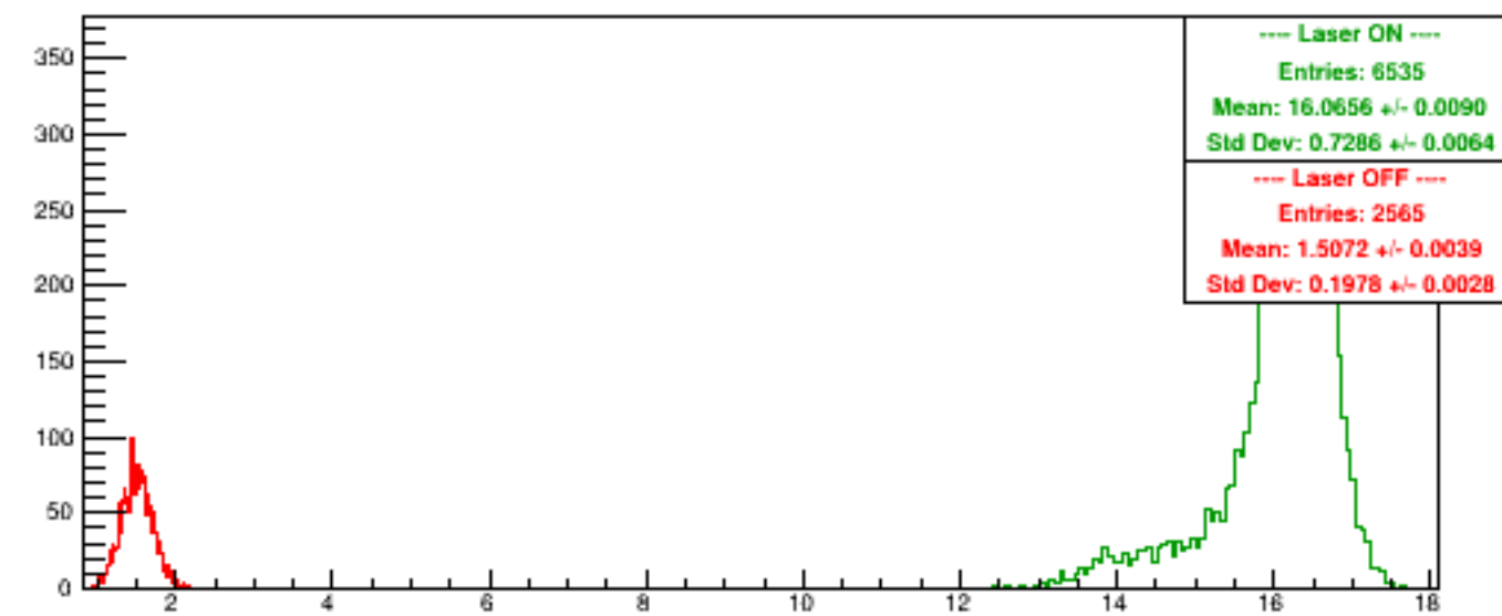
Run 5518 quartetwise, NegHelAcc0/NSamples0
