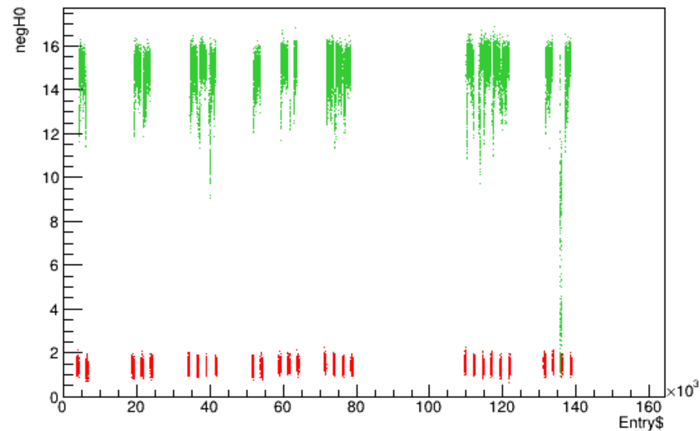
Run 5524 quartetwise, negH0 vs time
