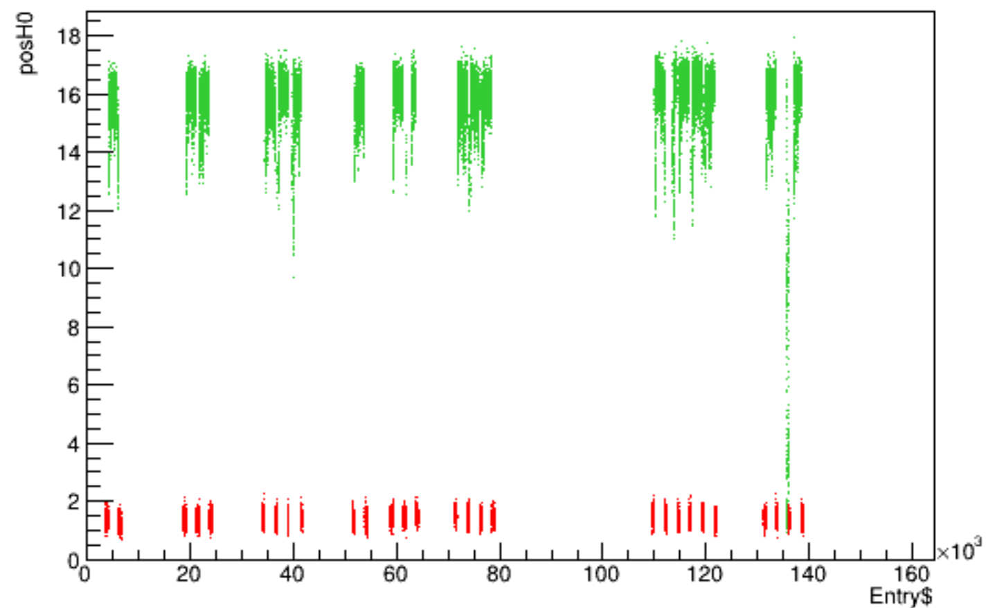
Run 5524 quartetwise, posH0 vs time
