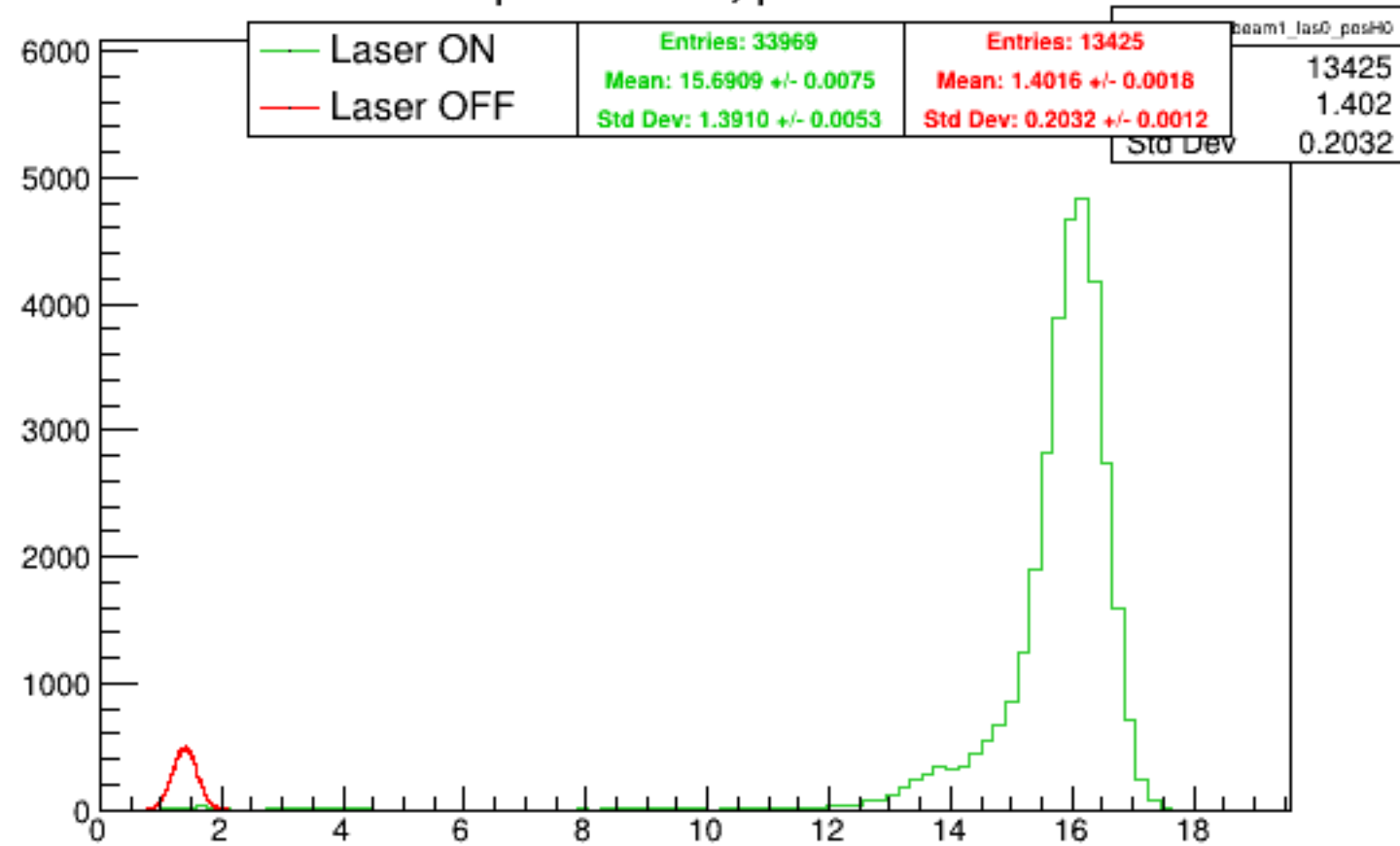
Run 5524 quartetwise, posH0: Beam ON
