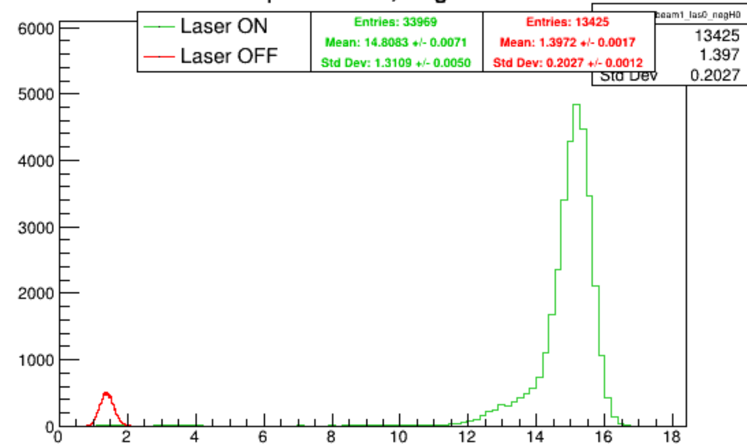
Run 5524 quartetwise, negH0: Beam ON
