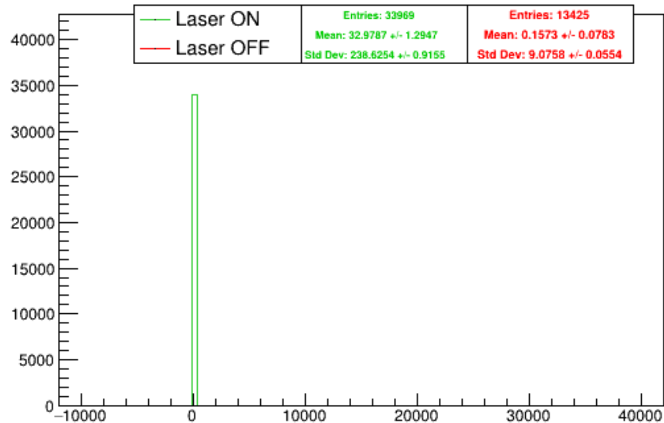
Run 5524 quartetwise, asym0sub: Beam ON
