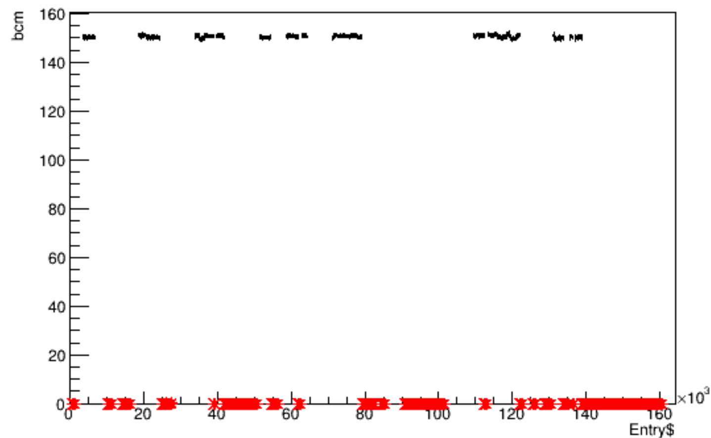
Run 5524 quartetwise, bcm vs time
