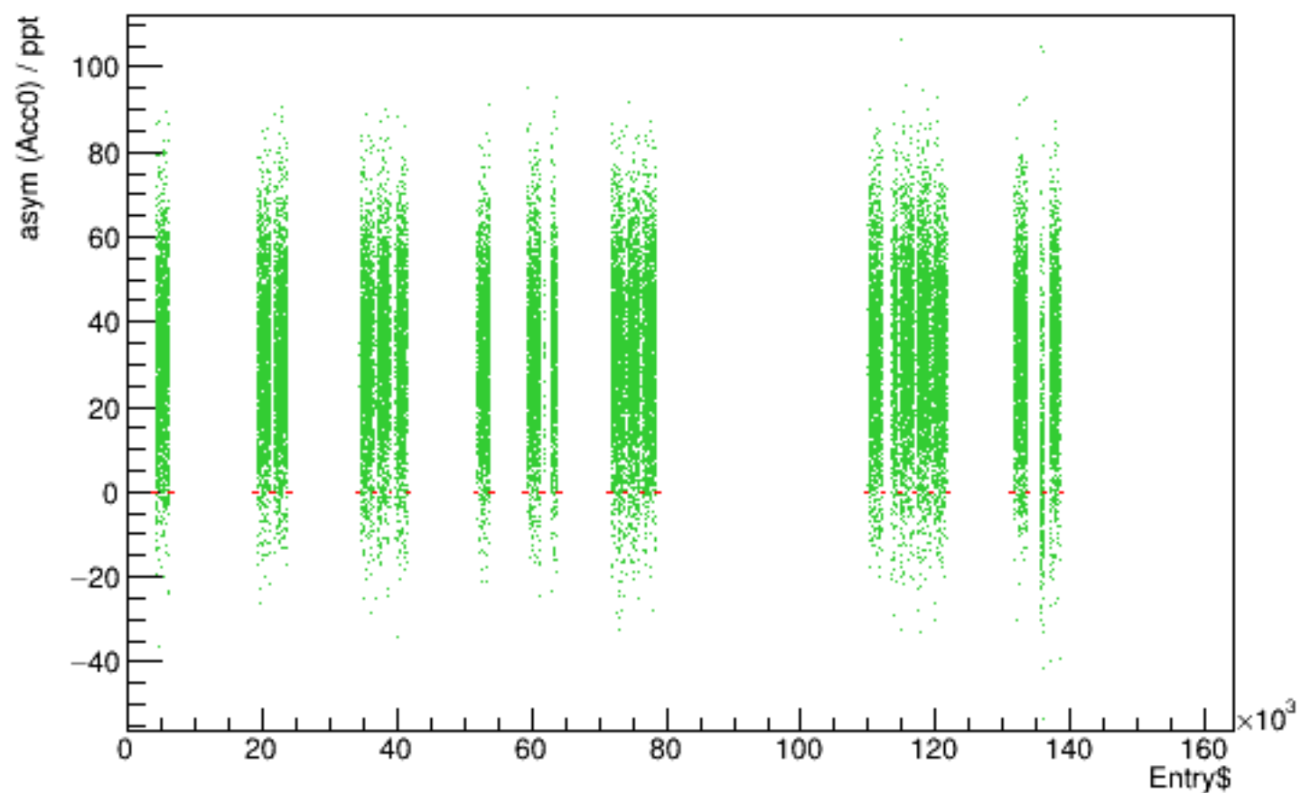
Run 5524 quartetwise, asym0sub vs time
