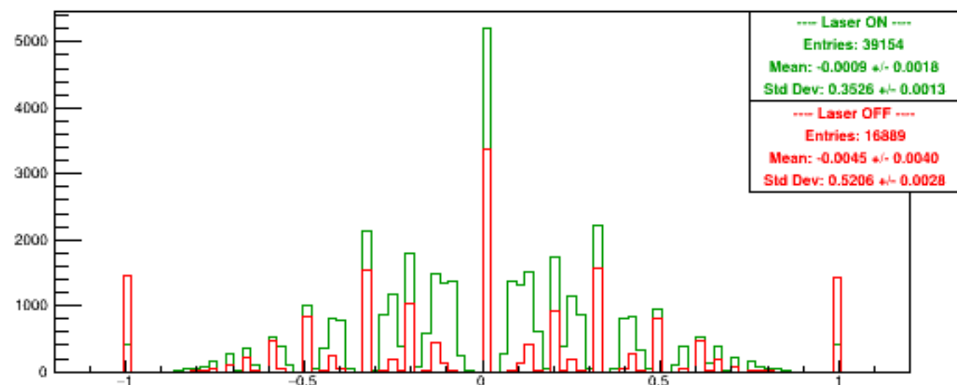
Run 5531 quartetwise, Asyms Horiz Finger
