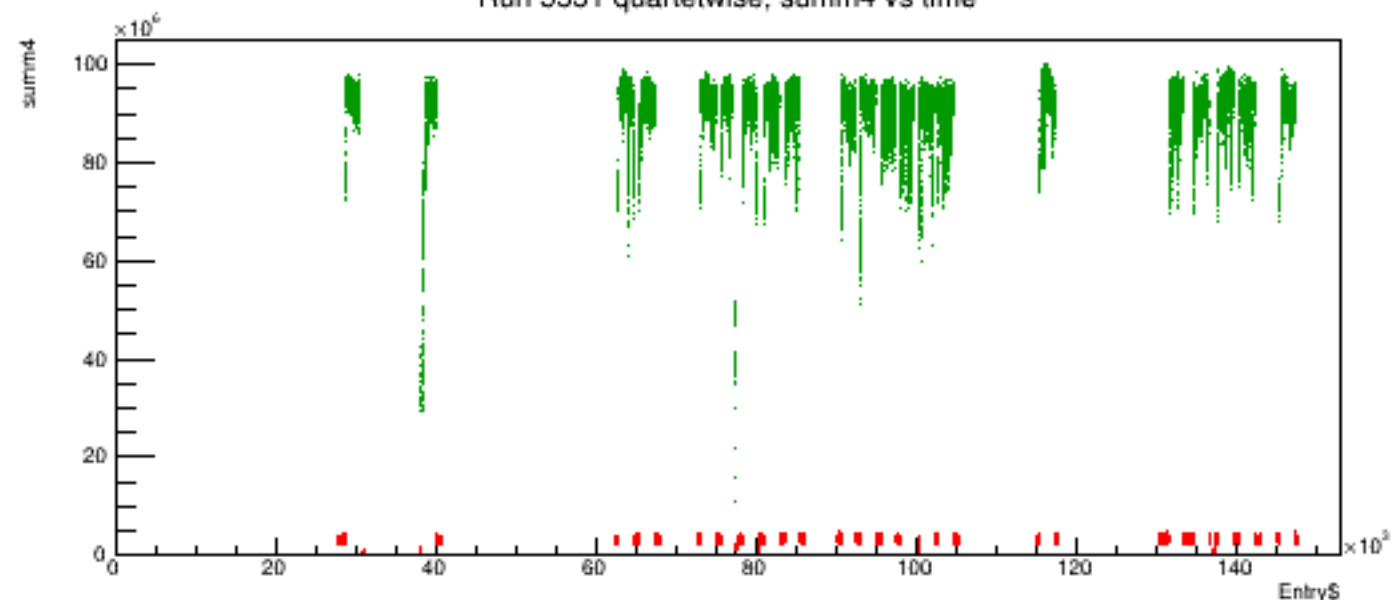
Run 5531 quartetwise, summ4 vs time
