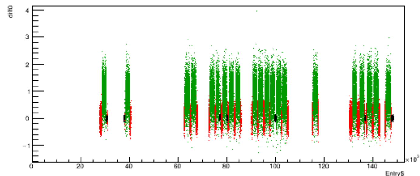
Run 5531 quartetwise, diff0 vs time
