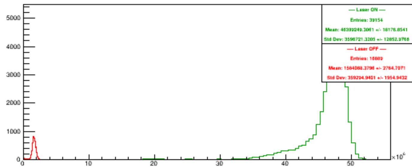
Run 5531 quartetwise, PosHelAcc4
