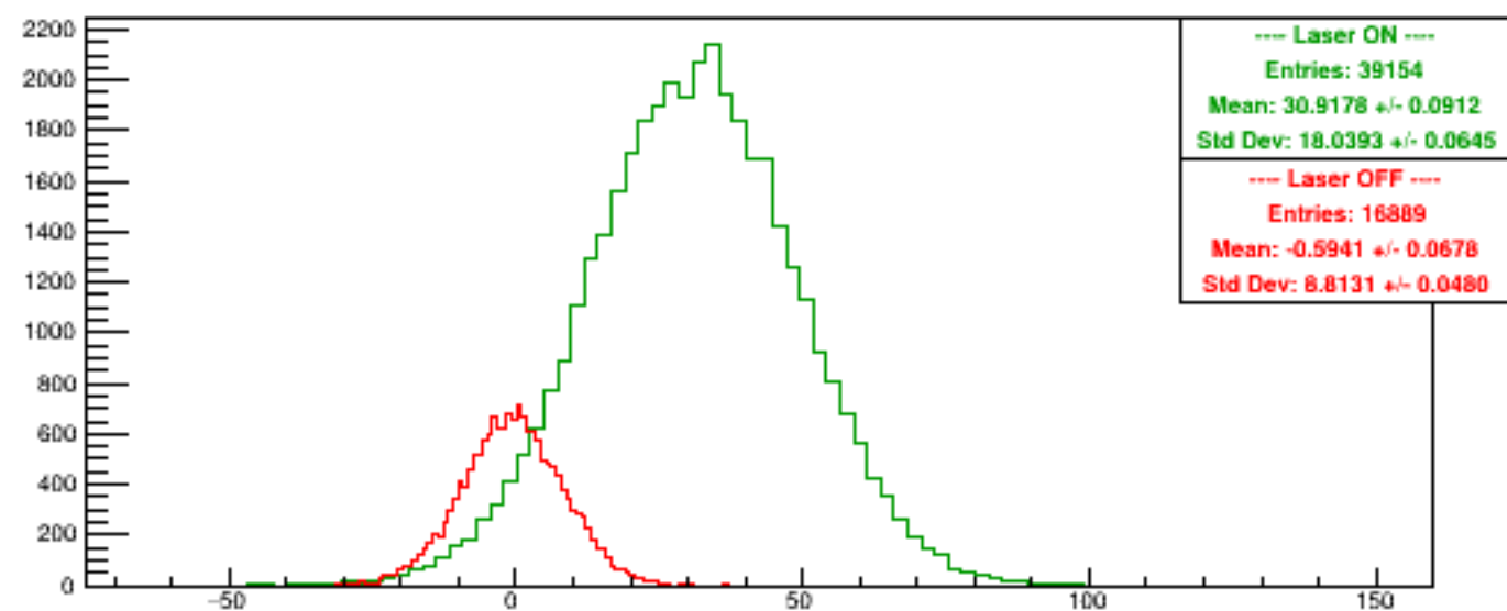
Run 5531 quartetwise, Asyms0
