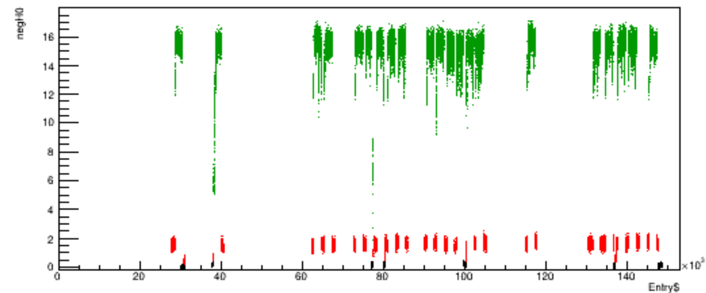
Run 5531 quartetwise, negH0 vs time
