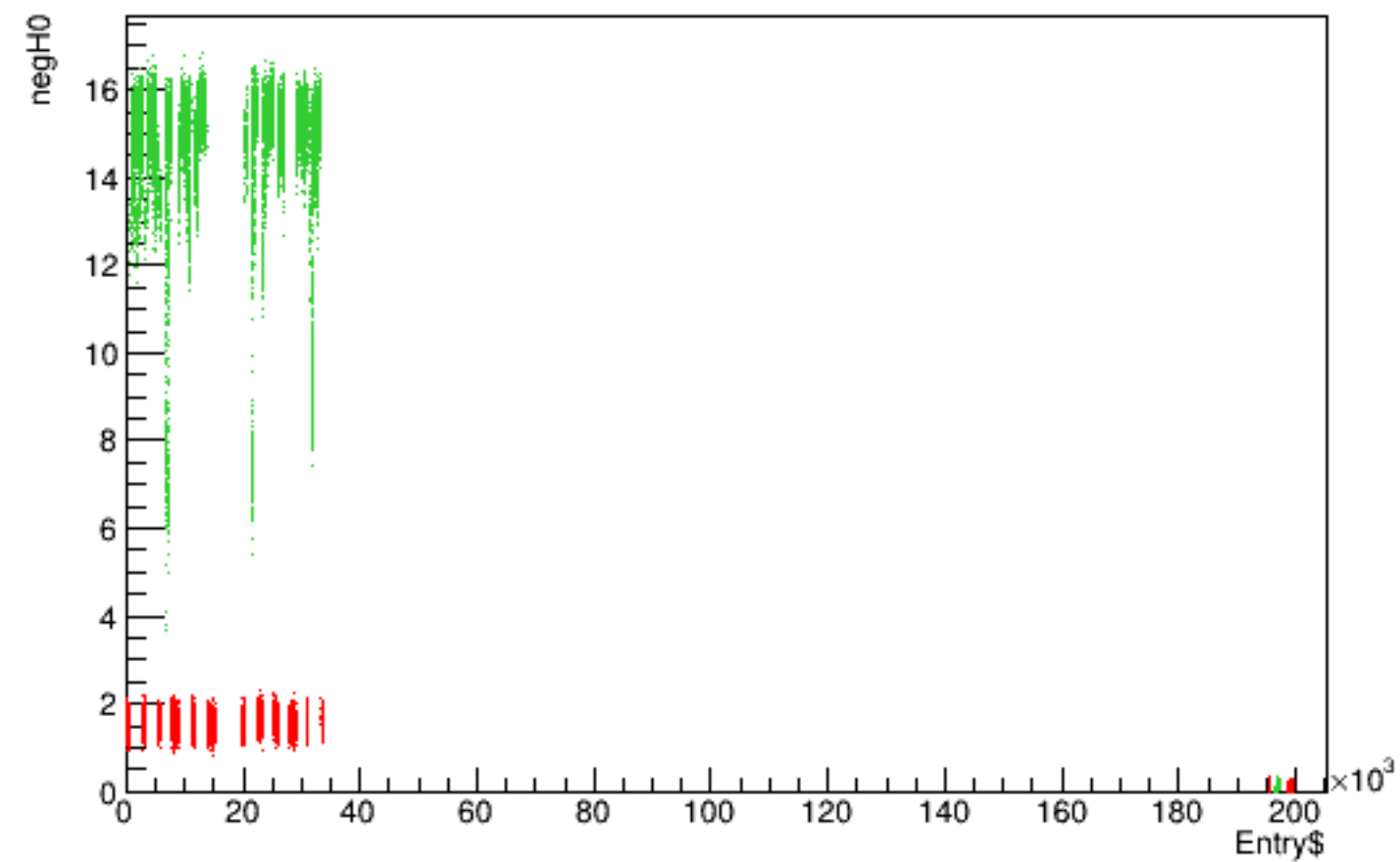
Run 5536 quartetwise, negH0 vs time
