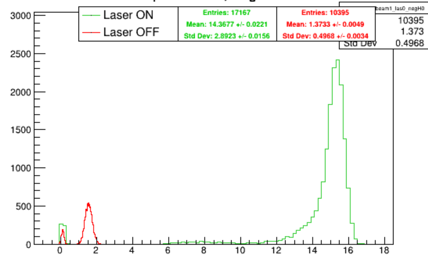
Run 5536 quartetwise, negH0: Beam ON
