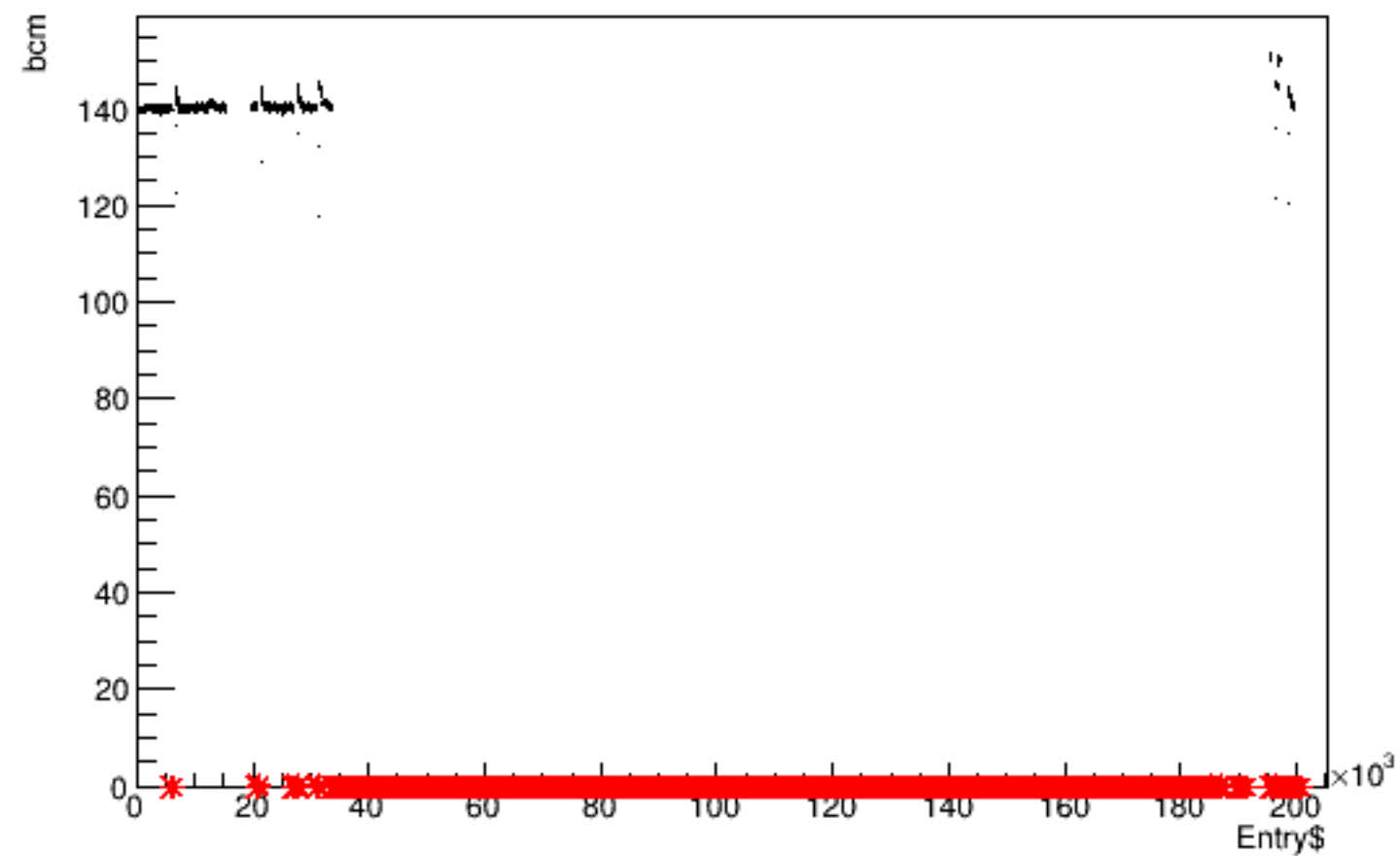
Run 5536 quartetwise, bcm vs time
