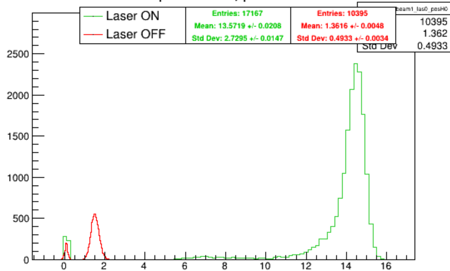
Run 5536 quartetwise, posH0: Beam ON
