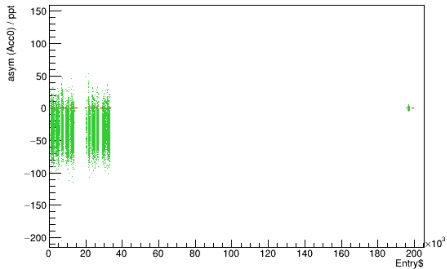
Run 5536 quartetwise, asym0sub vs time
