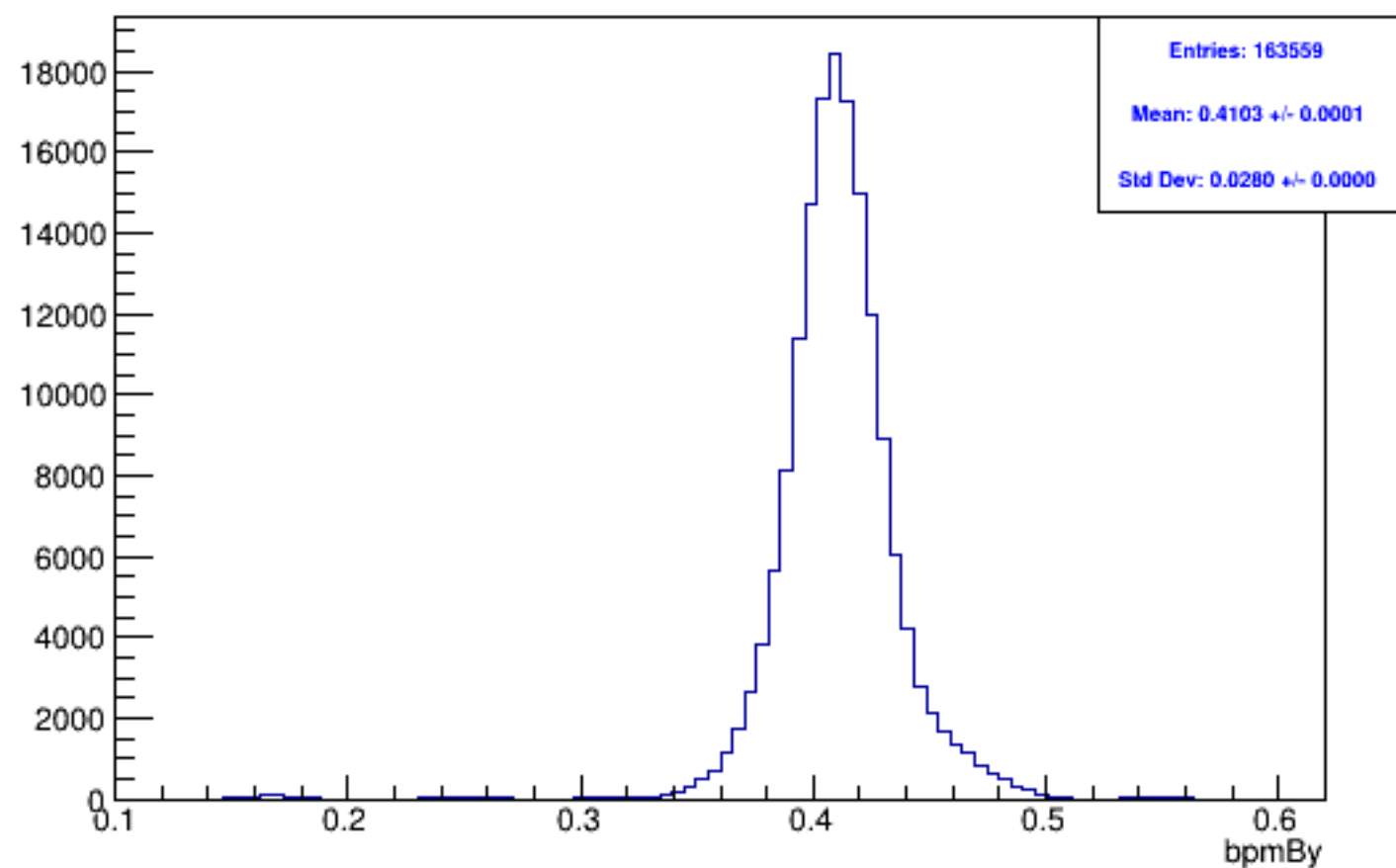
Run 5544, mpswise, bpmBy: Beam ON, Laser ON
