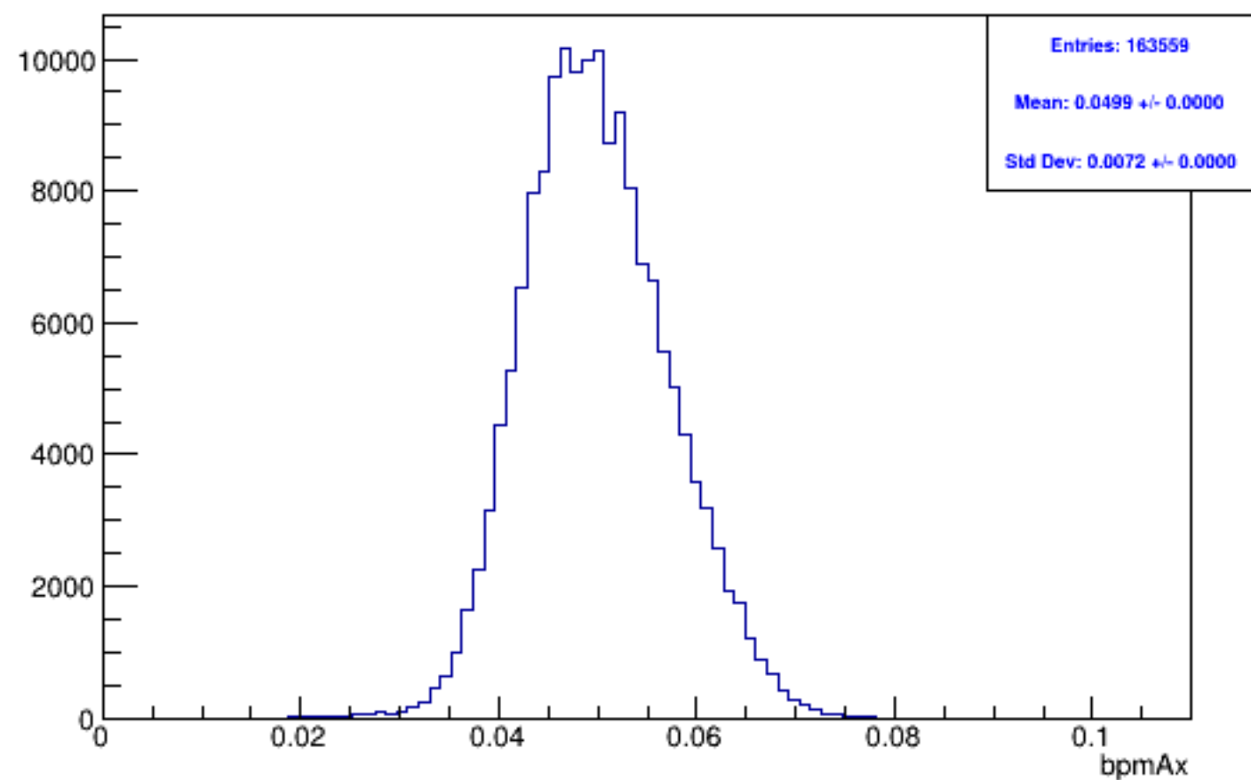
Run 5544, mpswise, bpmAx: Beam ON, Laser ON
