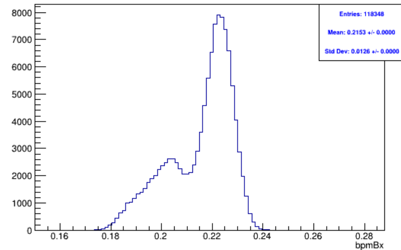
Run 5544, mpswise, bpmBx: Beam ON, Laser OFF
