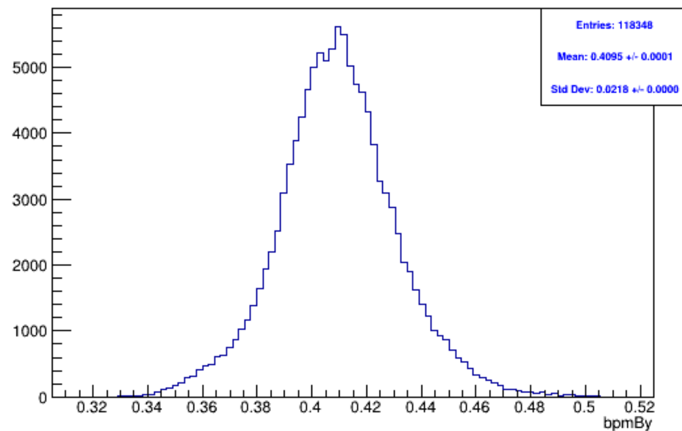
Run 5544, mpswise, bpmBy: Beam ON, Laser OFF
