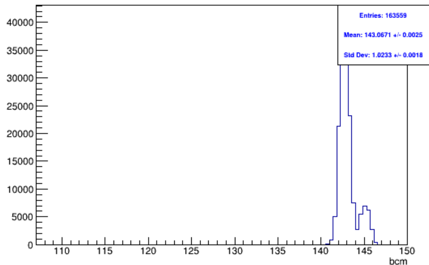
Run 5544, mpwise, BCM: Beam ON, Laser ON
