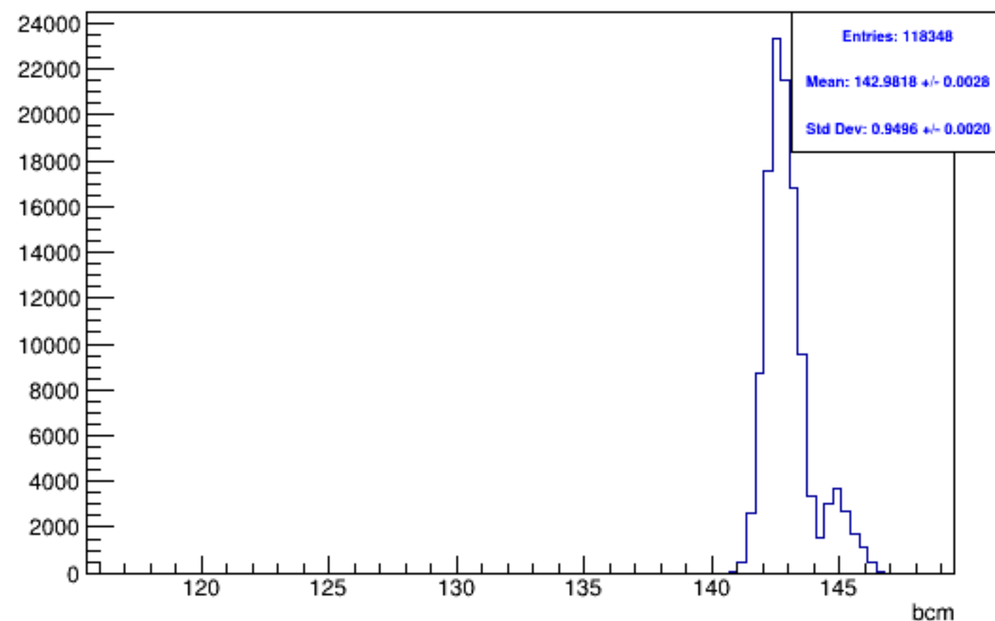
Run 5544, mpwise, BCM: Beam ON, Laser OFF
