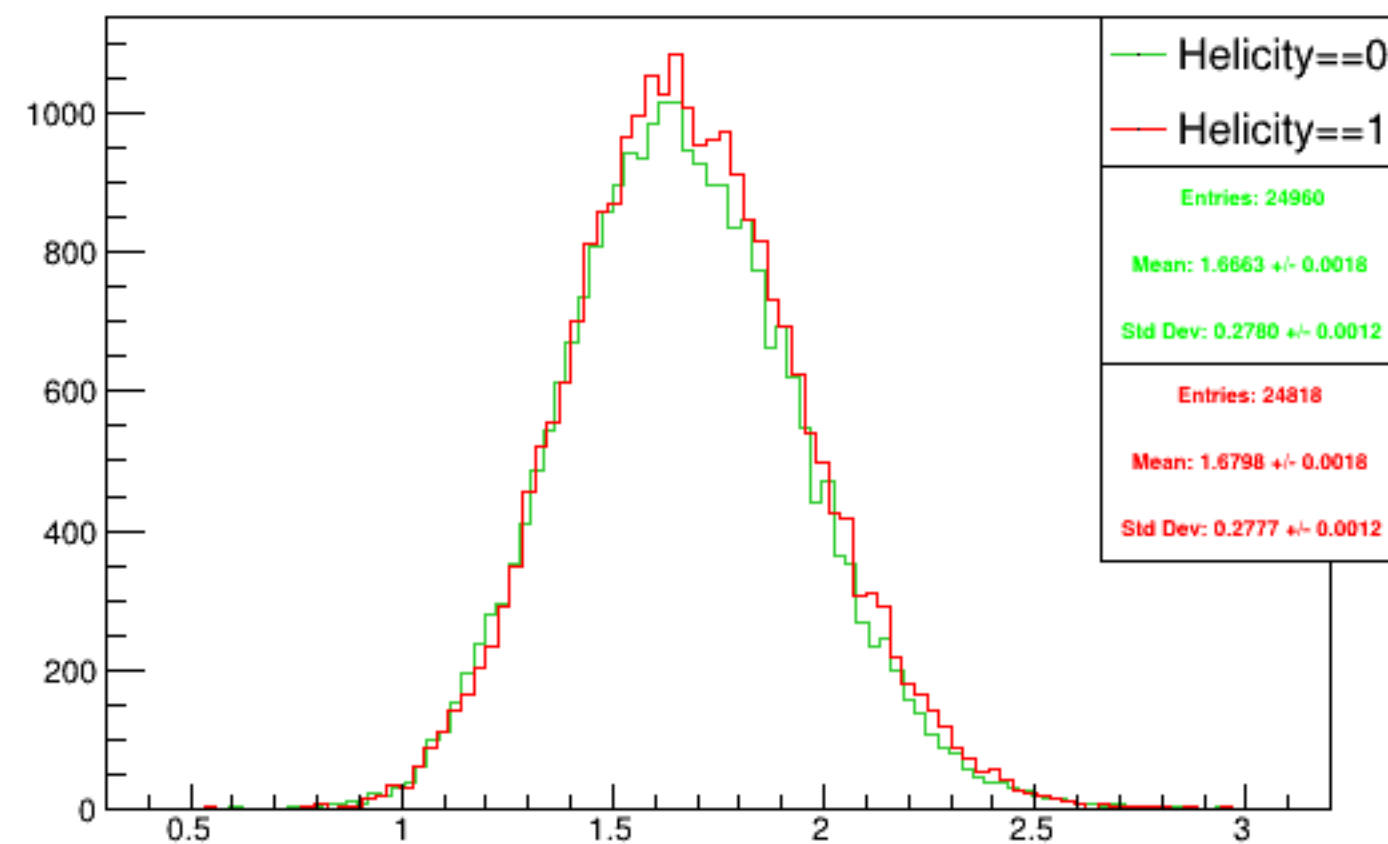
Run 5545 mpwise, acc0: Beam ON, Laser OFF
