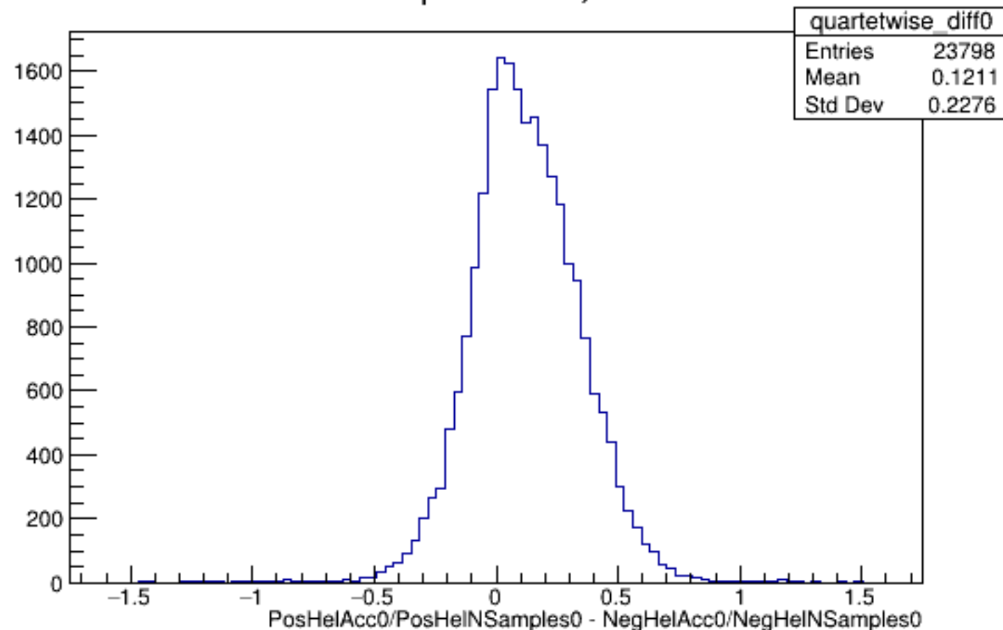
Run 5546 quartetwise, Diffs0: All
