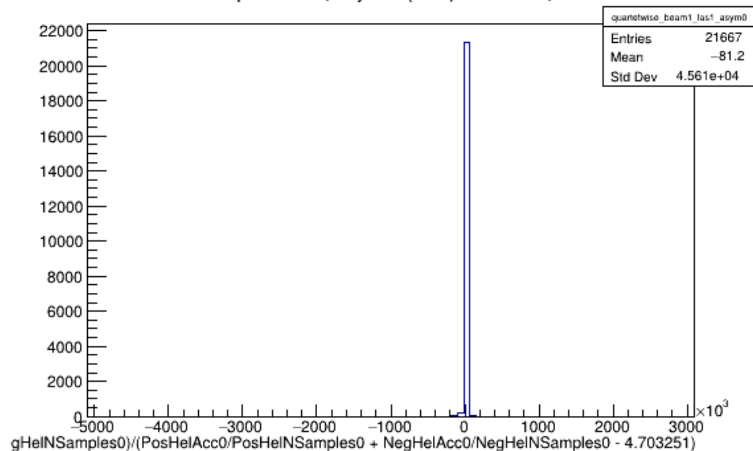
Run 5546 quartetwise, Asyms0 (Raw): Beam ON, Laser ON
