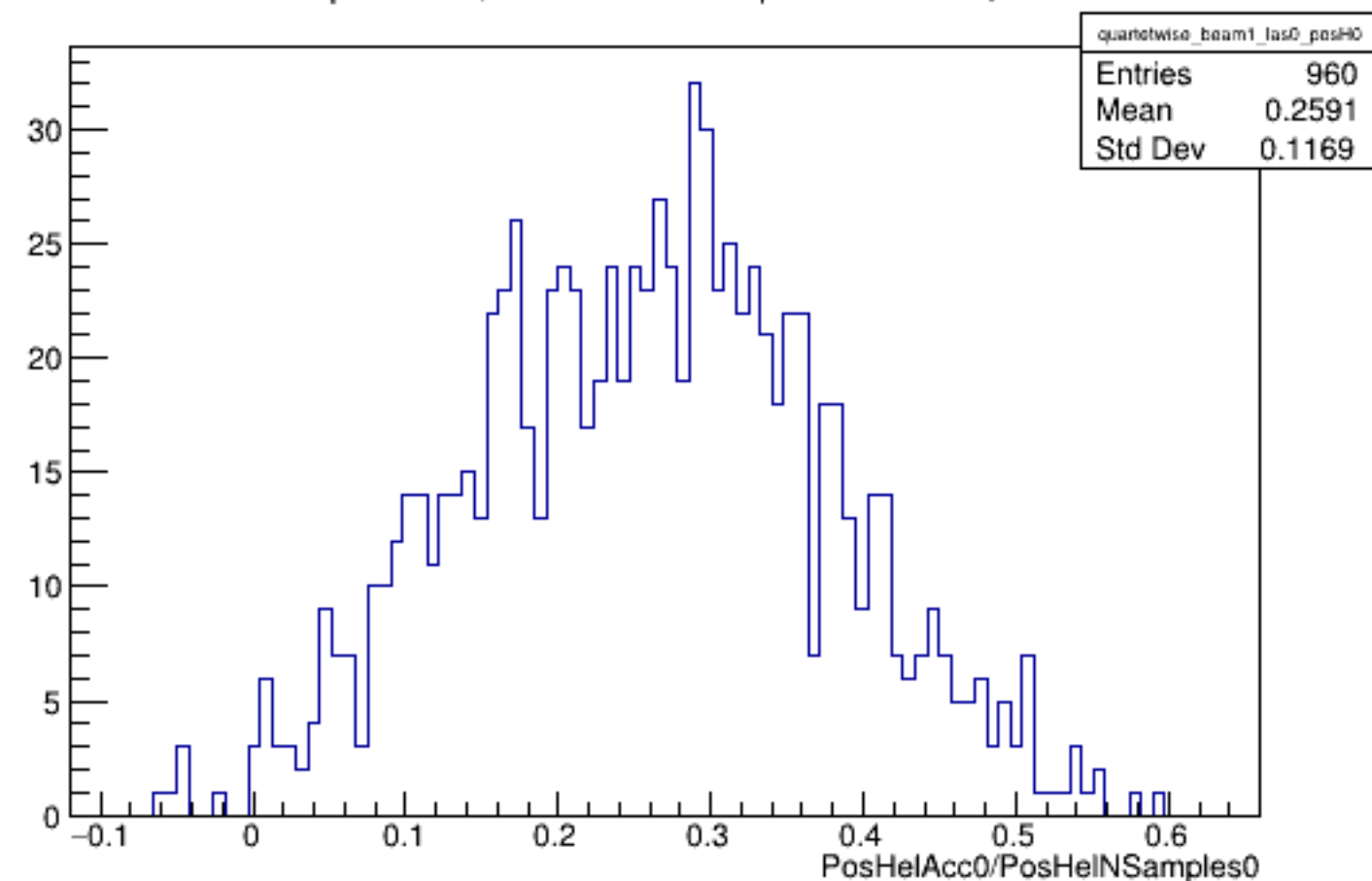
Run 5546 quartetwise, PosHelAcc0/NSamples0: Beam ON, Laser OFF
