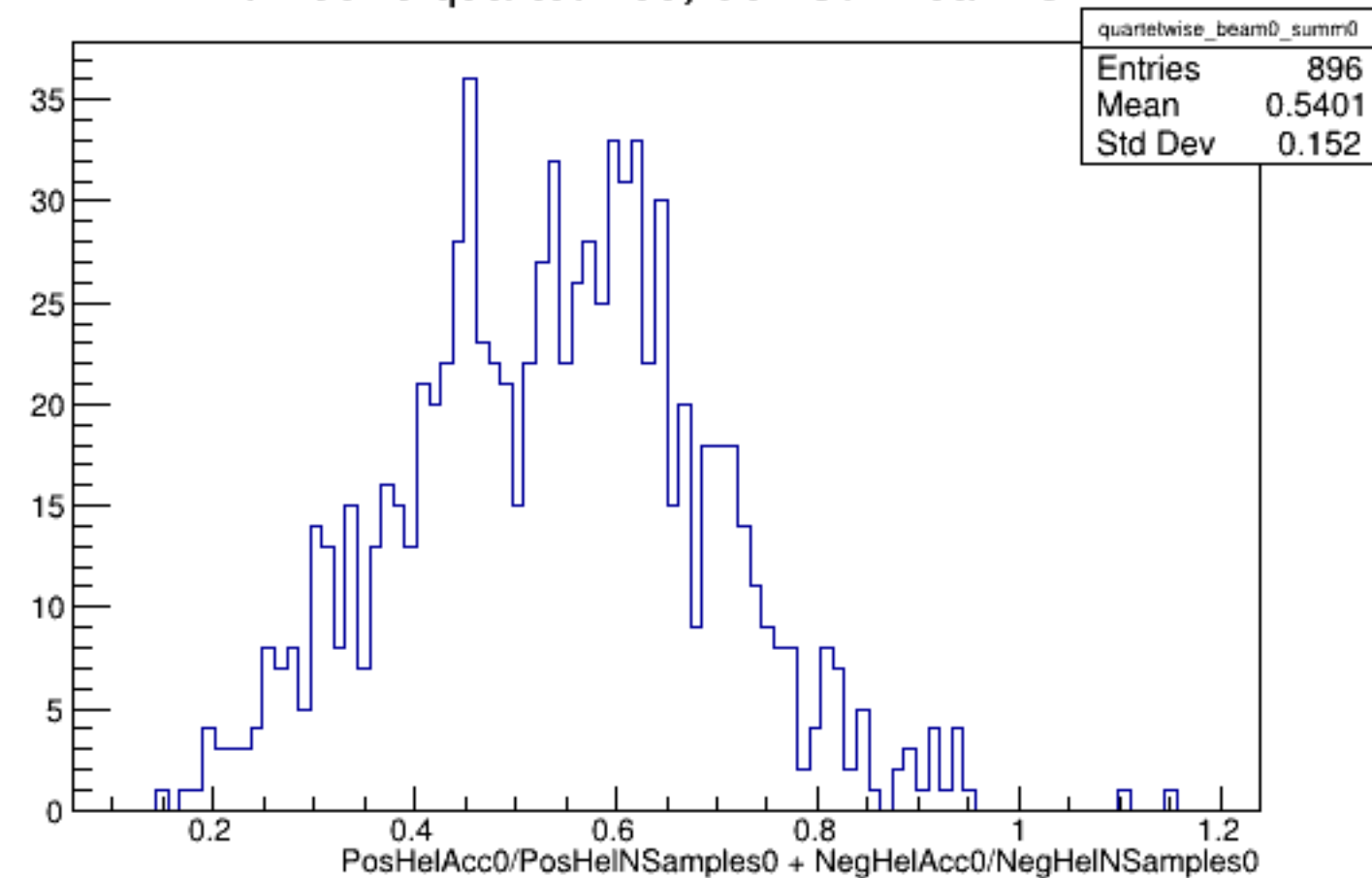
Run 5546 quartetwise, Sums0: Beam OFF
