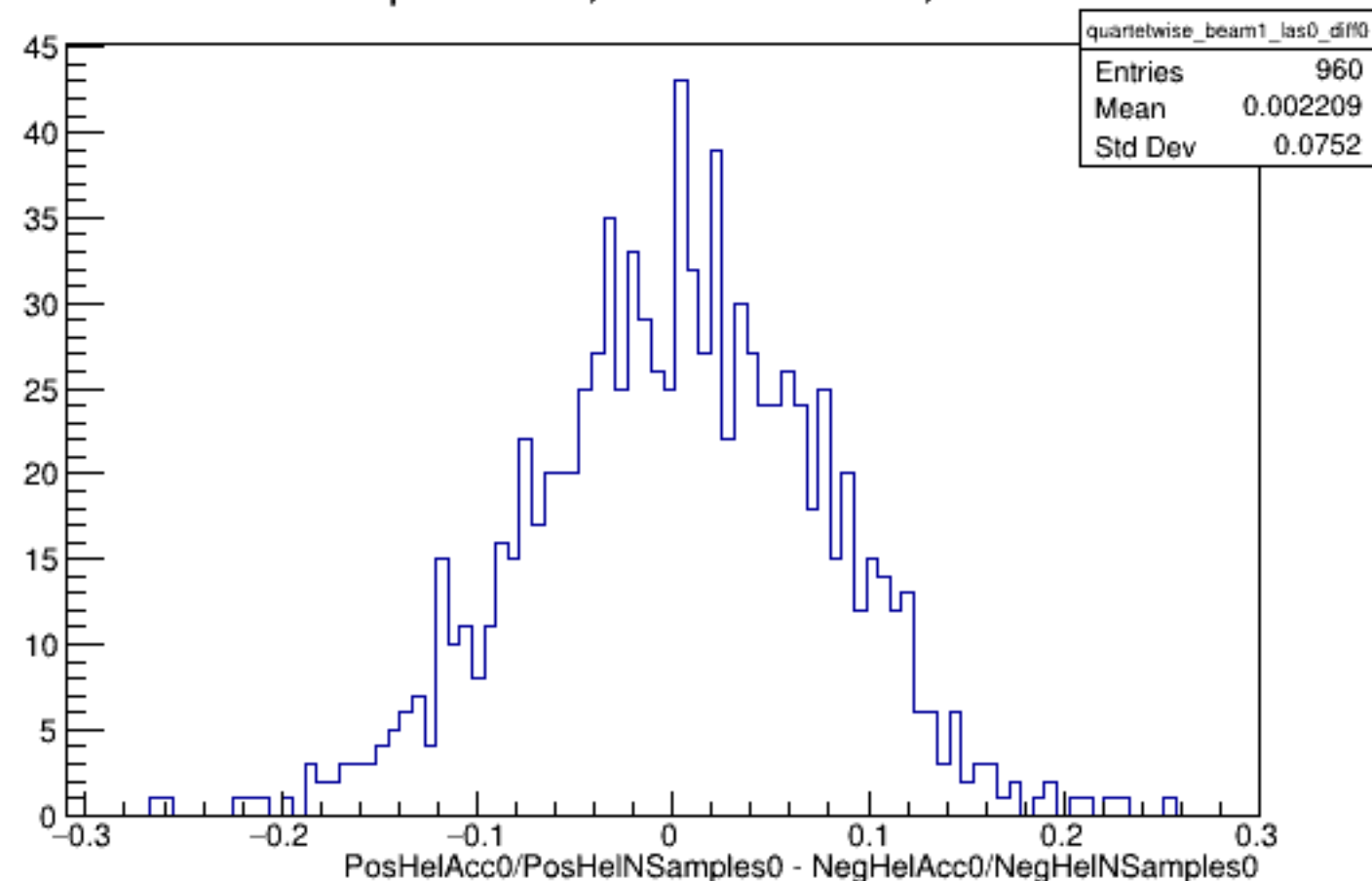
Run 5546 quartetwise, Diffs0: Beam ON, Laser OFF
