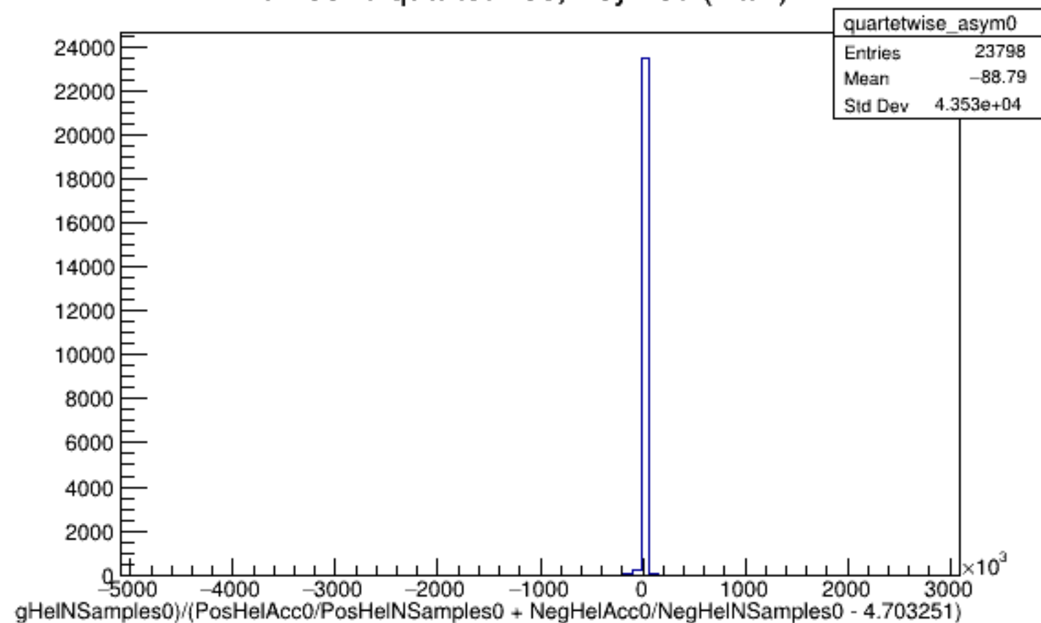
Run 5546 quartetwise, Asyms0 (Raw): All
