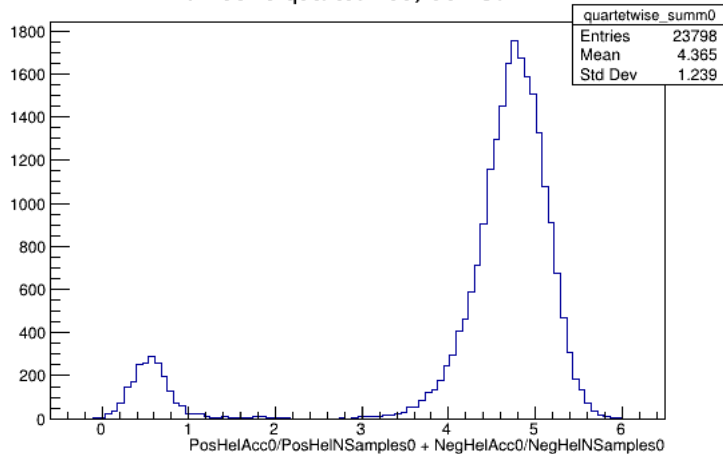
Run 5546 quartetwise, Sums0: All
