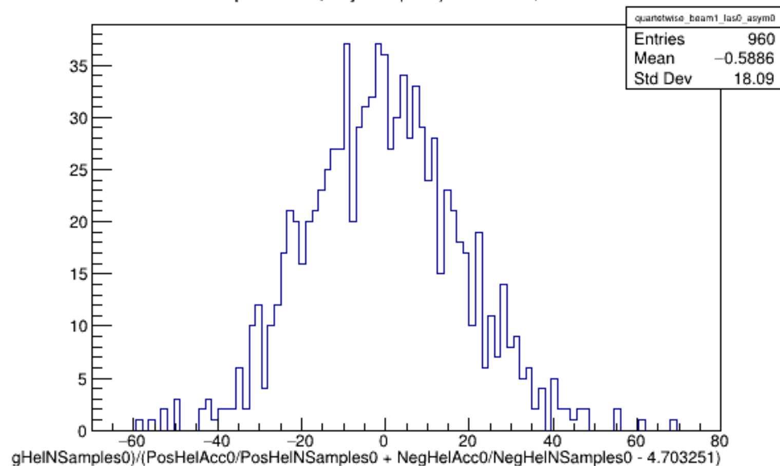
Run 5546 quartetwise, Asyms0 (Raw): Beam ON, Laser OFF
