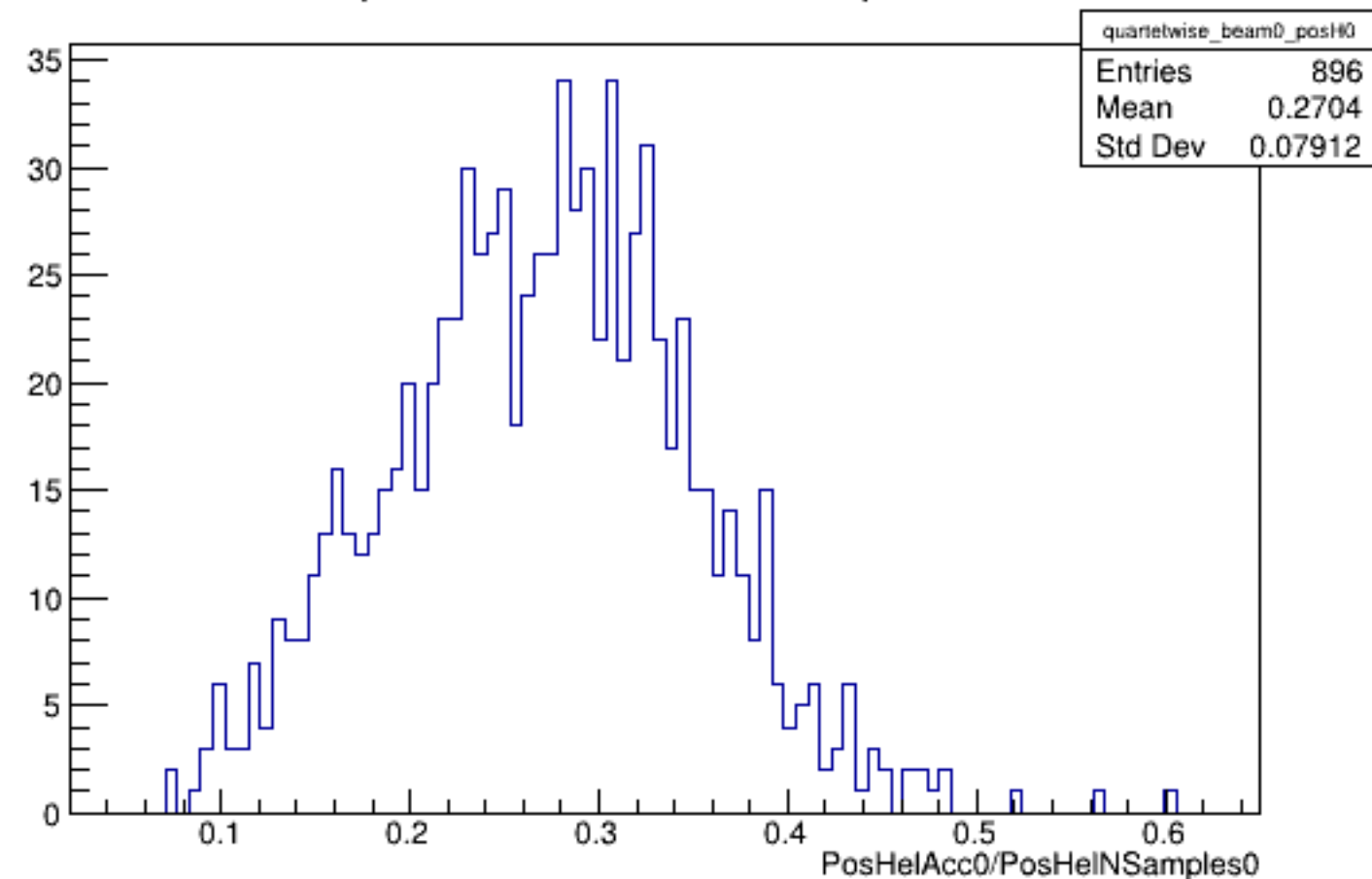
Run 5546 quartetwise, PosHelAcc0/NSamples0: Beam OFF
