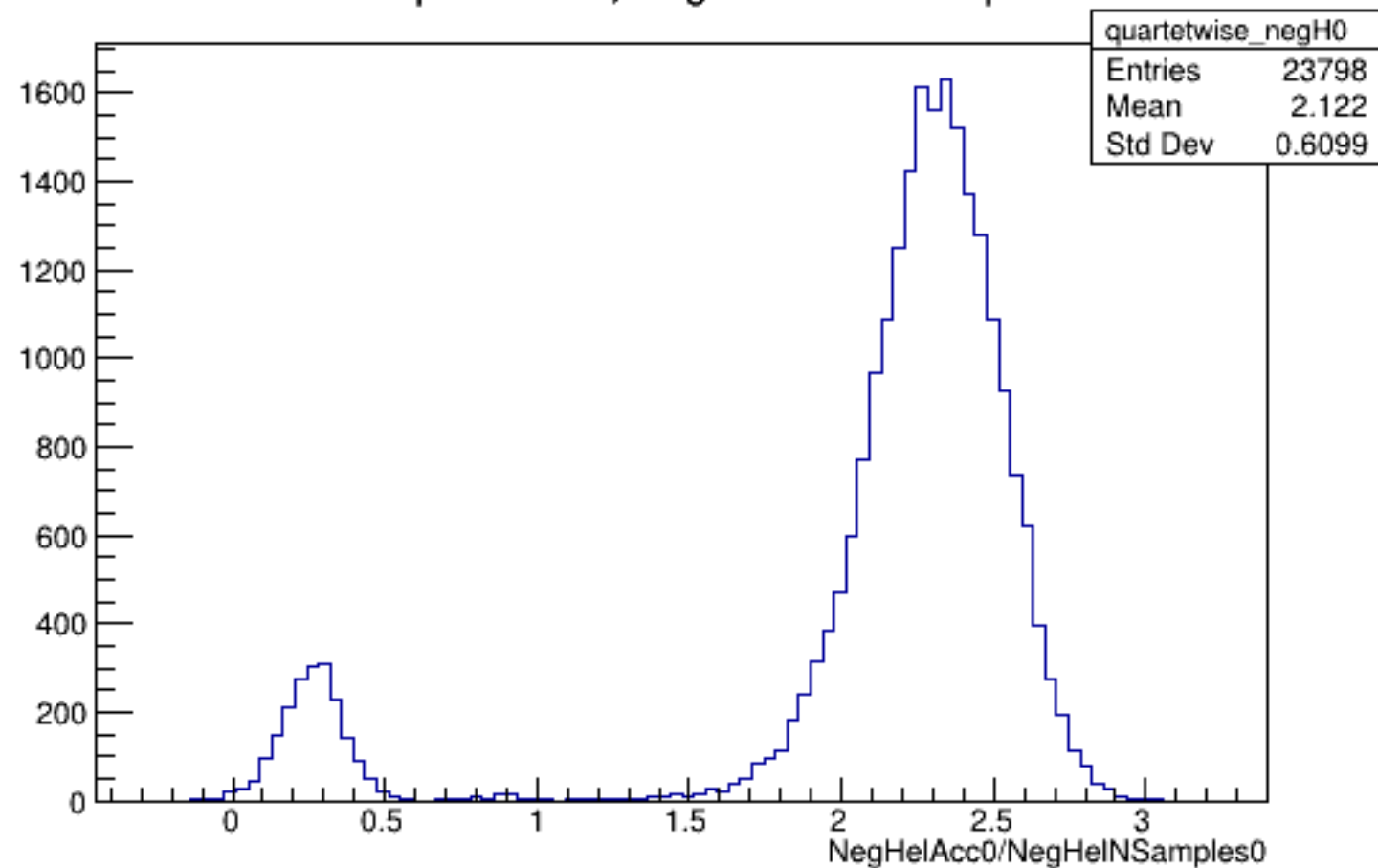
Run 5546 quartetwise, NegHelAcc0/NSamples0: All
