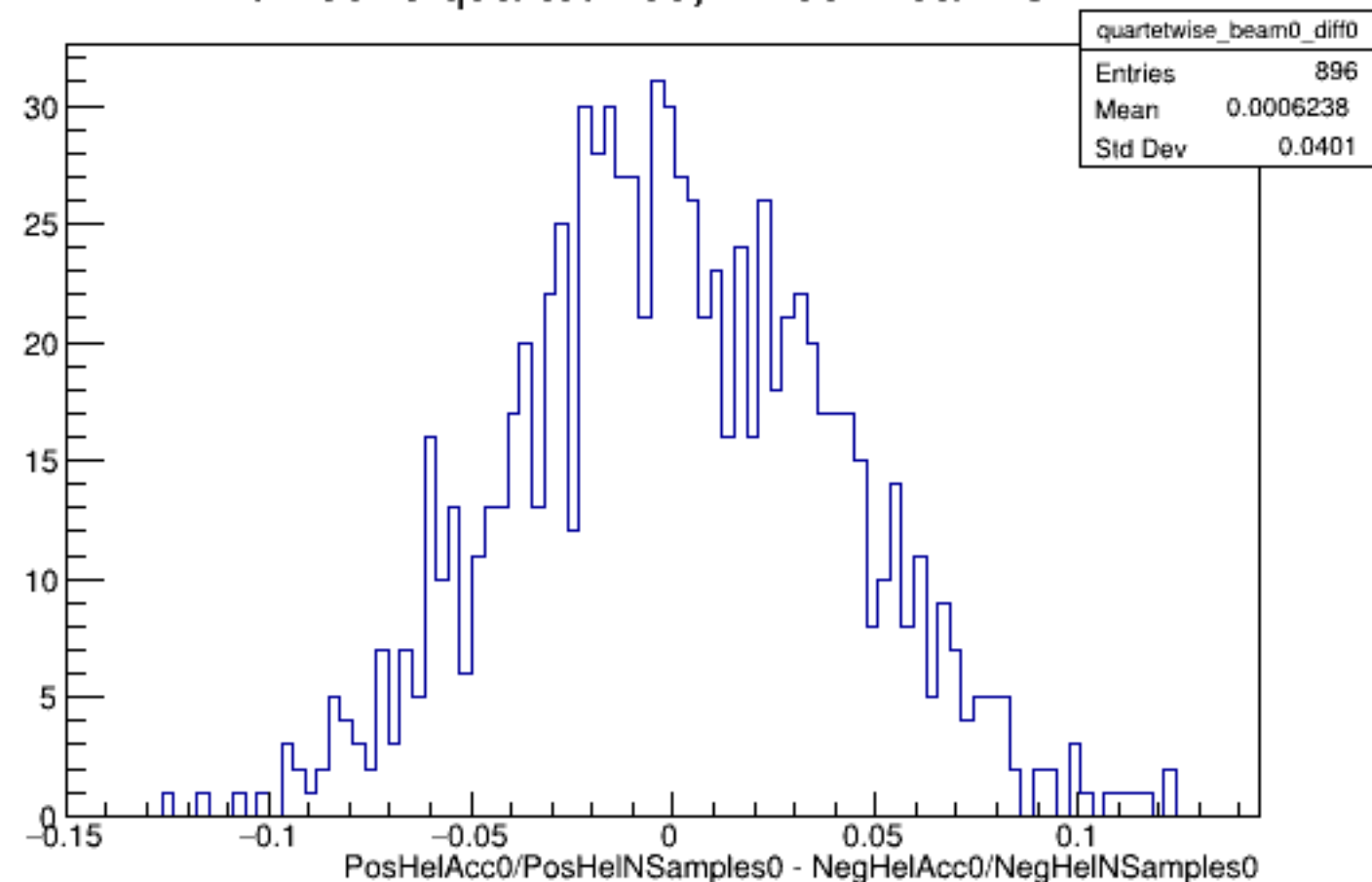
Run 5546 quartetwise, Diffs0: Beam OFF
