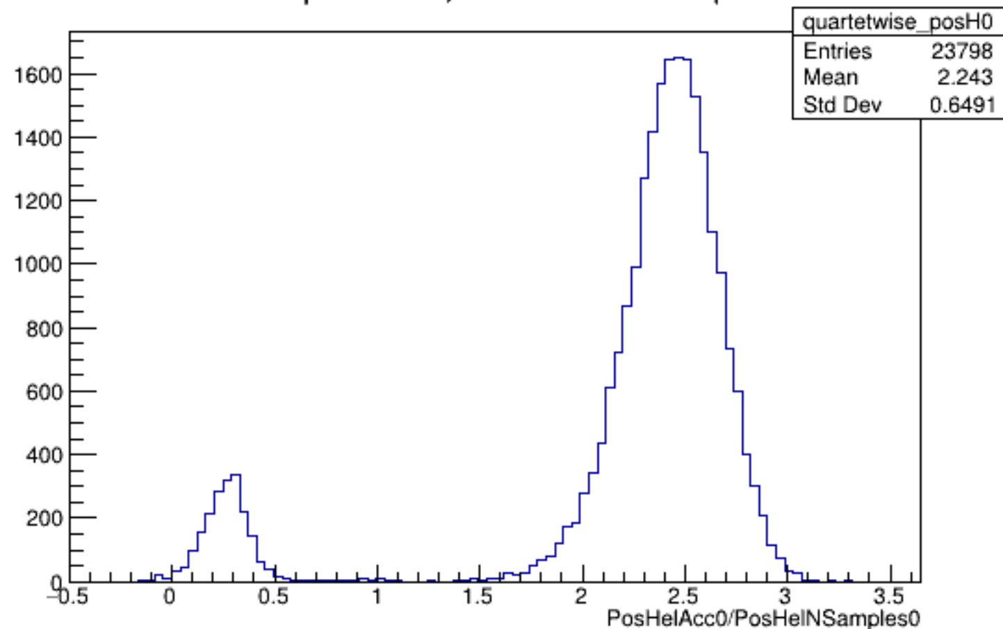
Run 5546 quartetwise, PosHelAcc0/NSamples0: All
