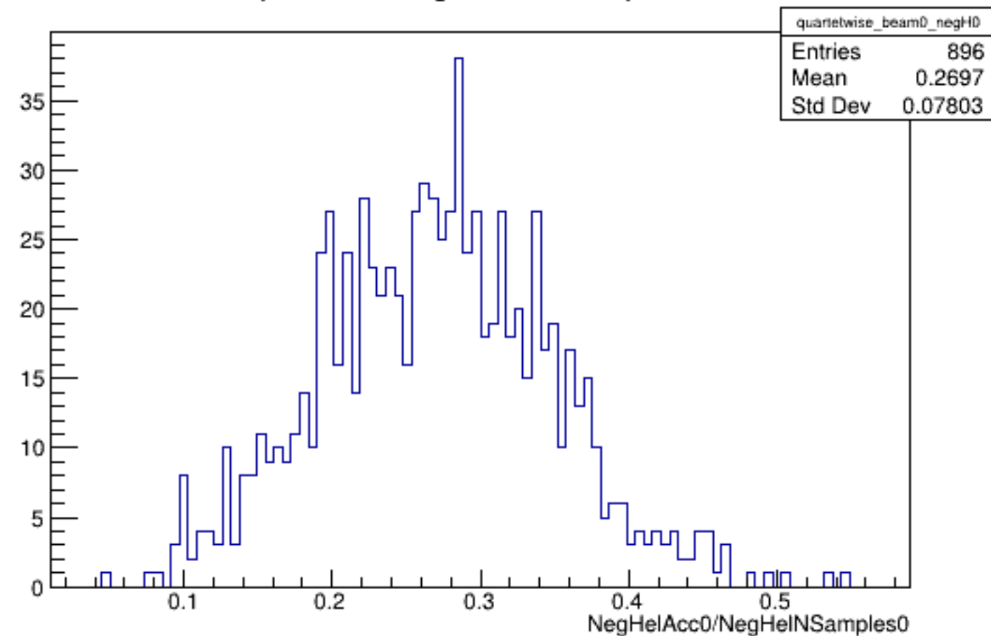
Run 5546 quartetwise, NegHelAcc0/NSamples0: Beam OFF
