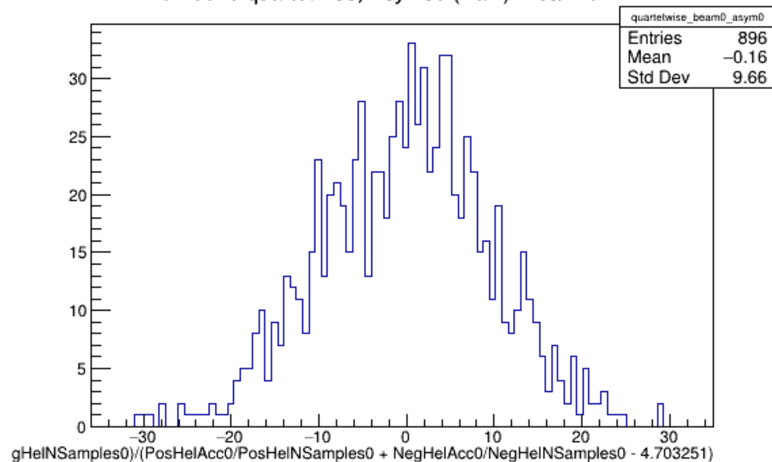
Run 5546 quartetwise, Asyms0 (Raw): Beam OFF
