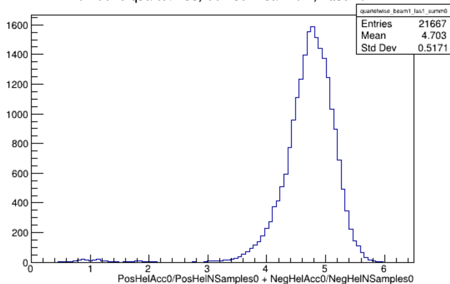
Run 5546 quartetwise, Sums0: Beam ON, Laser ON
