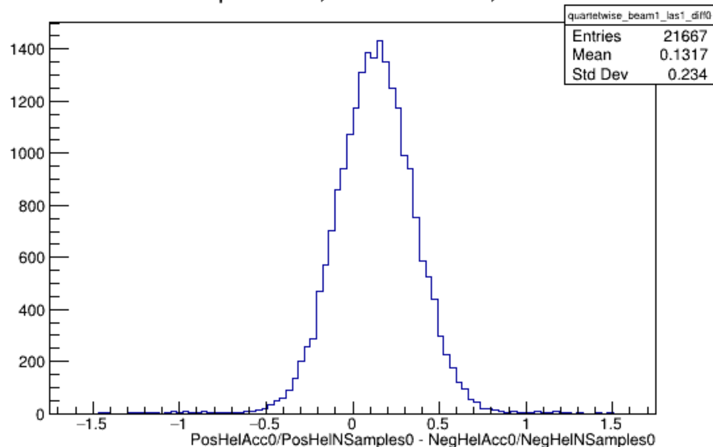
Run 5546 quartetwise, Diffs0: Beam ON, Laser ON
