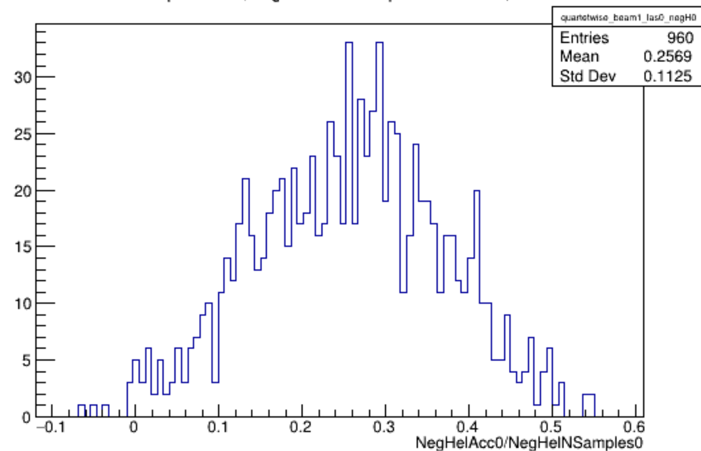
Run 5546 quartetwise, NegHelAcc0/NSamples0: Beam ON, Laser OFF
