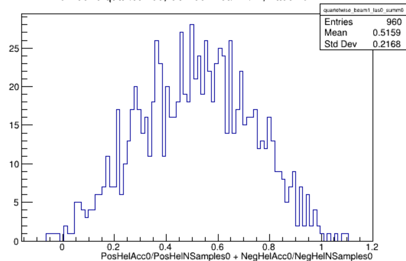
Run 5546 quartetwise, Sums0: Beam ON, Laser OFF
