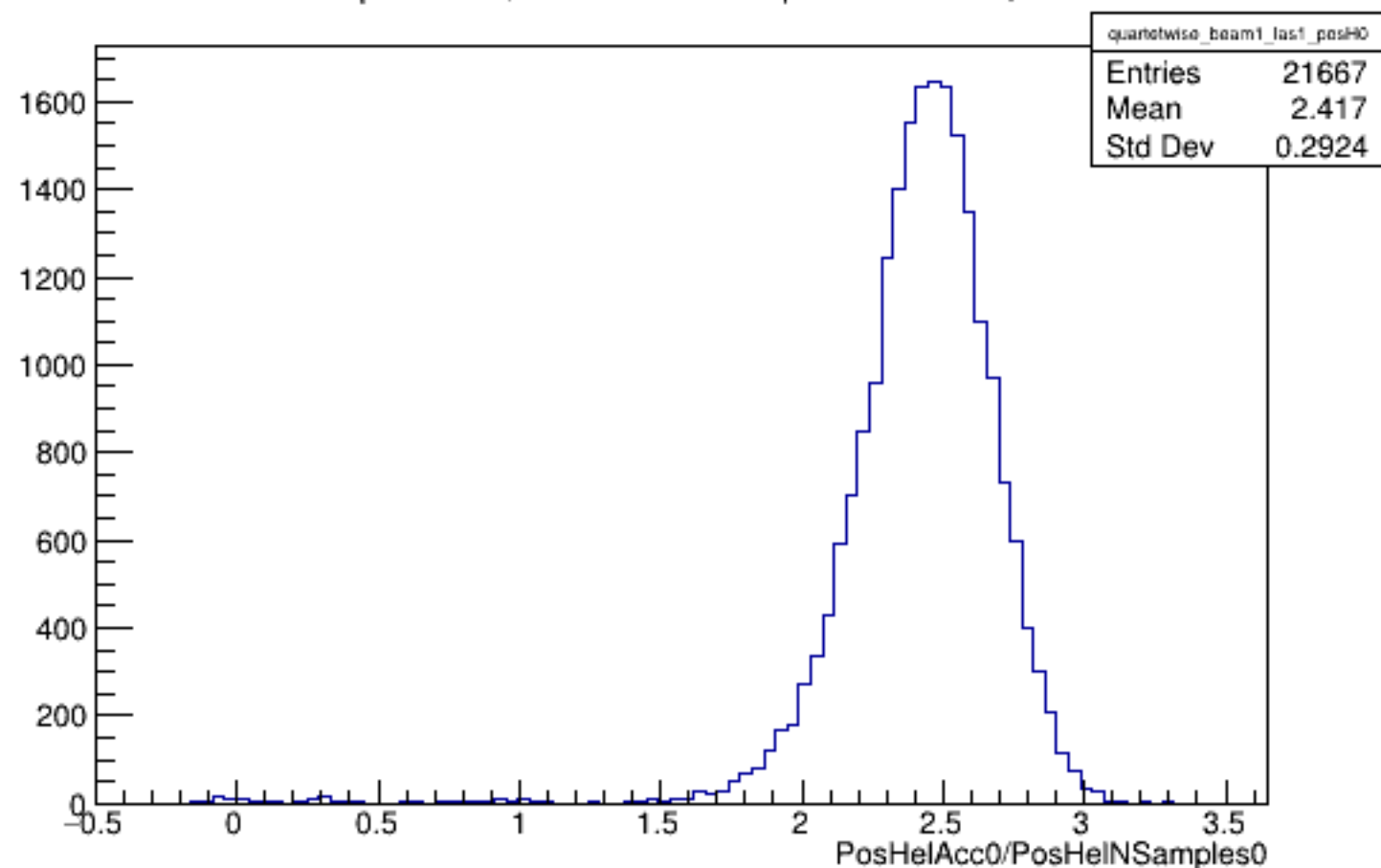
Run 5546 quartetwise, PosHelAcc0/NSamples0: Beam ON, Laser ON
