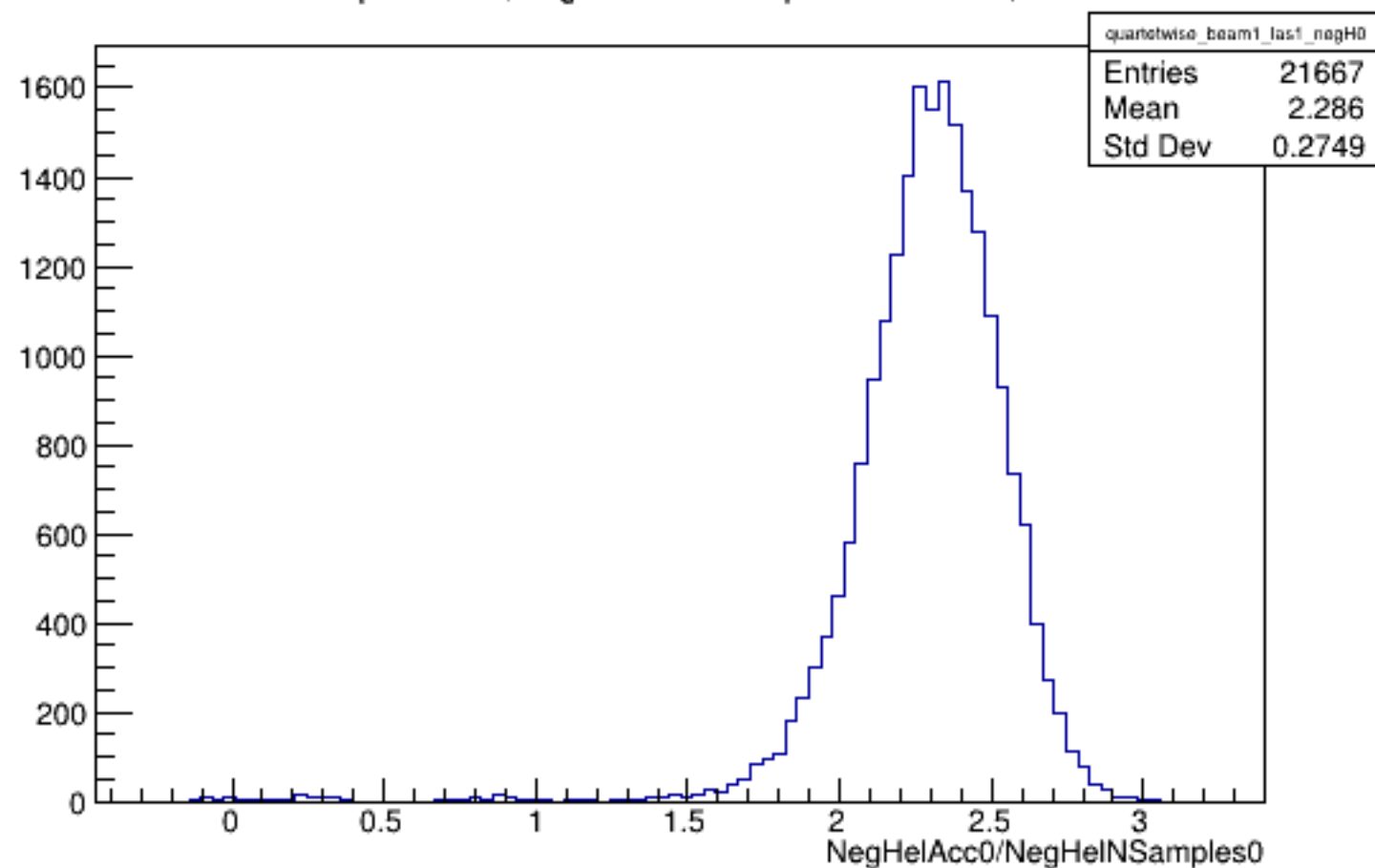
Run 5546 quartetwise, NegHelAcc0/NSamples0: Beam ON, Laser ON
