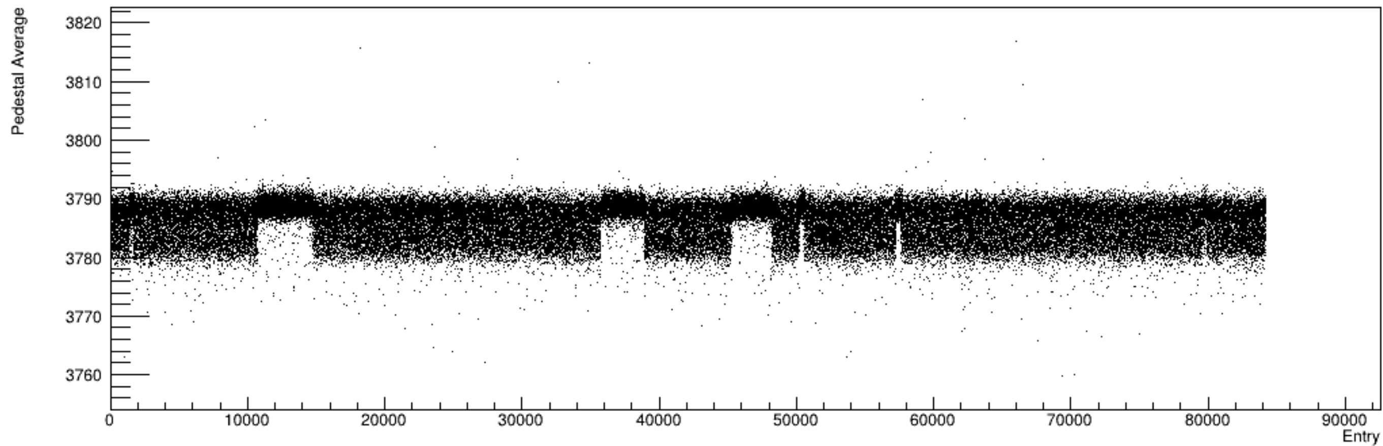
Run 5546, snapshots: Pedestal vs. Time
