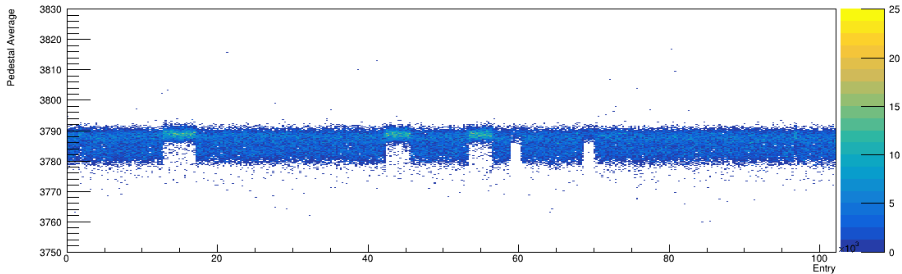
Run 5546, snapshots: Pedestal vs. Time
