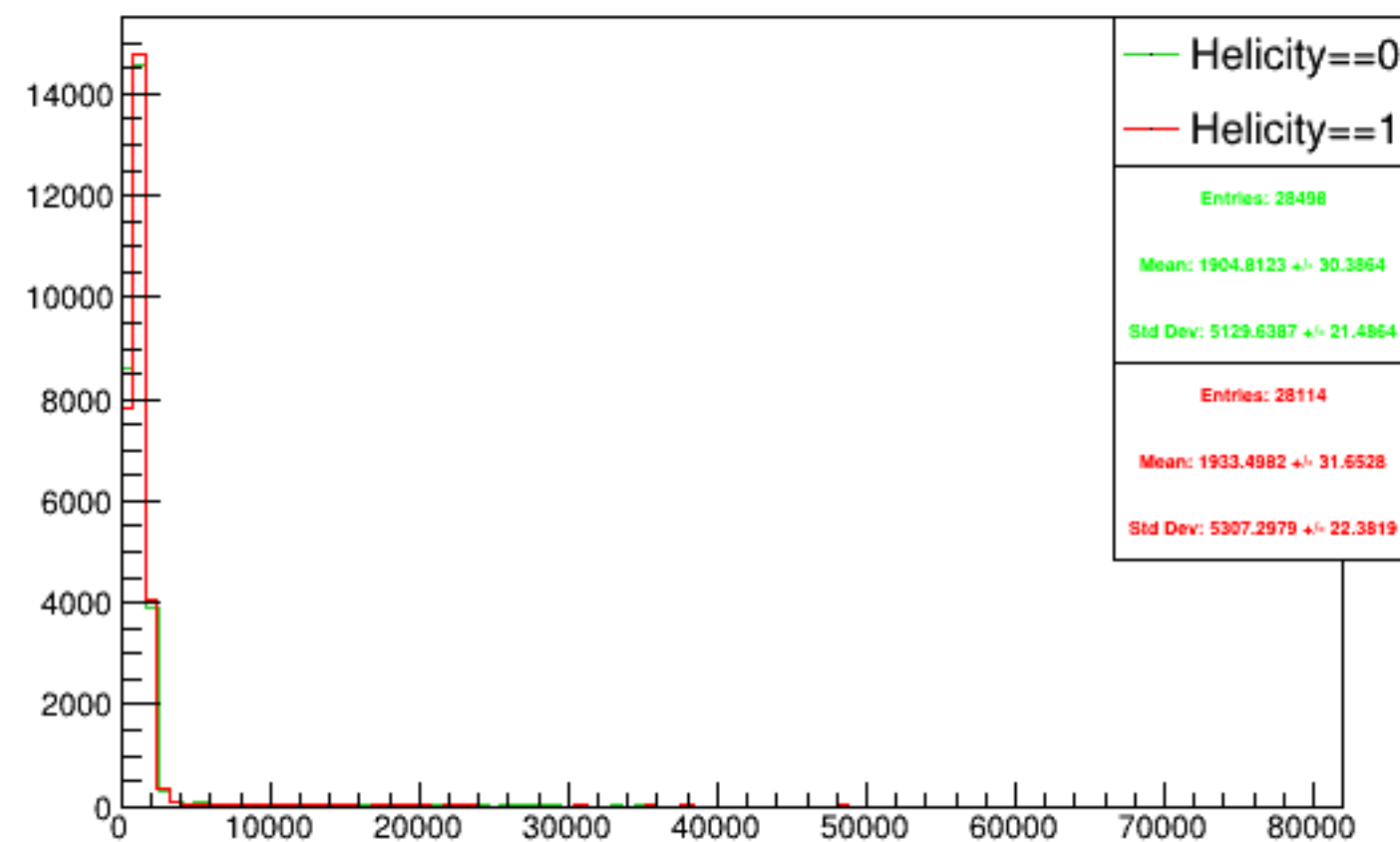
Run 5546 triggerwise, sums: Beam ON, Laser OFF
