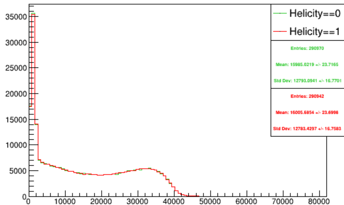
Run 5546 triggerwise, sums: Beam ON, Laser ON
