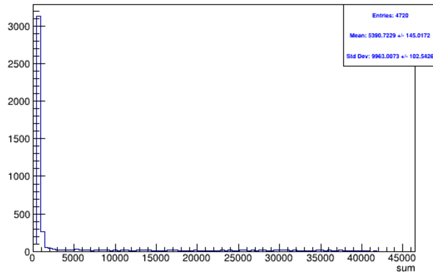
Run 5546 triggerwise, sums: Beam OFF
