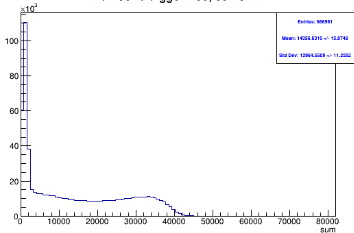
Run 5546 triggerwise, sums: All
