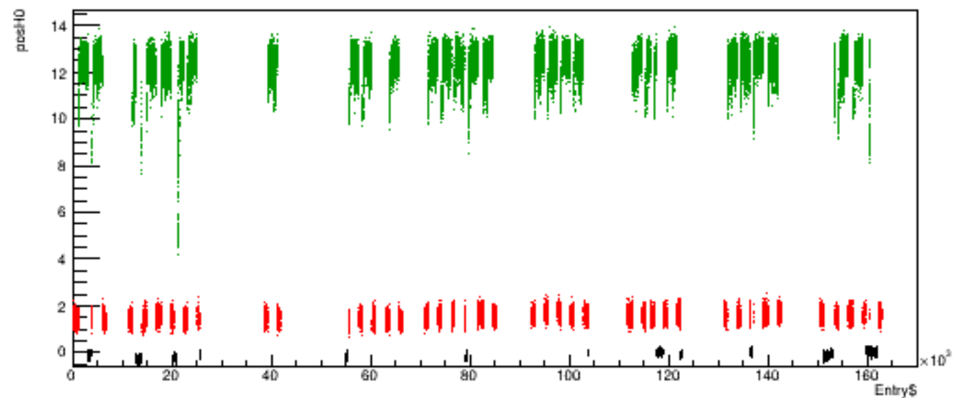
Run 5554 quartetwise, posH0 vs time
