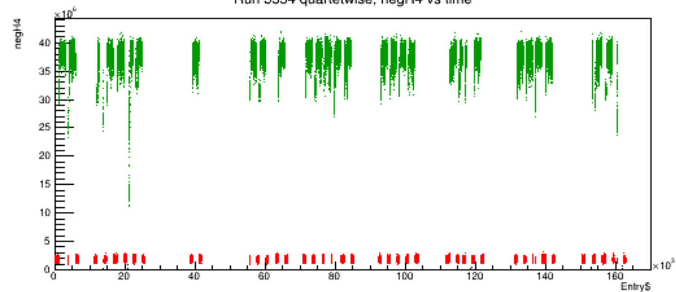
Run 5554 quartetwise, negH4 vs time
