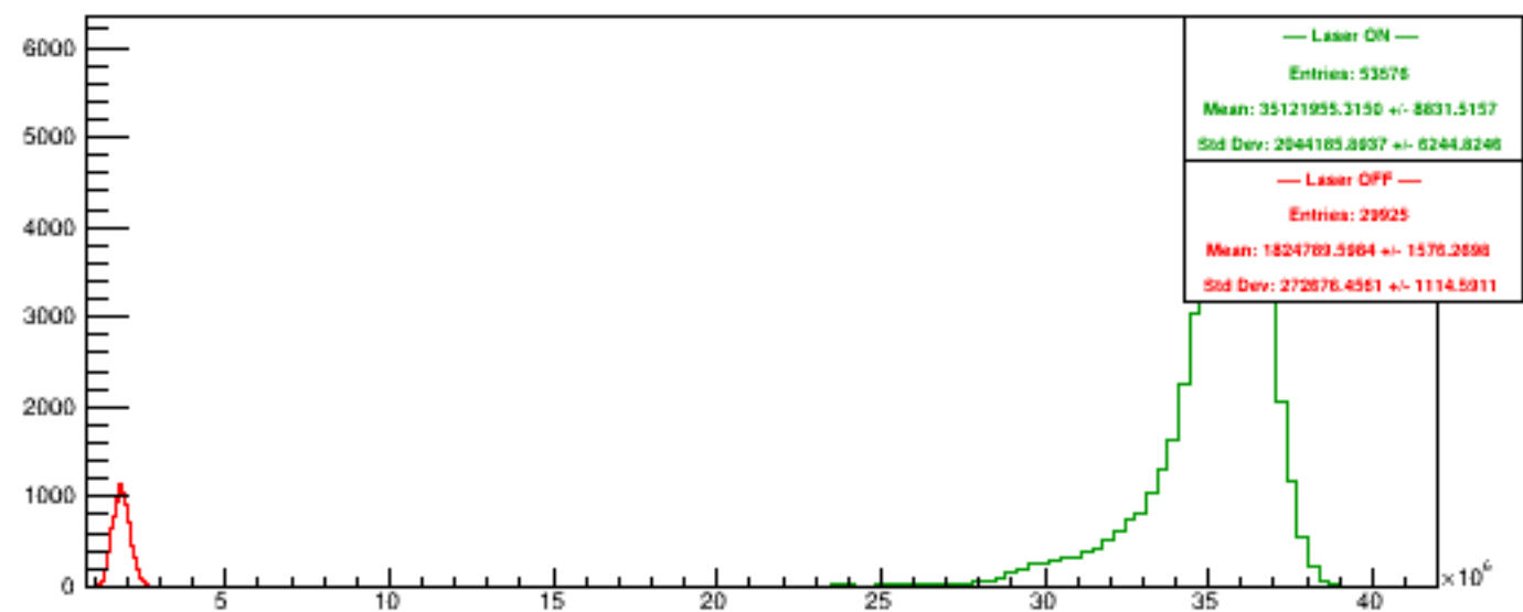
Run 5554 quartetwise, PosHelAcc4
