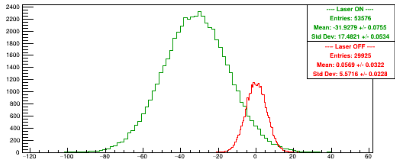
Run 5554 quartetwise, Asyms4
