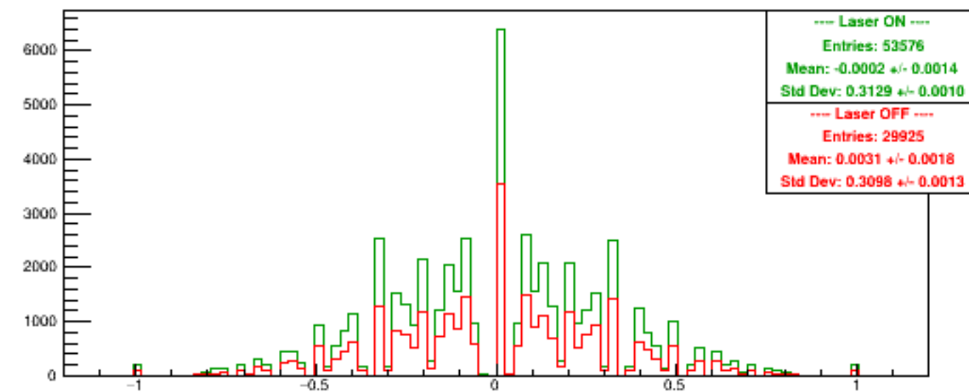
Run 5554 quartetwise, Asyms USbg2
