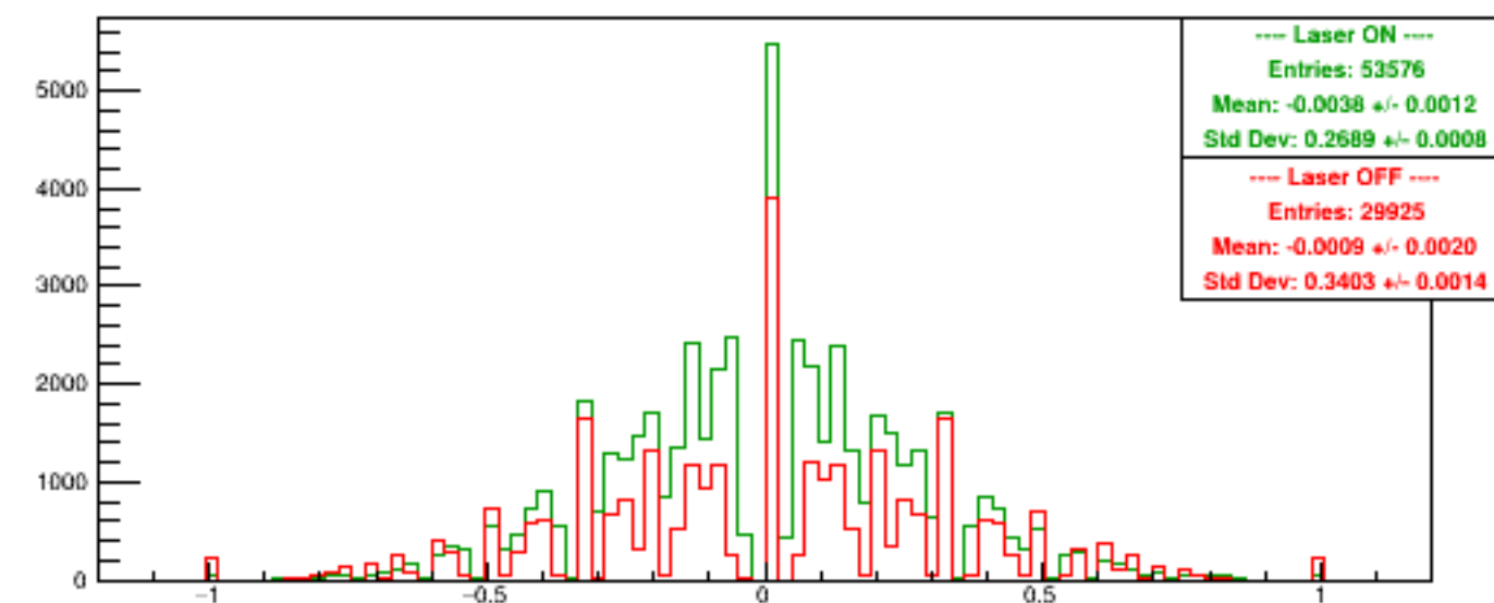
Run 5554 quartetwise, Asyms Vert Finger
