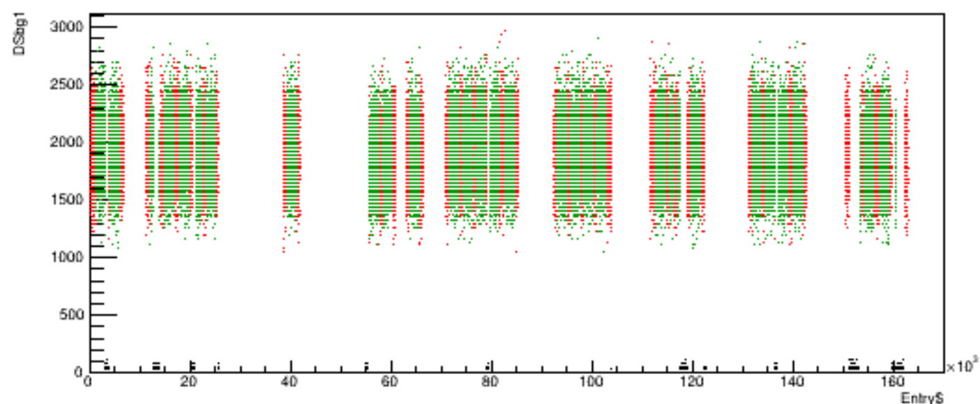
Run 5554 quartetwise, DSbg1 vs time
