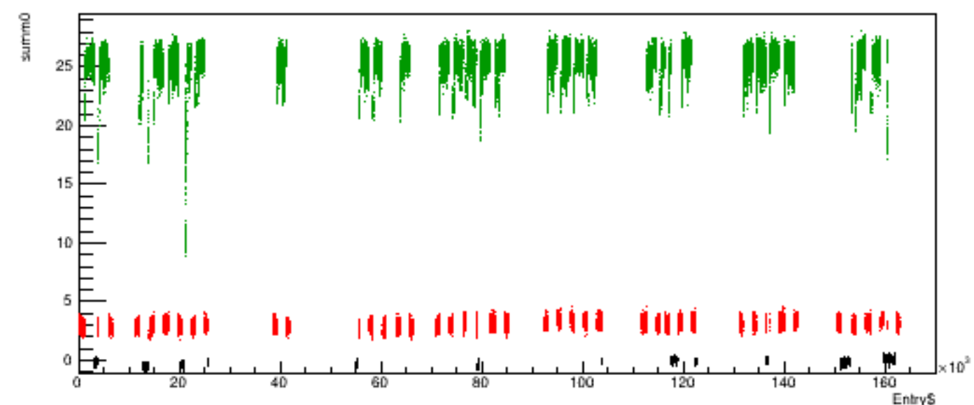
Run 5554 quartetwise, summ0 vs time
