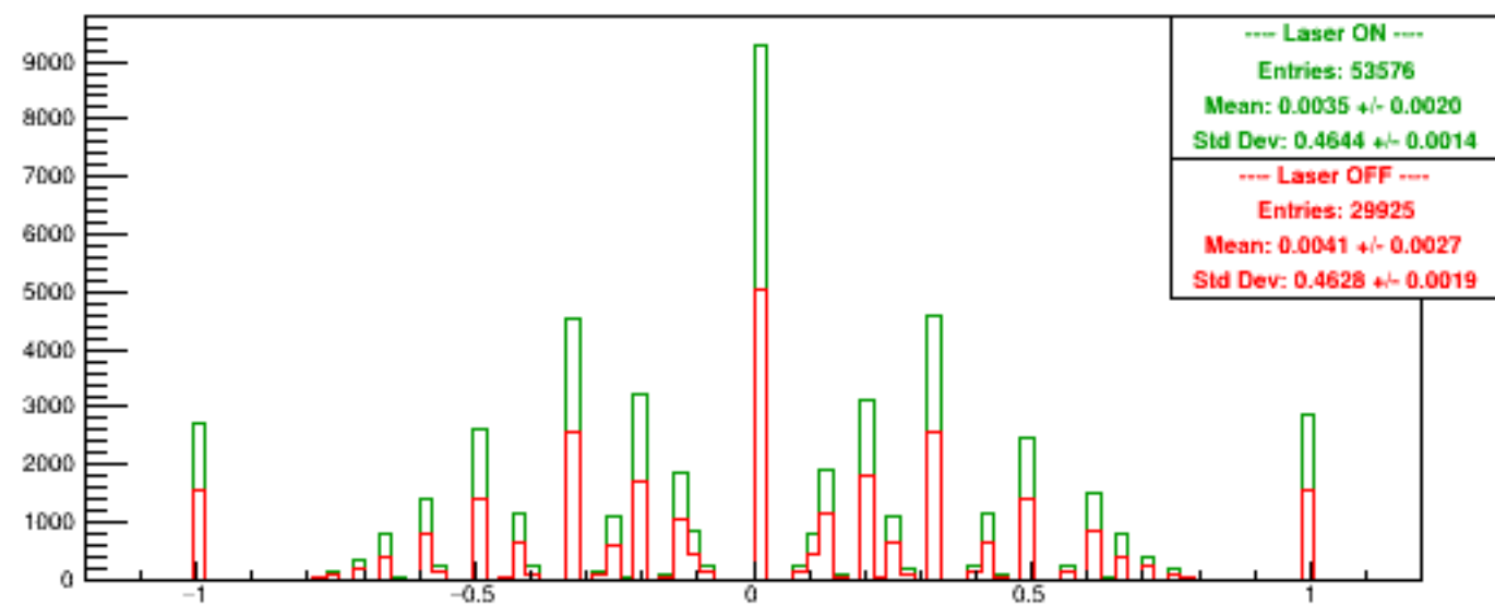
Run 5554 quartetwise, Asyms USbg1
