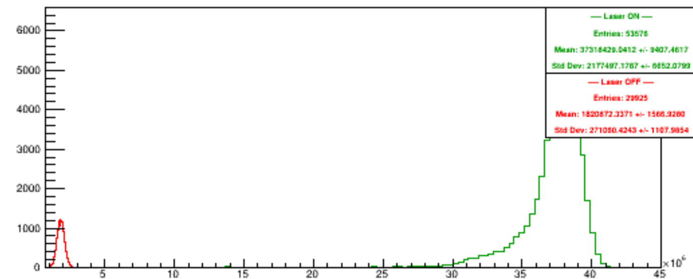
Run 5554 quartetwise, NegHelAcc4
