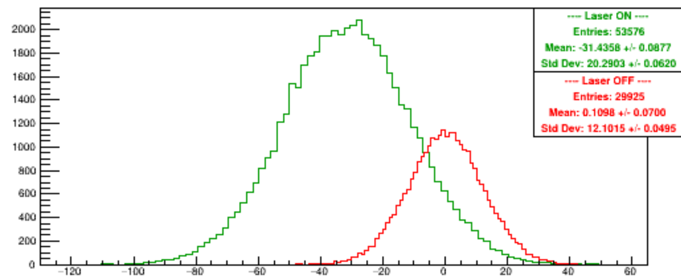
Run 5554 quartetwise, Asyms0
