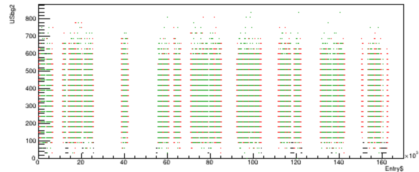
Run 5554 quartetwise, USbg2 vs time
