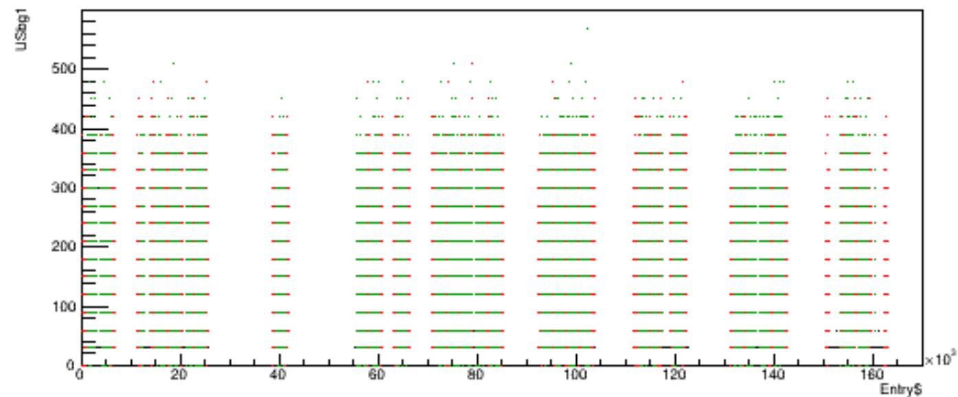
Run 5554 quartetwise, USbg1 vs time
