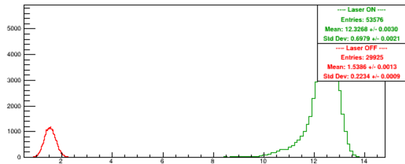
Run 5554 quartetwise, PosHelAcc0/NSamples0
