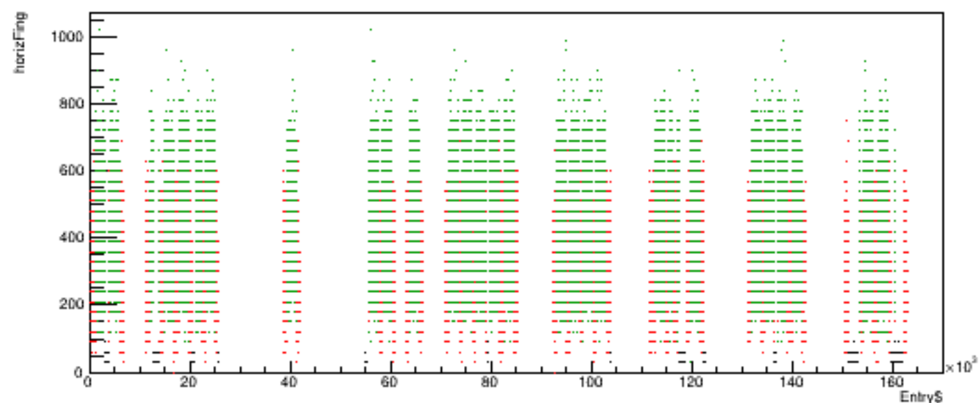
Run 5554 quartetwise, horizFing vs time
