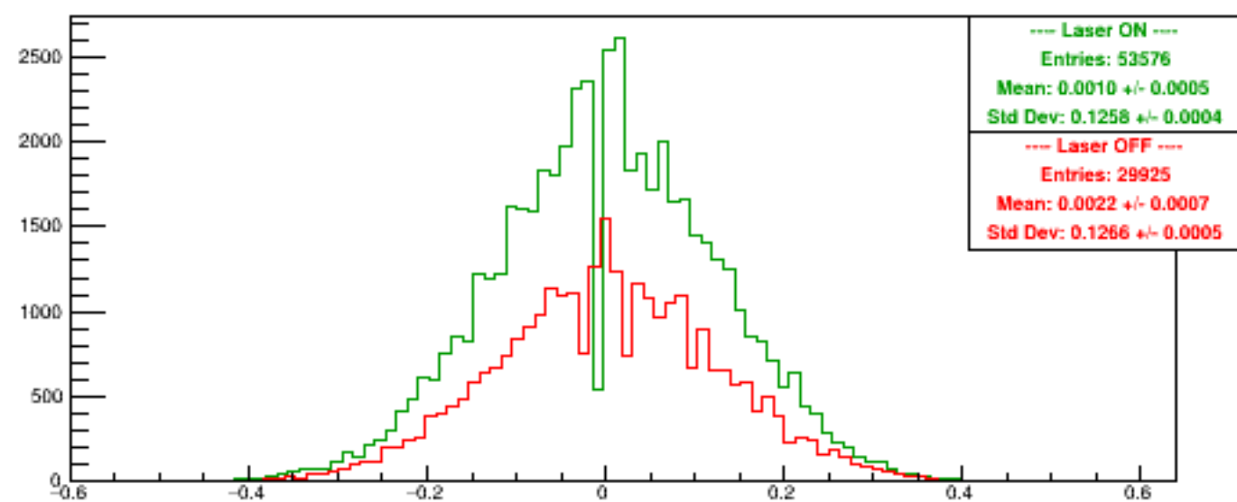
Run 5554 quartetwise, Asyms DSbg1
