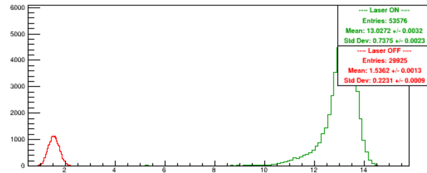
Run 5554 quartetwise, NegHelAcc0/NSamples0
