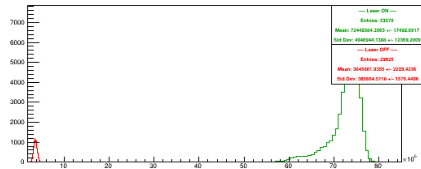
Run 5554 quartetwise, Sums4
