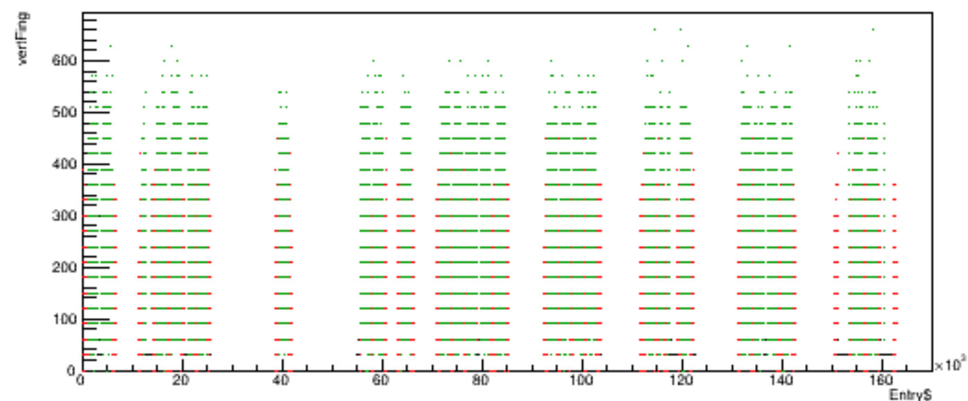
Run 5554 quartetwise, vertFing vs time
