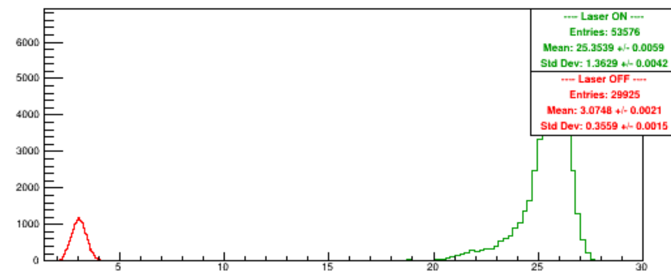
Run 5554 quartetwise, Sums0
