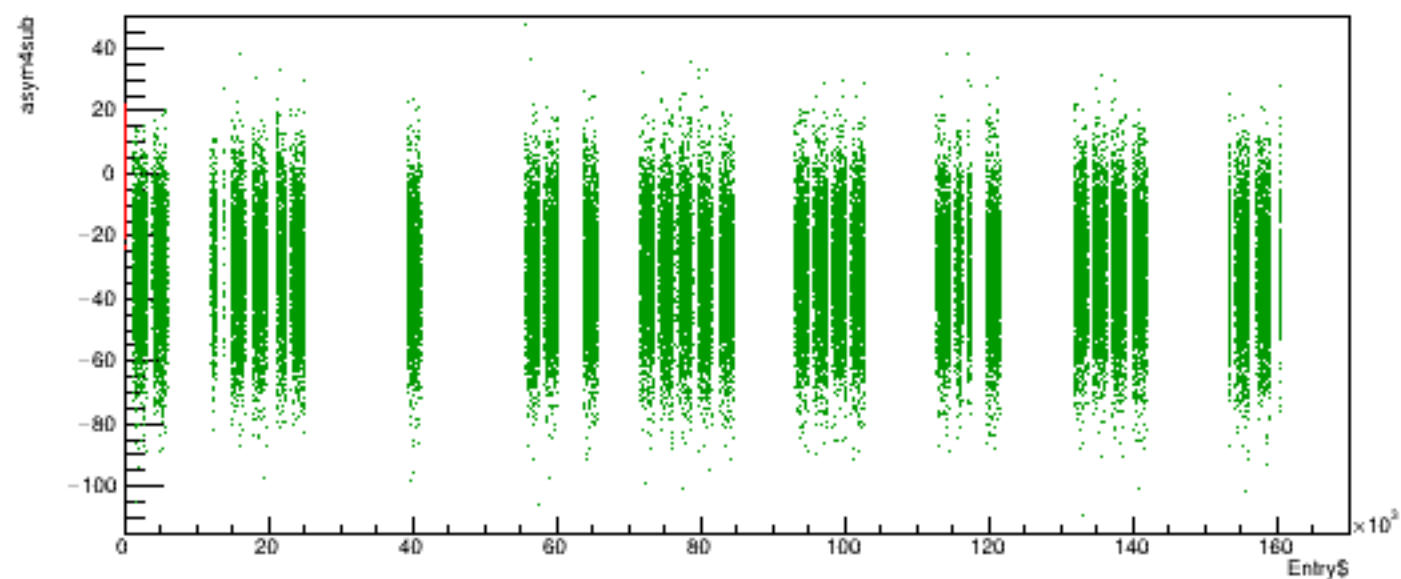
Run 5554 quartetwise, asym4sub vs time
