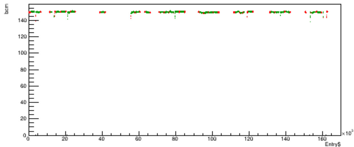
Run 5554 quartetwise, posH4 vs time
