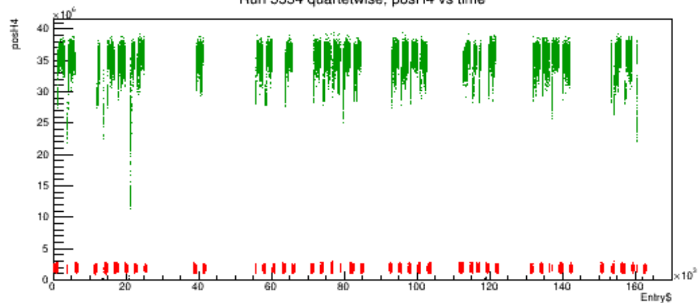
Run 5554 quartetwise, posH4 vs time
