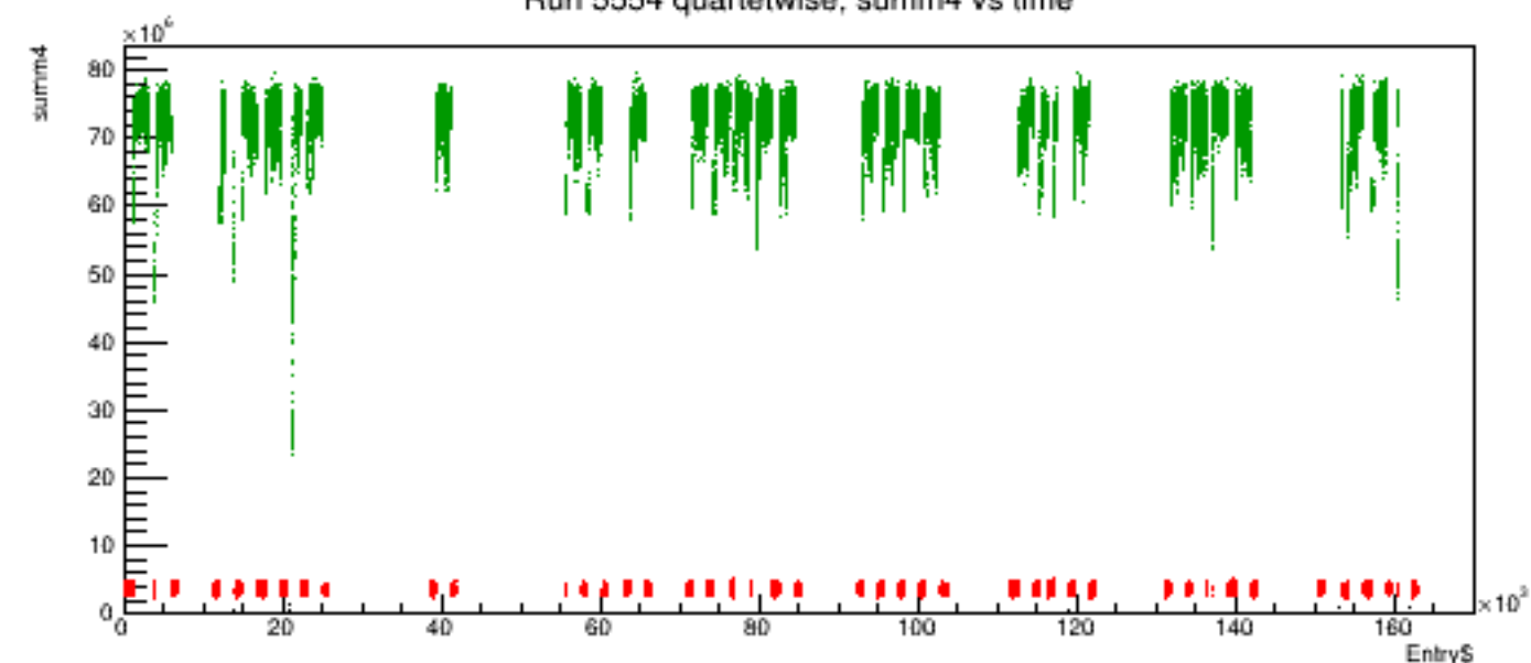
Run 5554 quartetwise, summ4 vs time
