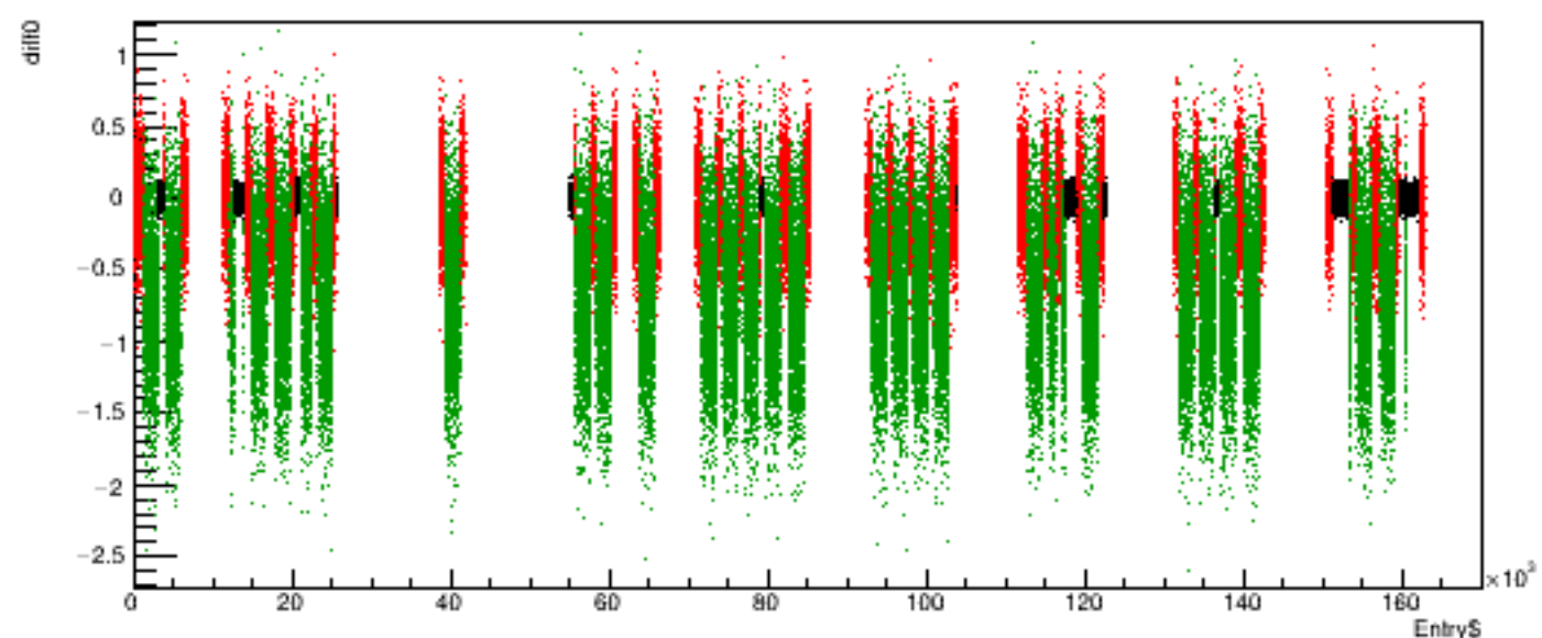
Run 5554 quartetwise, diff0 vs time
