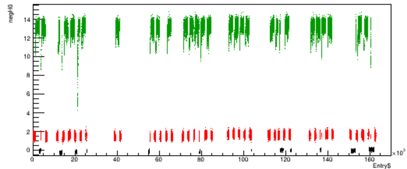
Run 5554 quartetwise, negH0 vs time
