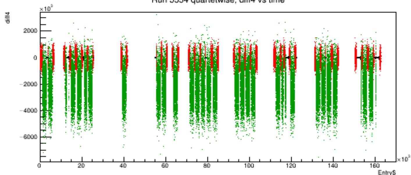
Run 5554 quartetwise, diff4 vs time
