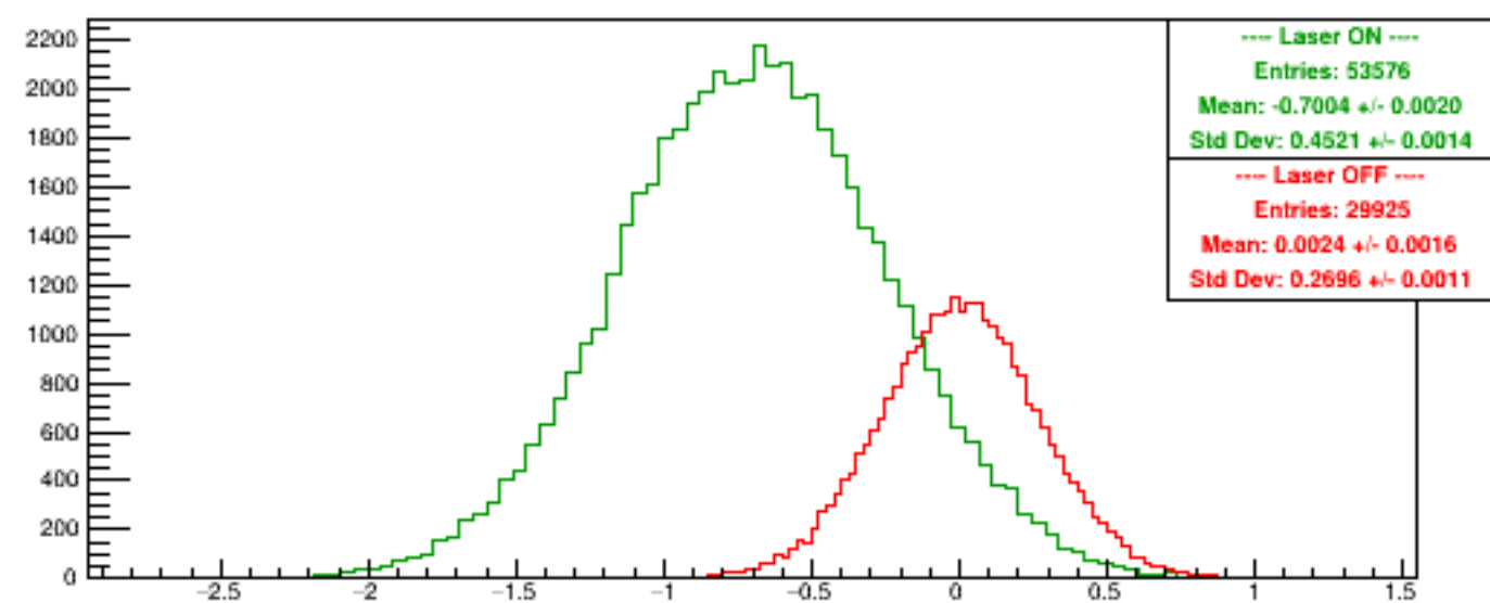
Run 5554 quartetwise, Diffs0
