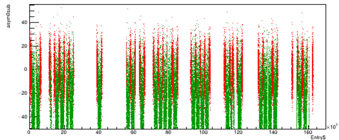
Run 5554 quartetwise, asym0sub vs time
