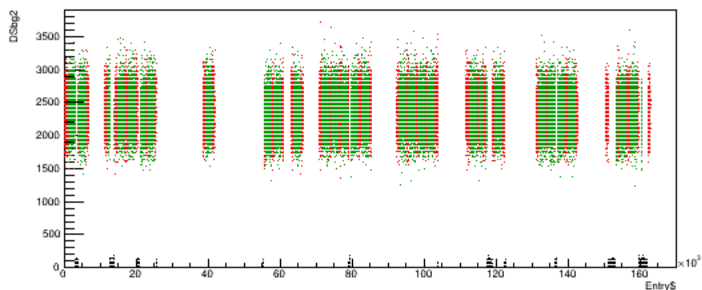
Run 5554 quartetwise, DSbg2 vs time
