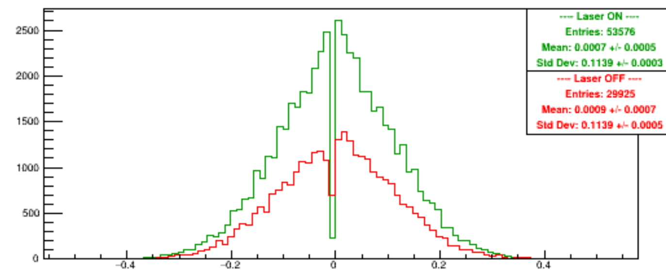
Run 5554 quartetwise, Asyms DSbg2
