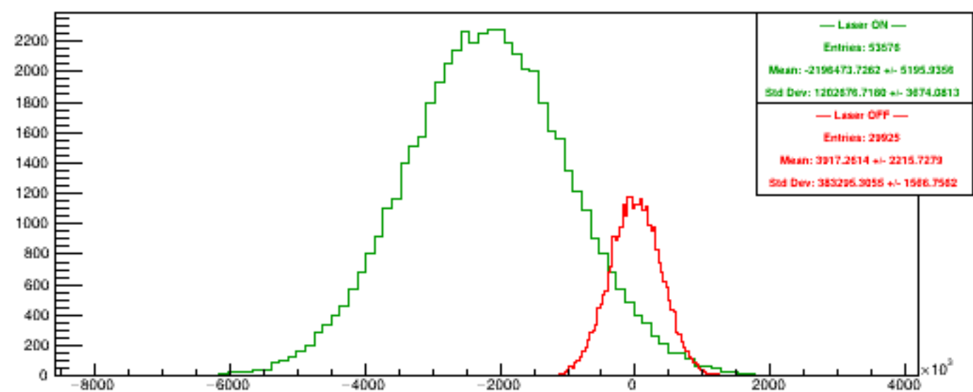
Run 5554 quartetwise, Diffs4
