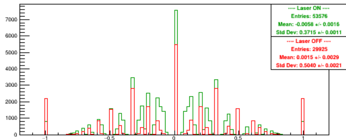
Run 5554 quartetwise, Asyms Horiz Finger
