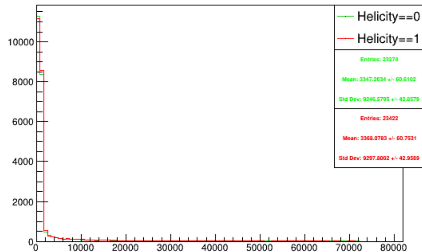
Run 5556 triggerwise, sums: Beam ON, Laser OFF
