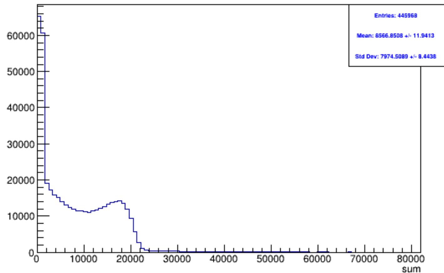
Run 5556 triggerwise, sums: All
