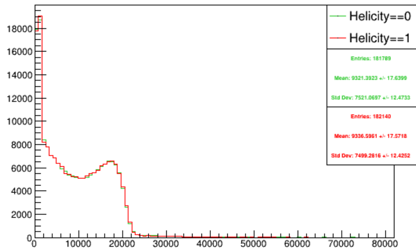
Run 5556 triggerwise, sums: Beam ON, Laser ON
