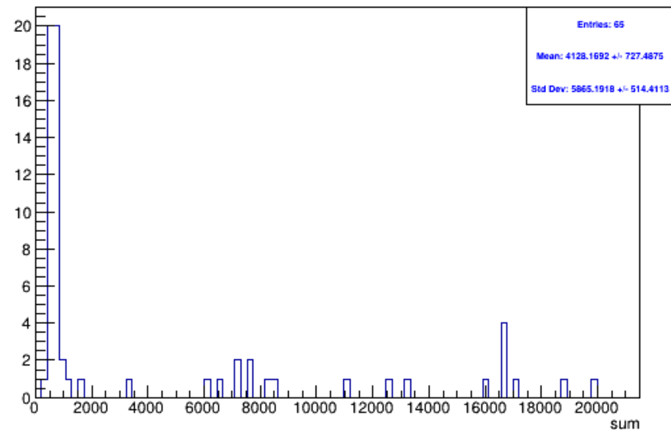
Run 5556 triggerwise, sums: Beam OFF
