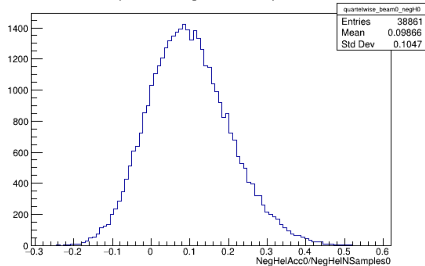
Run 5558 quartetwise, NegHelAcc0/NSamples0: Beam OFF
