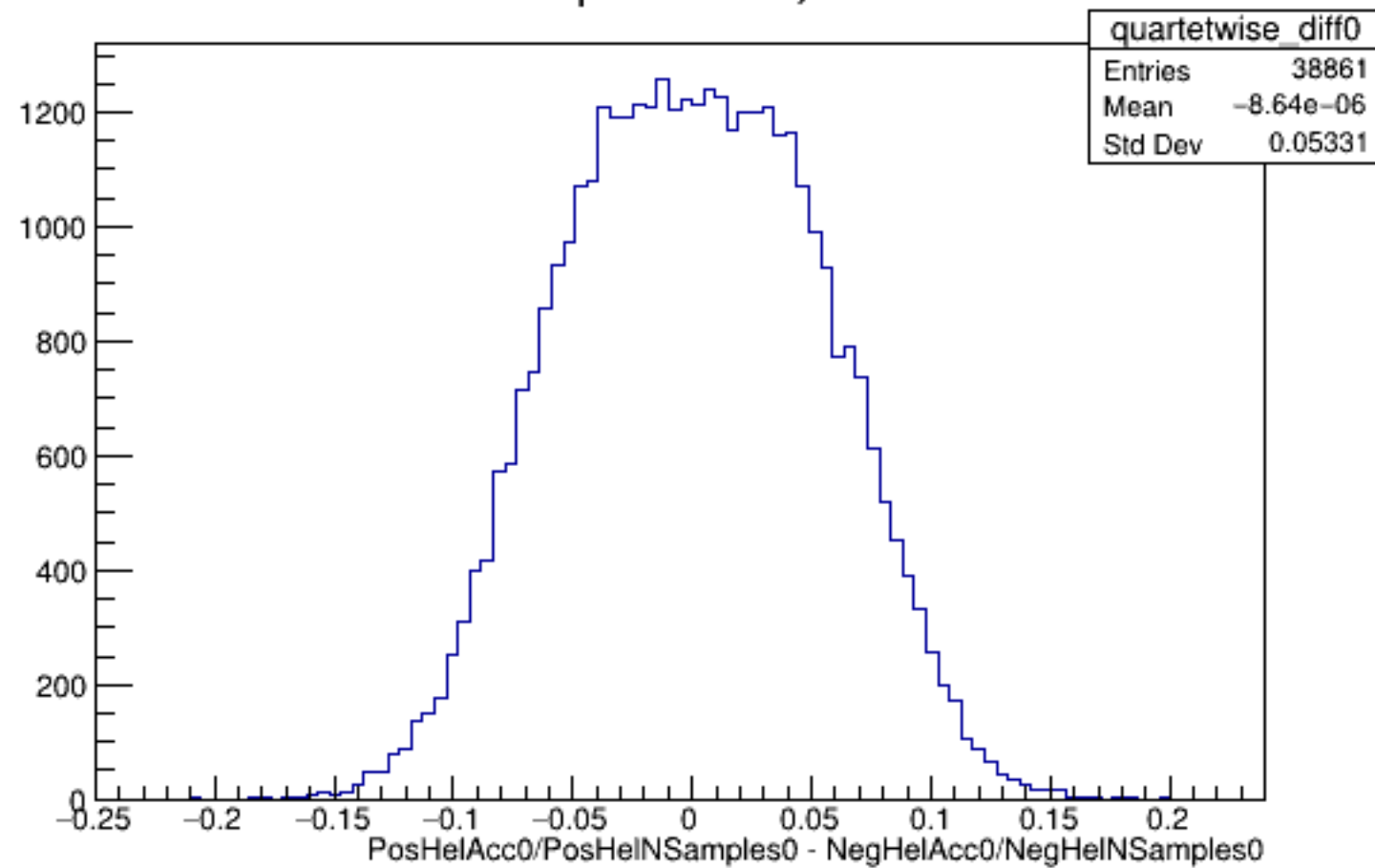
Run 5558 quartetwise, Diffs0: All
