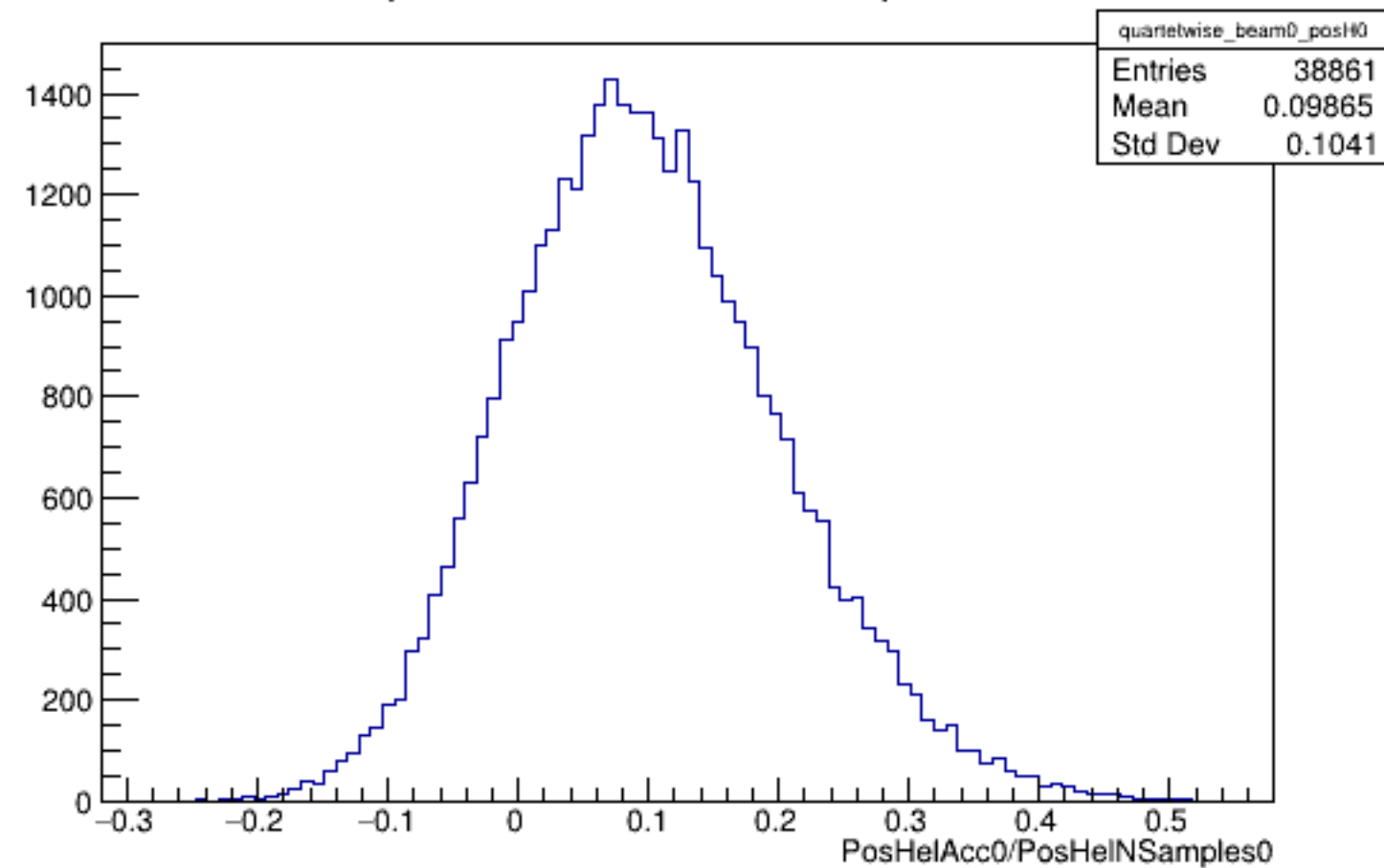
Run 5558 quartetwise, PosHelAcc0/NSamples0: Beam OFF
