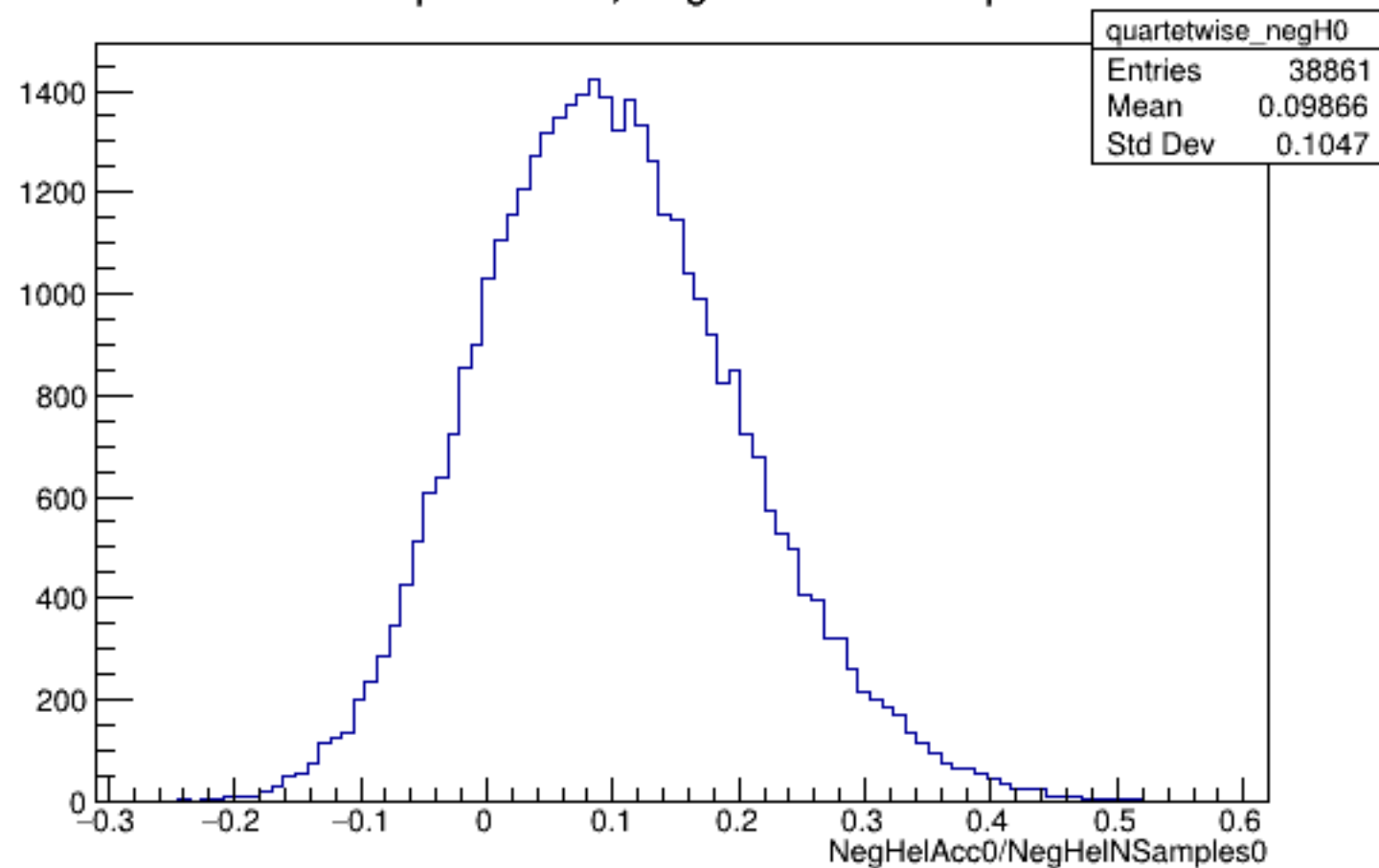
Run 5558 quartetwise, NegHelAcc0/NSamples0: All
