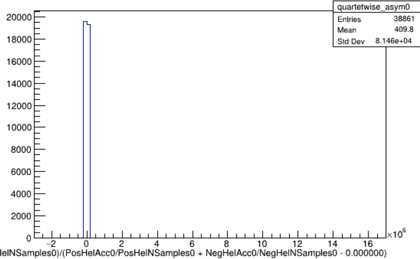
Run 5558 quartetwise, Asyms0 (Raw): All
