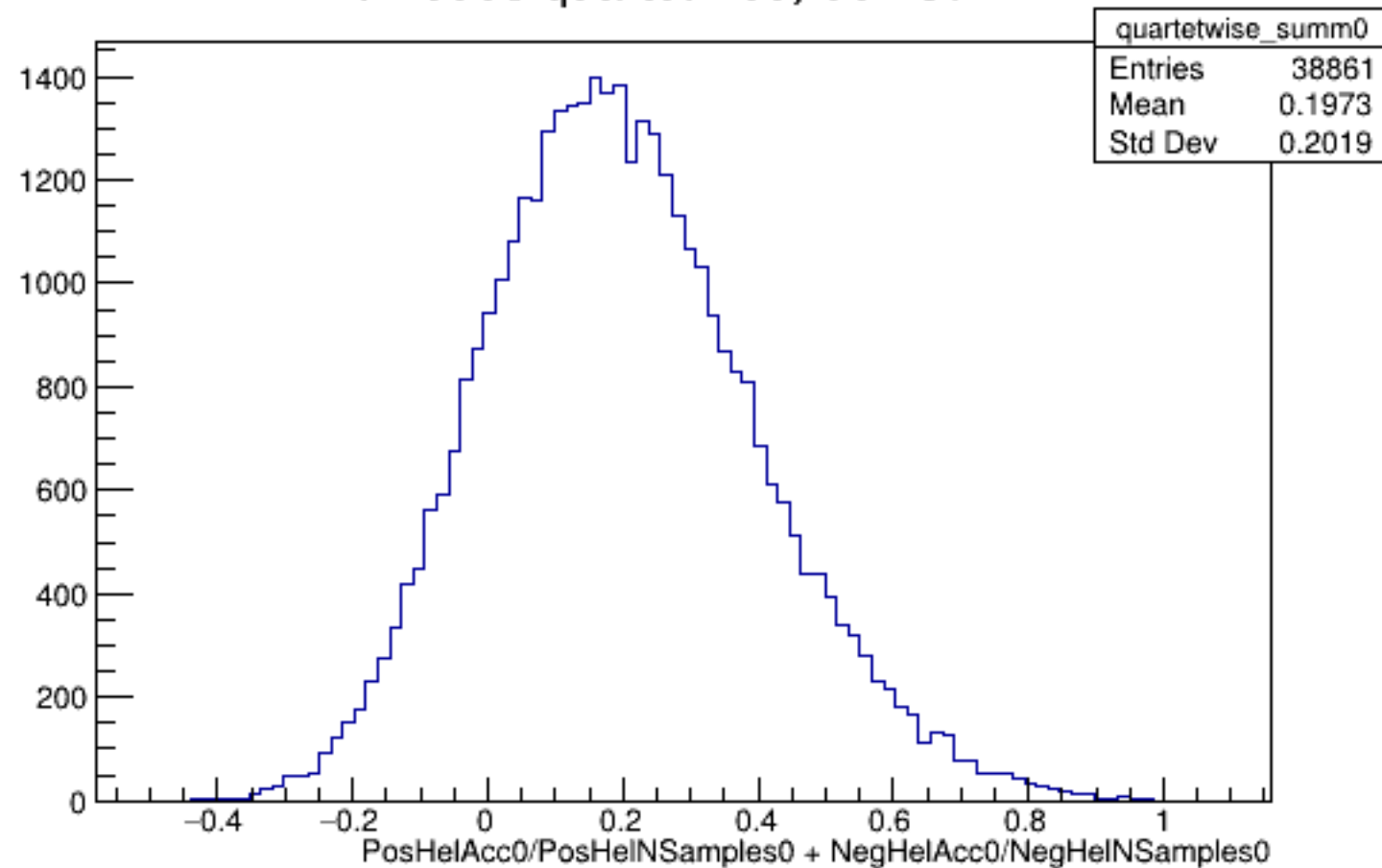
Run 5558 quartetwise, Sums0: All
