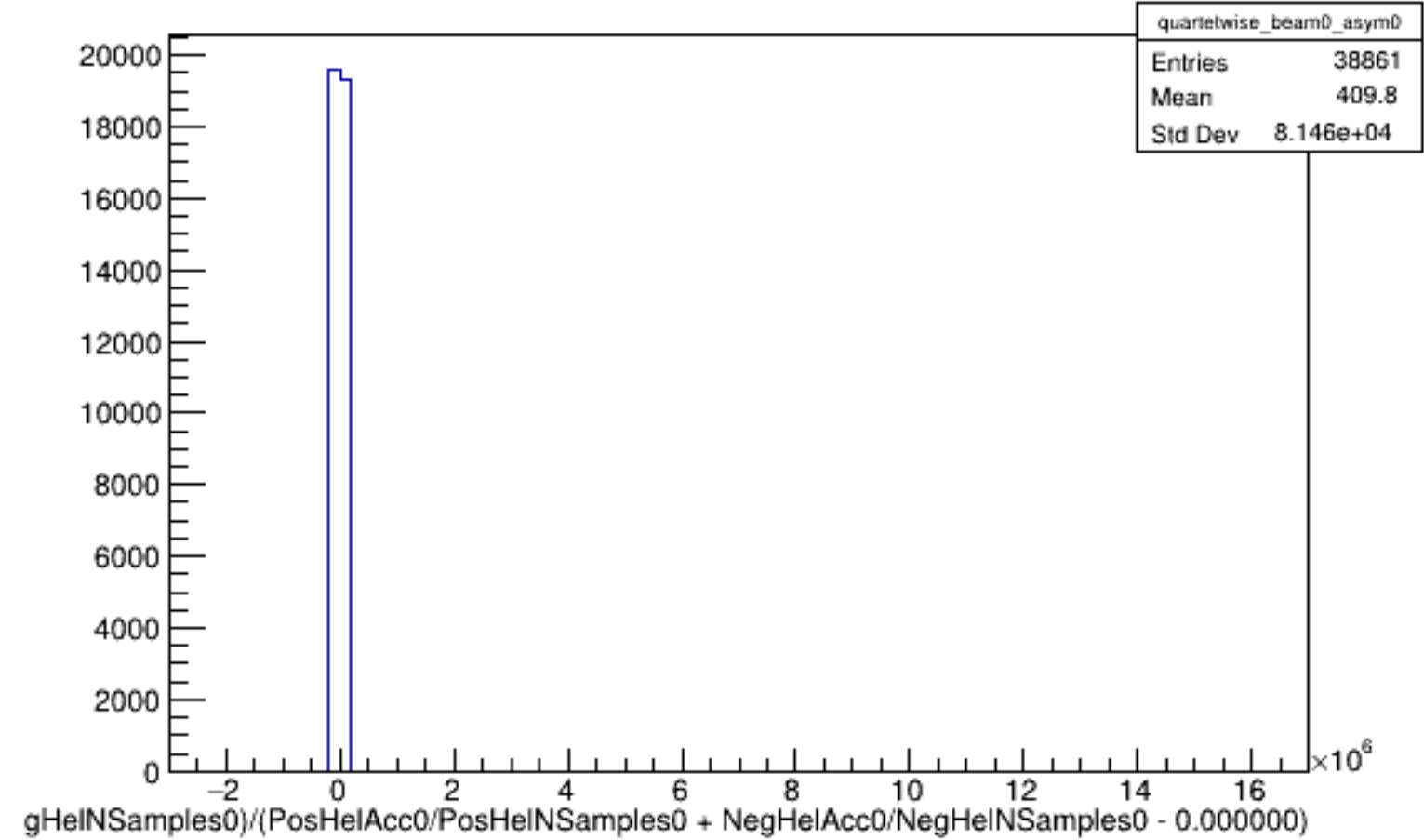
Run 5558 quartetwise, Asyms0 (Raw): Beam OFF
