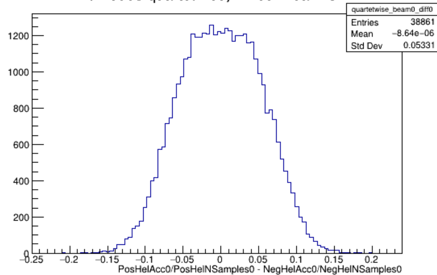
Run 5558 quartetwise, Diffs0: Beam OFF
