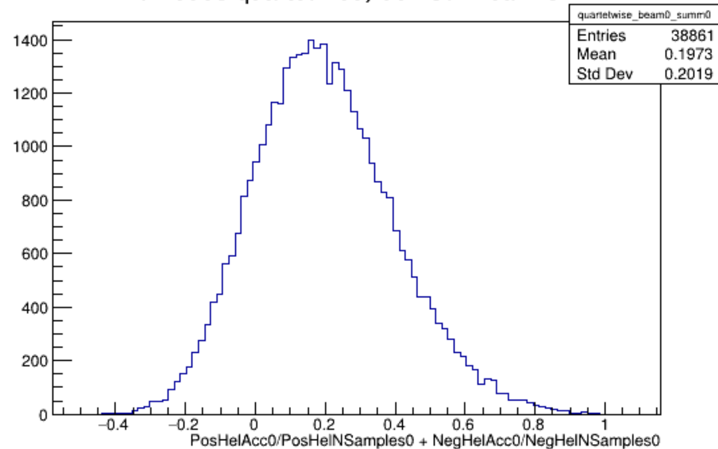
Run 5558 quartetwise, Sums0: Beam OFF
