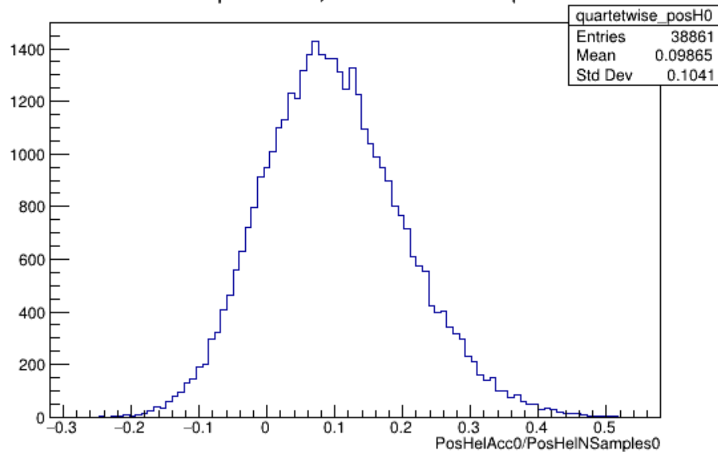
Run 5558 quartetwise, PosHelAcc0/NSamples0: All
