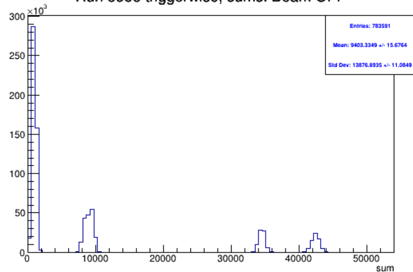
Run 5558 triggerwise, sums: Beam OFF
