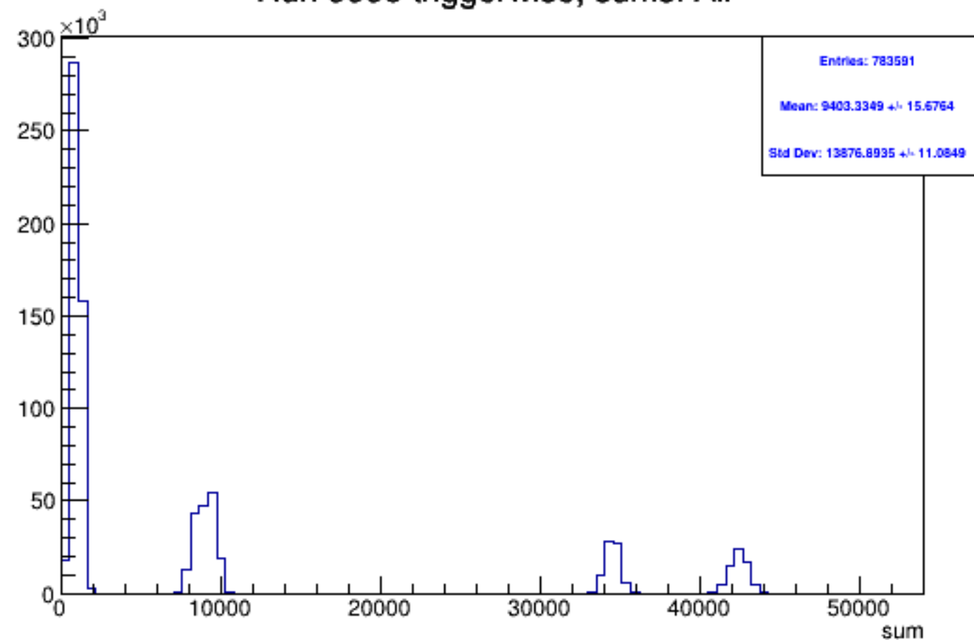
Run 5558 triggerwise, sums: All
