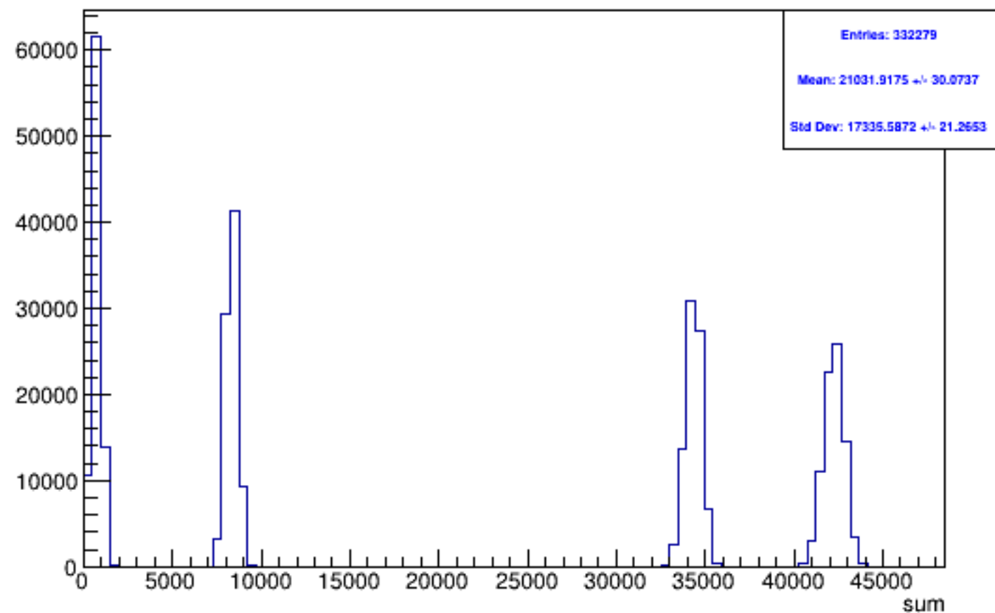
Run 5559 triggerwise, sums: All
