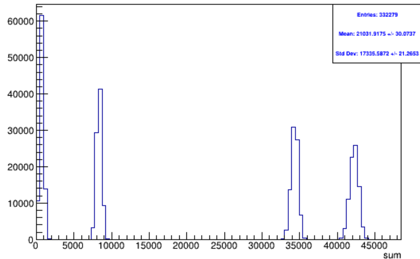
Run 5559 triggerwise, sums: Beam OFF
