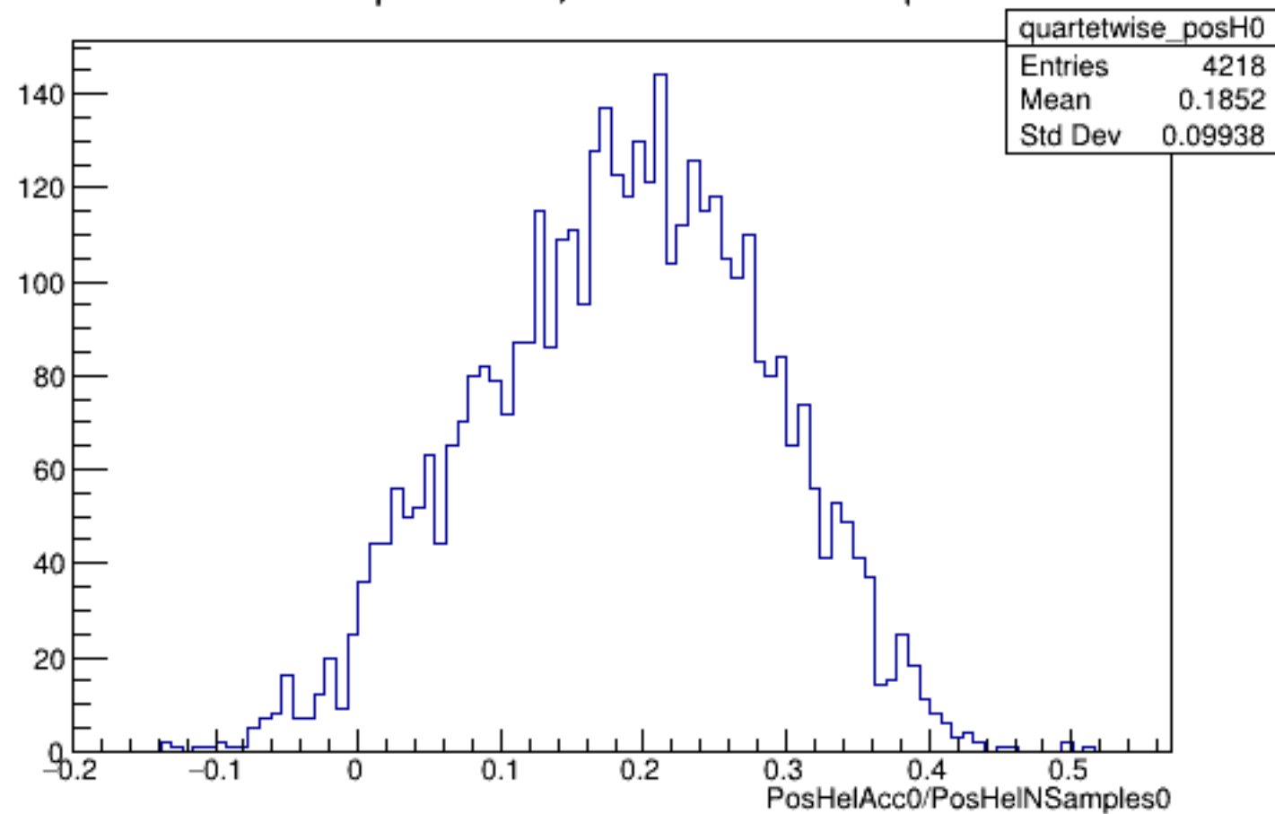
Run 5560 quartetwise, PosHelAcc0/NSamples0: All
