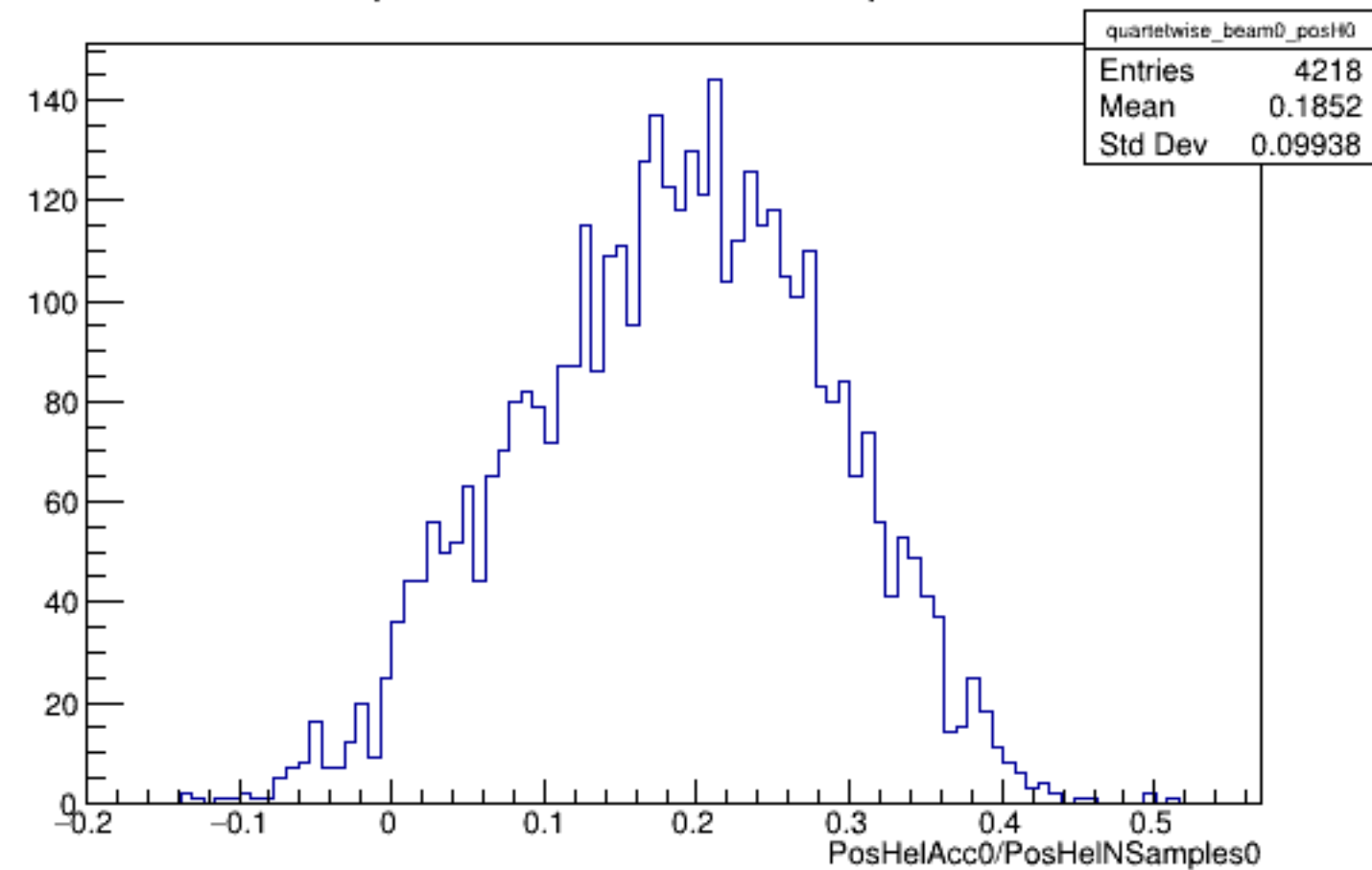
Run 5560 quartetwise, PosHelAcc0/NSamples0: Beam OFF
