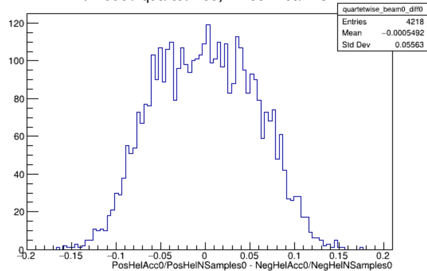
Run 5560 quartetwise, Diffs0: Beam OFF
