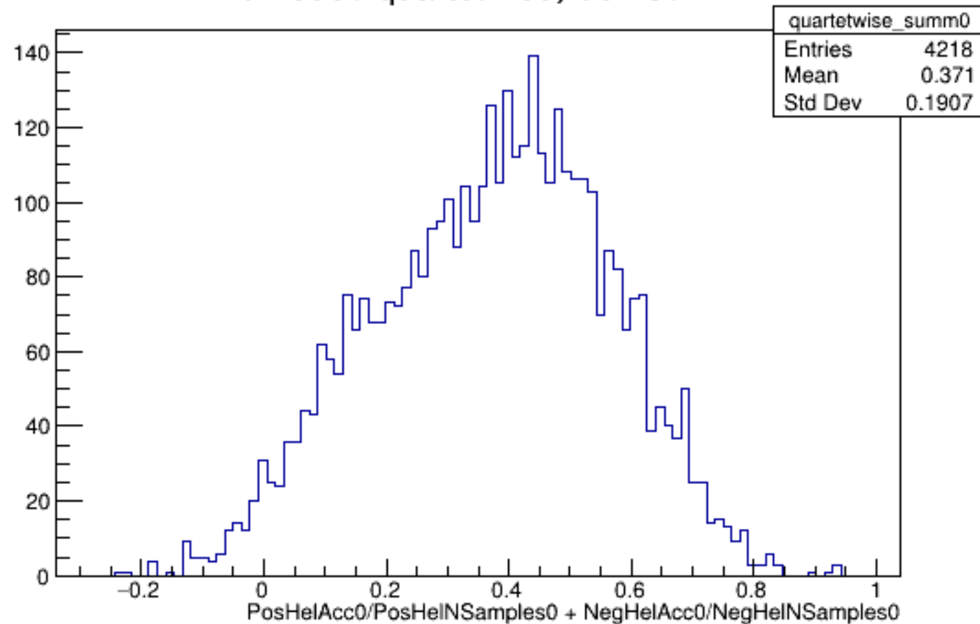
Run 5560 quartetwise, Sums0: All
