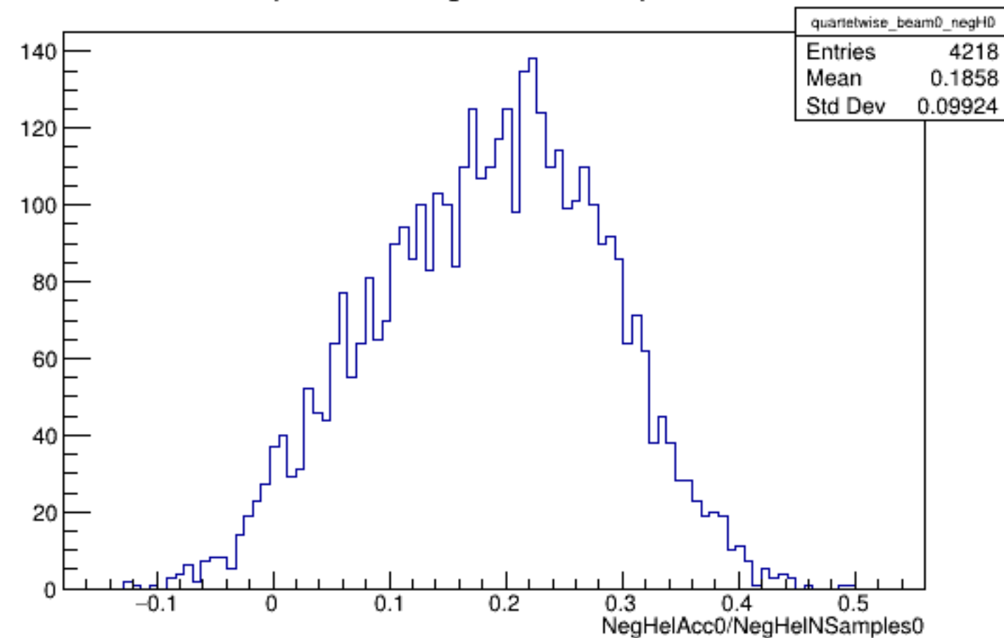
Run 5560 quartetwise, NegHelAcc0/NSamples0: Beam OFF
