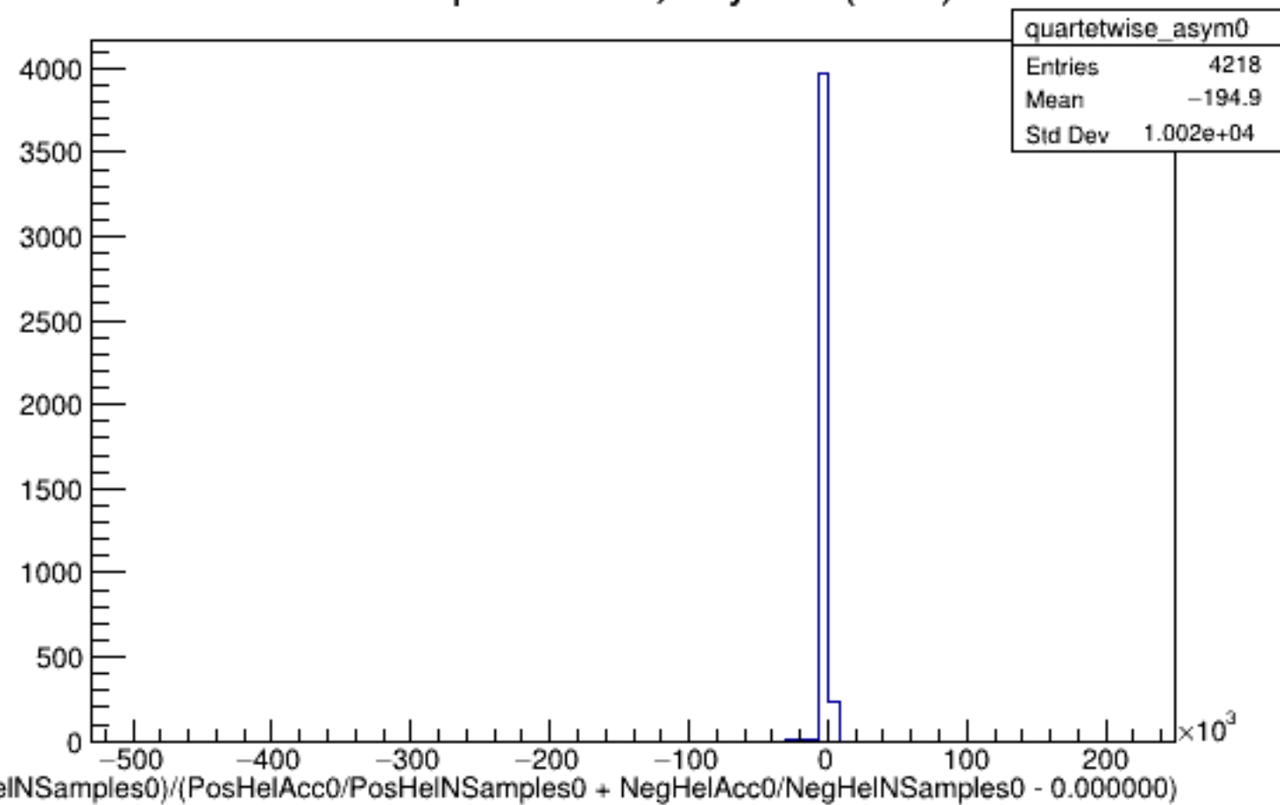
Run 5560 quartetwise, Asyms0 (Raw): All
