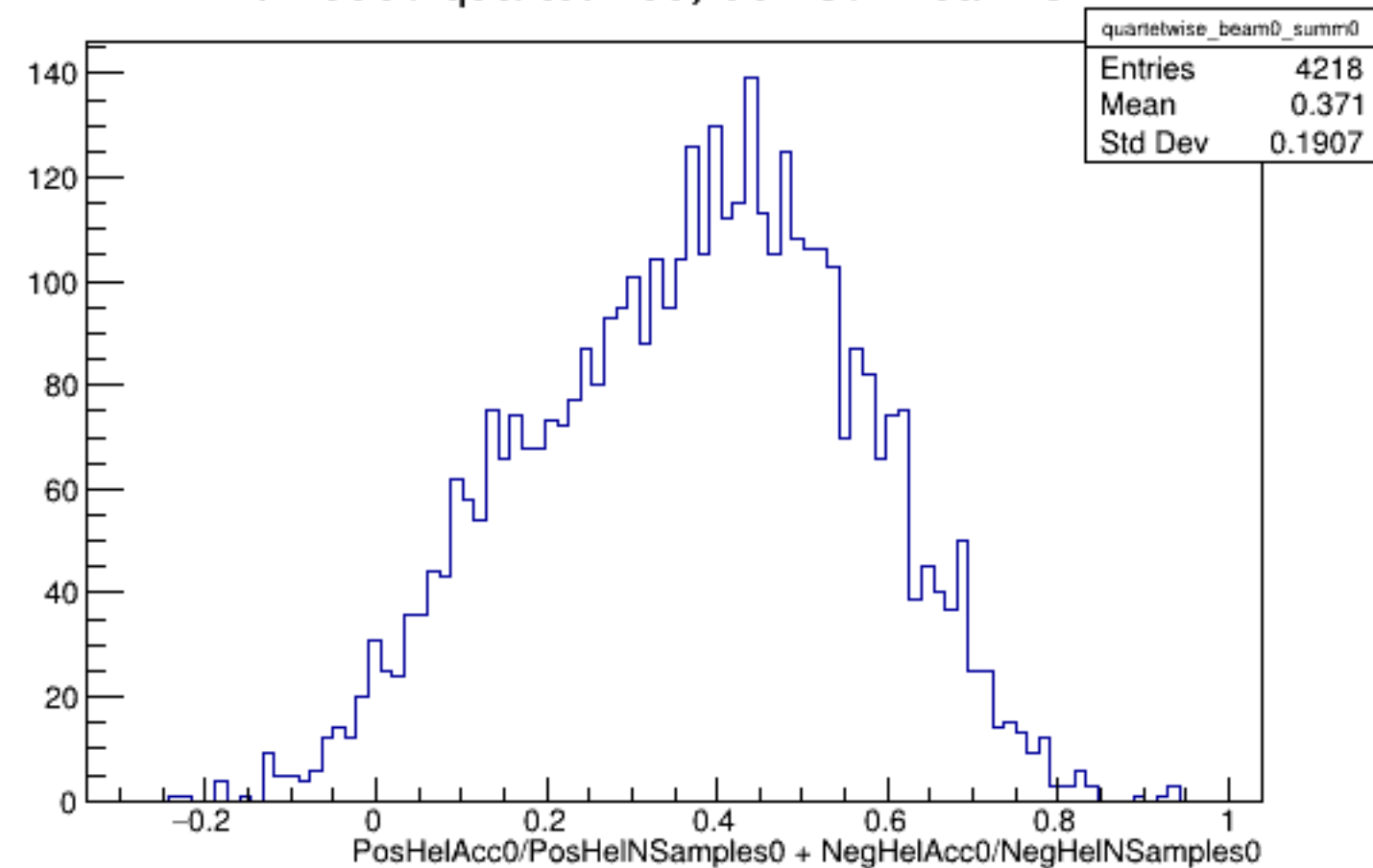
Run 5560 quartetwise, Sums0: Beam OFF
