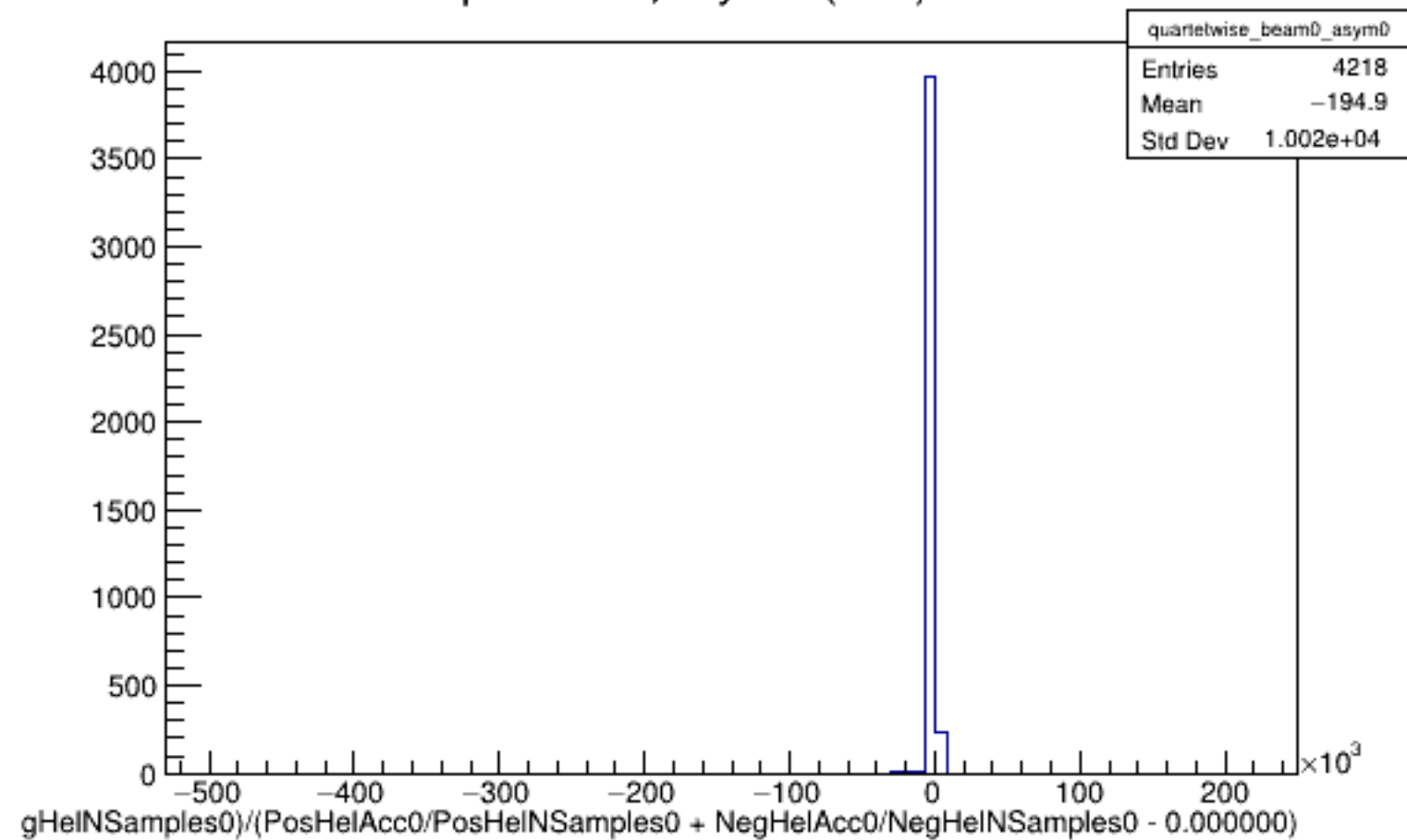
Run 5560 quartetwise, Asyms0 (Raw): Beam OFF
