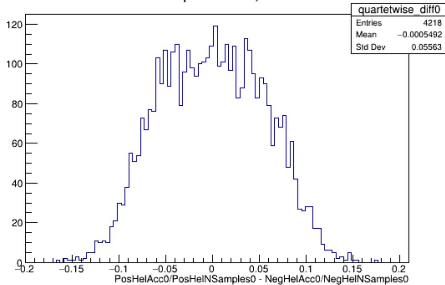
Run 5560 quartetwise, Diffs0: All
