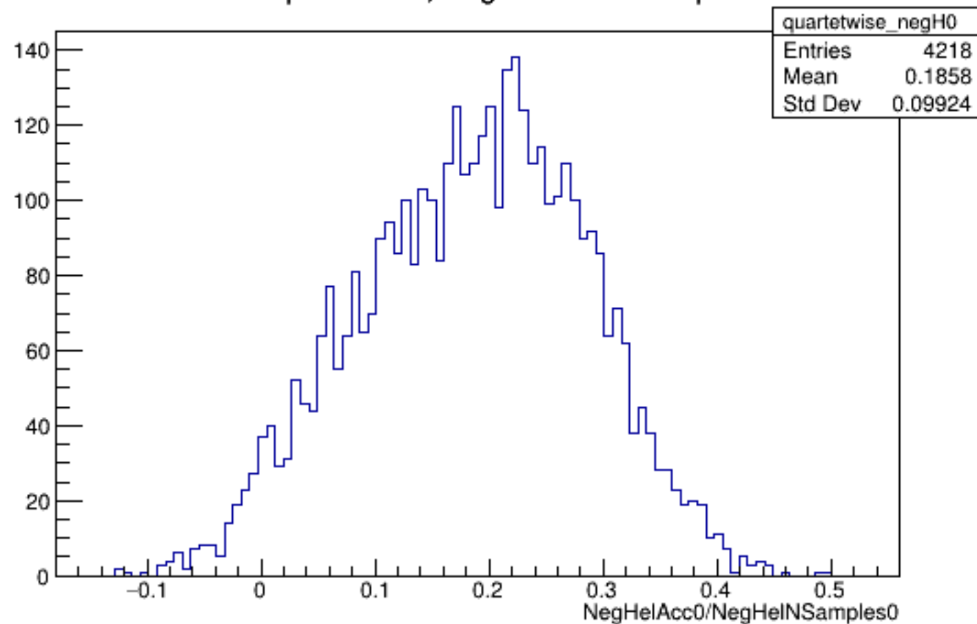
Run 5560 quartetwise, NegHelAcc0/NSamples0: All
