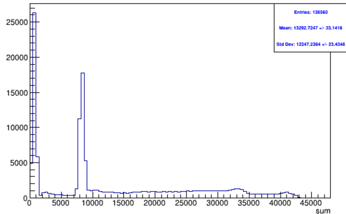
Run 5560 triggerwise, sums: Beam OFF
