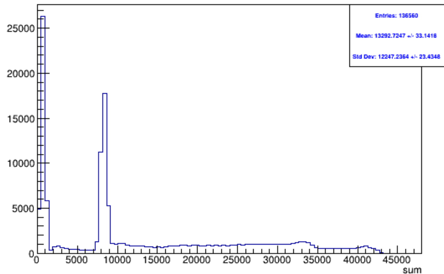
Run 5560 triggerwise, sums: All
