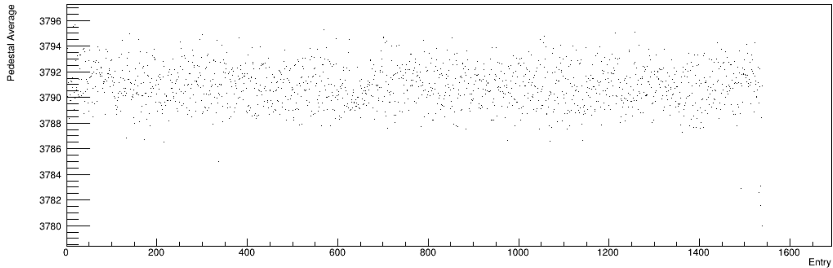
Run 5561, snapshots: Pedestal vs. Time
