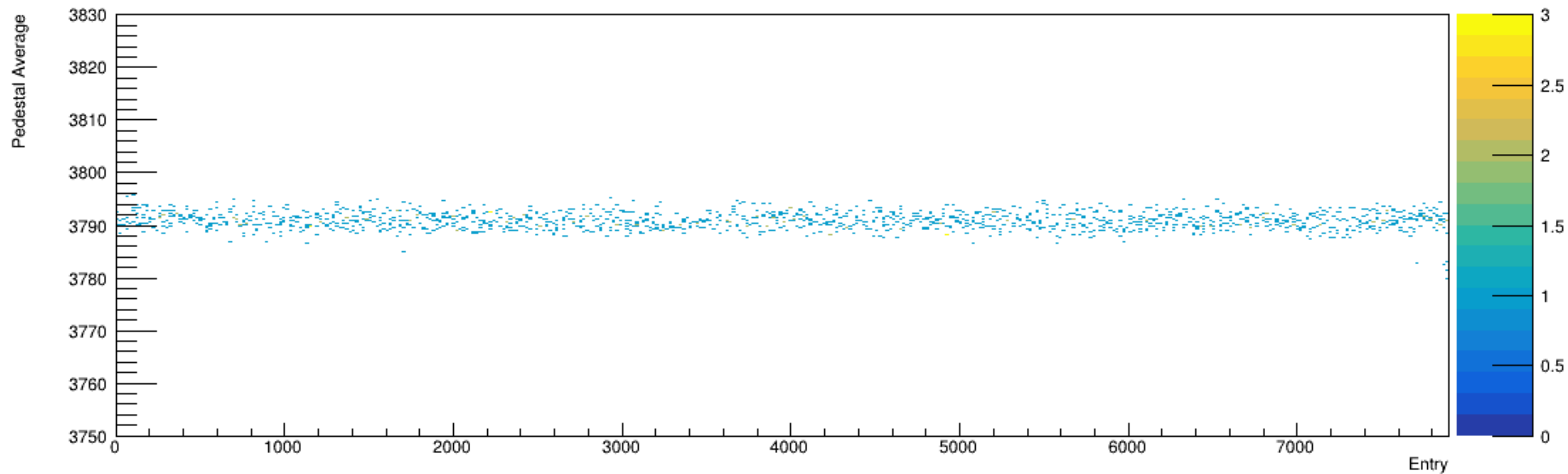
Run 5561, snapshots: Pedestal vs. Time
