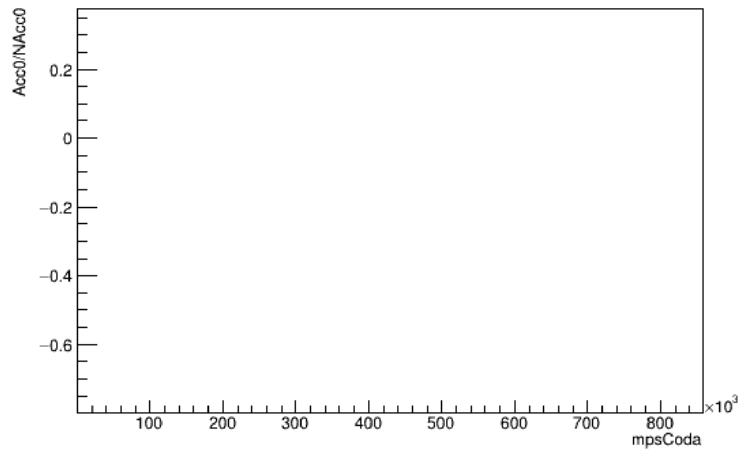
Run 5565 mpwise, Acc0 vs Time: Beam ON, Laser OFF
