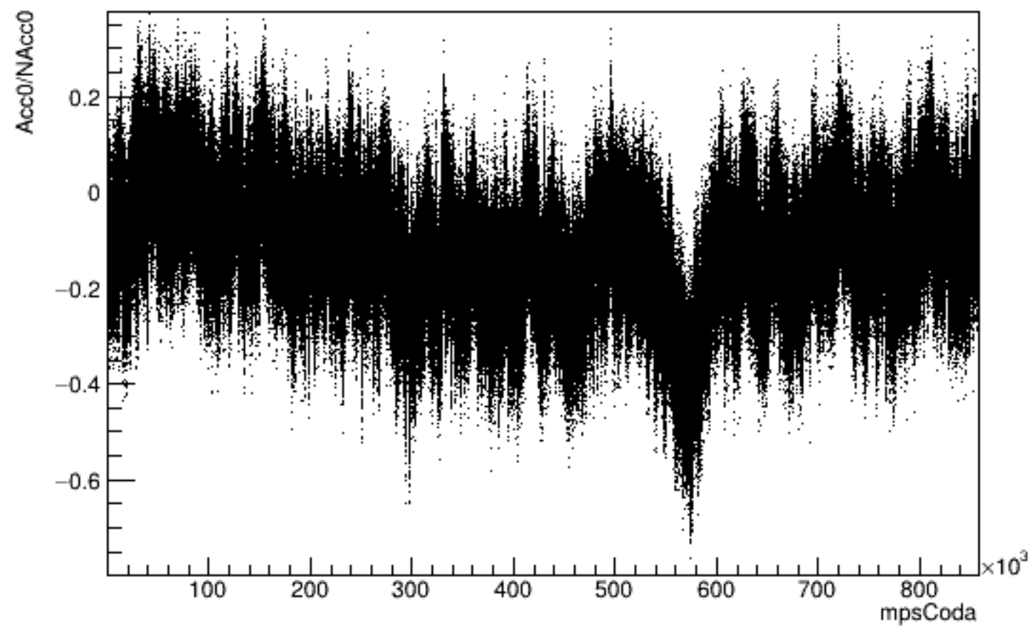
Run 5565 mpwise, Acc0 vs Time: All
