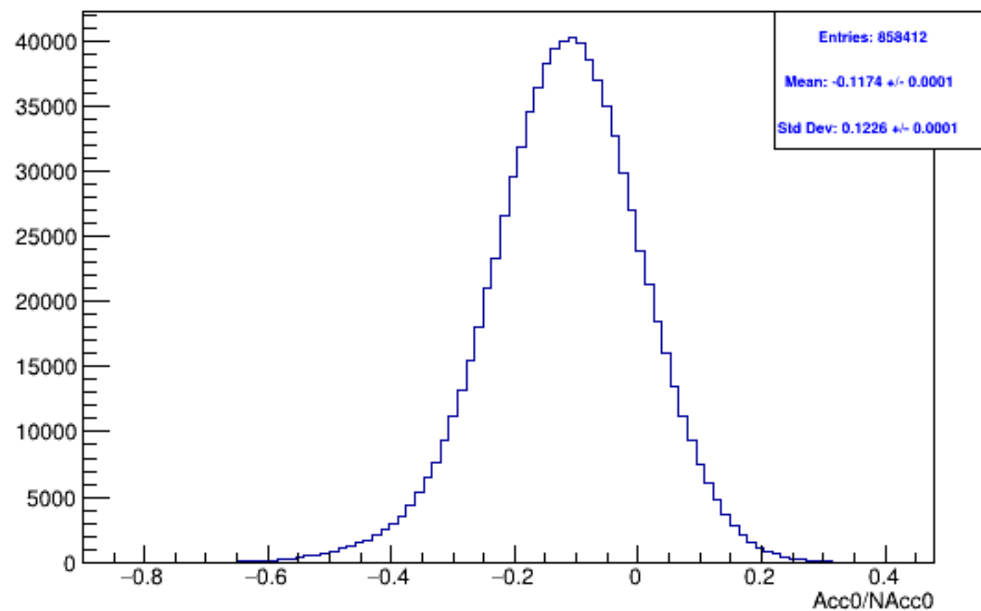
Run 5565 mpwise, acc0: All
