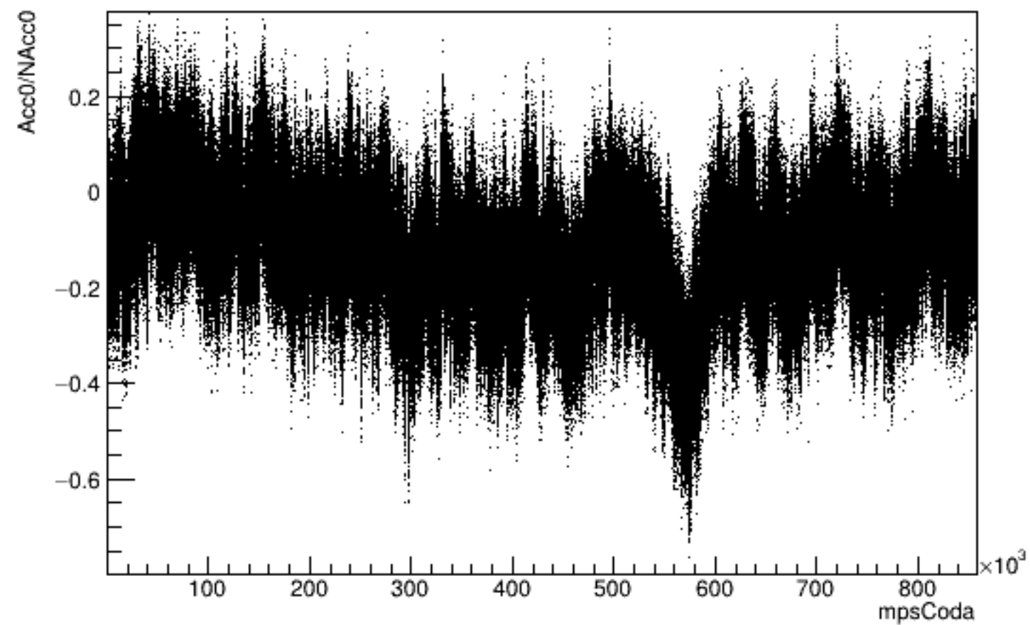
Run 5565 mpwise, Acc0 vs Time: Beam OFF
