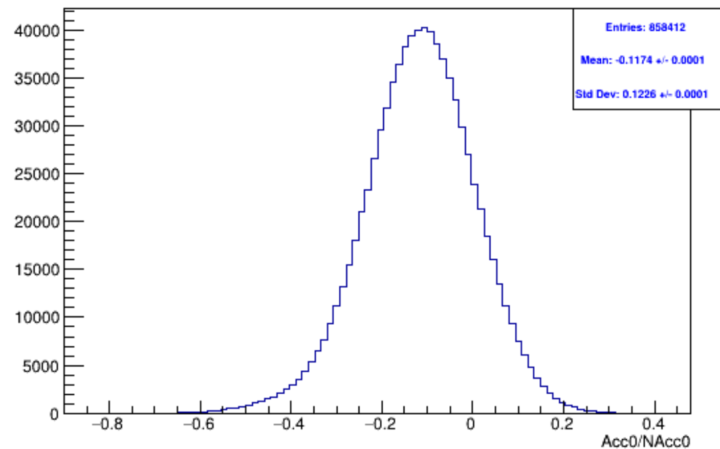
Run 5565 mpwise, acc0: Beam OFF
