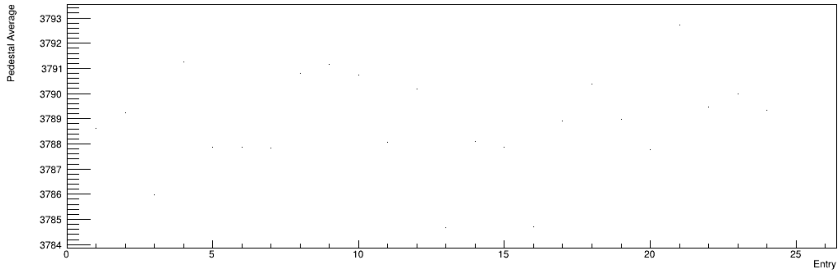
Run 5566, snapshots: Pedestal vs. Time
