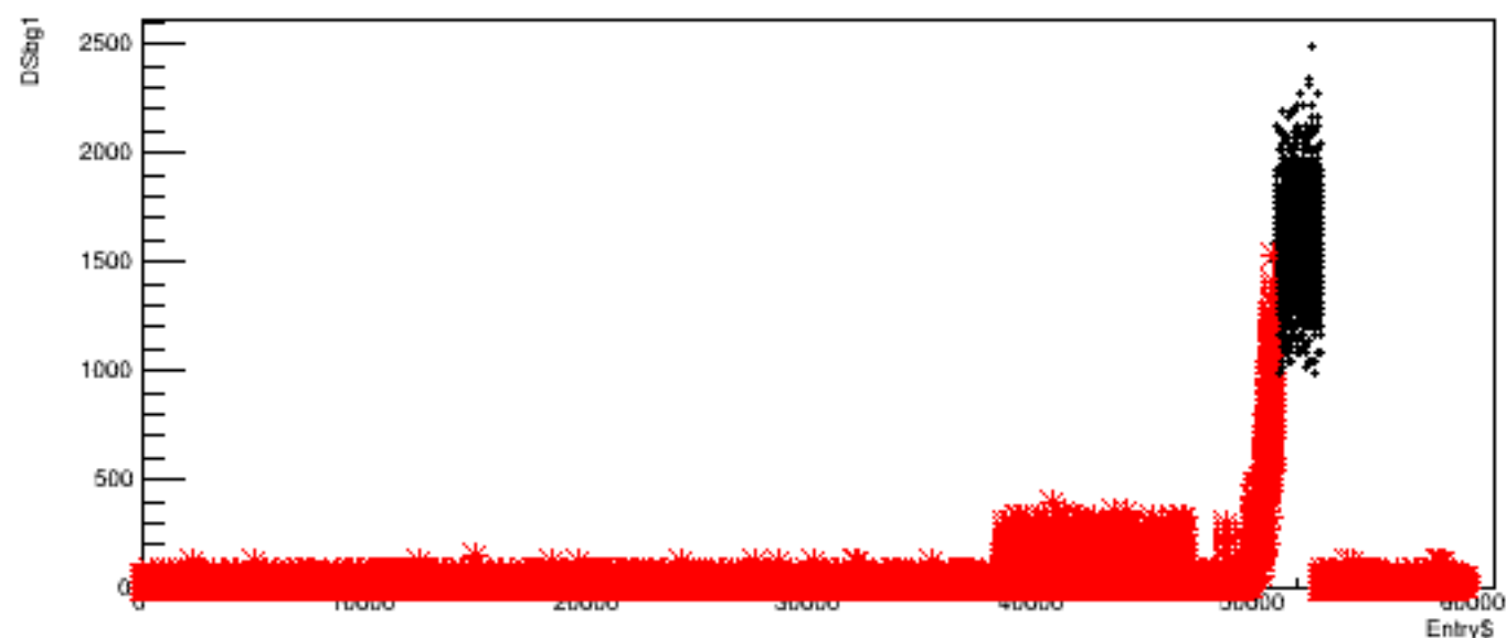
Run 5569, quartetwise: DSbg1 vs time
