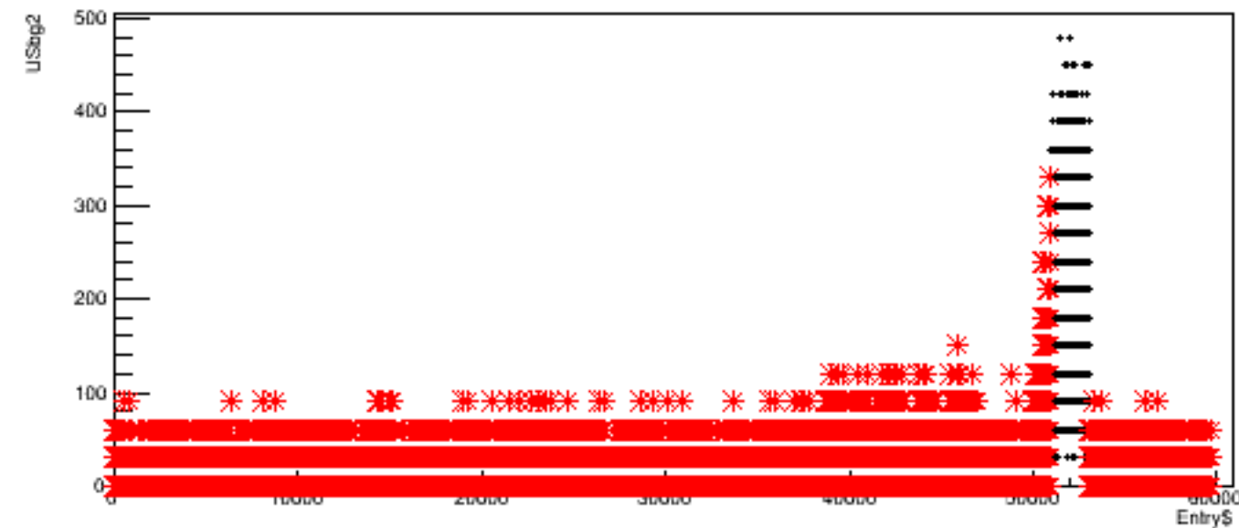
Run 5569, quartetwise: USbg2 vs time
