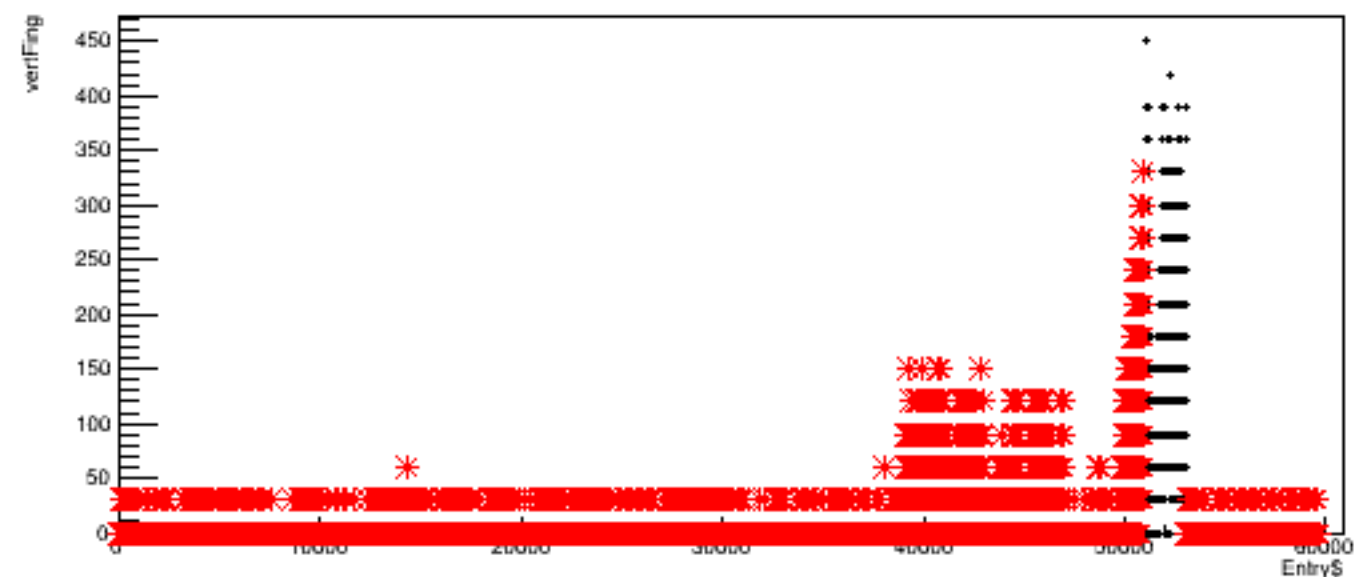
Run 5569, quartetwise: vertFing vs time
