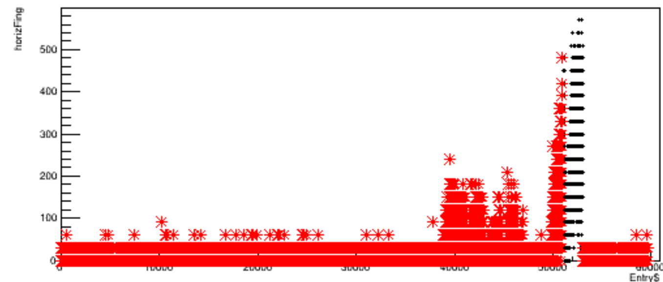
Run 5569, quartetwise: horizFing vs time
