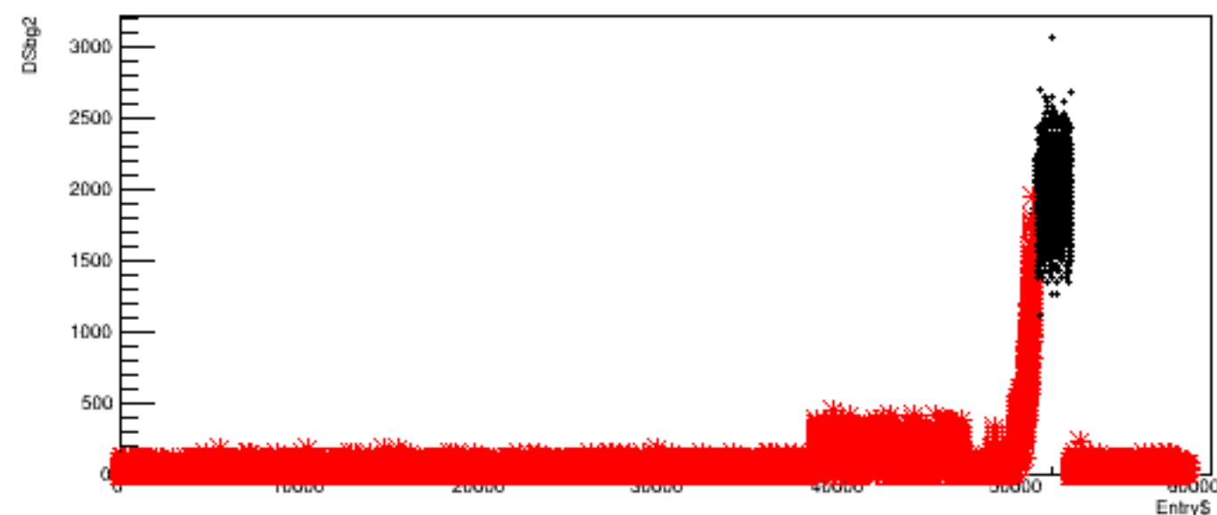
Run 5569, quartetwise: DSbg2 vs time
