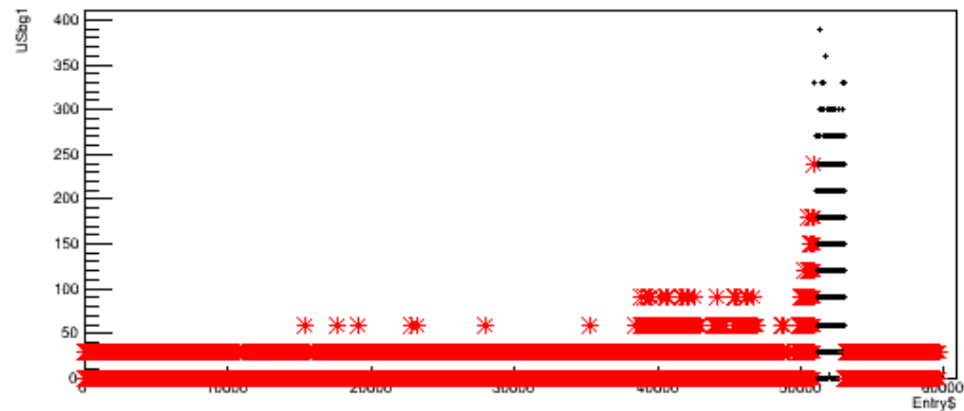
Run 5569, quartetwise: USbg1 vs time
