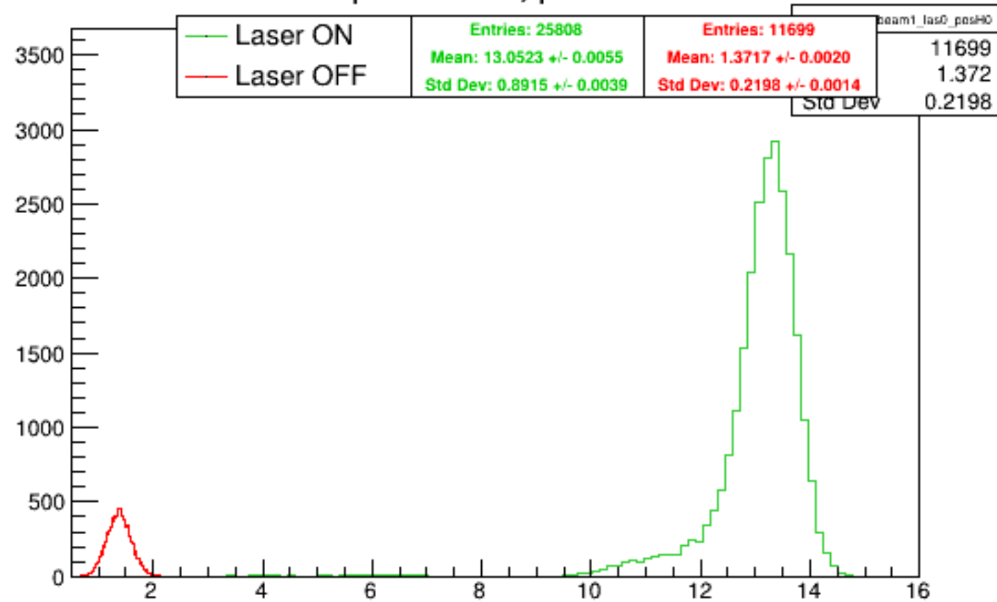
Run 5570 quartetwise, posH0: Beam ON
