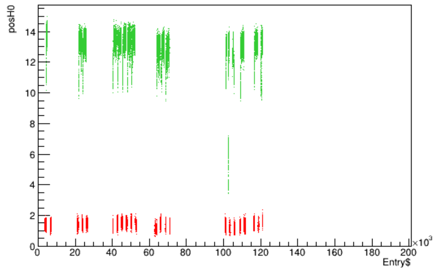
Run 5570 quartetwise, posH0 vs time
