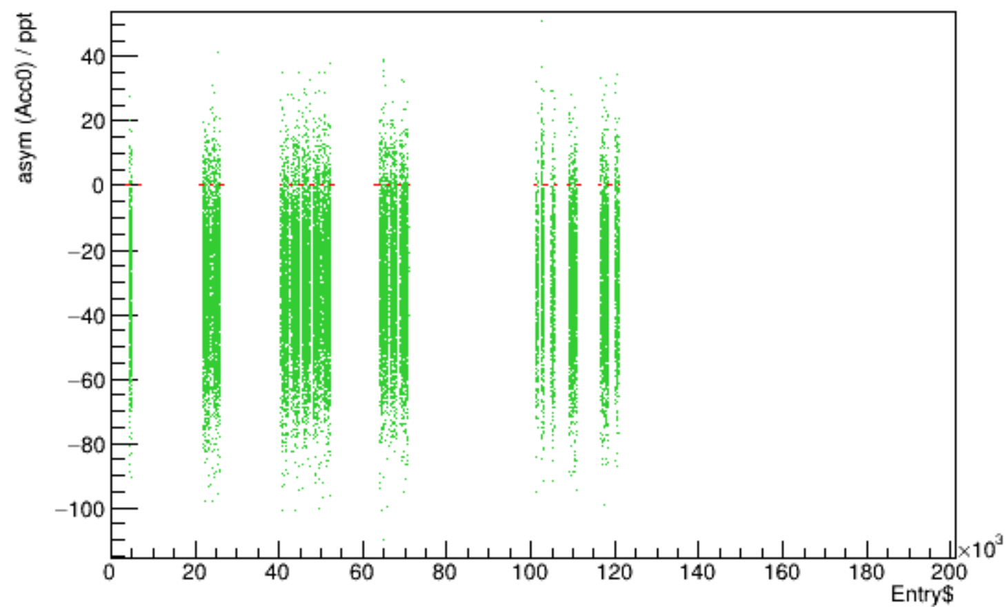
Run 5570 quartetwise, asym0sub vs time
