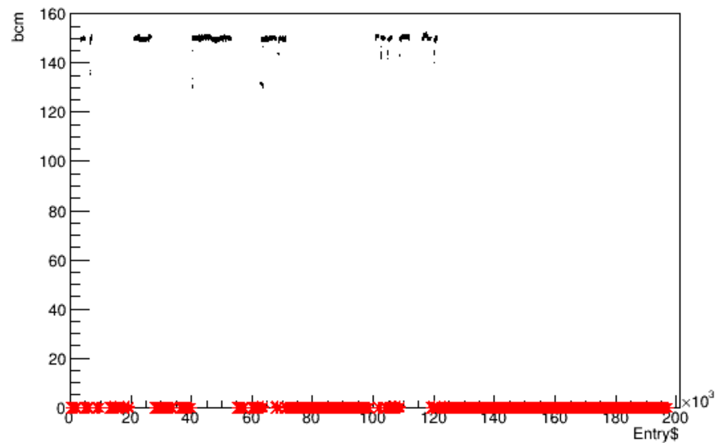
Run 5570 quartetwise, bcm vs time
