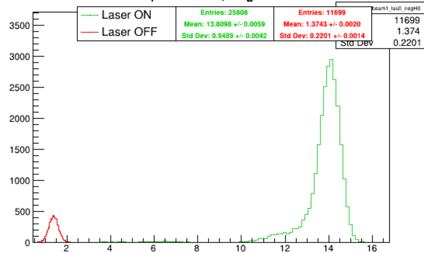
Run 5570 quartetwise, negH0: Beam ON
