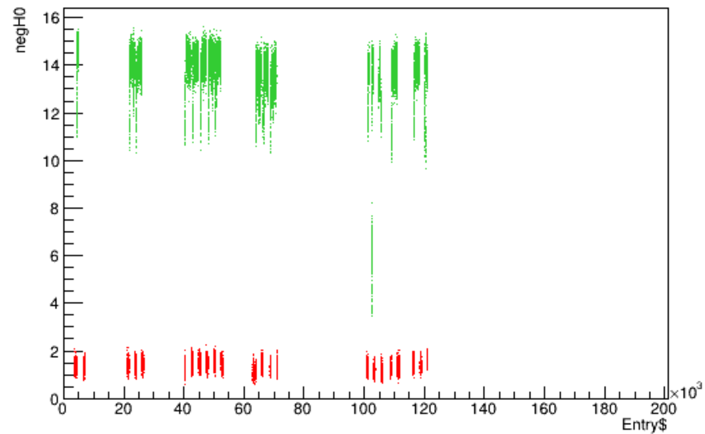
Run 5570 quartetwise, negH0 vs time
