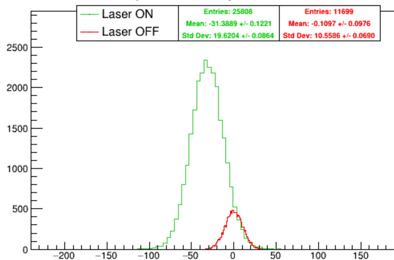
Run 5570 quartetwise, asym0sub: Beam ON
