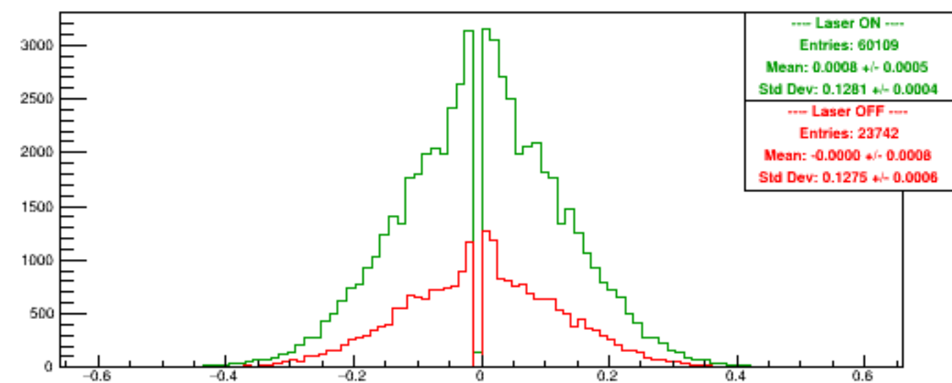
Run 5574 quartetwise, Asyms DSbg1
