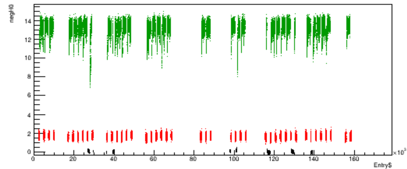
Run 5574 quartetwise, negH0 vs time
