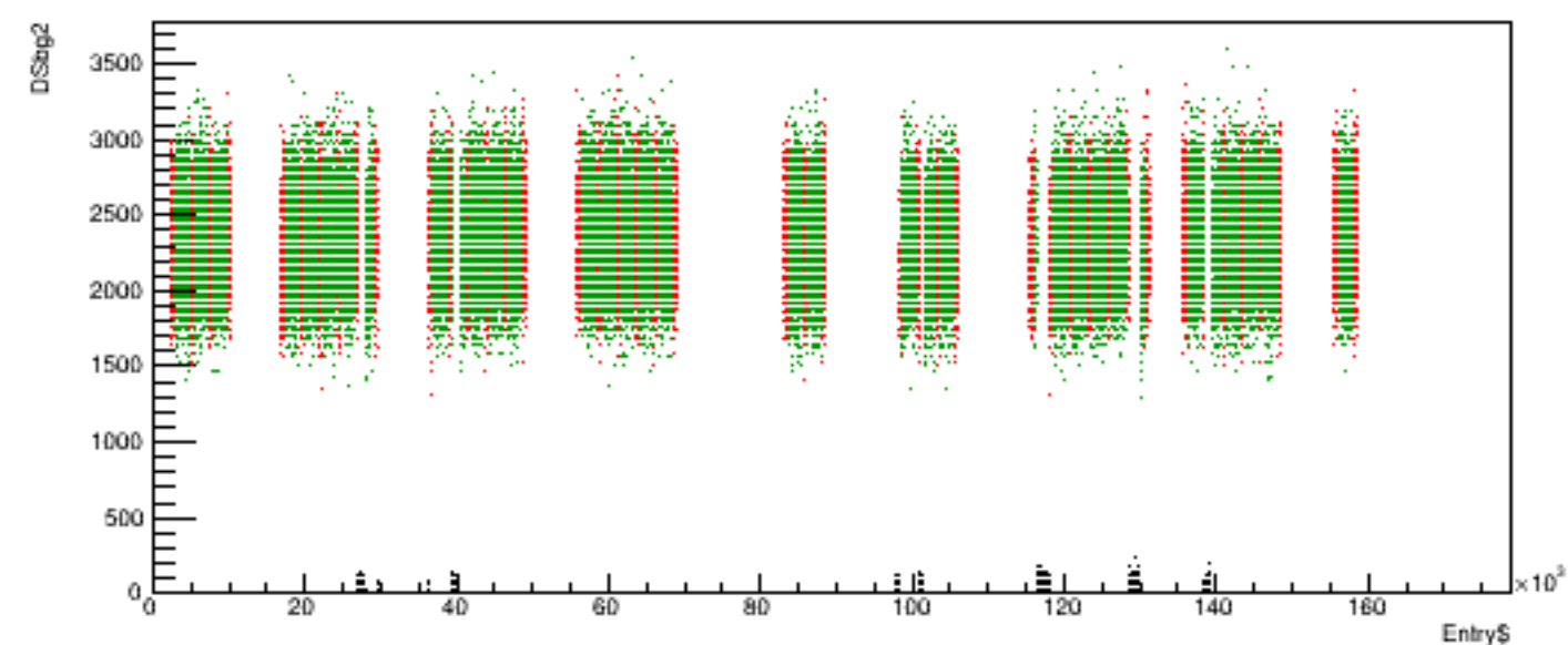
Run 5574 quartetwise, DSbg2 vs time
