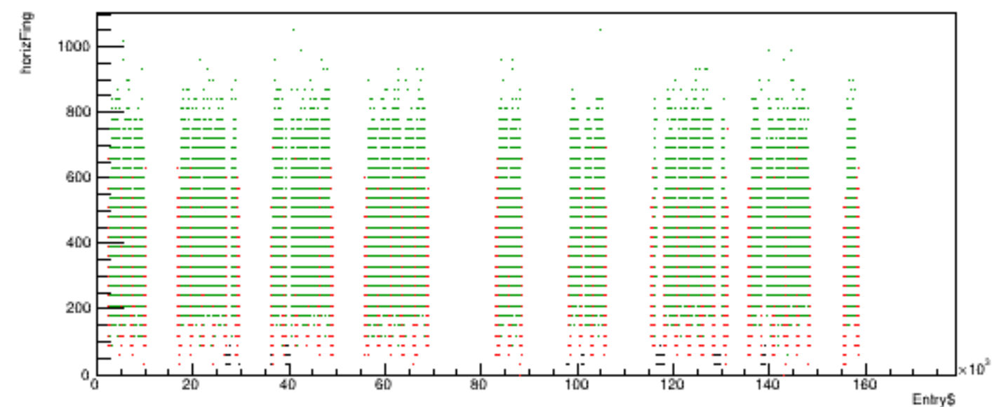
Run 5574 quartetwise, horizFing vs time
