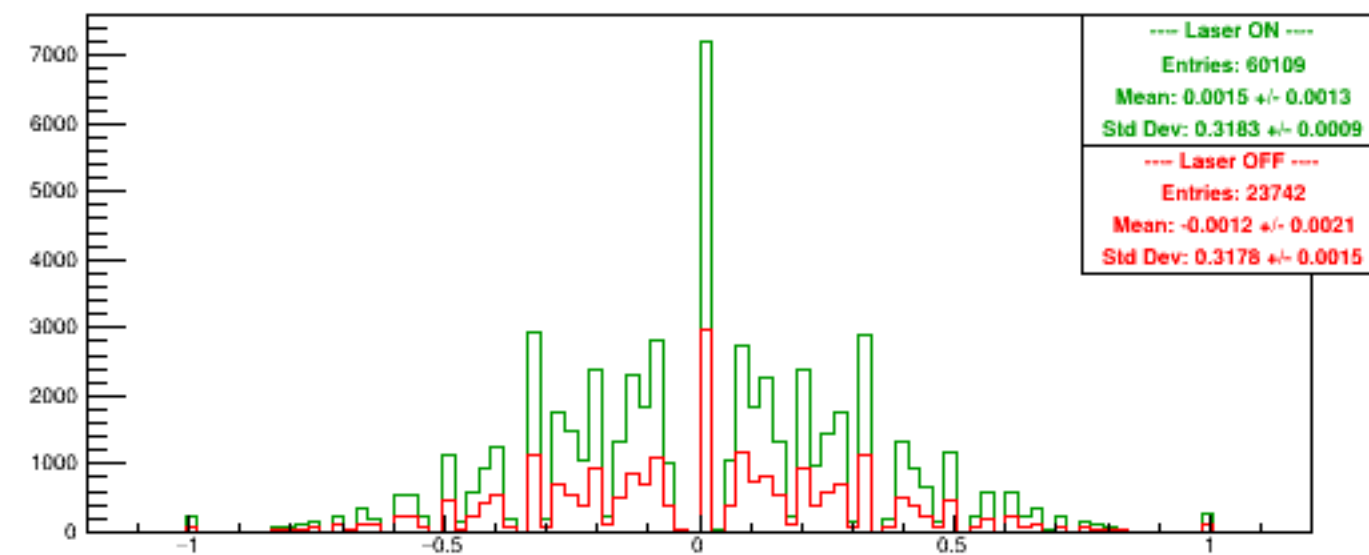
Run 5574 quartetwise, Asyms USbg2
