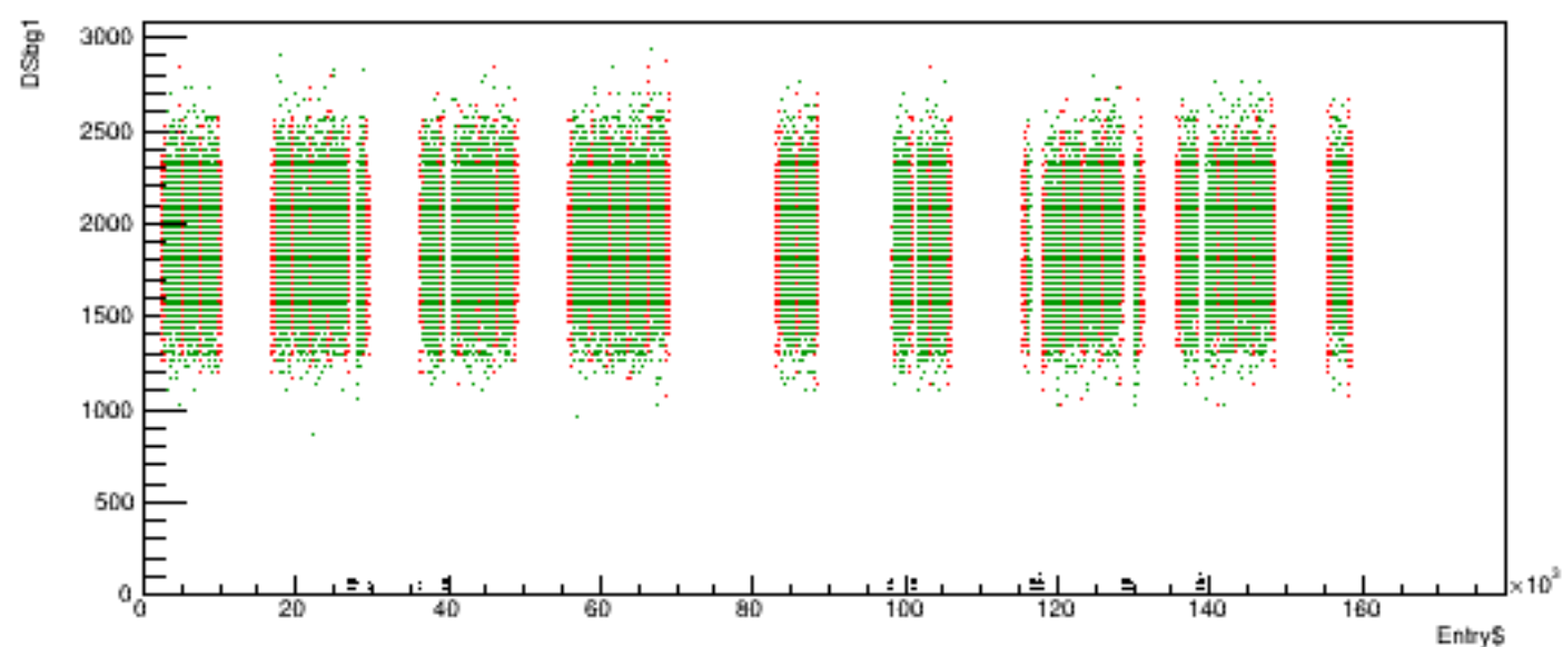
Run 5574 quartetwise, DSbg1 vs time
