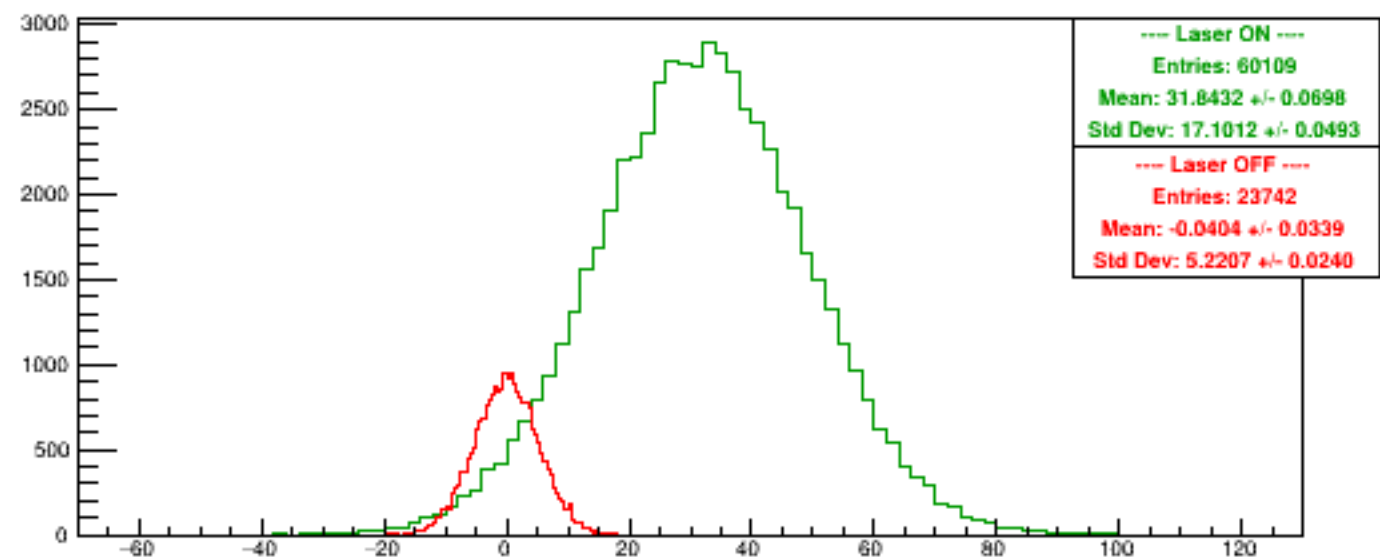
Run 5574 quartetwise, Asyms4
