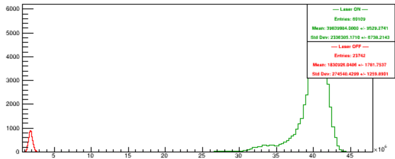
Run 5574 quartetwise, PosHelAcc4
