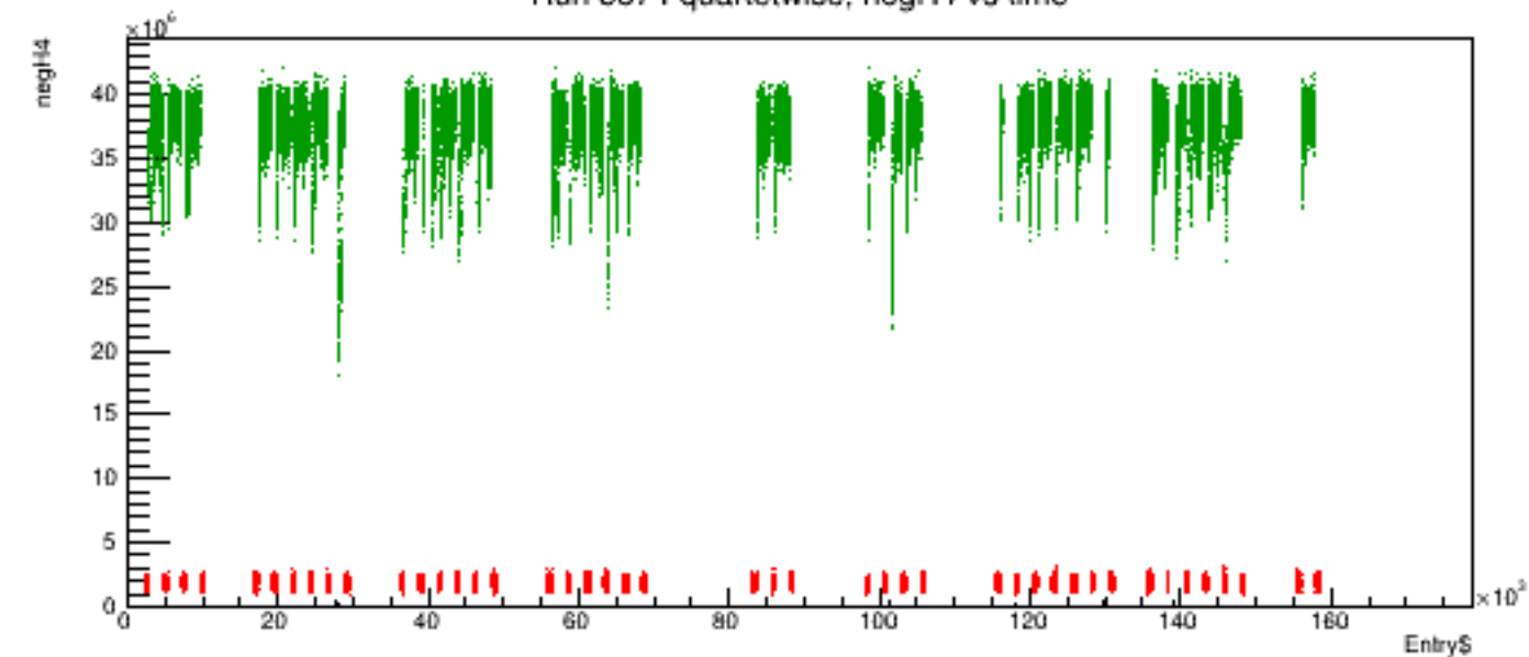
Run 5574 quartetwise, negH4 vs time
