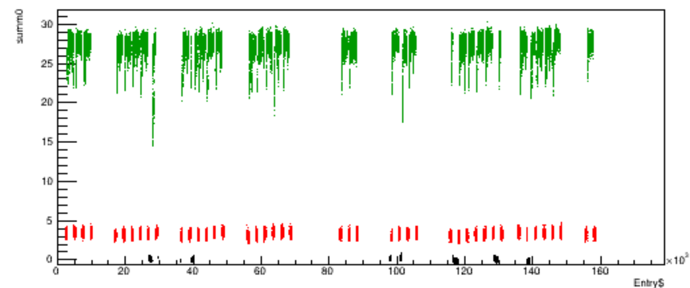
Run 5574 quartetwise, summ0 vs time
