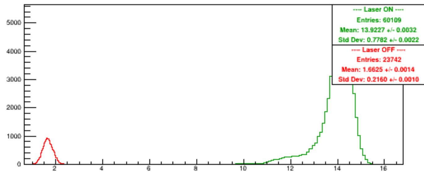
Run 5574 quartetwise, PosHelAcc0/NSamples0
