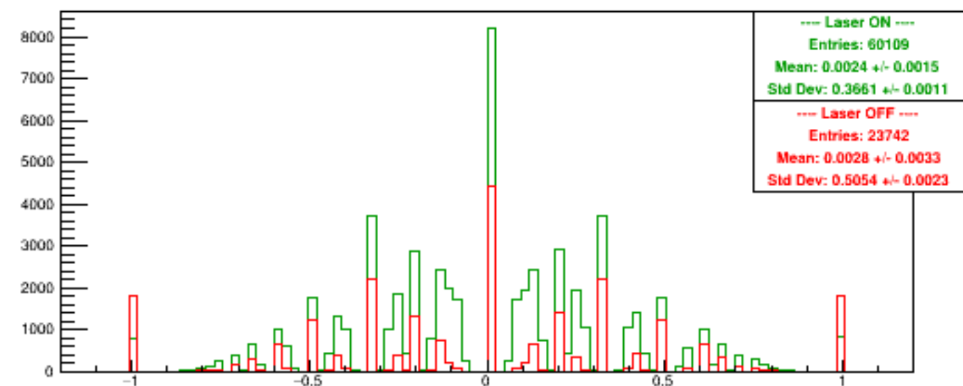
Run 5574 quartetwise, Asyms Horiz Finger
