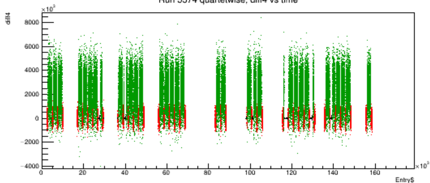
Run 5574 quartetwise, diff4 vs time
