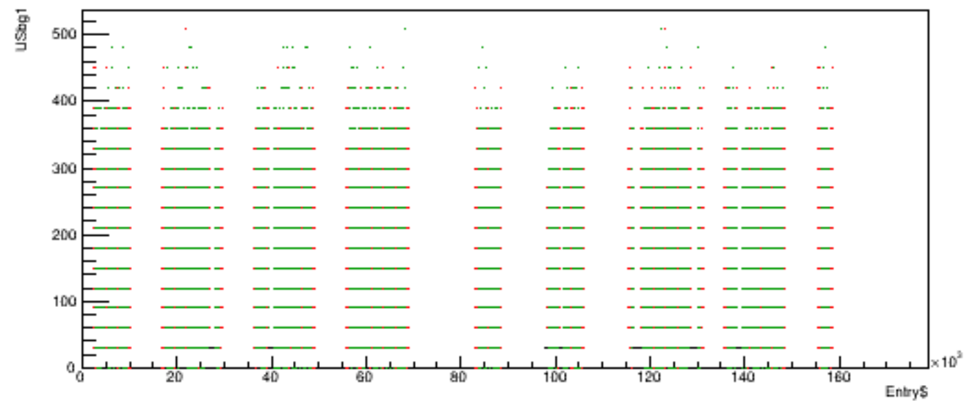
Run 5574 quartetwise, USbg1 vs time
