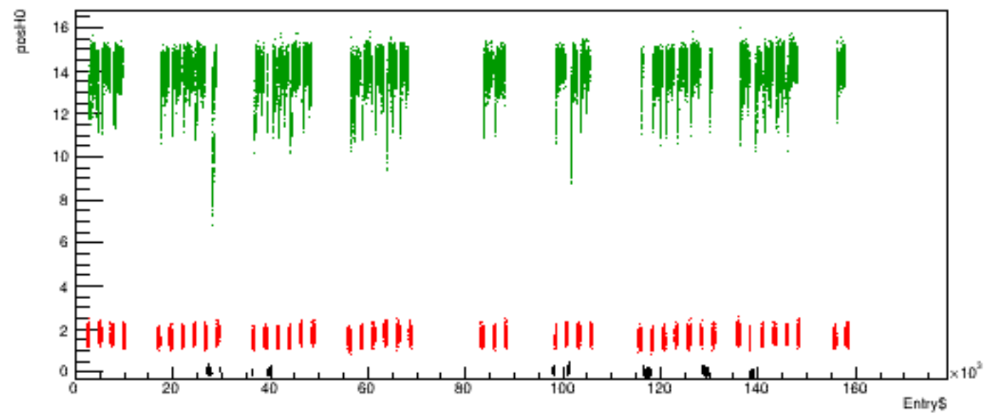
Run 5574 quartetwise, posH0 vs time
