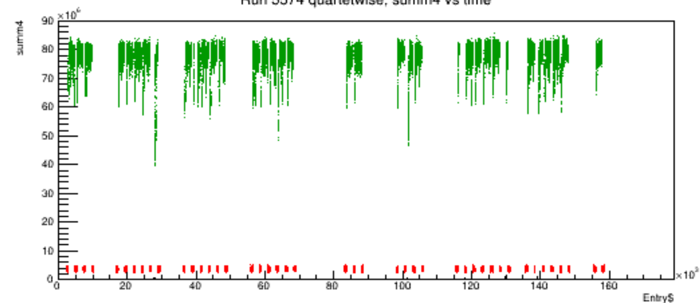
Run 5574 quartetwise, summ4 vs time
