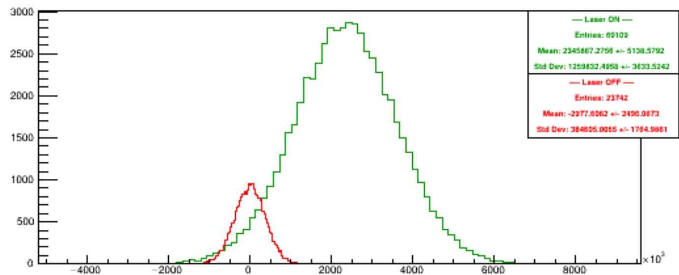
Run 5574 quartetwise, Diffs4
