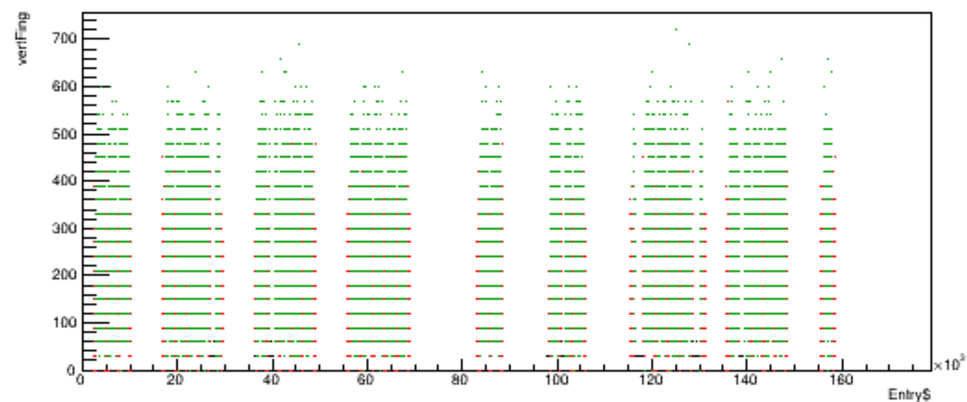
Run 5574 quartetwise, vertFing vs time
