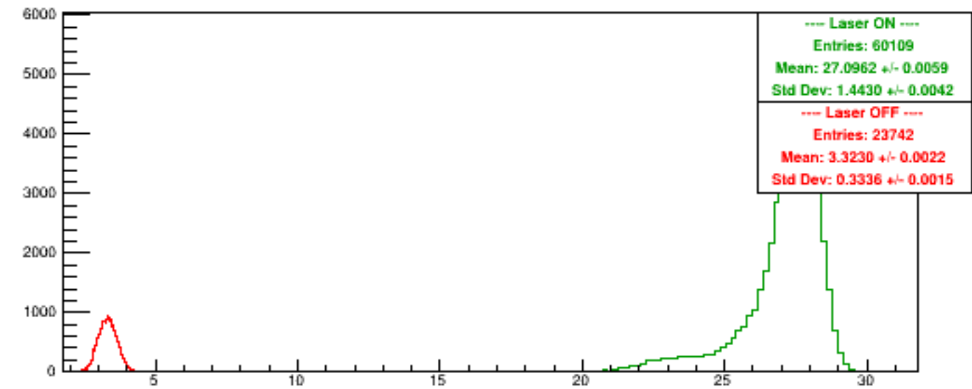
Run 5574 quartetwise, Sums0
