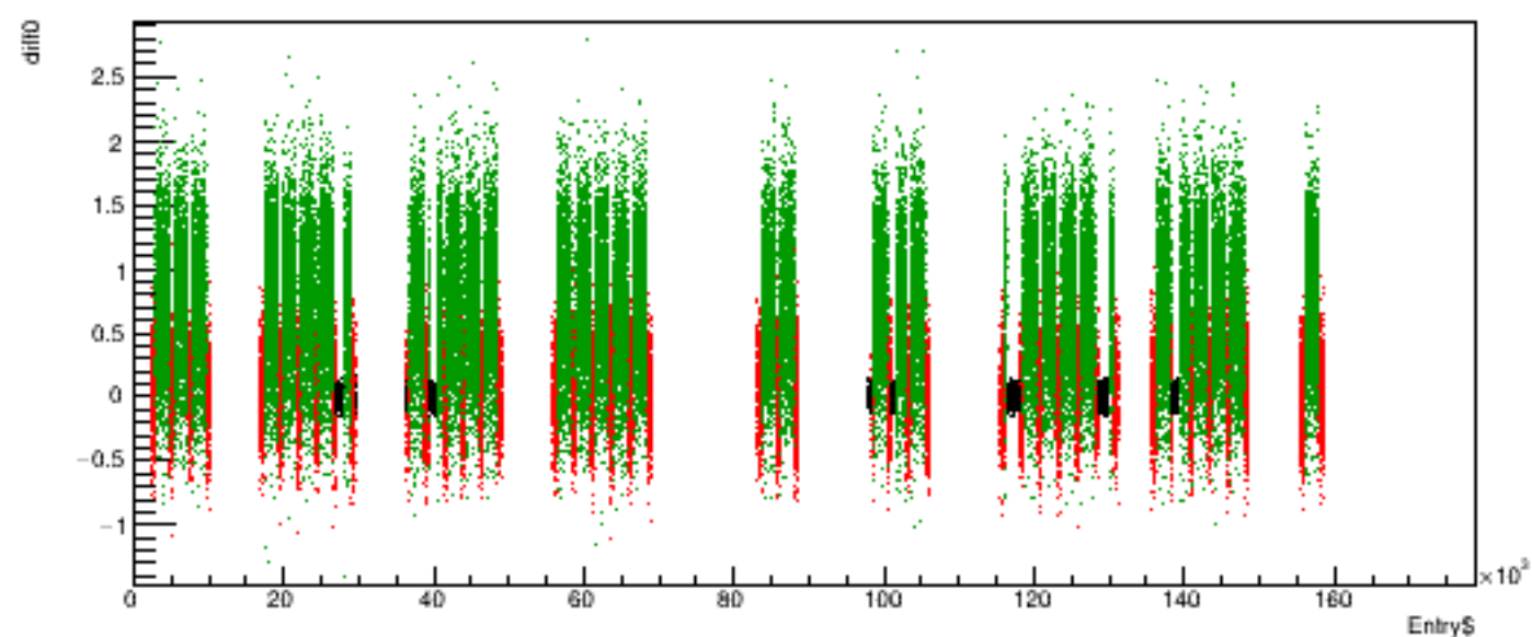
Run 5574 quartetwise, diff0 vs time
