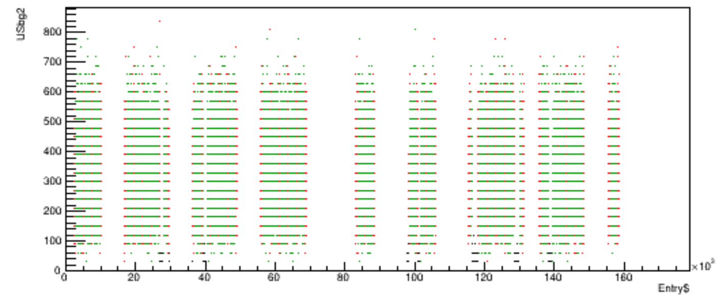
Run 5574 quartetwise, USbg2 vs time
