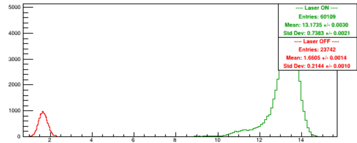
Run 5574 quartetwise, NegHelAcc0/NSamples0
