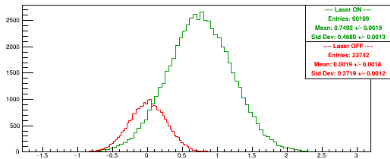
Run 5574 quartetwise, Diffs0
