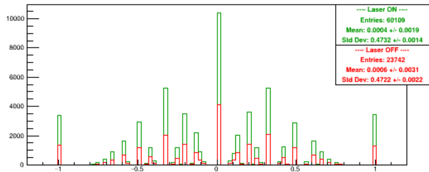
Run 5574 quartetwise, Asyms USbg1
