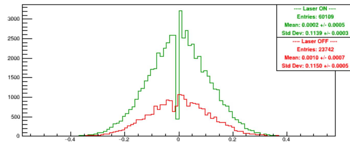
Run 5574 quartetwise, Asyms DSbg2
