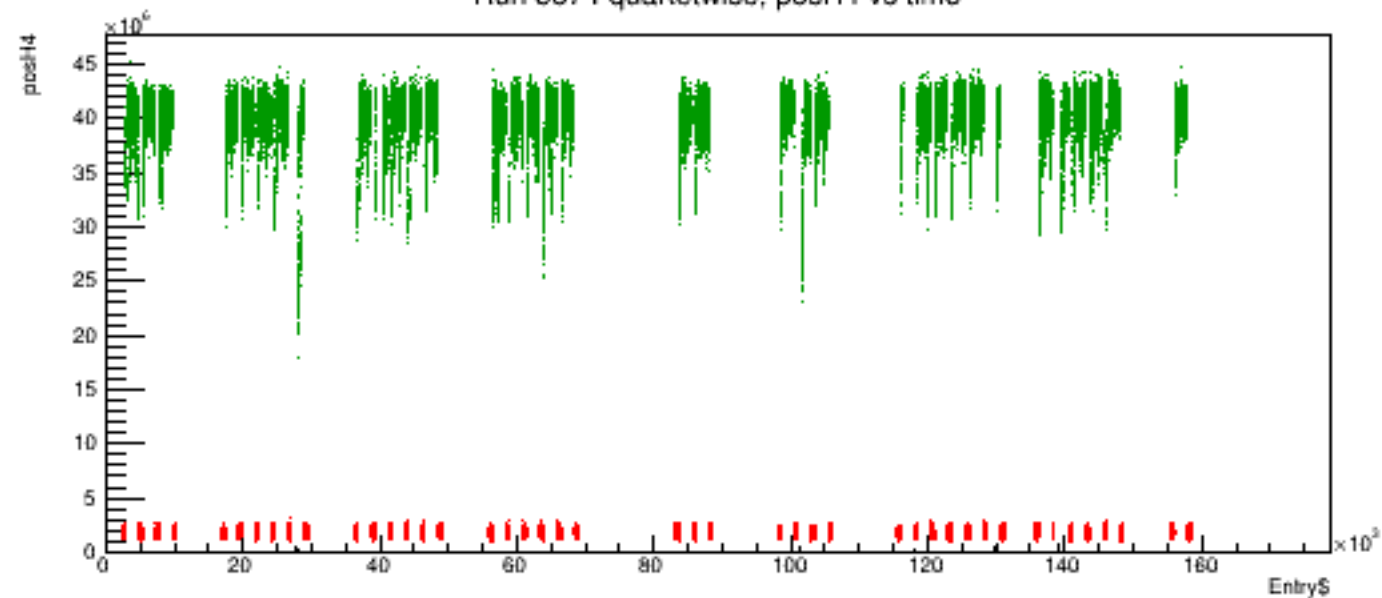
Run 5574 quartetwise, posH4 vs time
