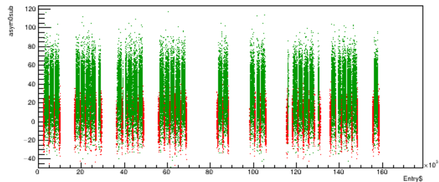
Run 5574 quartetwise, asym0sub vs time
