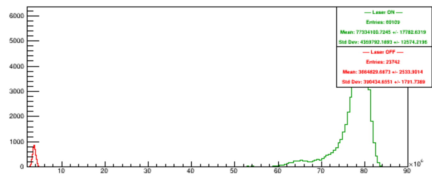
Run 5574 quartetwise, Sums4
