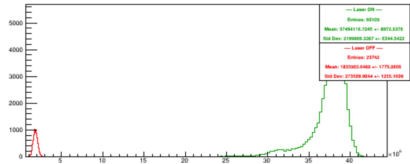
Run 5574 quartetwise, NegHelAcc4
