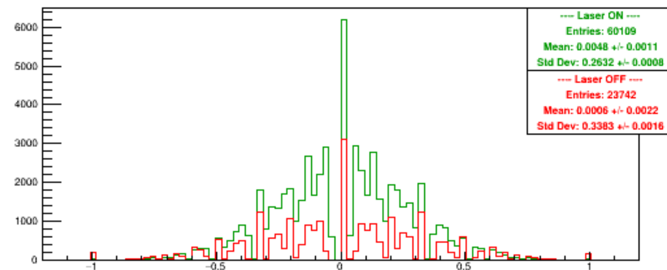
Run 5574 quartetwise, Asyms Vert Finger
