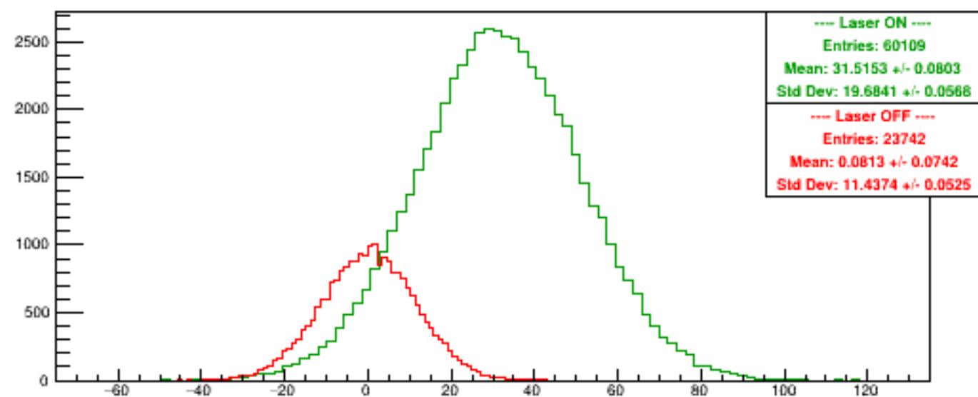
Run 5574 quartetwise, Asyms0
