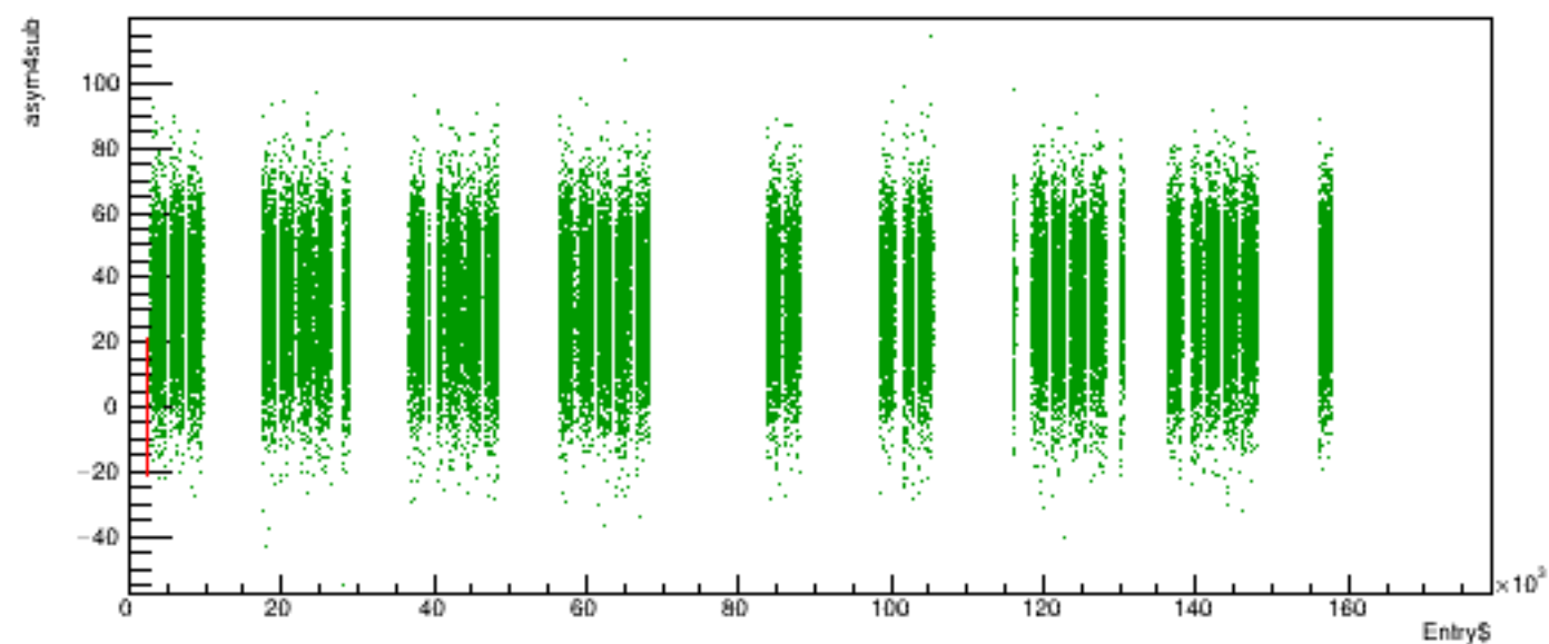
Run 5574 quartetwise, asym4sub vs time
