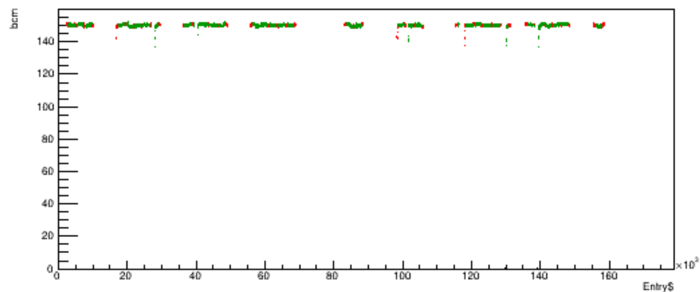
Run 5574 quartetwise, posH4 vs time
