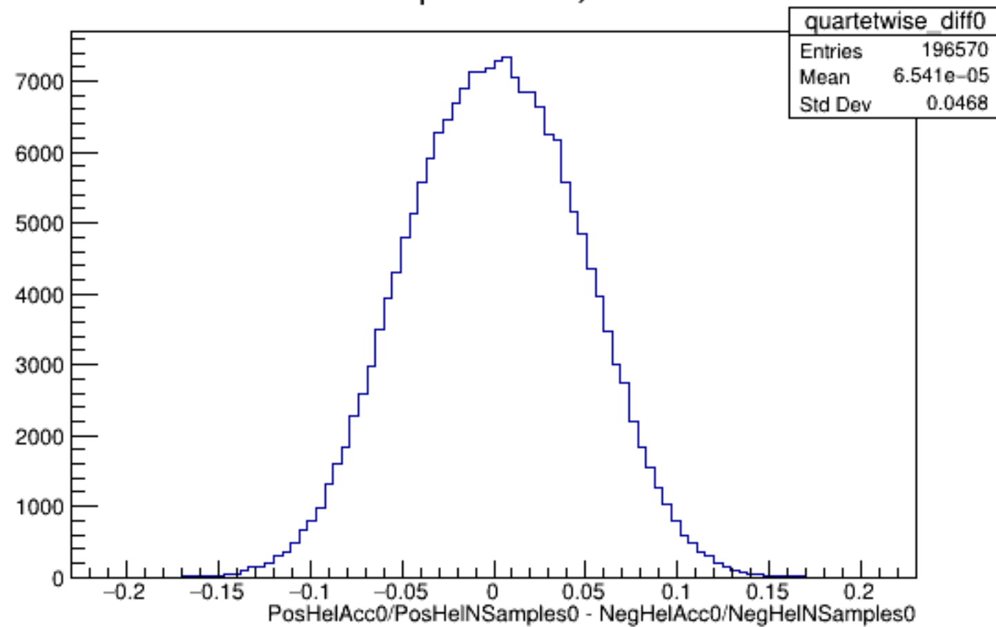
Run 5576 quartetwise, Diffs0: All
