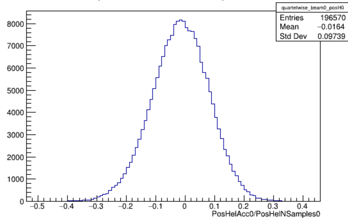
Run 5576 quartetwise, PosHelAcc0/NSamples0: Beam OFF
