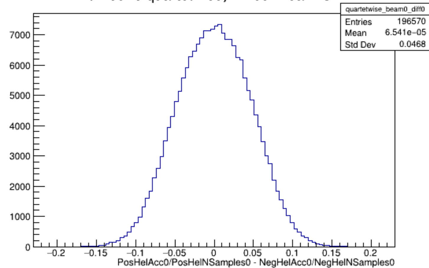
Run 5576 quartetwise, Diffs0: Beam OFF
