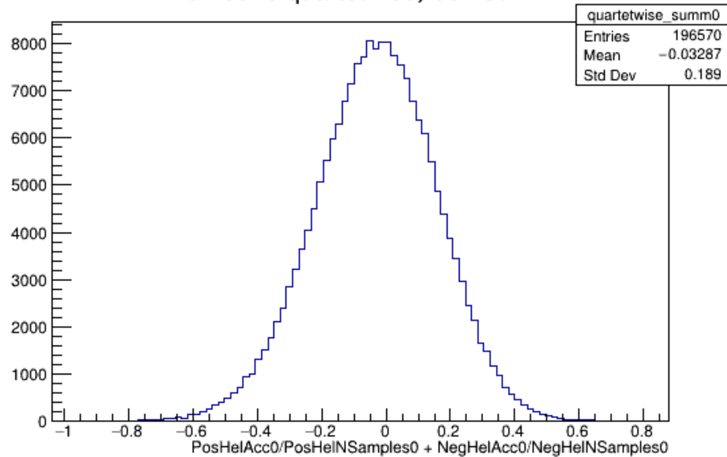
Run 5576 quartetwise, Sums0: All
