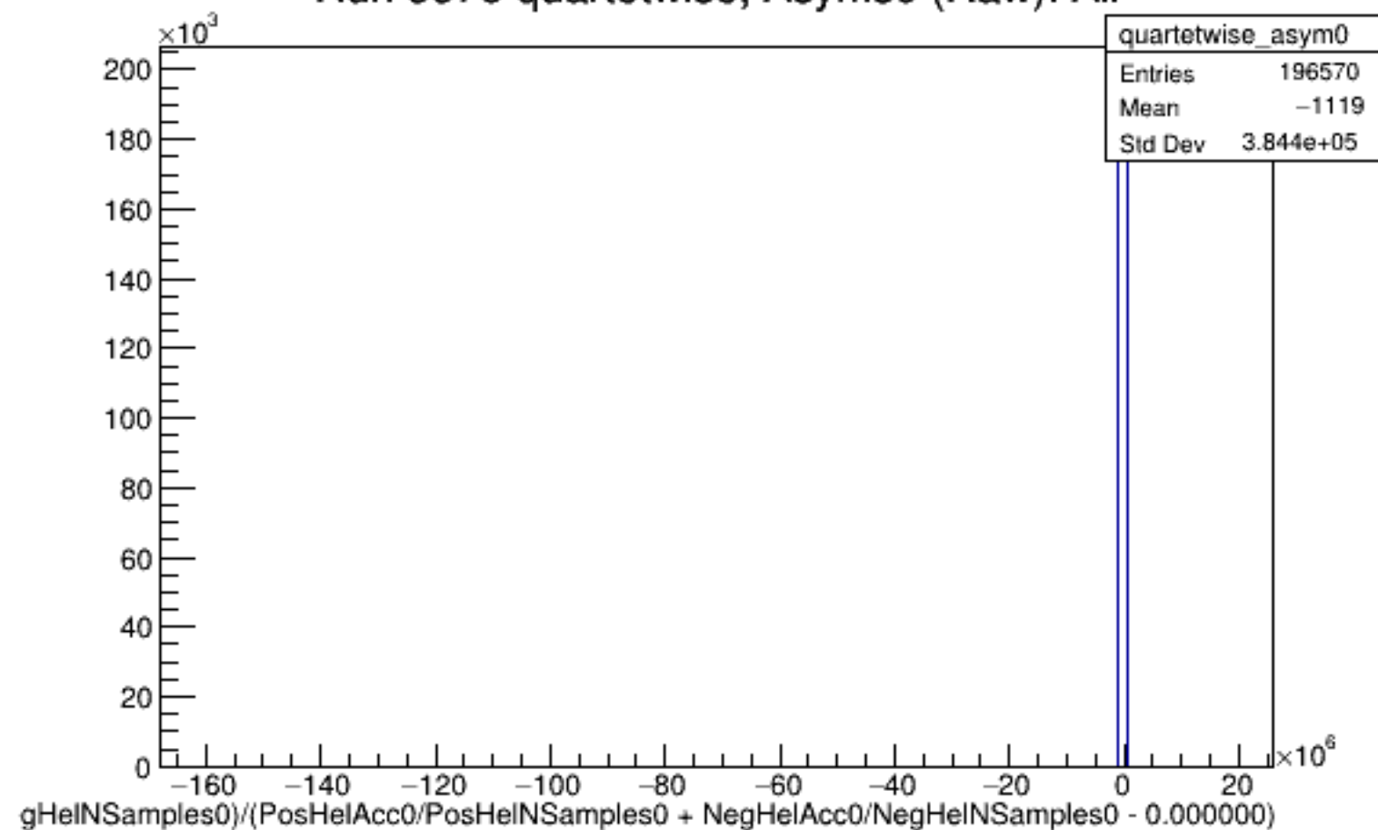
Run 5576 quartetwise, Asyms0 (Raw): All
