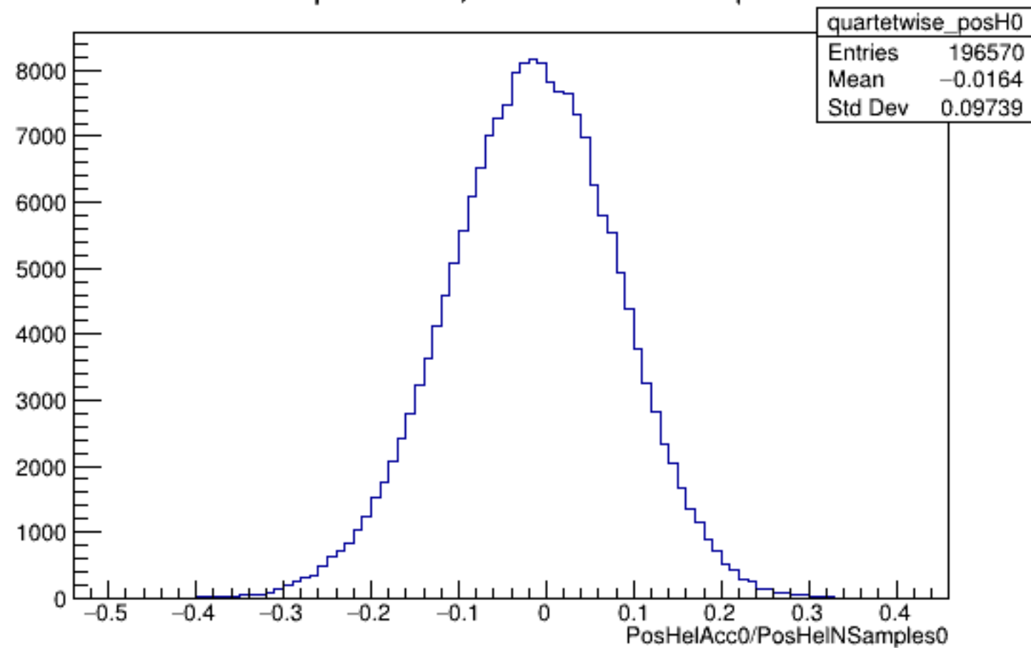
Run 5576 quartetwise, PosHelAcc0/NSamples0: All
