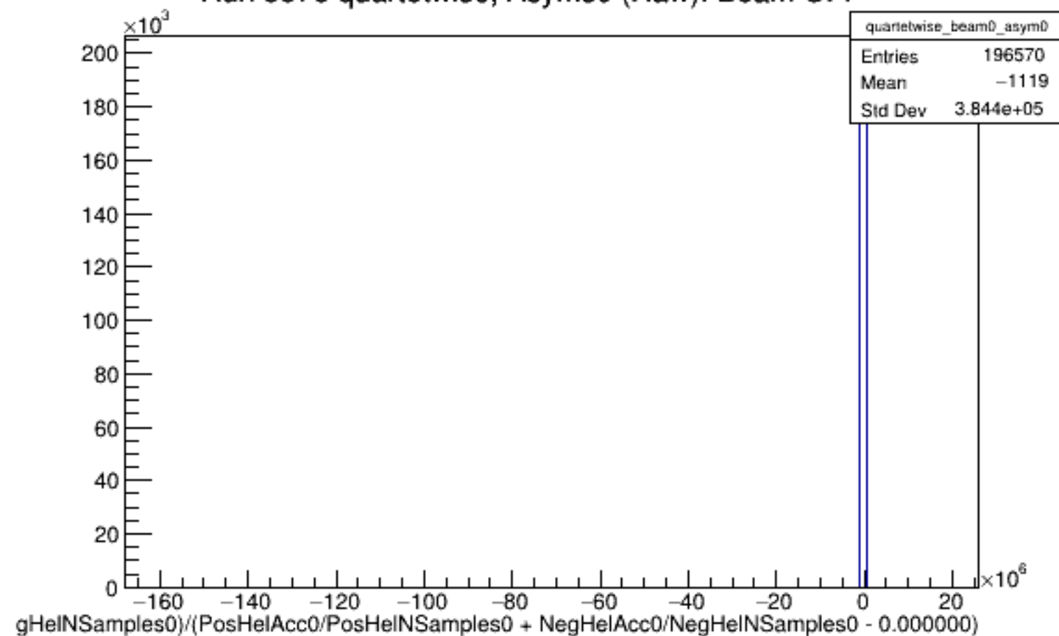
Run 5576 quartetwise, Asyms0 (Raw): Beam OFF
