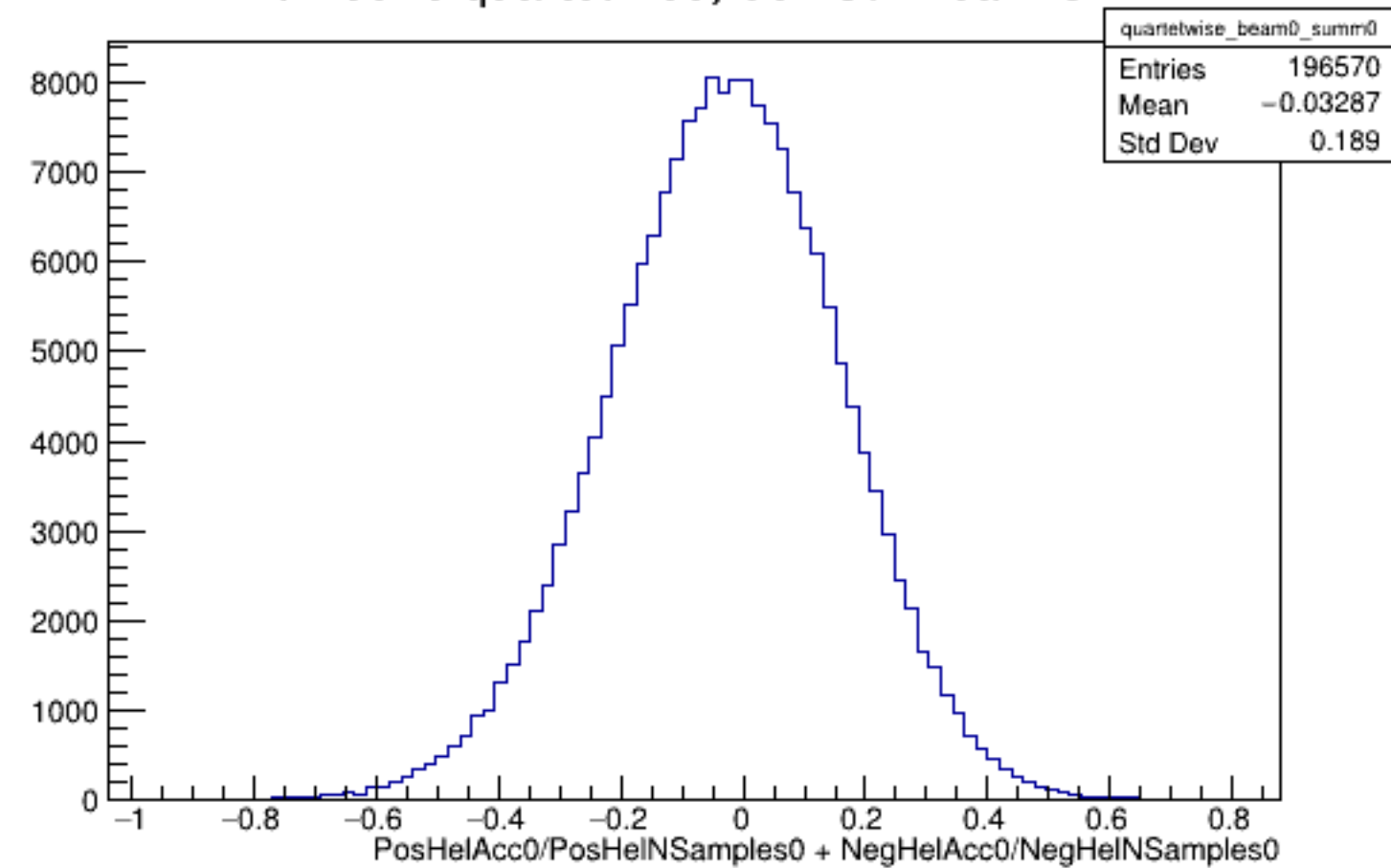
Run 5576 quartetwise, Sums0: Beam OFF
