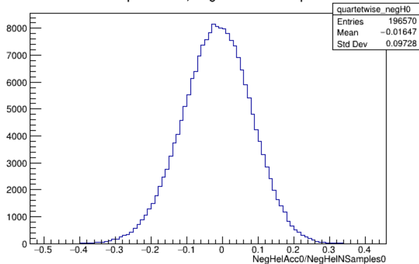
Run 5576 quartetwise, NegHelAcc0/NSamples0: All
