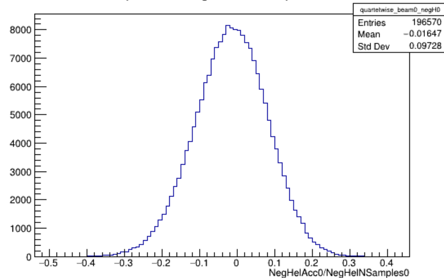
Run 5576 quartetwise, NegHelAcc0/NSamples0: Beam OFF
