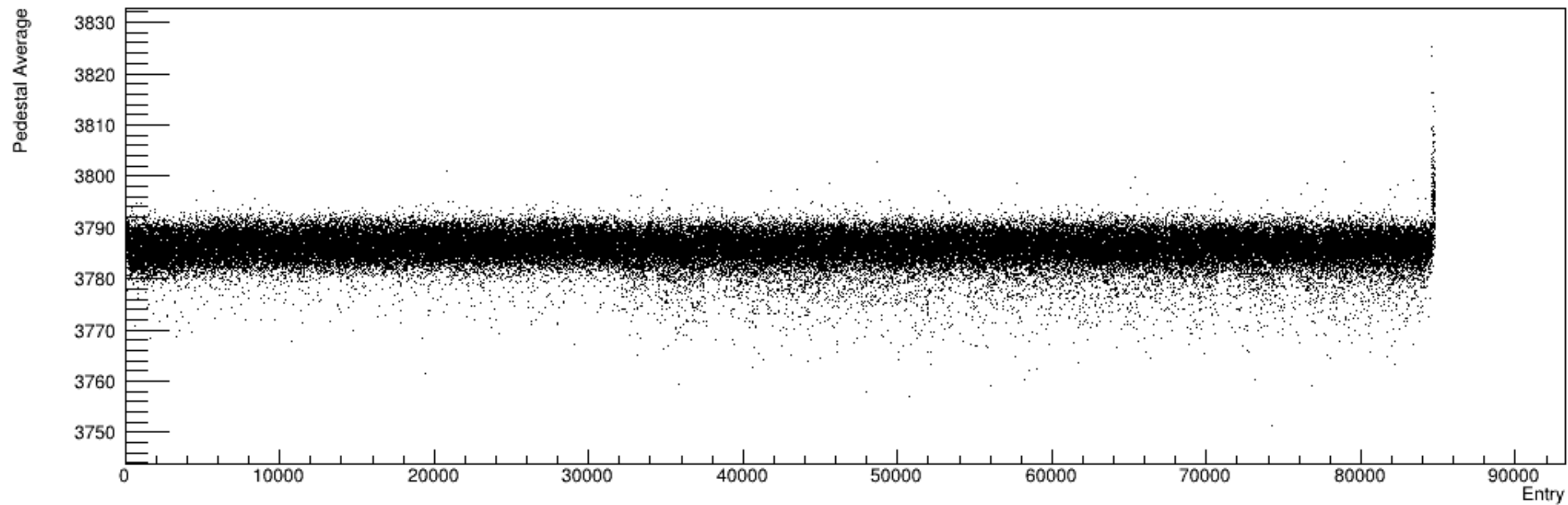
Run 5579, snapshots: Pedestal vs. Time
